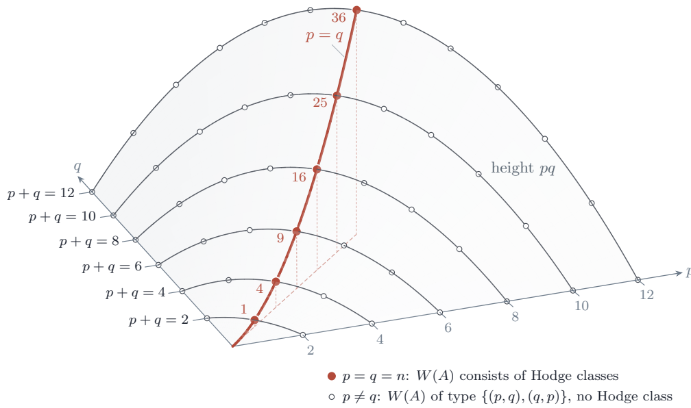
FIGURE 66. The signatures (p, q) of an imaginary quadratic action, with p + q = \dim A , drawn on the surface of height pq , which is the dimension of the family of abelian varieties carrying that action, the unitary Shimura variety of signature (p, q) . Each curve on the surface collects the signatures available in one dimension, and on it the diagonal point is the highest. The divisibility conditions of Theorem C.3 put no constraint on which of them occur when \text{End}^0(A) = K , by Proposition C.9(i) . By Proposition C.7 the Weil line consists of Hodge classes exactly at the filled points on the ridge p = q , and at every open point it is a rational sub-Hodge structure of type \{(p, 2n - p), (2n - p, p)\} carrying no Hodge class at all. The diagonal is the locus that Corollary B.9 shows to be an algebraic subvariety of the moduli.
