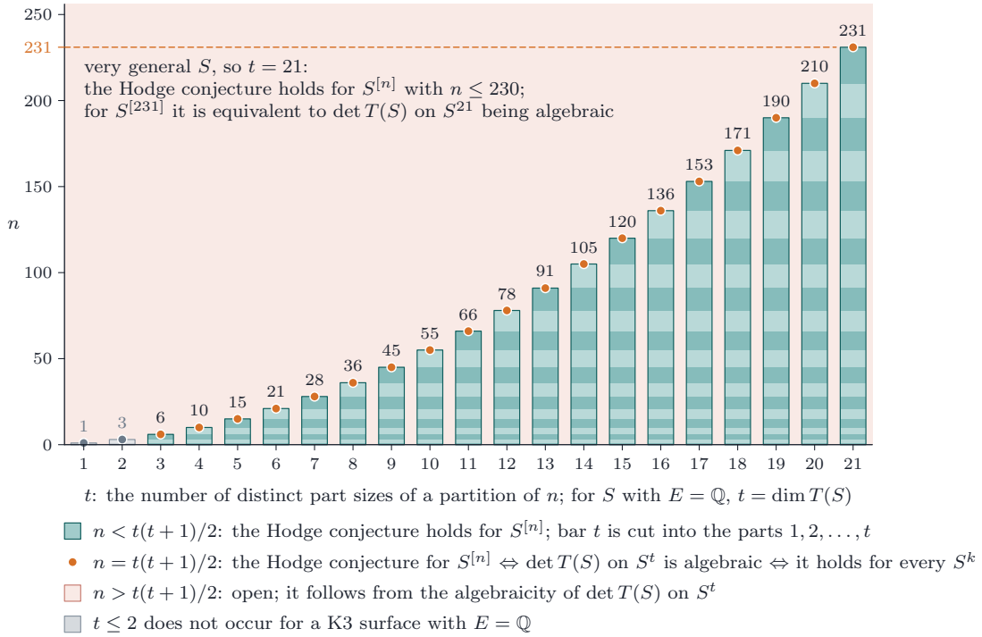
FIGURE 43. The threshold of Proposition 20.39(ii). For t = 1, \dots, 21 the bar rises to t(t+1)/2 , the least n that has a partition with t distinct part sizes, and is cut into the parts 1, 2, \dots, t of the partition that attains it. For a K3 surface S with E = \text{End}_{\text{Hdg}}(T(S)) = \mathbb{Q} and t = \dim T(S) , which is at least 3, the Hodge conjecture holds for S^{[n]} with n below the bar; at its top it is equivalent to the algebraicity of the class \det T(S) on S^t of Proposition 20.38, and to the Hodge conjecture for every power of S ; above it, it follows from that algebraicity. A very general S has t = 21 : the conjecture holds for S^{[n]} with n \leq 230 , and for S^{[231]} it is equivalent to the algebraicity of \det T(S) on S^{21} , one of the frontier cases of (F3') (Remark 20.67).
