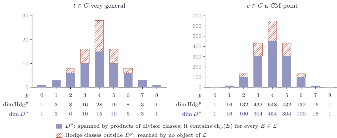
FIGURE 61. Theorem 21.36(ii). The Hodge classes of X_t \times X_t degree by degree, against the subring D^p generated by divisor classes, which contains the Chern character of every object of \mathcal{L} : at a very general point of the Mumford curve (left) and at a CM point (right). The hatched classes, the exceptional ones among them, are reached by no object of \mathcal{L} .
