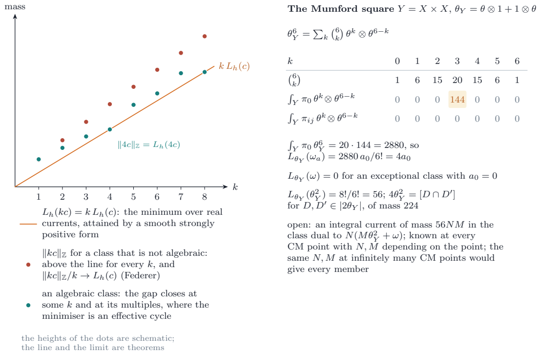
FIGURE 54. Theorem 20.77 and Example 20.78 . Left: the mass of a current in the class dual to kc against k . The line k L_h(c) is the minimum over closed real normal currents, attained by a smooth strongly positive form; the minima over closed integral currents lie on or above it, with \|kc\|_{\mathbb{Z}}/k \rightarrow L_h(c) by Federer's theorem, and for M large the class is algebraic exactly when one of them lies on the line, where the minimiser is an effective algebraic cycle. The heights of the dots are schematic. Right: the numbers of the Mumford square, in the split model. Of the seven terms \binom{6}{k} \theta^k \otimes \theta^{6-k} of \theta_Y^6 only k = 3 pairs with \pi_0 = \frac{1}{4} \theta \otimes \theta , giving 20 \cdot 144 = 2880 , and none pairs with the primitive summands; so L_{\theta_Y}(\omega_a) = 4a_0 , the Wirtinger bound of an exceptional class with a_0 = 0 is zero, and the perturbation of NM\theta_Y^2 by N\omega changes the bound 56NM by nothing.
