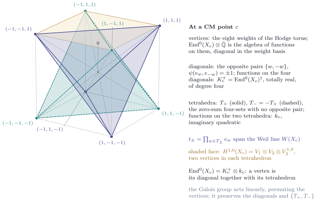
FIGURE 57. Proposition 21.29(i). The eight weights (\pm 1, \pm 1, \pm 1) of the Hodge torus at a CM point are the vertices of a cube. The four diagonals are the pairs of opposite weights, paired by the polarisation; the two inscribed tetrahedra T_+ (an even number of entries -1 ) and T_- = -T_+ are the only zero-sum four-sets without an opposite pair, and t_{\pm} = \prod_{w \in T_{\pm}} e_w span the Weil line. The Galois group acts by linear maps permuting the vertices, so it preserves the diagonals and the pair of tetrahedra: the functions constant on the tetrahedra form the imaginary quadratic Weil field k_c , those constant on the diagonals the totally real quartic algebra K_c^+ of Rosati-fixed endomorphisms, and \text{End}^0(X_c) = K_c^+ \otimes k_c because a vertex is determined by its diagonal and its tetrahedron.
