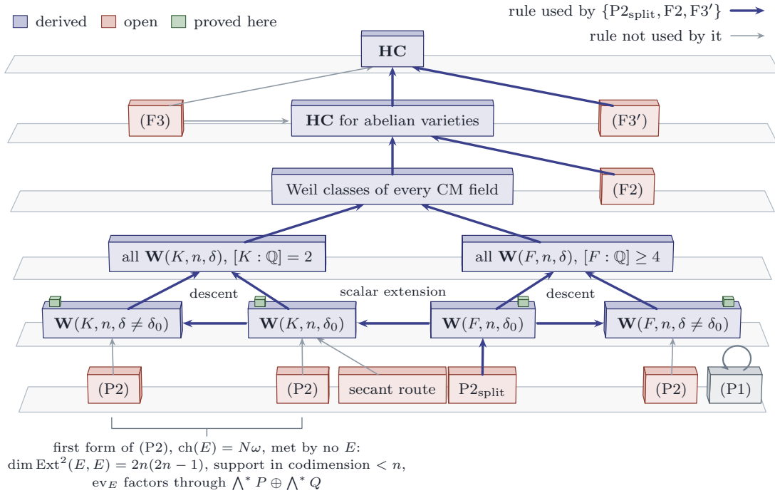
FIGURE 53. The route of this paper through the rule set of Theorem 20.69 , drawn as a stack of plates, one per level of the derivation; the other routes are drawn in Figure 52 . Heavy arrows are the rules used by the minimal set \{P2_{\text{split}}, F2, F3'\} , light arrows the rules it does not use. The bottom plate carries the propagation statement, read in the polarised form of Remark 17.6 , once for each of the four kinds of Weil family, with the secant route beside it. The small grass blocks on the next plate are the base points of Theorem 15.27 and Theorem 19.5 , one in every family. The three arrows inside that plate are Proposition 20.13 : descent from the trivial discriminant to the others, and scalar extension from the fields of degree at least four to the quadratic fields. With them (P2) is needed only for the split families of the fields of higher degree, and the other three (P2) blocks are not used. (F2) is the conjecture for the Hodge classes that no Weil line reaches, and (F3) is the whole conjecture ( Proposition 20.33 ), so the route is minimal only with (F3) replaced by (F3') of Definition 20.34 . The bracket under the two quadratic (P2) blocks records the first form of the criterion, in which the Chern character is exactly a Weil class, as Theorem 16.37 , Theorem 16.39 and Corollary 16.35 describe it; by Theorem 17.5 that form is met by no complex. The secant route reaches the trivial discriminant, since the member it is built on is split, and through descent the rest of the quadratic case; it has no edge to the fields of higher degree. The bounded criterion (P1) stands apart, closed on itself: it is equivalent to its own conclusion.
