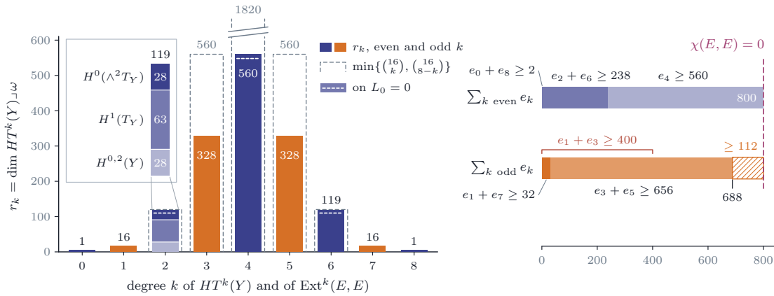
FIGURE 60. Theorem 21.34 . Left: the lower bounds r_k for \dim \text{Ext}^k(E, E) when \text{ch}(E) = N\omega , one bar per degree, symmetric about k = 4 as Lemma 21.33 predicts; the bar at k = 2 is the 119 of Theorem 21.21 , made of 28 classes in H^{0,2} , 63 in H^1(T) and 28 bivectors. On the hyperplane L_0 = 0 the bars at 2, 4 and 6 drop to 110, 548 and 110 at a sample point. Right: \chi(E, E) = 0 balances the even and the odd degrees, so the odd side, which Hochschild cohomology fills only to 688, carries at least 800.
