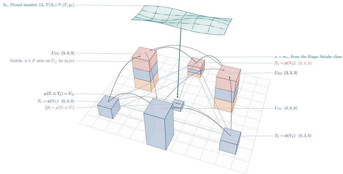
FIGURE 55. Proposition 21.2 and Lemma 21.3, drawn over the triangle of the three factors of the Hodge group; every height is a dimension. At the corners stand the summands T_i = \mathfrak{sl}(V_i) of T = \text{Lie } G , banded by Hodge type after the Tate twist T(-1) : blue for (1, 1) , clay for (2, 0) and amber for (0, 2) , so that only T_3 carries the K3 type. On the edges stand the three summands U_{ij} of the primitive part of H^2(X) , of dimension nine, U_{12} of pure type (1, 1) and the other two in three bands of three; in the middle is the line of \theta . The solid arcs are the product map \mu , which carries T_i \otimes T_j onto U_{ij} , and the dashed ones carry T_i \otimes T_i to \mathbb{Q}\theta . The violet arcs are the Galois group permuting the U_{ij} as it permutes the embeddings of F , which is why the two exceptional classes may be taken to be the trace-zero part of a cubic field. Above, the K3 surface S_\lambda of Theorem 21.4, whose Kuga–Satake class, if algebraic, comes down to T as the map \kappa = m_e .
