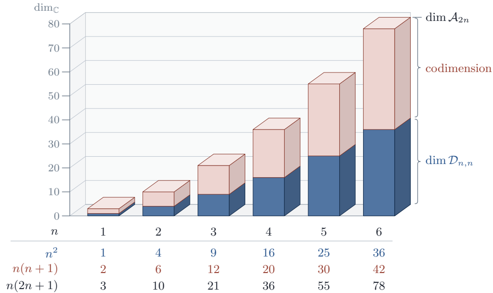
FIGURE 65. The Weil locus inside the moduli of principally polarised abelian 2n -folds, for n = 1, \dots, 6 . Each prism has the height n(2n+1) of the moduli space \mathcal{A}_{2n} ; its lower part, of height n^2 , is the dimension of the period domain \mathcal{D}_{n,n} of Proposition B.8, and its upper part is the codimension n(n+1) . The codimension grows quadratically, so the Weil locus is thin, and by Corollary B.9 it is an algebraic subvariety. Both facts matter for propagation: the locus along which one would have to deform is small and is a variety, but neither fact produces a cycle on it.
