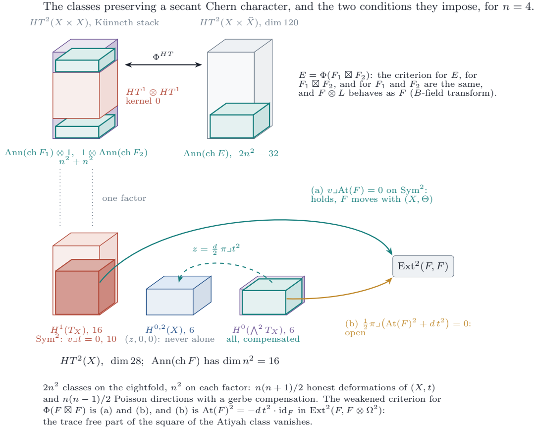
FIGURE 32. Theorem 18.58 for n = 4 . Top: the Künneth stack of HT^2(X \times X) , whose middle summand HT^1 \otimes HT^1 meets the kernel in zero by (i), so that the classes preserving \text{ch}(F_1 \boxtimes F_2) are two copies of the kernel on one factor; across Orlov's isomorphism, HT^2 of the eightfold with the 2n^2 classes preserving \text{ch}(E) . Bottom: HT^2(X) as three slabs with heights proportional to their dimensions, and inside them the n^2 classes of (56): the polarised deformations in front of H^1(T_X) , and the whole of H^0(\wedge^2 T_X) , each bivector tilted into H^{0,2} by its compensation \frac{d}{2} \pi \lrcorner t^2 ; nothing in H^{0,2} alone preserves \text{ch}(F) . On the right, the two conditions that the evaluation map imposes on the two parts, (a) closed by the construction of \mathcal{F} and (b) the identity (58).
