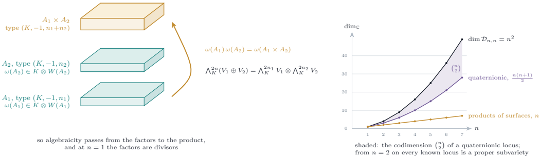
FIGURE 17. Theorem 15.7 and its reach. Left: the Weil line of each factor is a K -line, the Weil line of the product is the tensor product of the two over K , and the K -valued Weil class is multiplicative. Algebraicity therefore passes from the factors to the product, and at n = 1 the factors are divisor classes, so a product of n abelian surfaces of Weil type carries an explicit algebraic Weil class in every dimension. Right: the dimensions of the loci on which the class is known to be algebraic, against the dimension n^2 of the family. Both the quaternionic locus and the product locus are proper subvarieties once n \geq 2 , and a general member lies on neither.
