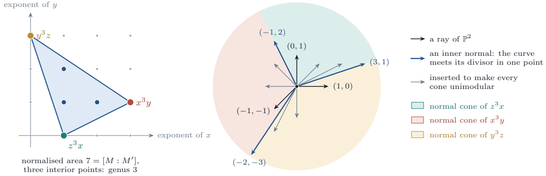
FIGURE 45. The Klein quartic x^3y + y^3z + z^3x in the proof of Theorem 20.52 . Left: its Newton triangle in the lattice M of the torus of \mathbb{P}^2 , in the chart z = 1 , with normalised area 7 = [M : M'] and three interior points, the genus. Right: the rays of a smooth fan adapted to it, the three rays of \mathbb{P}^2 , the three inner normals of the triangle and the six rays inserted to make every cone unimodular. The curve meets only the three divisors of the inner normals, in one point each, the lattice length of the edge, so its Euler number is -7 + 3 = -4 . With e_A = 7 the isogeny of the proof makes it the quotient of the Fermat septic by a group of order seven.
