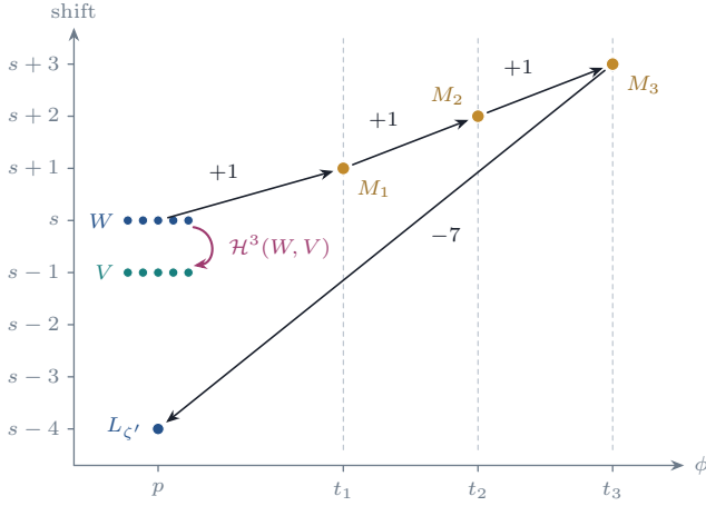
FIGURE 28. Lemma 18.38 and Theorem 18.39, in the placement p < t_1 < t_2 < t_3 . Horizontal: the value \phi of a piece; vertical: its shift. The pieces L_\zeta with \prod \zeta = \epsilon sit at the shift s and the others at s - 1 . A run through the multiples, up three times with Ext degree 0 and down once with Ext degree 8, ends four shifts lower, the least drop of Lemma 18.38(iii), so it never joins a top piece W to a partner V one shift lower; the group \mathcal{H}^3(W, V) survives in \text{Ext}^2(E, E) .
