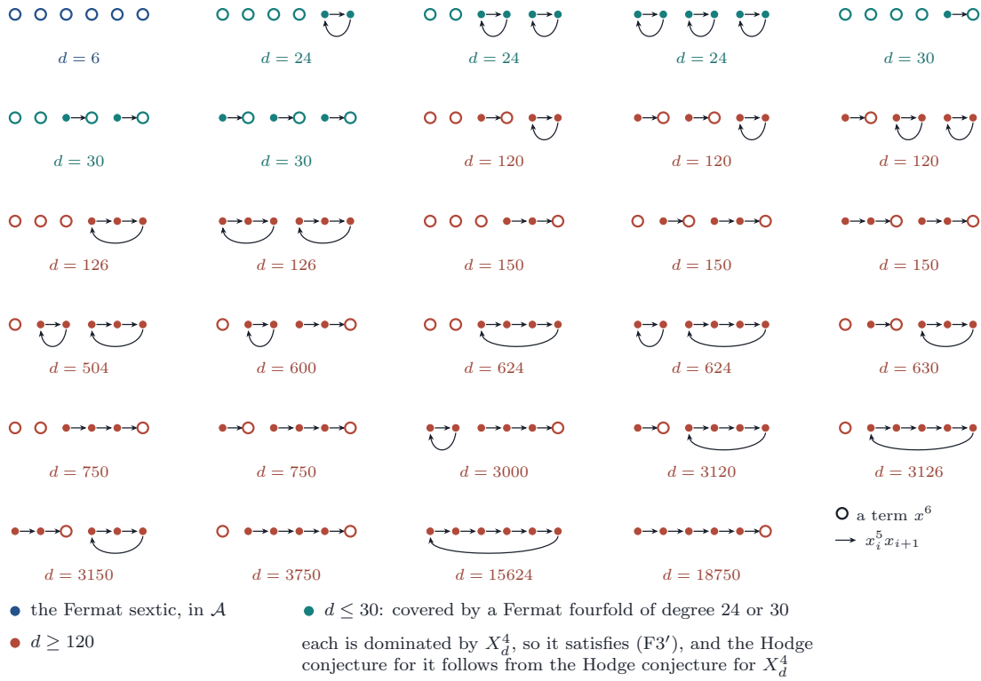
FIGURE 44. The 29 smooth sextic fourfolds of Proposition 20.48(iii), up to a renumbering of the variables. Each is drawn on its six variables: an arrow from x_i to x_j is a term x_i^5 x_j , and a ring is a term x^6 , so a chain is a path of arrows ending at a ring and a loop is a cycle of arrows. Under each is the least d with dA^{-1} integral, the degree of the Fermat fourfold that covers it. All of them satisfy (F3').
