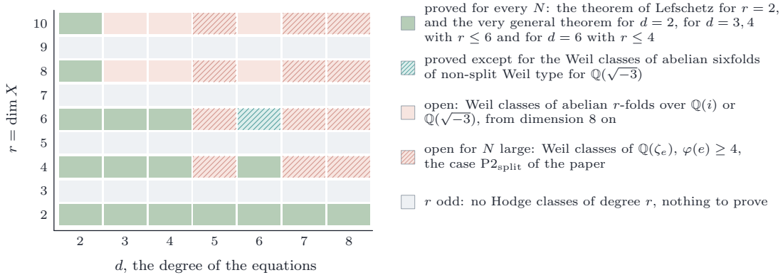
FIGURE 50. The Hodge conjecture for the very general complete intersection X_{d,r}(\lambda) of Vandermonde type, for every N . Grass: proved, by the theorem of Lefschetz for r = 2 and by Theorem 20.65 for d = 2 , for d = 3, 4 with r \leq 6 and for d = 6 with r \leq 4 . Teal hatching: proved except for the Weil classes of abelian sixfolds of non-split Weil type for \mathbb{Q}(\sqrt{-3}) . Clay: open, the Weil classes of abelian varieties of Weil type over \mathbb{Q}(i) or \mathbb{Q}(\sqrt{-3}) in dimension at least eight, or, hatched, of a CM field of degree at least four (Remark 20.66). For odd r there is nothing to prove.
