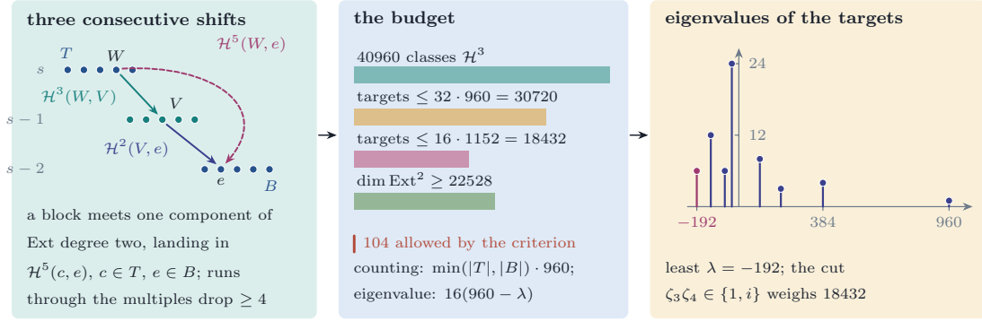
FIGURE 29. Theorem 18.40 . Left: the pieces L_\zeta at three consecutive shifts, those of one parity at s - 1 and the others split between T at s and B at s - 2 ; a group \mathcal{H}^3 between two pieces that differ in three coordinates (teal) can meet a component of Ext degree two (indigo) only in a group \mathcal{H}^5(c, e) with c \in T and e \in B (magenta). Middle: the 40960 classes against the targets, at most 30720 by counting and 18432 by the least eigenvalue, against the 104 that the criterion allows. Right: the eigenvalues of the Cayley graph of the targets.
