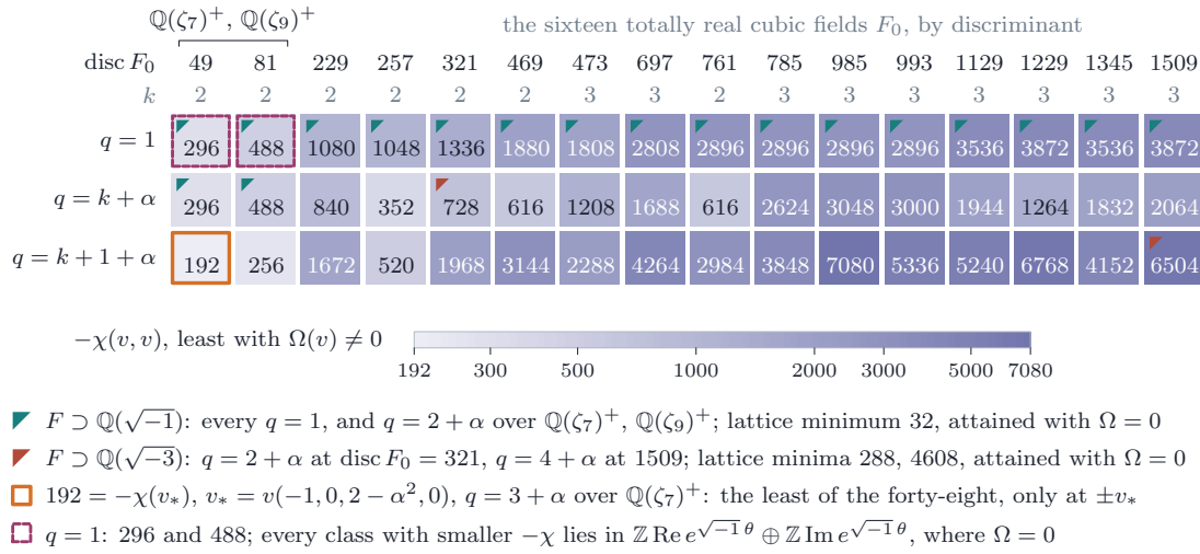
FIGURE 39. Proposition 19.52 case by case. For each of the sixteen totally real cubic fields F_0 of Proposition 19.50(v), ordered by discriminant, and each of q = 1 , k + \alpha and k + 1 + \alpha , the cell gives the least -\chi(v, v) of an integral point v of S(0, q) whose Orlov square has a nonzero F -Weil part, that is with \Omega(v) \neq 0 (Lemma 19.51), as computed in [BMB26]; the shading is logarithmic in this value, which lies between 192 and 7080, and between 296 and 3872 for q = 1 . A corner mark shows that F = F_0(\sqrt{-q}) contains an imaginary quadratic field, \mathbb{Q}(\sqrt{-1}) in eighteen cases and \mathbb{Q}(\sqrt{-3}) in two (Proposition 19.52(ii)); in those cases the lattice has classes of smaller -\chi , namely 32, respectively 288 and 4608, all with \Omega = 0 . The heavy frame marks the least value 192, attained only at \pm v_* over \mathbb{Q}(\zeta_7)^+ with q = 3 + \alpha , the target of Remark 19.53; the dashed frames mark the values 296 and 488 for q = 1 over \mathbb{Q}(\zeta_7)^+ and \mathbb{Q}(\zeta_9)^+ , below which every integral class lies in \mathbb{Z} \operatorname{Re} e^{\sqrt{-1}\theta} \oplus \mathbb{Z} \operatorname{Im} e^{\sqrt{-1}\theta} (Proposition 19.52(iii)). These are least values over the lattices computed, not bounds, and a character does not give a complex.
