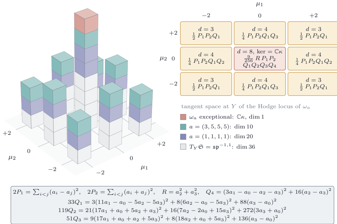
FIGURE 57. Theorem 21.21 . Left: the Siegel space \mathfrak{S} of dimension 36 near Y = X_c \times X_c and three Hodge loci through it, labelled by the tangent dimension T at Y : the class with equal coefficients ( T = 20 ), the products of divisor classes with a_1 = a_2 = a_3 ( T = 10 , the diagonal Siegel space), and a rational exceptional class ( T = 1 ), whose locus is the compact Mumford curve with its CM points (hollow). The dashed rim is the boundary of \mathfrak{S} , which the curve does not reach. Right: the nine weight blocks of \mathfrak{sp}^{-1,1} under the torus of the first two factors, with their dimensions and the forms whose product is the Gram determinant of each; only the block of weight (0, 0) has a kernel, the direction \kappa of the curve. The same holds in the 46 blocks of HT^2(Y) off the hyperplane L_0 = 0 . Below: the sums of squares that make the determinants nonzero at the conjugates of an irrational element of F .
