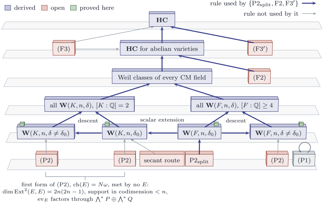
FIGURE 54. The route of this paper through the rule set of Theorem 20.68, drawn as a stack of plates, one per level of the derivation; the other routes are drawn in Figure 53. Heavy arrows are the rules used by the minimal set \{P2_{\text{split}}, F2, F3'\} , light arrows the rules it does not use. The bottom plate carries the propagation statement, read in the polarised form of Remark 17.6, once for each of the four kinds of Weil family, with the secant route beside it. The small grass blocks on the next plate are the base points of Theorem 15.27 and Theorem 19.5, one in every family. The three arrows inside that plate are Proposition 20.13: descent from the trivial discriminant to the others, and scalar extension from the fields of degree at least four to the quadratic fields. With them (P2) is needed only for the split families of the fields of higher degree, and the other three (P2) blocks are not used. (F2) is the conjecture for the Hodge classes that no Weil line reaches, and (F3) is the whole conjecture (Proposition 20.33), so the route is minimal only with (F3) replaced by (F3') of Definition 20.34. The bracket under the two quadratic (P2) blocks records the first form of the criterion, in which the Chern character is exactly a Weil class, as Theorem 16.36, Theorem 16.38 and Corollary 16.34 describe it; by Theorem 17.5 that form is met by no complex. The secant route reaches the trivial discriminant, since the member it is built on is split, and through descent the rest of the quadratic case; it has no edge to the fields of higher degree. The bounded criterion (P1) stands apart, closed on itself: it is equivalent to its own conclusion.
