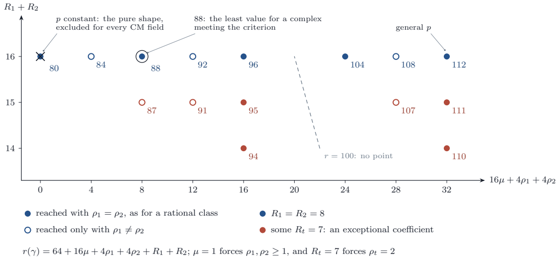
FIGURE 38. The rank r(\gamma) of Theorem 19.29, over the plane of the Hankel part 16\mu + 4\rho_1 + 4\rho_2 and of R_1 + R_2 . The fifteen points are the tuples allowed by the two conditions of the theorem, and each carries its value. Filled points are reached with \rho_1 = \rho_2 , as the character of a complex with rational coefficients is (Corollary 19.30(ii)); red points need an exceptional coefficient at one place at least. The value 80 is the pure shape, excluded for every CM field by Theorem 19.19; so 88 is the least rank a complex meeting the criterion can have. The level r = 100 meets no point.
