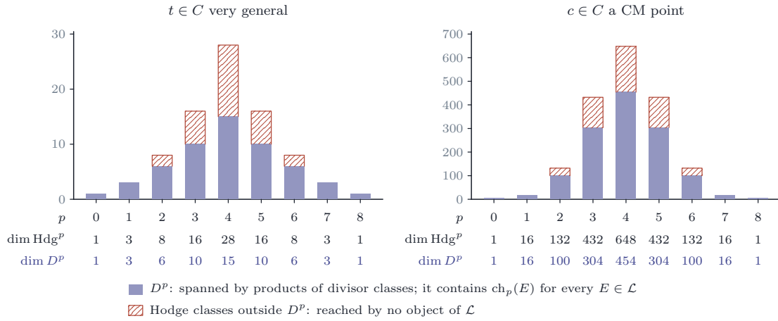
FIGURE 62. Theorem 21.36(ii). The Hodge classes of X_t \times X_t degree by degree, against the subring D^p generated by divisor classes, which contains the Chern character of every object of \mathcal{L} : at a very general point of the Mumford curve (left) and at a CM point (right). The hatched classes, the exceptional ones among them, are reached by no object of \mathcal{L} .
