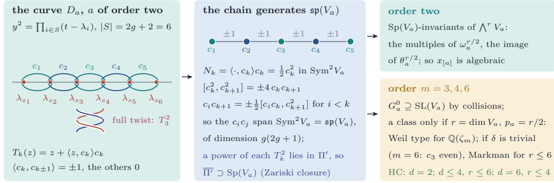
FIGURE 49. The proof of Theorem 20.64 . Left: the hyperelliptic curve D_a of a character of order two, drawn over the six points of its support for g = 2 , with the chain of vanishing cycles c_1, \dots, c_5 ; a full twist of two neighbouring branch points, drawn as a braid, acts by the square of the transvection T_k . Middle: the chain as a graph, and the induction in \text{Sym}^2 V_a by which the logarithms N_k generate \mathfrak{sp}(V_a) . Right: what the monodromy leaves of the Hodge classes, the powers of the polarisation for characters of order two, and for characters of order three, four and six the Weil classes of an abelian variety of Weil type for \mathbb{Q}(\sqrt{-3}) or \mathbb{Q}(i) .
