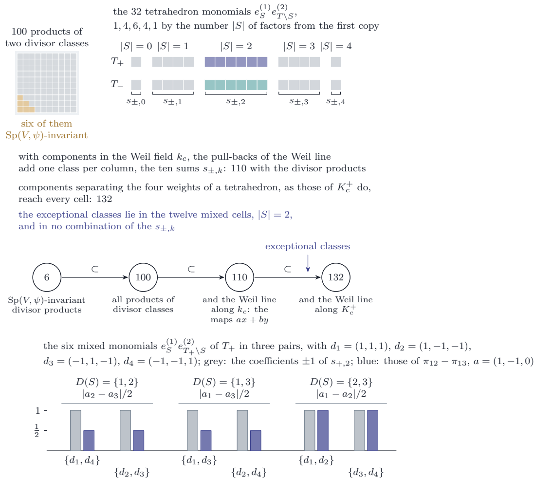
FIGURE 59. Proposition 21.29(ii) and (iii). Top: the 132 Hodge classes of degree four on the square at a CM point, one cell per monomial of weight zero. The 100 products of divisor classes are the cells with an opposite pair; the 32 tetrahedron monomials e_S^{(1)} e_{T \setminus S}^{(2)} are arranged by tetrahedron and by the number |S| of factors from the first copy. Pull-backs of the Weil line along homomorphisms with components in k_c add only the ten symmetric sums s_{\pm,k} , one per column, giving 110; components separating the four weights of a tetrahedron, as those of K_c^+ do, separate the monomials and give all 132. Bottom: on the six mixed monomials of one tetrahedron, grouped in the three pairs by the coordinates in which the two weights of S differ, the symmetric sum s_{+,2} has coefficients \pm 1 throughout, while an exceptional class \omega_a has coefficients of absolute value |a_2 - a_3|/2 , |a_1 - a_3|/2 , |a_1 - a_2|/2 , drawn for \pi_{12} - \pi_{13} ; two equal absolute values would be a linear relation among the conjugates of an irrational element of F .
