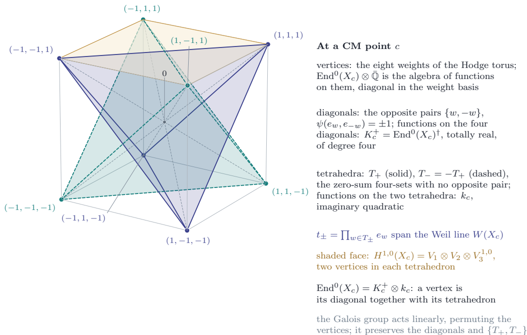
FIGURE 58. Proposition 21.29(i) . The eight weights (\pm 1, \pm 1, \pm 1) of the Hodge torus at a CM point are the vertices of a cube. The four diagonals are the pairs of opposite weights, paired by the polarisation; the two inscribed tetrahedra T_+ (an even number of entries -1 ) and T_- = -T_+ are the only zero-sum four-sets without an opposite pair, and t_{\pm} = \prod_{w \in T_{\pm}} e_w span the Weil line. The Galois group acts by linear maps permuting the vertices, so it preserves the diagonals and the pair of tetrahedra: the functions constant on the tetrahedra form the imaginary quadratic Weil field k_c , those constant on the diagonals the totally real quartic algebra K_c^+ of Rosati-fixed endomorphisms, and \text{End}^0(X_c) = K_c^+ \otimes k_c because a vertex is determined by its diagonal and its tetrahedron.
