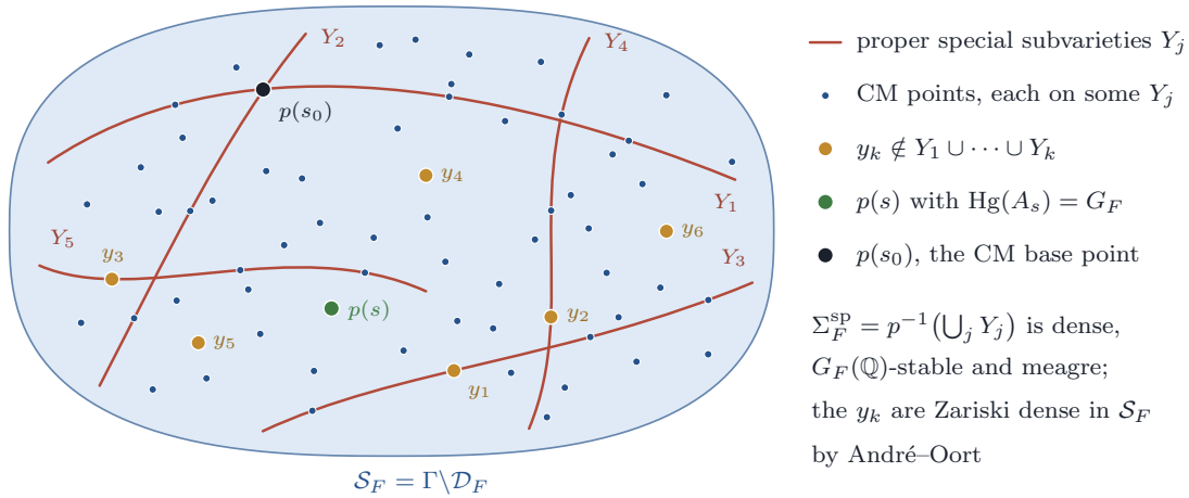
FIGURE 36. Proposition 19.12 and Theorem 19.14 on the quotient \mathcal{S}_F . The curves are five of the countably many proper special subvarieties Y_j , whose union is the image of the special locus; it contains p(s_0) and is dense and meagre. The small dots are CM points, each lying on some Y_j , drawn or not. The points y_1, \dots, y_6 begin an escaping sequence chosen as in the proof of Theorem 19.14(i) : y_k lies on no Y_j with j \leq k , so y_1 may lie on Y_3 and y_2 on Y_4 . A point p(s) at which the Hodge group is all of G_F lies on none of them.
