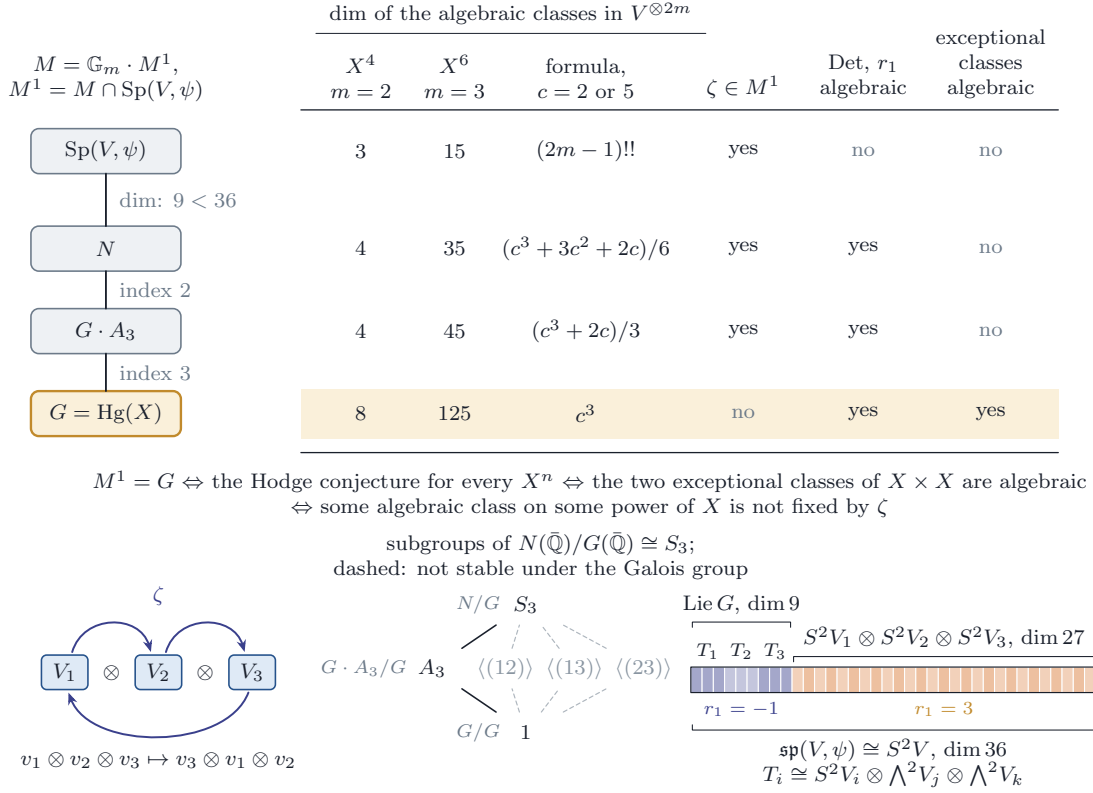
FIGURE 63. The four possible groups M^1 = M \cap \mathrm{Sp}(V, \psi) of Proposition 21.47, where M = \mathbb{G}_m \cdot M^1 , as the chain G \subset G \cdot A_3 \subset N \subset \mathrm{Sp}(V, \psi) : the first two inclusions have index 3 and 2, and N , whose identity component is G , has dimension 9 against 36. For each case the table gives the dimension of the algebraic classes in the multilinear part V^{\otimes 2m} of H^{2m}(X^{2m}, \mathbb{Q}) for m = 2 and m = 3 , from the c = 2 , respectively c = 5 , non-crossing pairings (a computation in [BMB26]); whether M^1 contains the cyclic permutation \zeta of the three tensor factors; whether Det and r_1 are algebraic; and whether the two exceptional classes of X \times X are. Only M^1 = G makes the exceptional classes algebraic, and it is equivalent to the Hodge conjecture for every power of X (Proposition 21.47(ii)); the proposition does not decide which of the four cases occurs. Below, from left to right: \zeta ; the subgroups of N(\bar{\mathbb{Q}})/G(\bar{\mathbb{Q}}) \cong S_3 , of which only 1, A_3 and S_3 are stable under the Galois group, which acts transitively on the three factors; and \mathfrak{sp}(V, \psi) = \mathrm{Lie} G \oplus S^2 V_1 \otimes S^2 V_2 \otimes S^2 V_3 , 36 = 9 + 27 , the second summand irreducible under G , with the eigenvalues -1 and 3 of r_1 on the two summands.
