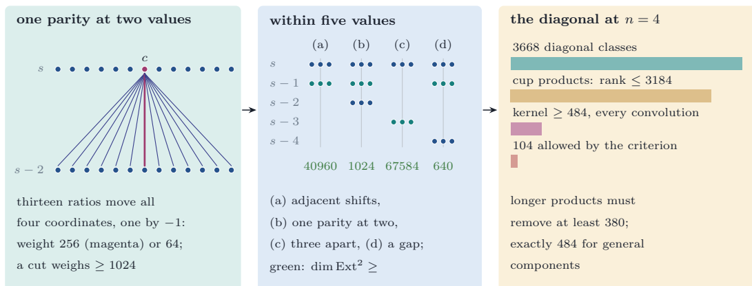
FIGURE 31. The shift arrangements of the pieces L_\zeta on E_0^8 . Left: one parity at two values two apart; a piece c is joined to the thirteen pieces whose ratio moves every coordinate, one by -1 , and the groups \mathcal{H}^4 of the edges crossing between the values survive, weighing at least 1024 (Lemma 18.41(ii), Lemma 18.42). Middle: the four kinds of arrangement within five consecutive values, with the result that excludes each and its bound on \dim \text{Ext}^2 . Right: the diagonal at n = 4 ; the cup products leave at least 484 of the 3668 classes, and the criterion allows 104 (Proposition 18.51).
