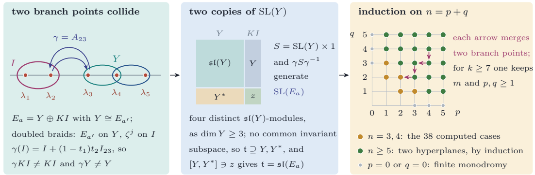
FIGURE 48. The proof of Proposition 20.62. Left: two branch points \lambda_1, \lambda_2 collide inside a disc (Lemma 20.59); the cycles outside the disc form the hyperplane Y \cong E_{a'} , the cycle I of the disc spans the complementary line, and the twist \gamma of the second and third points moves both. Middle: the two copies of SL(Y) of Lemma 20.60 generate SL(E_a) . Right: the induction on n = k - 2 , each merge lowering p or q by one (Lemma 20.61), down to the 38 computed cases with n = 3, 4 .
