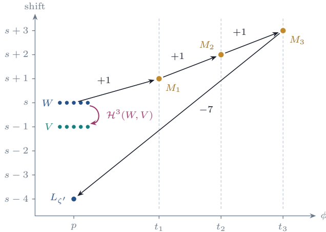
FIGURE 29. Lemma 18.38 and Theorem 18.39, in the placement p < t_1 < t_2 < t_3 . Horizontal: the value \phi of a piece; vertical: its shift. The pieces L_\zeta with \prod \zeta = \epsilon sit at the shift s and the others at s - 1 . A run through the multiples, up three times with Ext degree 0 and down once with Ext degree 8, ends four shifts lower, the least drop of Lemma 18.38(iii), so it never joins a top piece W to a partner V one shift lower; the group \mathcal{H}^3(W, V) survives in \text{Ext}^2(E, E) .
