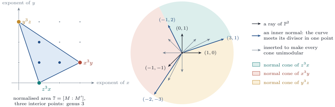
FIGURE 46. The Klein quartic x^3y + y^3z + z^3x in the proof of Theorem 20.51 . Left: its Newton triangle in the lattice M of the torus of \mathbb{P}^2 , in the chart z = 1 , with normalised area 7 = [M : M'] and three interior points, the genus. Right: the rays of a smooth fan adapted to it, the three rays of \mathbb{P}^2 , the three inner normals of the triangle and the six rays inserted to make every cone unimodular. The curve meets only the three divisors of the inner normals, in one point each, the lattice length of the edge, so its Euler number is -7 + 3 = -4 . With e_A = 7 the isogeny of the proof makes it the quotient of the Fermat septic by a group of order seven.
