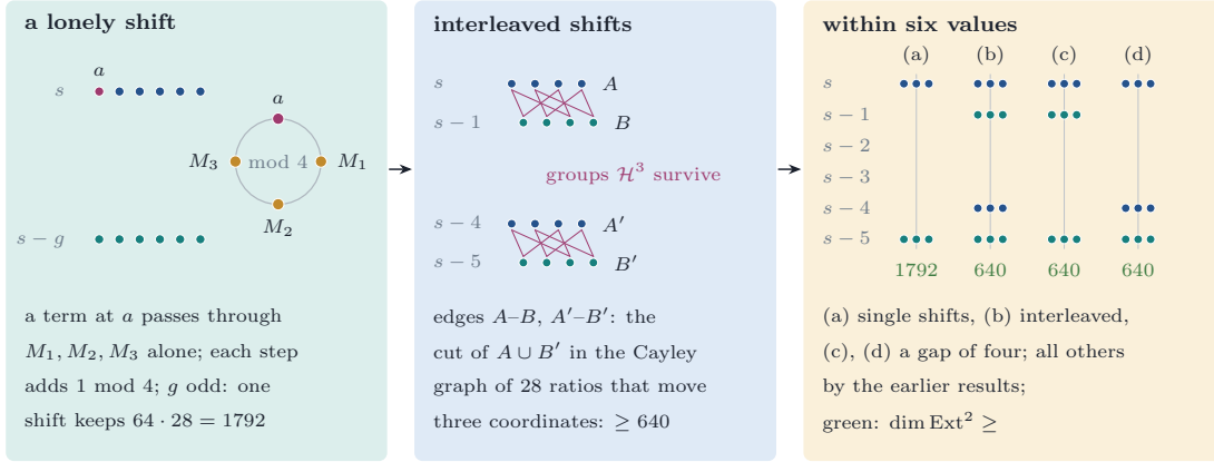
FIGURE 32. The arrangements within six consecutive values on E_0^8 . Left: the parities at single shifts s and s-g , g odd and at least five; a term on a diagonal class at a piece a runs through M_1, M_2, M_3 and no other piece, and since each step adds one to the shift modulo 4 the four nodes have distinct residues, so the multiples serve at most one of the two shifts and the 1792 diagonal classes at the other survive (Lemma 18.47, Proposition 18.48). Middle: the interleaved shifts; the groups \mathcal{H}^3 between A and B and between A' and B' survive and form a cut of the Cayley graph of the 28 ratios that move three coordinates, of weight at least 640 (Proposition 18.49). Right: the four arrangements left within six values by the results for five values, each with its bound on \dim \text{Ext}^2 (Corollary 18.50).
