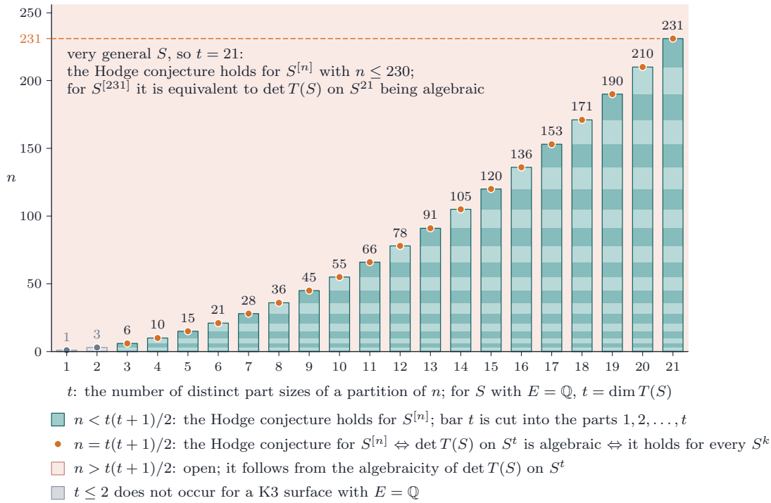
FIGURE 44. The threshold of Proposition 20.39(ii). For t = 1, \dots, 21 the bar rises to t(t+1)/2 , the least n that has a partition with t distinct part sizes, and is cut into the parts 1, 2, \dots, t of the partition that attains it. For a K3 surface S with E = \text{End}_{\text{Hdg}}(T(S)) = \mathbb{Q} and t = \dim T(S) , which is at least 3, the Hodge conjecture holds for S^{[n]} with n below the bar; at its top it is equivalent to the algebraicity of the class \det T(S) on S^t of Proposition 20.38, and to the Hodge conjecture for every power of S ; above it, it follows from that algebraicity. A very general S has t = 21 : the conjecture holds for S^{[n]} with n \leq 230 , and for S^{[231]} it is equivalent to the algebraicity of \det T(S) on S^{21} , one of the frontier cases of (F3') (Remark 20.66).
