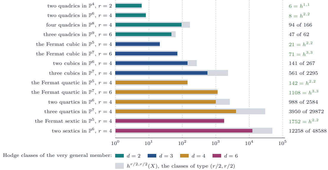
FIGURE 50. The dimension of the space of Hodge classes of degree r on the very general member, from Theorem 20.64(iii) , against the Hodge number h^{r/2, r/2} , on a logarithmic scale. Where the two agree, the space H^{r/2, r/2} is spanned by Hodge classes at every configuration; elsewhere the very general member has fewer Hodge classes, and the members with more lie over a countable union of proper closed subsets of the space of configurations.
