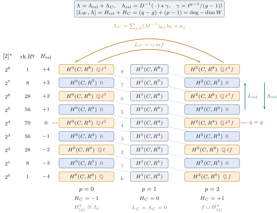
FIGURE 42. The proof of Theorem 20.21 for relative dimension four. The boxes are the summands H^p(C, R^q \pi_* \mathbb{Q}) of H^*(W, \mathbb{Q}) , split off by the eigenvalue 2^q of [2]^* shown on the left; the dotted diagonals join the summands of one H^k(W, \mathbb{Q}) , k = p + q , and the dashed magenta line is the axis q = g of hard Lefschetz on the fibres. The relative operators L_{\text{rel}} and \Lambda_{\text{rel}} , in teal, move within a column; \Lambda_{\text{rel}} is a Pontryagin product with an algebraic class on every abelian scheme ( Proposition 20.20 ). The base operators L_C and \Lambda_C , in ochre, move along a row between the outer columns and kill the middle one; \Lambda_C is the displayed cycle built from bases (a_j) , (b_k) of the invariant summands, and is algebraic exactly when the invariant cycles are. Below each column is the weight of H = [L_W, \Lambda] on it, and the panel at the top is Step 6 of the proof. The ochre boxes carry the invariant cycles and their images under L_C ; for a Mumford family they are the lines listed in magenta on the right, spanned by \ell^i f (and by \ell^i in the left column), and the other boxes of the outer columns are zero ( Corollary 20.22 ).
