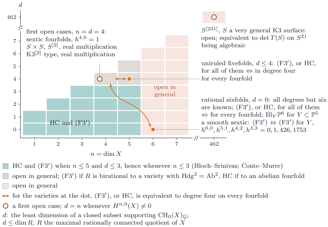
FIGURE 52. What arguments on zero-cycles and on rationally connected fibrations give for (F3') and for the Hodge conjecture (HC in the figure) on a variety X , over the plane of n = \dim X and the least dimension d of a closed subset supporting \mathrm{CH}_0(X)_{\mathbb{Q}} ; d is at most the dimension of the maximal rationally connected quotient R of X , and d = n whenever H^{n,0}(X) \neq 0 (Remark 20.45). Both hold when n \leq 5 and d \leq 3 (Proposition 20.43), hence on every variety of dimension at most three. In the hatched cells (F3') holds when R is birational to a variety with \mathrm{Hdg}^2 = \mathrm{Ab}^2 , for instance a member of \mathcal{A} , and the Hodge conjecture when R is birational to an abelian fourfold (Proposition 20.44). The double arrows are the equivalences of Remark 20.45: (F3'), and the Hodge conjecture, hold for every uniruled fivefold, and for every rational sixfold, if and only if they hold in degree four for every fourfold; the sixfold \mathrm{Bly} \mathbb{P}^6 of a smooth sextic fourfold Y in a hyperplane carries the Hodge numbers listed. The rings are the frontier cases (Remark 20.66): the sextic fourfolds, the first family of smooth hypersurfaces beyond these results (the 29 Delsarte sextics lie in \mathcal{A} by Corollary 20.52); S \times S and S^{[2]} for a K3 surface S with real multiplication, such as S_{\lambda} ; the fourfolds of \mathrm{K3}^{[2]} type with real multiplication, among them F(Y) ; and, beyond the breaks of the axes, S^{[231]} for a very general K3 surface, which is equivalent to the algebraicity of \det T(S) on S^{21} (Proposition 20.39, Figure 44).
