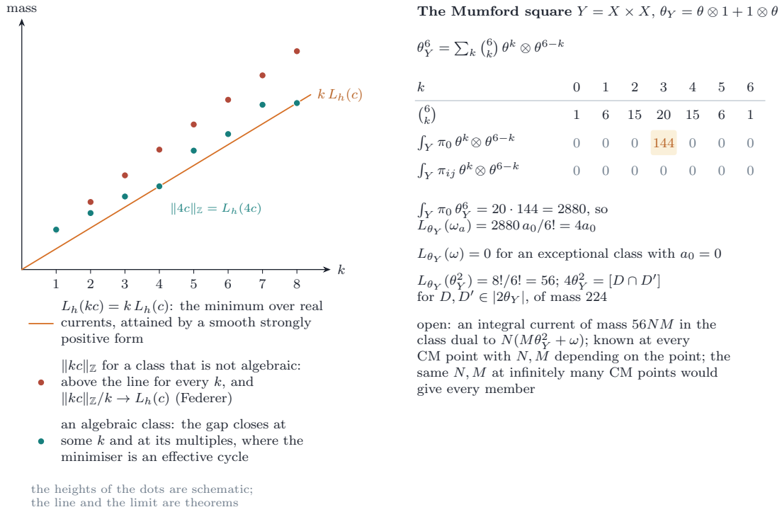
FIGURE 43. Theorem 20.68 and Example 20.69 . Left: the mass of a current in the class dual to kc against k . The line k L_h(c) is the minimum over closed real normal currents, attained by a smooth strongly positive form; the minima over closed integral currents lie on or above it, with \|kc\|_{\mathbb{Z}}/k \rightarrow L_h(c) by Federer's theorem, and for M large the class is algebraic exactly when one of them lies on the line, where the minimiser is an effective algebraic cycle. The heights of the dots are schematic. Right: the numbers of the Mumford square, computed in the split model of [BMB26] . Of the seven terms \binom{6}{k} \theta^k \otimes \theta^{6-k} of \theta_Y^6 only k = 3 pairs with \pi_0 = \frac{1}{4} \theta \otimes \theta , giving 20 \cdot 144 = 2880 , and none pairs with the primitive summands; so L_{\theta_Y}(\omega_a) = 4a_0 , the Wirtinger bound of an exceptional class with a_0 = 0 is zero, and the perturbation of NM\theta_Y^2 by N\omega changes the bound 56NM by nothing.
