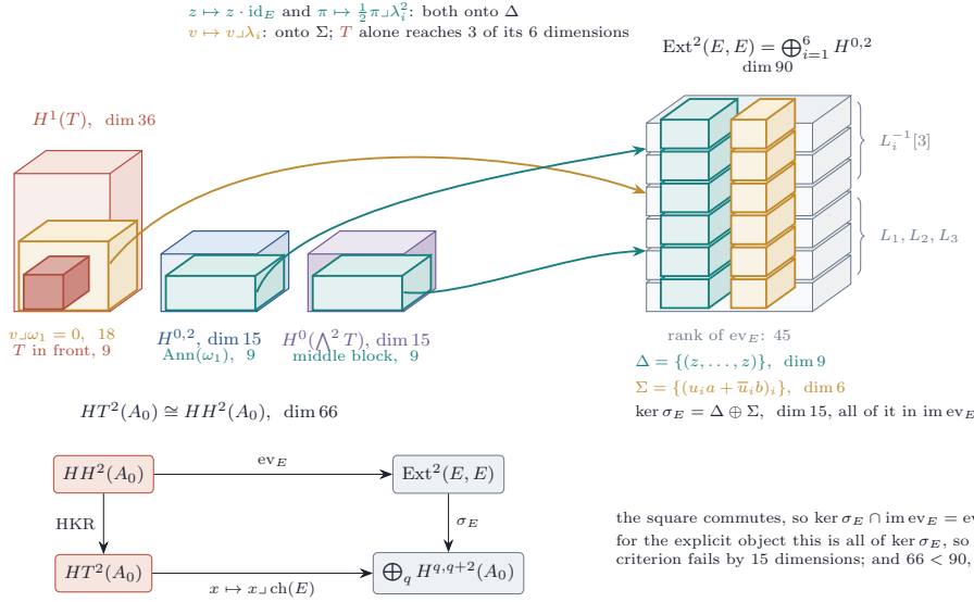
FIGURE 25. Proposition 18.18 for the explicit object at n = 3 . Left: the three summands of HT^2(A_0) , drawn with heights proportional to their dimensions, and inside each the part that preserves \text{ch}(E) to first order: the annihilator of \omega_1 , the deformations killing \omega_1 with the polarised K -commuting tangent space T in front, and the middle block of bivectors. Right: \text{Ext}^2(E, E) as six stacked copies of H^{0,2} , one per summand of E , and inside it the kernel of \sigma_E : the column \Delta , one and the same class in every layer, and the column \Sigma , whose entries depend on the summand through u_i . The three arrows are the evaluation map on the three kernels; the two teal ones both land on \Delta , the ochre one on \Sigma , and together they cover the kernel. Below, the commutative square that makes this a statement about the weakened criterion of [Mar25b, Question 11.4] .
