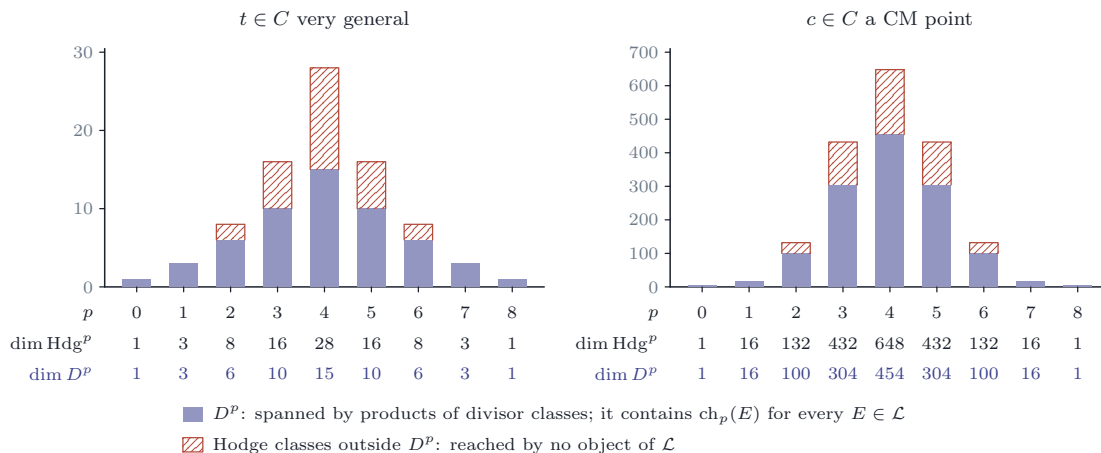
FIGURE 61. Theorem 21.36(ii) . The Hodge classes of X_t \times X_t degree by degree, against the subring D^p generated by divisor classes, which contains the Chern character of every object of \mathcal{L} : at a very general point of the Mumford curve (left) and at a CM point (right). The hatched classes, the exceptional ones among them, are reached by no object of \mathcal{L} .
