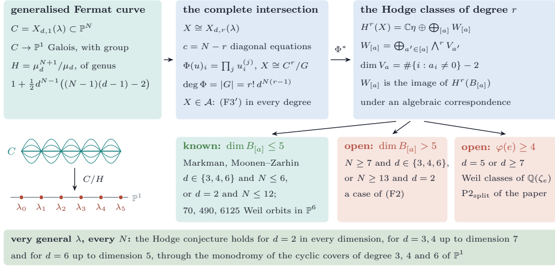
FIGURE 46. Theorem 20.54 and Corollary 20.55 . Left: the generalised Fermat curve C over \mathbb{P}^1 , its sheets meeting over the branch points \lambda_0, \dots, \lambda_N (five sheets stand for the d^N of the cover). Top: C , the complete intersection X \cong C^r/G with the map \Phi of degree |G| , and the decomposition of H^r(X) through \Phi^* . Bottom: where the Hodge conjecture for X stands at an arbitrary configuration, according to the abelian varieties B_{[a]} that carry its Hodge classes: known when they have dimension at most five, which happens for d \in \{3, 4, 6\} and N \leq 6 and for d = 2 and N \leq 12 , and open when they are larger, a case of (F2), or carry Weil classes of \mathbb{Q}(\zeta_e) with \varphi(e) \geq 4 , the case \text{P2}_{\text{split}} of the paper. Foot: the very general configuration, Theorem 20.64 .
