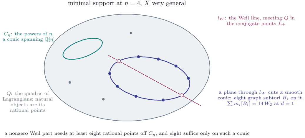
FIGURE 24. Theorem 17.26 . The quadric Q of Lagrangians; the rational points are the Chern characters of the natural objects on the split member at n = 4 , up to the Veronese map \nu_4 . The powers of the polarisation fill the conic C_\eta (teal), and the Weil line is spanned by the conjugate points L_\pm (open circles) in which the line l_W (dashed) meets Q . A combination of natural characters with a nonzero Weil part needs at least eight rational points off C_\eta , and with eight they lie on one conic cut out by a plane through l_W (indigo), such as the eight graph subvarieties B_i of Example 17.27 ; the grey points are natural objects off any such conic, which no relation of this size can use.
