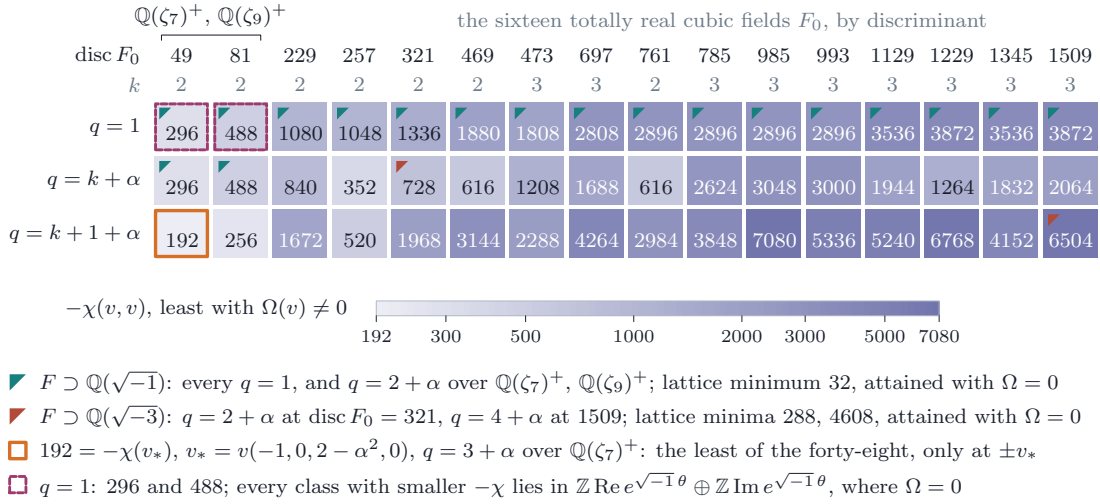
FIGURE 39. Proposition 19.52 case by case. For each of the sixteen totally real cubic fields F_0 of Proposition 19.50(v) , ordered by discriminant, and each of q = 1 , k + \alpha and k + 1 + \alpha , the cell gives the least -\chi(v, v) of an integral point v of S(0, q) whose Orlov square has a nonzero F -Weil part, that is with \Omega(v) \neq 0 ( Lemma 19.51 ), as computed in [BMB26] ; the shading is logarithmic in this value, which lies between 192 and 7080, and between 296 and 3872 for q = 1 . A corner mark shows that F = F_0(\sqrt{-q}) contains an imaginary quadratic field, \mathbb{Q}(\sqrt{-1}) in eighteen cases and \mathbb{Q}(\sqrt{-3}) in two ( Proposition 19.52(ii) ); in those cases the lattice has classes of smaller -\chi , namely 32, respectively 288 and 4608, all with \Omega = 0 . The heavy frame marks the least value 192, attained only at \pm v_* over \mathbb{Q}(\zeta_7)^+ with q = 3 + \alpha , the target of Remark 19.53 ; the dashed frames mark the values 296 and 488 for q = 1 over \mathbb{Q}(\zeta_7)^+ and \mathbb{Q}(\zeta_9)^+ , below which every integral class lies in \mathbb{Z} \operatorname{Re} e^{\sqrt{-1}\theta} \oplus \mathbb{Z} \operatorname{Im} e^{\sqrt{-1}\theta} ( Proposition 19.52(iii) ). These are least values over the lattices computed, not bounds, and a character does not give a complex.
