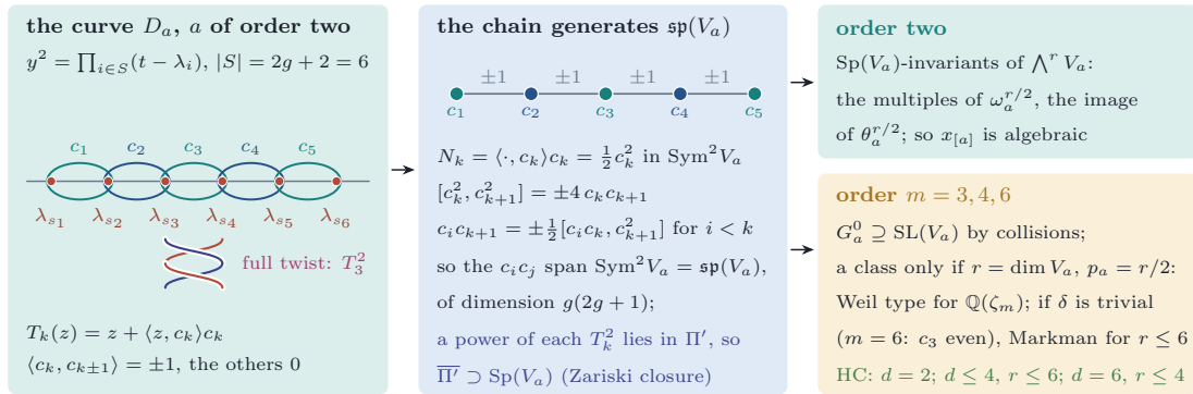
FIGURE 48. The proof of Theorem 20.64 . Left: the hyperelliptic curve D_a of a character of order two, drawn over the six points of its support for g = 2 , with the chain of vanishing cycles c_1, \dots, c_5 ; a full twist of two neighbouring branch points, drawn as a braid, acts by the square of the transvection T_k . Middle: the chain as a graph, and the induction in \text{Sym}^2 V_a by which the logarithms N_k generate \mathfrak{sp}(V_a) . Right: what the monodromy leaves of the Hodge classes, the powers of the polarisation for characters of order two, and for characters of order three, four and six the Weil classes of an abelian variety of Weil type for \mathbb{Q}(\sqrt{-3}) or \mathbb{Q}(i) .
