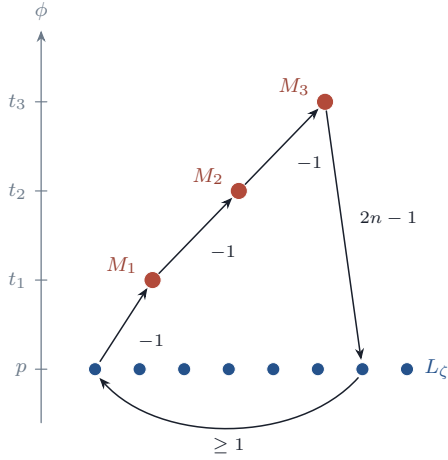
(a) the excess of a cycle, n \geq 3
