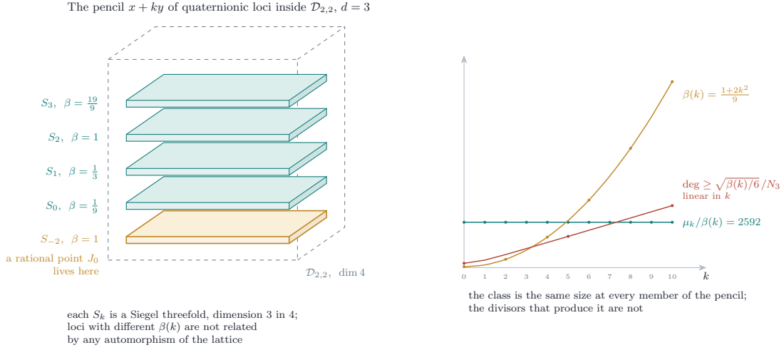
FIGURE 20. Proposition 16.24 at d = 3 . Left: the members S_k of the pencil, each a Siegel threefold inside the four-dimensional family, with the member k = -2 , where \beta = 1 and a rational point J_0 can be written down, drawn apart. Right: along the pencil the ratio \mu_k/\beta(k) is the constant 2592 = \int \eta^4/12 , so \mu_k grows like k^2 and the least degree of a divisor not proportional to \eta grows linearly in k . The Weil class is a flat class of the one fixed lattice and does not change; the divisors that produce it must.
