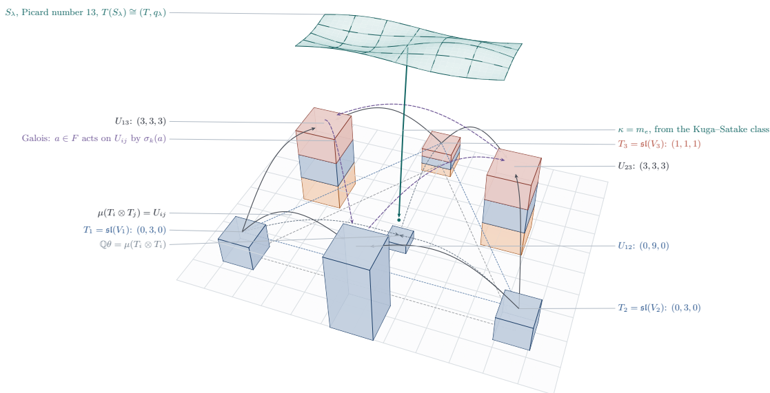
FIGURE 27. Proposition 16.45 and Lemma 16.46 , drawn over the triangle of the three factors of the Hodge group; every height is a dimension. At the corners stand the summands T_i = \mathfrak{sl}(V_i) of T = \text{Lie } G , banded by Hodge type after the Tate twist T(-1) : blue for (1, 1) , clay for (2, 0) and amber for (0, 2) , so that only T_3 carries the K3 type. On the edges stand the three summands U_{ij} of the primitive part of H^2(X) , of dimension nine, U_{12} of pure type (1, 1) and the other two in three bands of three; in the middle is the line of \theta . The solid arcs are the product map \mu , which carries T_i \otimes T_j onto U_{ij} , and the dashed ones carry T_i \otimes T_i to \mathbb{Q}\theta . The violet arcs are the Galois group permuting the U_{ij} as it permutes the embeddings of F , which is why the two exceptional classes may be taken to be the trace-zero part of a cubic field. Above, the K3 surface S_\lambda of Theorem 16.47 , whose Kuga–Satake class, if algebraic, comes down to T as the map \kappa = m_e .
