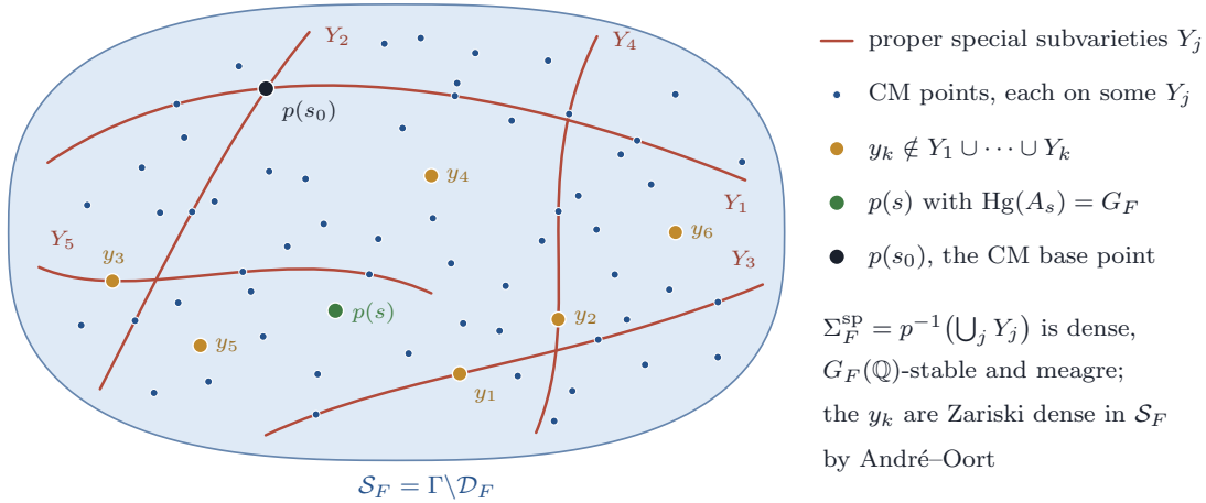
FIGURE 30. Proposition 19.12 and Theorem 19.14 on the quotient \mathcal{S}_F . The curves are five of the countably many proper special subvarieties Y_j , whose union is the image of the special locus; it contains p(s_0) and is dense and meagre. The small dots are CM points, each lying on some Y_j , drawn or not. The points y_1, \dots, y_6 begin an escaping sequence chosen as in the proof of Theorem 19.14(i) : y_k lies on no Y_j with j \leq k , so y_1 may lie on Y_3 and y_2 on Y_4 . A point p(s) at which the Hodge group is all of G_F lies on none of them.
