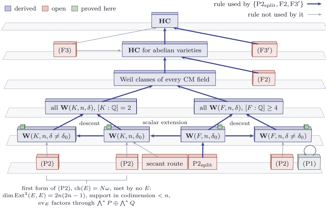
FIGURE 44. The route of this paper through the rule set of Theorem 20.61 , drawn as a stack of plates, one per level of the derivation; the other routes are drawn in Figure 43 . Heavy arrows are the rules used by the minimal set \{P2_{\text{split}}, F2, F3'\} , light arrows the rules it does not use. The bottom plate carries the propagation statement, read in the polarised form of Remark 17.6 , once for each of the four kinds of Weil family, with the secant route beside it. The small grass blocks on the next plate are the base points of Theorem 15.27 and Theorem 19.5 , one in every family. The three arrows inside that plate are Proposition 20.13 : descent from the trivial discriminant to the others, and scalar extension from the fields of degree at least four to the quadratic fields. With them (P2) is needed only for the split families of the fields of higher degree, and the other three (P2) blocks are not used. (F2) is the conjecture for the Hodge classes that no Weil line reaches, and (F3) is the whole conjecture ( Proposition 20.35 ), so the route is minimal only with (F3) replaced by (F3') of Definition 20.36 . The bracket under the two quadratic (P2) blocks records the first form of the criterion, in which the Chern character is exactly a Weil class, as Theorem 16.36 , Theorem 16.38 and Corollary 16.34 describe it; by Theorem 17.5 that form is met by no complex. The secant route reaches the trivial discriminant, since the member it is built on is split, and through descent the rest of the quadratic case; it has no edge to the fields of higher degree. The bounded criterion (P1) stands apart, closed on itself: it is equivalent to its own conclusion.
