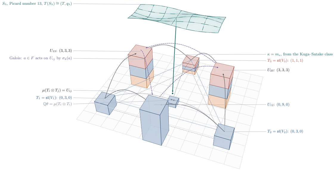
FIGURE 46. Proposition 21.2 and Lemma 21.3 , drawn over the triangle of the three factors of the Hodge group; every height is a dimension. At the corners stand the summands T_i = \mathfrak{sl}(V_i) of T = \text{Lie } G , banded by Hodge type after the Tate twist T(-1) : blue for (1, 1) , clay for (2, 0) and amber for (0, 2) , so that only T_3 carries the K3 type. On the edges stand the three summands U_{ij} of the primitive part of H^2(X) , of dimension nine, U_{12} of pure type (1, 1) and the other two in three bands of three; in the middle is the line of \theta . The solid arcs are the product map \mu , which carries T_i \otimes T_j onto U_{ij} , and the dashed ones carry T_i \otimes T_i to \mathbb{Q}\theta . The violet arcs are the Galois group permuting the U_{ij} as it permutes the embeddings of F , which is why the two exceptional classes may be taken to be the trace-zero part of a cubic field. Above, the K3 surface S_\lambda of Theorem 21.4 , whose Kuga–Satake class, if algebraic, comes down to T as the map \kappa = m_e .
