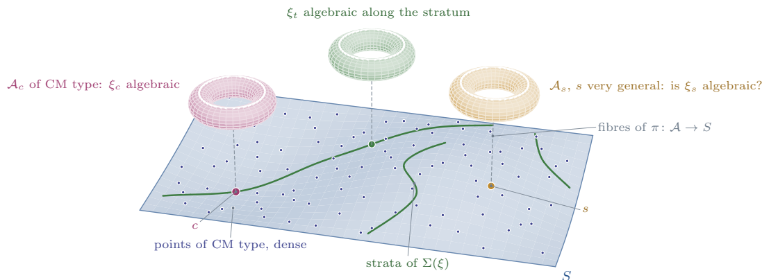
FIGURE 53. Theorem 22.5 in one family. The sheet is the base S of a polarised abelian scheme \pi: \mathcal{A} \rightarrow S through a given Hodge class, as in Proposition 22.4 ; the small dots are its points of CM type, dense by Lemma 22.3 , and the green curves are strata of the algebraic locus \Sigma(\xi) of the flat class \xi ( Lemma 22.2 ). Above three points the fibres are drawn as tori, and the loop on each stands for \xi , carried from fibre to fibre by parallel transport. At the CM member \mathcal{A}_c the class is algebraic, and it stays algebraic along the stratum through c . At a very general member \mathcal{A}_s it is algebraic exactly when \Sigma(\xi) has an interior point, and (F2) is the statement that this happens in every such family.
