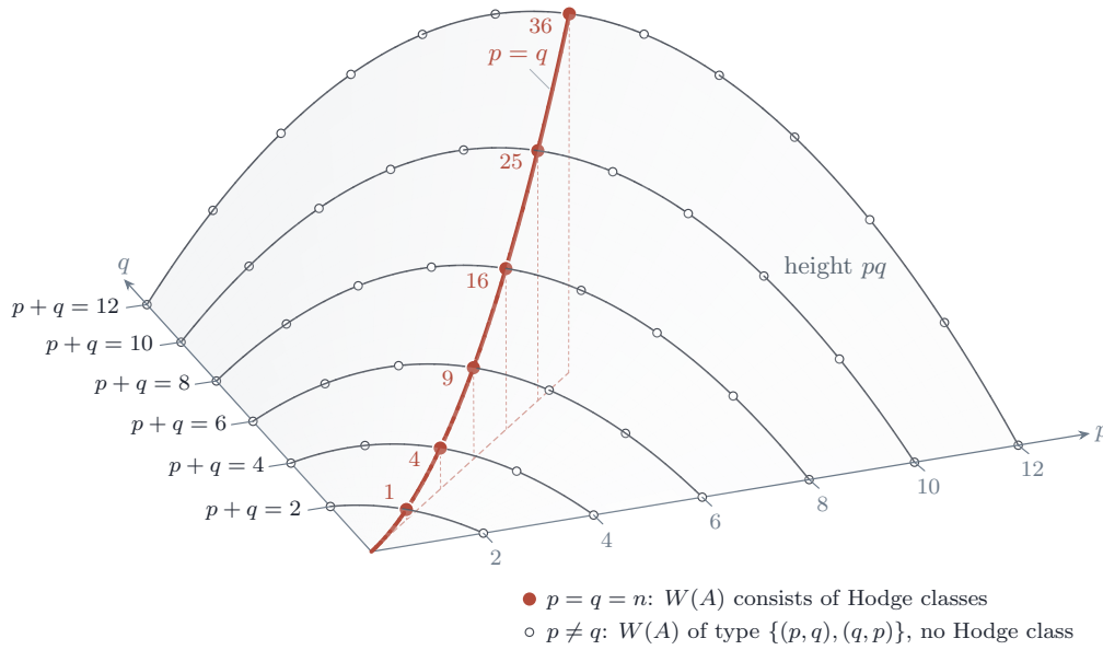
FIGURE 55. The signatures (p, q) of an imaginary quadratic action, with p + q = \dim A , drawn on the surface of height pq , which is the dimension of the family of abelian varieties carrying that action, the unitary Shimura variety of signature (p, q) . Each curve on the surface collects the signatures available in one dimension, and on it the diagonal point is the highest. The divisibility conditions of Theorem C.3 put no constraint on which of them occur when \text{End}^0(A) = K , by Proposition C.9(i) . By Proposition C.7 the Weil line consists of Hodge classes exactly at the filled points on the ridge p = q , and at every open point it is a rational sub-Hodge structure of type \{(p, 2n - p), (2n - p, p)\} carrying no Hodge class at all. The diagonal is the locus that Corollary B.9 shows to be an algebraic subvariety of the moduli.
