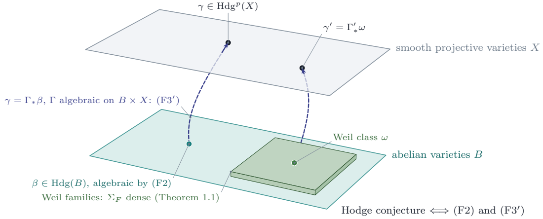
FIGURE 54. The two halves of the conjecture in Theorem 23.1(vi) . A Hodge class \gamma on a smooth projective variety X is the image \Gamma_*\beta of a Hodge class \beta on an abelian variety B under an algebraic correspondence \Gamma on B \times X , which is (F3'); the class \beta is algebraic, which is (F2), equivalently the conjecture for abelian varieties ( Proposition 21.49 ). The raised plate on the lower sheet stands for the families of Weil type, on which Theorem 1.1 makes the algebraic locus of the Weil class \omega dense; the dashed part of each correspondence is the part behind the upper sheet.
