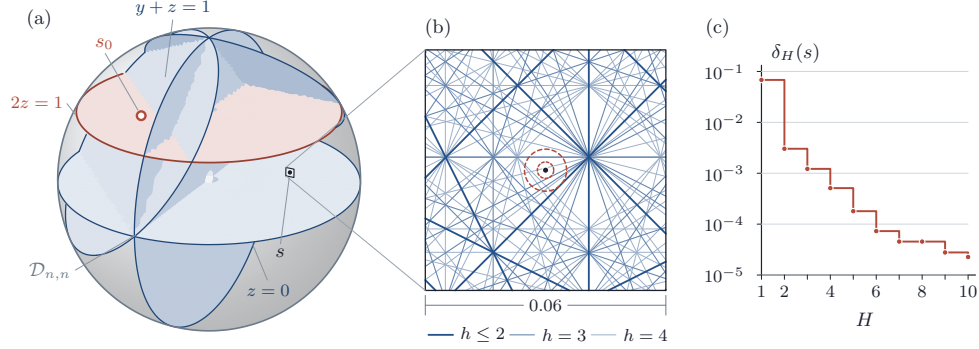
FIGURE 17. The dichotomy of Corollary 16.5 . Each stratum \Sigma_{\underline{P},\underline{q}} is Zariski closed by Theorem 16.4 , and there are countably many of them; the base point s_0 of Theorem 15.27 lies on one. By Proposition 16.7 the union of the strata is dense, so every neighbourhood of a point s lying off all of them meets infinitely many strata. The conjecture for the family is the assertion that no such s exists, and by Corollary 16.5 it is enough that one stratum has nonempty interior.
