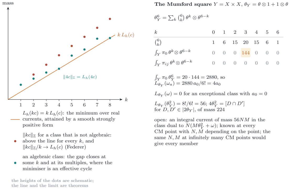
FIGURE 45. Theorem 20.71 and Example 20.72 . Left: the mass of a current in the class dual to kc against k . The line k L_h(c) is the minimum over closed real normal currents, attained by a smooth strongly positive form; the minima over closed integral currents lie on or above it, with \|kc\|_{\mathbb{Z}}/k \rightarrow L_h(c) by Federer's theorem, and for M large the class is algebraic exactly when one of them lies on the line, where the minimiser is an effective algebraic cycle. The heights of the dots are schematic. Right: the numbers of the Mumford square, computed in the split model of [BMB26] . Of the seven terms \binom{6}{k} \theta^k \otimes \theta^{6-k} of \theta_Y^6 only k = 3 pairs with \pi_0 = \frac{1}{4} \theta \otimes \theta , giving 20 \cdot 144 = 2880 , and none pairs with the primitive summands; so L_{\theta_Y}(\omega_a) = 4a_0 , the Wirtinger bound of an exceptional class with a_0 = 0 is zero, and the perturbation of NM\theta_Y^2 by N\omega changes the bound 56NM by nothing.
