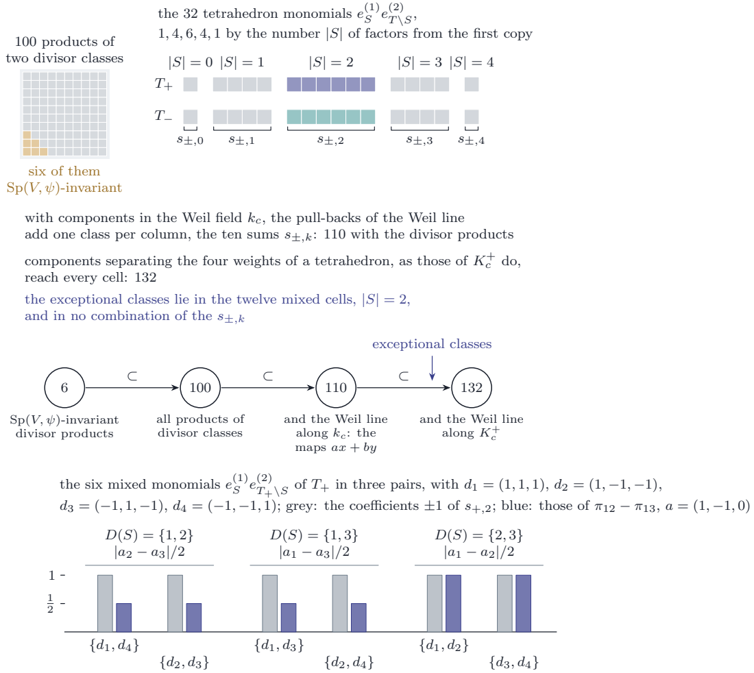
FIGURE 49. Proposition 21.29(ii) and (iii). Top: the 132 Hodge classes of degree four on the square at a CM point, one cell per monomial of weight zero. The 100 products of divisor classes are the cells with an opposite pair; the 32 tetrahedron monomials e_S^{(1)} e_{T \setminus S}^{(2)} are arranged by tetrahedron and by the number |S| of factors from the first copy. Pull-backs of the Weil line along homomorphisms with components in k_c add only the ten symmetric sums s_{\pm,k} , one per column, giving 110; components separating the four weights of a tetrahedron, as those of K_c^+ do, separate the monomials and give all 132. Bottom: on the six mixed monomials of one tetrahedron, grouped in the three pairs by the coordinates in which the two weights of S differ, the symmetric sum s_{+,2} has coefficients \pm 1 throughout, while an exceptional class \omega_a has coefficients of absolute value |a_2 - a_3|/2 , |a_1 - a_3|/2 , |a_1 - a_2|/2 , drawn for \pi_{12} - \pi_{13} ; two equal absolute values would be a linear relation among the conjugates of an irrational element of F .
