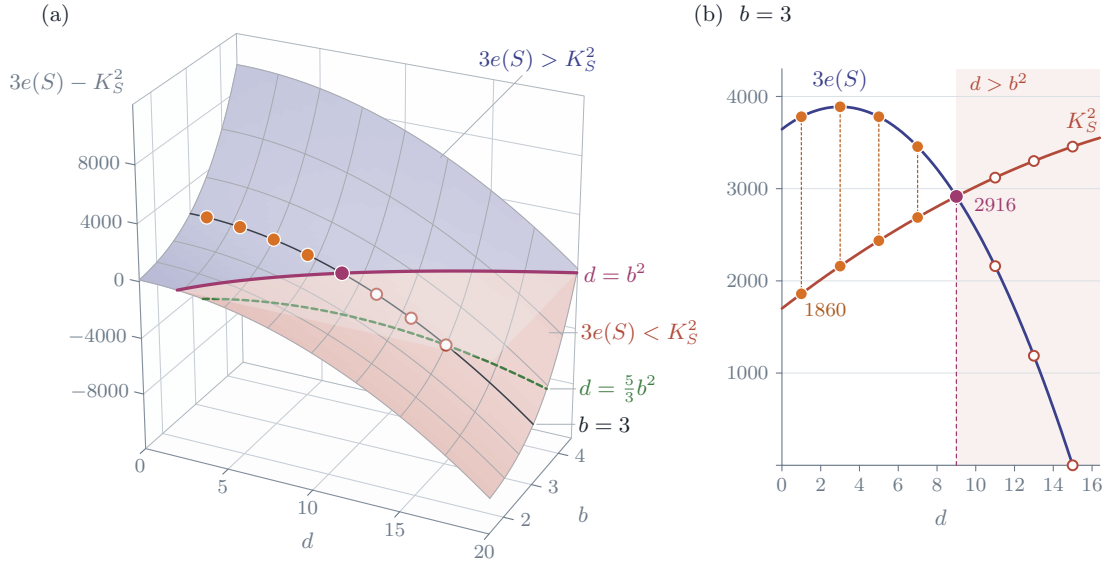
FIGURE 29. Theorem 18.57 over the quarter plane of (b, d) . The height of the surface is the defect 3e(S) - K_S^2 = 24(b^4 - d^2) in the Bogomolov–Miyaoka–Yau inequality for the surface the theorem attaches to the pair, compressed by a signed cube root so that four orders of magnitude fit one frame; the compression is odd and monotone, so the zero locus and the sign are the true ones. The surface is drawn indigo where the defect is positive and clay where it is negative, and it crosses zero along d = b^2 , which is therefore the whole content of the inequality. The weaker wall d = \frac{5}{3}b^2 , where e(S) itself changes sign, is drawn dashed and lies above it. On the line b = 3 , which is the value Proposition 18.42(iii) forces on the fourfold, the four squarefree discriminants d = 1, 3, 5, 7 with N an integer sit above the wall and are marked with their drop lines; d = 9 sits exactly on it, the equality case, and d = 11, 13, 15 sit below and are excluded.
