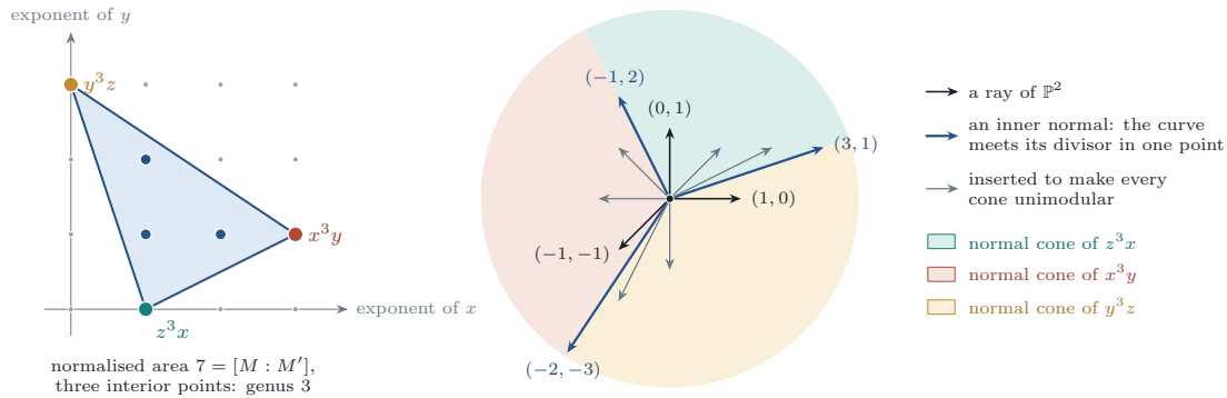
FIGURE 40. The Klein quartic x^3y + y^3z + z^3x in the proof of Theorem 20.53 . Left: its Newton triangle in the lattice M of the torus of \mathbb{P}^2 , in the chart z = 1 , with normalised area 7 = [M : M'] and three interior points, the genus. Right: the rays of a smooth fan adapted to it, the three rays of \mathbb{P}^2 , the three inner normals of the triangle and the six rays inserted to make every cone unimodular. The curve meets only the three divisors of the inner normals, in one point each, the lattice length of the edge, so its Euler number is -7 + 3 = -4 . With e_A = 7 the isogeny of the proof makes it the quotient of the Fermat septic by a group of order seven.
