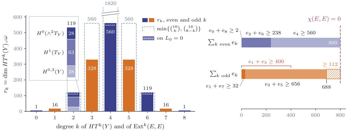
FIGURE 51. Theorem 21.34 . Left: the lower bounds r_k for \dim \text{Ext}^k(E, E) when \text{ch}(E) = N\omega , one bar per degree, symmetric about k = 4 as Lemma 21.33 predicts; the bar at k = 2 is the 119 of Theorem 21.21 , made of 28 classes in H^{0,2} , 63 in H^1(T) and 28 bivectors. On the hyperplane L_0 = 0 the bars at 2, 4 and 6 drop to 110, 548 and 110 at a sample point. Right: \chi(E, E) = 0 balances the even and the odd degrees, so the odd side, which Hochschild cohomology fills only to 688, carries at least 800.
