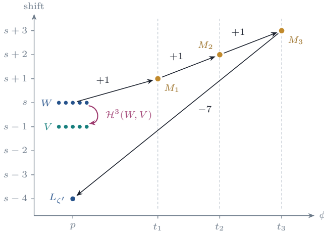
FIGURE 26. Lemma 18.38 and Theorem 18.39 , in the placement p < t_1 < t_2 < t_3 . Horizontal: the value \phi of a piece; vertical: its shift. The pieces L_\zeta with \prod \zeta = \epsilon sit at the shift s and the others at s - 1 . A run through the multiples, up three times with Ext degree 0 and down once with Ext degree 8, ends four shifts lower, the least drop of Lemma 18.38(iii) , so it never joins a top piece W to a partner V one shift lower; the group \mathcal{H}^3(W, V) survives in \text{Ext}^2(E, E) .
