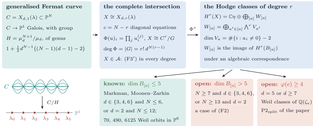
FIGURE 41. Theorem 20.56 and Corollary 20.57 . Left: the generalised Fermat curve C over \mathbb{P}^1 , its sheets meeting over the branch points \lambda_0, \dots, \lambda_N (five sheets stand for the d^N of the cover). Top: C , the complete intersection X \cong C^r/G with the map \Phi of degree |G| , and the decomposition of H^r(X) through \Phi^* . Bottom: where the Hodge conjecture for X stands, according to the abelian varieties B_{[a]} that carry its Hodge classes: known when they have dimension at most five, which happens for d \in \{3, 4, 6\} and N \leq 6 and for d = 2 and N \leq 12 , and open when they are larger, a case of (F2), or carry Weil classes of \mathbb{Q}(\zeta_e) with \varphi(e) \geq 4 , the case P2_{\text{split}} of the paper.
