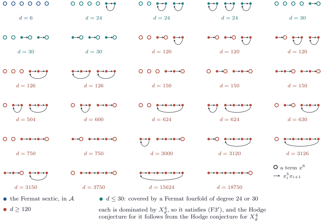
FIGURE 39. The 29 smooth sextic fourfolds of Proposition 20.49(iii), up to a renumbering of the variables. Each is drawn on its six variables: an arrow from x_i to x_j is a term x_i^5 x_j , and a ring is a term x^6 , so a chain is a path of arrows ending at a ring and a loop is a cycle of arrows. Under each is the least d with dA^{-1} integral, the degree of the Fermat fourfold that covers it. All of them satisfy (F3').
