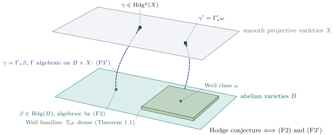
FIGURE 62. The two halves of the conjecture in Theorem 24.1(vi) . A Hodge class \gamma on a smooth projective variety X is the image \Gamma_*\beta of a Hodge class \beta on an abelian variety B under an algebraic correspondence \Gamma on B \times X , which is (F3'); the class \beta is algebraic, which is (F2), equivalently the conjecture for abelian varieties ( Proposition 21.49 ). The raised plate on the lower sheet stands for the families of Weil type, on which Theorem 1.1 makes the algebraic locus of the Weil class \omega dense; the dashed part of each correspondence is the part behind the upper sheet.
