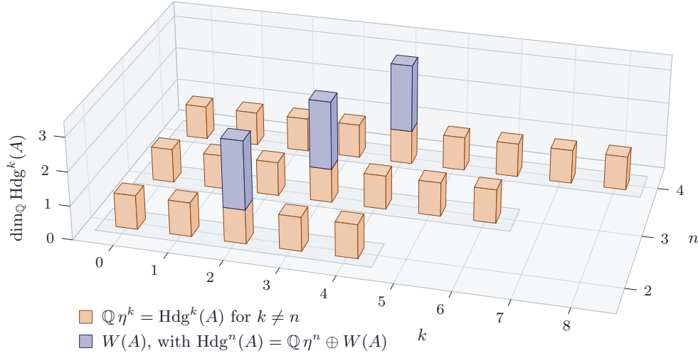
FIGURE 4. The dimensions of \mathrm{Hdg}^k(A) for a general abelian variety of (K, -1, n) -Weil type, 0 \leq k \leq 2n , at n = 2, 3, 4 , as computed in Theorem 4.14 . Every degree carries the line \mathbb{Q}\eta^k ; the middle degree k = n carries in addition the two dimensions of the Weil line W(A) , and nothing else occurs. The profile is the same for every n .
