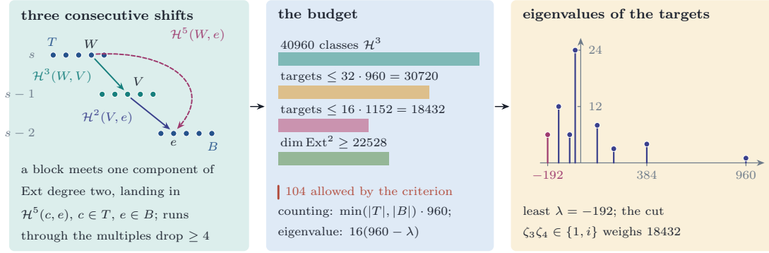
FIGURE 29. Theorem 18.38. Left: the pieces L_\zeta at three consecutive shifts, those of one parity at s - 1 and the others split between T at s and B at s - 2 ; a group \mathcal{H}^3 between two pieces that differ in three coordinates (teal) can meet a component of Ext degree two (indigo) only in a group \mathcal{H}^5(c, e) with c \in T and e \in B (magenta). Middle: the 40960 classes against the targets, at most 30720 by counting and 18432 by the least eigenvalue, against the 104 that the criterion allows. Right: the eigenvalues of the Cayley graph of the targets.
