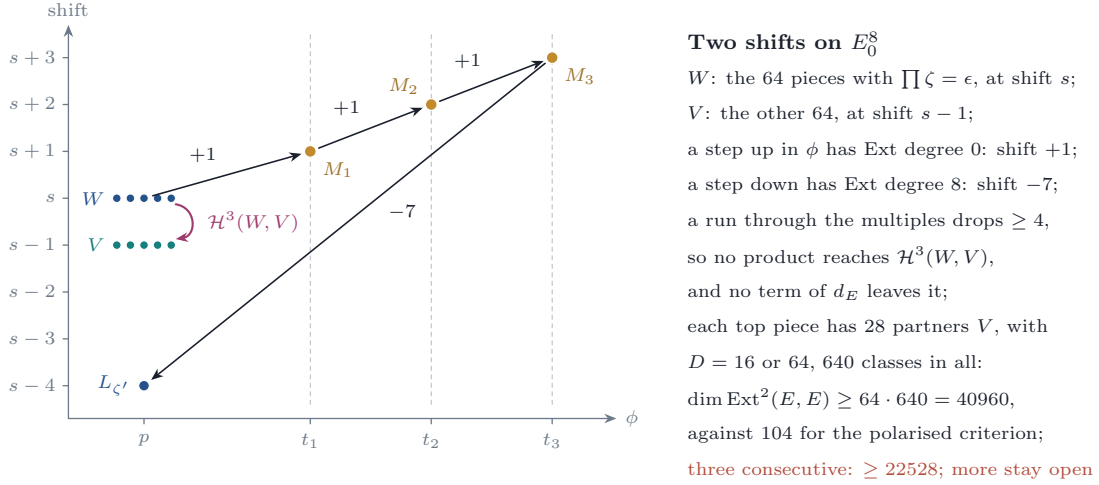
FIGURE 28. Lemma 18.36 and Theorem 18.37, in the placement p < t_1 < t_2 < t_3 . Horizontal: the value \phi of a piece; vertical: its shift. The pieces L_\zeta with \prod \zeta = \epsilon sit at the shift s and the others at s - 1 . A run through the multiples, up three times with Ext degree 0 and down once with Ext degree 8, ends four shifts lower, the least drop of Lemma 18.36(iii), so it never joins a top piece W to a partner V one shift lower; the group \mathcal{H}^3(W, V) survives in \text{Ext}^2(E, E) .
