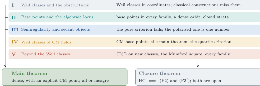
FIGURE 1. The five parts of the paper. Parts I to IV lead to Theorem 1.1 ; all five lead to the closure theorem of Section 24 , by which the Hodge conjecture is equivalent to the two statements (F2) and (F3'), both of which remain open.
