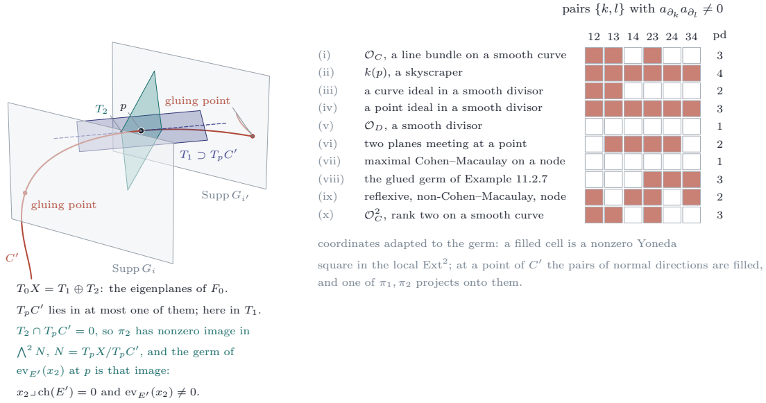
FIGURE 31. Theorem 19.39 and Corollary 19.41 . Left: the support of Markman's sheaf E' near a point p of the glued curve C' , between two of the translated supports that the curve crosses at its gluing points. The tangent space at p is the sum of the eigenplanes T_1 and T_2 of the real multiplication; the tangent line of C' lies in at most one of them, here in T_1 , so \pi_2 has nonzero image in \wedge^2 N , N = T_pX/T_pC' , which is the germ of \text{ev}_{E'}(x_2) at p . Right: for ten germs at the origin of \mathbb{C}^4 , the pairs \{k, l\} of coordinate directions whose jet classes have nonzero product in the local \text{Ext}^2 , and the projective dimension; rows (i), (ii) and (x) are Lemma 19.37 , row (iii) is Lemma 19.38 , row (vi) is Lemma 18.44 .
