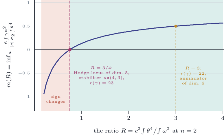
FIGURE 24. The exceptional ratio of Remark 17.12. By the identity displayed there, which is linear in \gamma , the infimum over the Kähler cone of 6 \int \gamma \kappa^2 / (|c| \sigma_2(h) \int \theta^4) is m(R) = 1 - \sqrt{3/(4R)} , approached at the boundary of the cone by a positive hermitian form of rank two whose Plücker coordinates satisfy |\xi_{01} \xi_{23}| = \frac{1}{4} . It is negative exactly for R < 3/4 , and R = 3/4 is also where the Hodge locus of \gamma jumps from dimension 4 to 5 and its stabiliser becomes \mathfrak{so}(4, 3) , with r(\gamma) = 23 ; at R = 3 the annihilator has dimension 6 and r(\gamma) = 22 . The computations of [BMB26] check these values.
