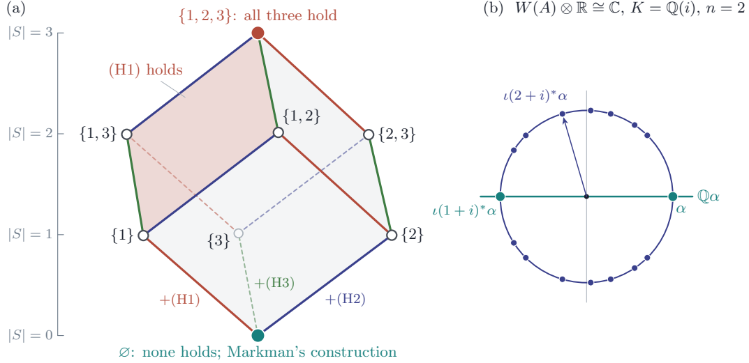
FIGURE 14. (a) The eight positions a construction can occupy, drawn as the Boolean lattice of the subsets S of three hypotheses: (H1) the Chern character of the input lies in the subring generated by divisor classes; (H2) the output is a K^\times -eigenclass; (H3) the output spans a single line rather than a plane. (H1) and (H2) are the hypotheses negated in (i) and (iii) of Proposition 13.5 , and (H3) is what Corollary 13.2 excludes for a nonzero Weil class. At the top vertex all three hold, and both Theorem 7.3 and Theorem 5.6 apply; on the shaded face (H1) holds, and Theorem 7.3 alone already applies. Markman's construction sits at the bottom vertex, where none of the three holds. (b) The orbit of a Weil class \alpha under K^\times for K = \mathbb{Q}(i) and n = 2 , in W(A) \otimes \mathbb{R} \cong \mathbb{C} and normalised to the unit circle. Since \iota(\tau)^* acts through \tau^4 , the class \iota(1+i)^*\alpha = -4\alpha stays on the line \mathbb{Q}\alpha , while \iota(2+i)^*\alpha , with (2+i)^4 = -7 + 24i , does not; the orbit spans the plane, as Proposition 13.1 asserts.
