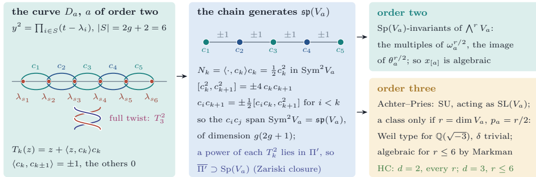
FIGURE 45. The proof of Theorem 20.57 . Left: the hyperelliptic curve D_a of a character of order two, drawn over the six points of its support for g = 2 , with the chain of vanishing cycles c_1, \dots, c_5 ; a full twist of two neighbouring branch points, drawn as a braid, acts by the square of the transvection T_k . Middle: the chain as a graph, and the induction in \text{Sym}^2 V_a by which the logarithms N_k generate \mathfrak{sp}(V_a) . Right: what the monodromy leaves of the Hodge classes, the powers of the polarisation for characters of order two, and for characters of order three the Weil classes of an abelian variety of Weil type for \mathbb{Q}(\sqrt{-3}) of trivial discriminant.
