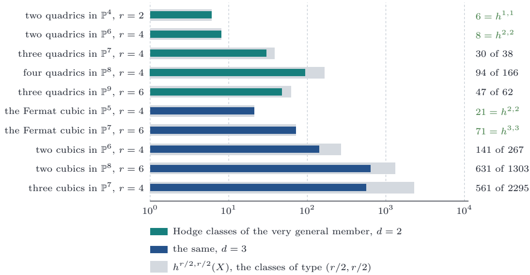
FIGURE 46. The dimension of the space of Hodge classes of degree r on the very general member, from Theorem 20.57(iii), against the Hodge number h^{r/2, r/2} , on a logarithmic scale. Where the two agree, the space H^{r/2, r/2} is spanned by Hodge classes at every configuration; elsewhere the very general member has fewer Hodge classes, and the members with more lie over a countable union of proper closed subsets of the space of configurations.
