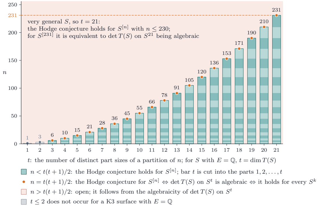
FIGURE 41. The threshold of Proposition 20.39(ii). For t = 1, \dots, 21 the bar rises to t(t+1)/2 , the least n that has a partition with t distinct part sizes, and is cut into the parts 1, 2, \dots, t of the partition that attains it. For a K3 surface S with E = \text{End}_{\text{Hdg}}(T(S)) = \mathbb{Q} and t = \dim T(S) , which is at least 3, the Hodge conjecture holds for S^{[n]} with n below the bar; at its top it is equivalent to the algebraicity of the class \det T(S) on S^t of Proposition 20.38, and to the Hodge conjecture for every power of S ; above it, it follows from that algebraicity. A very general S has t = 21 : the conjecture holds for S^{[n]} with n \leq 230 , and for S^{[231]} it is equivalent to the algebraicity of \det T(S) on S^{21} , one of the frontier cases of (F3') (Remark 20.59).
