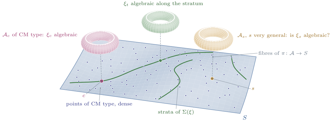
FIGURE 60. Theorem 22.5 in one family. The sheet is the base S of a polarised abelian scheme \pi: \mathcal{A} \rightarrow S through a given Hodge class, as in Proposition 22.4 ; the small dots are its points of CM type, dense by Lemma 22.3 , and the green curves are strata of the algebraic locus \Sigma(\xi) of the flat class \xi ( Lemma 22.2 ). Above three points the fibres are drawn as tori, and the loop on each stands for \xi , carried from fibre to fibre by parallel transport. At the CM member \mathcal{A}_c the class is algebraic, and it stays algebraic along the stratum through c . At a very general member \mathcal{A}_s it is algebraic exactly when \Sigma(\xi) has an interior point, and (F2) is the statement that this happens in every such family.
