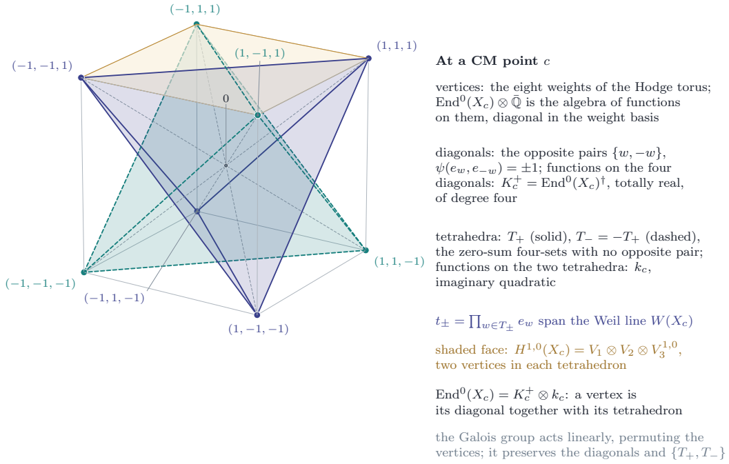
FIGURE 54. Proposition 21.29(i) . The eight weights (\pm 1, \pm 1, \pm 1) of the Hodge torus at a CM point are the vertices of a cube. The four diagonals are the pairs of opposite weights, paired by the polarisation; the two inscribed tetrahedra T_+ (an even number of entries -1 ) and T_- = -T_+ are the only zero-sum four-sets without an opposite pair, and t_{\pm} = \prod_{w \in T_{\pm}} e_w span the Weil line. The Galois group acts by linear maps permuting the vertices, so it preserves the diagonals and the pair of tetrahedra: the functions constant on the tetrahedra form the imaginary quadratic Weil field k_c , those constant on the diagonals the totally real quartic algebra K_c^+ of Rosati-fixed endomorphisms, and \text{End}^0(X_c) = K_c^+ \otimes k_c because a vertex is determined by its diagonal and its tetrahedron.
