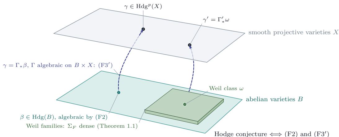
FIGURE 61. The two halves of the conjecture in Theorem 23.1(vi) . A Hodge class \gamma on a smooth projective variety X is the image \Gamma_*\beta of a Hodge class \beta on an abelian variety B under an algebraic correspondence \Gamma on B \times X , which is (F3'); the class \beta is algebraic, which is (F2), equivalently the conjecture for abelian varieties ( Proposition 21.49 ). The raised plate on the lower sheet stands for the families of Weil type, on which Theorem 1.1 makes the algebraic locus of the Weil class \omega dense; the dashed part of each correspondence is the part behind the upper sheet.
