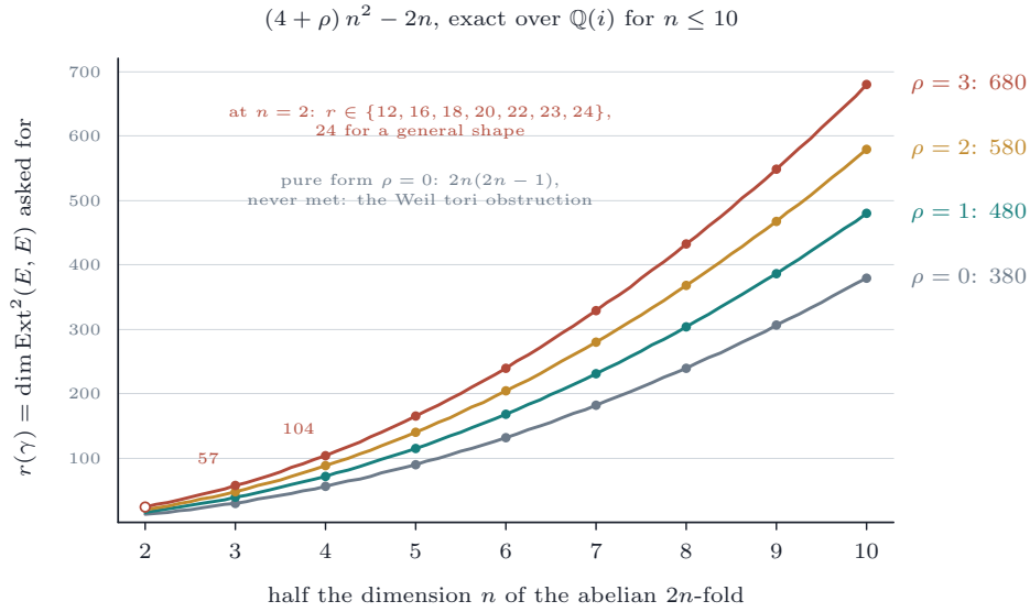
FIGURE 23. The dimension r(\gamma) = (4 + \rho)n^2 - 2n that \text{Ext}^2(E, E) must have for a complex with Chern character \gamma = N\omega_1 + \sum_k c_k \theta^k to meet the polarised criterion, for the four Hankel ranks \rho of Theorem 17.9; the dots are the values computed exactly over \mathbb{Q}(i) by [BMB26], through n = 10 , where HT^2 has dimension 780. The pure form, \rho = 0 , is the bottom curve 2n(2n - 1) , which no complex attains (Theorem 17.5); a general shape lies on the top curve 7n^2 - 2n . At n = 2 the weight argument fails for one pair of weights and seven values occur.
