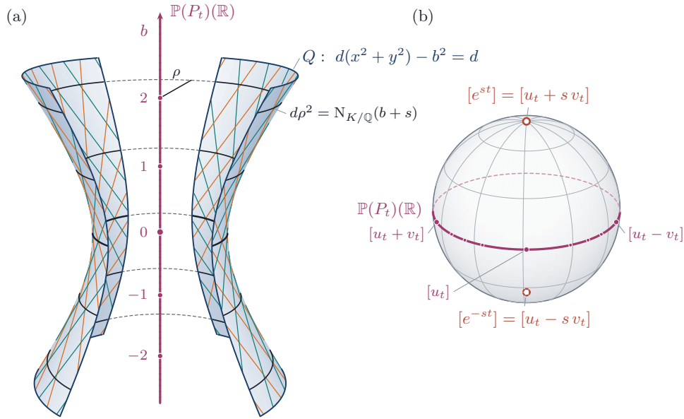
FIGURE 17. The geometry of Theorem 14.5 in the first case, n = 2 . The even spinor variety is then the smooth six-dimensional quadric of classes isotropic for the Mukai pairing in \mathbb{P}(H^{\text{ev}}(X, \mathbb{C})) \cong \mathbb{P}^7 , and the figure shows a real two-dimensional section of it, a quadric surface with its two rulings. The line \mathbb{P}(P_t) of Definition 14.4 is defined over \mathbb{Q} and meets the quadric only in the two points [e^{\pm st}] , which are conjugate over K and not individually rational; they are drawn as real points. This is the configuration the Weil line demands: a class defined over \mathbb{Q} cannot single out one of the two points, so the construction must carry the pair, and the pair spans a plane rather than a line. Proposition 13.1 is the same statement on the cohomological side, and Figure 14 places it among the hypotheses a construction can satisfy.
