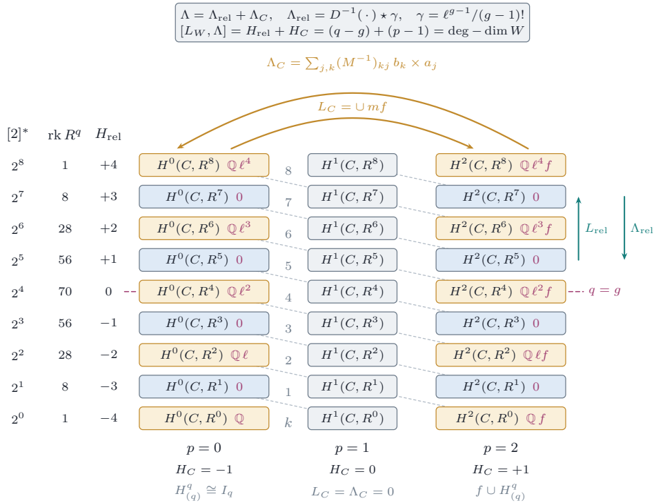
FIGURE 39. The proof of Theorem 20.21 for relative dimension four. The boxes are the summands H^p(C, R^q \pi_* \mathbb{Q}) of H^*(W, \mathbb{Q}) , split off by the eigenvalue 2^q of [2]^* shown on the left; the dotted diagonals join the summands of one H^k(W, \mathbb{Q}) , k = p + q , and the dashed magenta line is the axis q = g of hard Lefschetz on the fibres. The relative operators L_{\text{rel}} and \Lambda_{\text{rel}} , in teal, move within a column; \Lambda_{\text{rel}} is a Pontryagin product with an algebraic class on every abelian scheme ( Proposition 20.20 ). The base operators L_C and \Lambda_C , in ochre, move along a row between the outer columns and kill the middle one; \Lambda_C is the displayed cycle built from bases (a_j) , (b_k) of the invariant summands, and is algebraic exactly when the invariant cycles are. Below each column is the weight of H = [L_W, \Lambda] on it, and the panel at the top is Step 6 of the proof. The ochre boxes carry the invariant cycles and their images under L_C ; for a Mumford family they are the lines listed in magenta on the right, spanned by \ell^i f (and by \ell^i in the left column), and the other boxes of the outer columns are zero ( Corollary 20.22 ).
