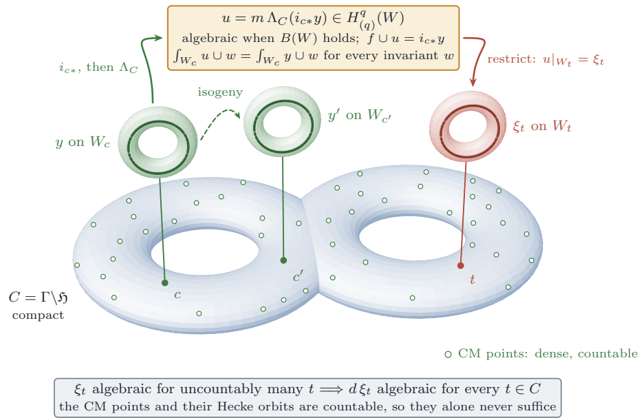
FIGURE 40. Theorem 20.28(ii) along a compact Shimura curve C . An algebraic class y on one fibre, at a base point of a Weil family or at a CM point of a Mumford family (hollow dots: the CM points, countable and dense), is pushed into W by the Gysin map and brought back to the invariant summand by the base operator \Lambda_C . When B(W) holds the result u is an algebraic class on W , pinned down by the displayed pairing against the invariant classes, and its restriction to a very general fibre is the invariant part of y . The dashed arcs are isogenies between CM members along Hecke orbits: they carry algebraic classes to algebraic classes but reach only countably many points, and Lemma 20.27 , in the box, needs uncountably many. This is how Corollary 20.31 and Corollary 20.30 turn each target into one case of (L).
