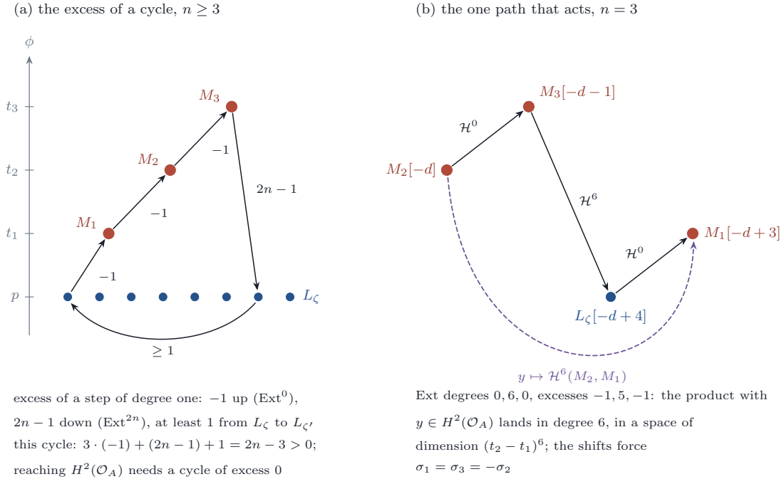
FIGURE 27. The pieces of Proposition 18.28 at their values \phi , with \phi(L_\zeta) = p and \phi(M_i) = t_i . (a) A step of degree one between pieces with a definite difference has Ext degree 0 going up and 2n going down, so excess -1 or 2n - 1 ; a step between two L_\zeta has excess at least 1. The cycle drawn runs up through all three M_i and down once, the worst case, and still has excess 2n - 3 > 0 , so for n \geq 3 no term reaches the diagonal ( Proposition 18.30 ). (b) The one path whose products act on the diagonal at n = 3 when the t_i lie above p ( Theorem 18.32(i) ), drawn at the same heights and in the order of the convolution, with the Ext degrees of its steps and the shifts they force; the dashed arrow is the value of the product with a diagonal class y .
