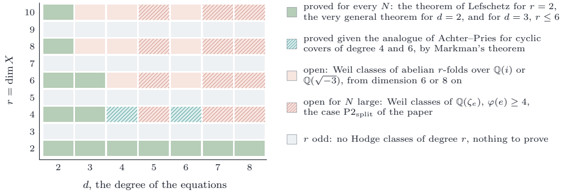
FIGURE 47. The Hodge conjecture for the very general complete intersection X_{d,r}(\lambda) of Vandermonde type, for every N . Grass: proved, by the theorem of Lefschetz for r = 2 and by Theorem 20.57 for d = 2 and for d = 3 , r \leq 6 . Teal hatching: it would follow from the analogue of the theorem of Achter and Pries for cyclic covers of degree four and six. Clay: open, the Weil classes of abelian varieties of Weil type over \mathbb{Q}(i) or \mathbb{Q}(\sqrt{-3}) in dimension at least six, or, hatched, of a CM field of degree at least four (Remark 20.58). For odd r there is nothing to prove.
