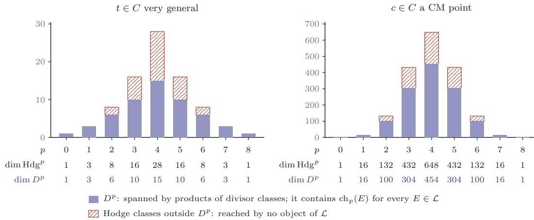
FIGURE 58. Theorem 21.36(ii) . The Hodge classes of X_t \times X_t degree by degree, against the subring D^p generated by divisor classes, which contains the Chern character of every object of \mathcal{L} : at a very general point of the Mumford curve (left) and at a CM point (right). The hatched classes, the exceptional ones among them, are reached by no object of \mathcal{L} .
