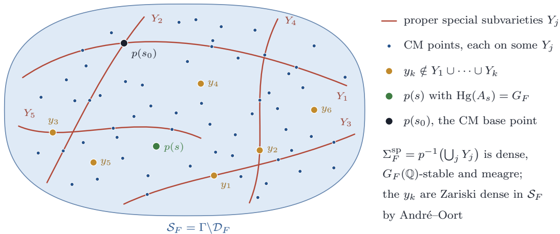
FIGURE 33. Proposition 19.12 and Theorem 19.14 on the quotient \mathcal{S}_F . The curves are five of the countably many proper special subvarieties Y_j , whose union is the image of the special locus; it contains p(s_0) and is dense and meagre. The small dots are CM points, each lying on some Y_j , drawn or not. The points y_1, \dots, y_6 begin an escaping sequence chosen as in the proof of Theorem 19.14 (i): y_k lies on no Y_j with j \leq k , so y_1 may lie on Y_3 and y_2 on Y_4 . A point p(s) at which the Hodge group is all of G_F lies on none of them.
