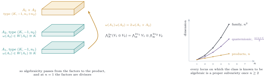
FIGURE 18. Theorem 15.7 and its reach. Left: the Weil line of each factor is a K -line, the Weil line of the product is the tensor product of the two over K , and in the K -valued notation the class is multiplicative up to the factor 2. Algebraicity therefore passes from the factors to the product, and at n = 1 the factors are divisor classes, so a product of n abelian surfaces of Weil type carries an explicit algebraic Weil class in every dimension. Right: the dimensions of the loci on which the class is known to be algebraic, against the dimension n^2 of the family. Both the quaternionic locus and the product locus are proper subvarieties once n \geq 2 , and a general member lies on neither.
