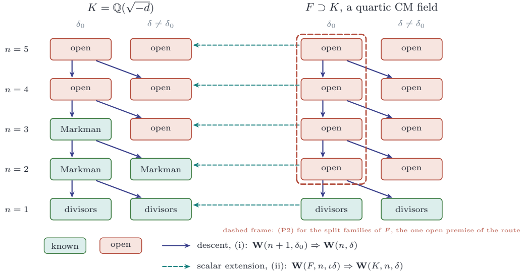
FIGURE 38. The Weil families of an imaginary quadratic field K and of a quartic CM field F \supset K , one cell for each n and each kind of discriminant, grass where the Weil classes are proved algebraic (divisor classes at n = 1 ; Markman [Mar25a, Mar25b] at n = 2 and at n = 3 , \delta = \delta_0 ) and clay where they are reached through the propagation statement. The indigo arrows are the descent of Proposition 20.13(i), from the trivial discriminant in dimension n+1 to every discriminant in dimension n ; the dashed teal arrows are the scalar extension of Proposition 20.13(ii). The dashed frame is the propagation statement for the split families of the field of higher degree, which by Theorem 20.61(ii) is the only form of (P2) that any minimal route to the conjecture uses: every clay cell of the left panel lies below it.
