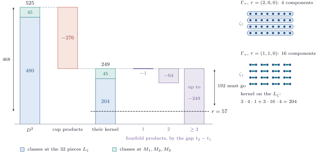
FIGURE 28. The 525 diagonal classes of degree two at n = 3 (Proposition 18.31 and Theorem 18.32). The cup products remove 276 of them for general components, and at most that many in any case, leaving 204 at the pieces L_\zeta and the 45 at the M_i ; when the t_i lie on one side of p , the fourfold products of the surviving path remove at most (t_2 - t_1)^6 more, which is 1 or 64 for the gaps 1 and 2 and no constraint from the third gap on. The criterion asks for 57, so 468 classes must disappear in all and 192 after the cup products. On the right, the graphs \Gamma_\tau on the 32 pieces, one row for each value of \zeta_1 : for \tau = (2, 0, 0) each row is a component, for \tau = (1, 1, 0) the components are the pairs differing in the sign of \zeta_3 ; a class constant on the components of every \Gamma_\tau has vanishing cup products.
