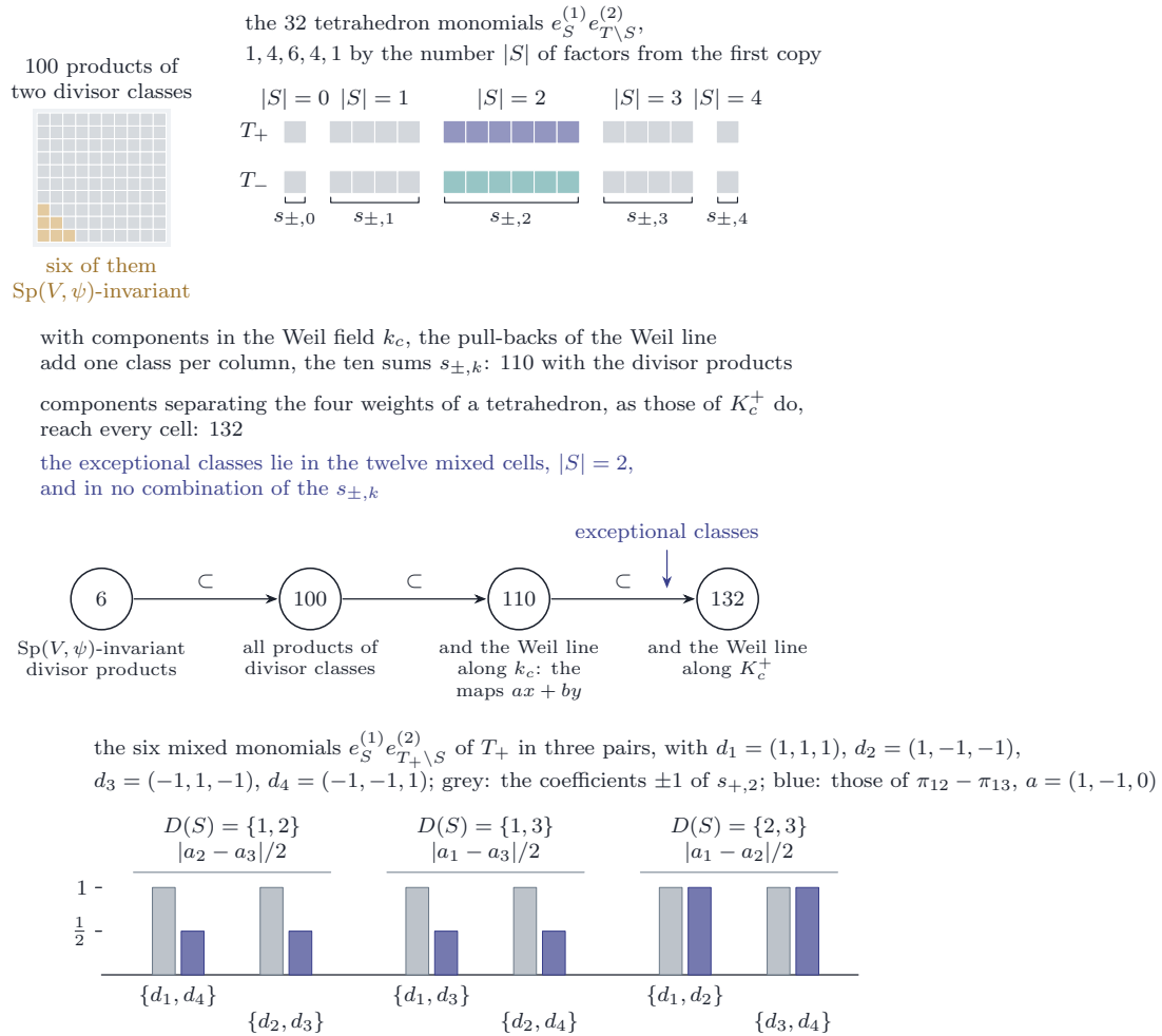
FIGURE 55. Proposition 21.29(ii) and (iii). Top: the 132 Hodge classes of degree four on the square at a CM point, one cell per monomial of weight zero. The 100 products of divisor classes are the cells with an opposite pair; the 32 tetrahedron monomials e_S^{(1)} e_{T \setminus S}^{(2)} are arranged by tetrahedron and by the number |S| of factors from the first copy. Pull-backs of the Weil line along homomorphisms with components in k_c add only the ten symmetric sums s_{\pm,k} , one per column, giving 110; components separating the four weights of a tetrahedron, as those of K_c^+ do, separate the monomials and give all 132. Bottom: on the six mixed monomials of one tetrahedron, grouped in the three pairs by the coordinates in which the two weights of S differ, the symmetric sum s_{+,2} has coefficients \pm 1 throughout, while an exceptional class \omega_a has coefficients of absolute value |a_2 - a_3|/2 , |a_1 - a_3|/2 , |a_1 - a_2|/2 , drawn for \pi_{12} - \pi_{13} ; two equal absolute values would be a linear relation among the conjugates of an irrational element of F .
