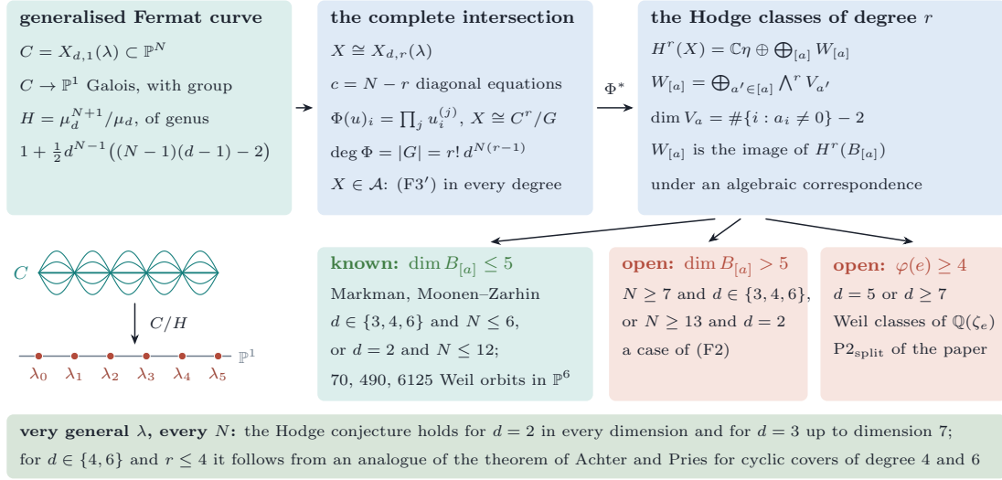
FIGURE 44. Theorem 20.54 and Corollary 20.55 . Left: the generalised Fermat curve C over \mathbb{P}^1 , its sheets meeting over the branch points \lambda_0, \dots, \lambda_N (five sheets stand for the d^N of the cover). Top: C , the complete intersection X \cong C^r/G with the map \Phi of degree |G| , and the decomposition of H^r(X) through \Phi^* . Bottom: where the Hodge conjecture for X stands at an arbitrary configuration, according to the abelian varieties B_{[a]} that carry its Hodge classes: known when they have dimension at most five, which happens for d \in \{3, 4, 6\} and N \leq 6 and for d = 2 and N \leq 12 , and open when they are larger, a case of (F2), or carry Weil classes of \mathbb{Q}(\zeta_e) with \varphi(e) \geq 4 , the case \text{P2}_{\text{split}} of the paper. Foot: the very general configuration, Theorem 20.57 .
