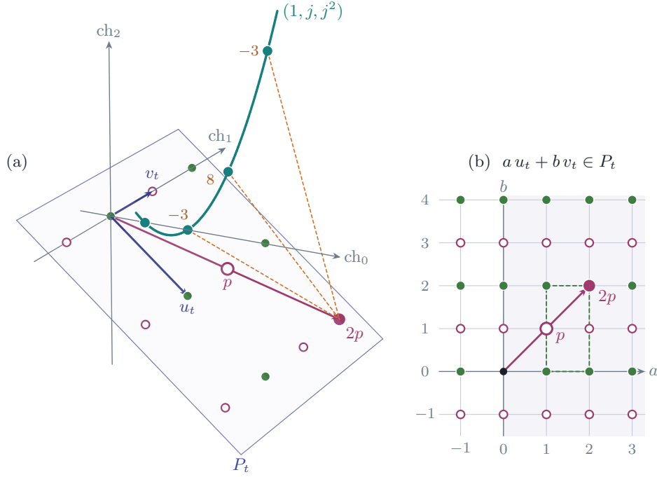
FIGURE 16. Theorem 14.13 at n = 2 and d = 2 . (a) The coordinates (ch_0, ch_1, ch_2) in the basis 1, t, t^2/2 . The Chern characters of the powers of one line bundle lie on the moment curve j \mapsto (1, j, j^2) , and the Vandermonde determinant says that any three of its points are affinely independent. The integral points of P_t = \mathbb{Q}u_t \oplus \mathbb{Q}v_t split by the criterion ch_2 \equiv ch_1 \pmod{2} into those reached by integer combinations of line bundles, drawn filled, and those missed, drawn open. The point p = u_t + v_t is missed and 2p is reached, by the witness -3[\mathcal{O}_X] + 8[\mathcal{O}_X(t)] - 3[\mathcal{O}_X(2t)] , whose three terms are joined to 2p by dashed segments. (b) The same points in the coordinates (a, b) of au_t + bv_t . Here ch_1 = b and ch_2 = -2a , so the criterion reads b \equiv 0 \pmod{2} ; the shaded half-plane a > 0 is the range of Theorem 14.13 .
