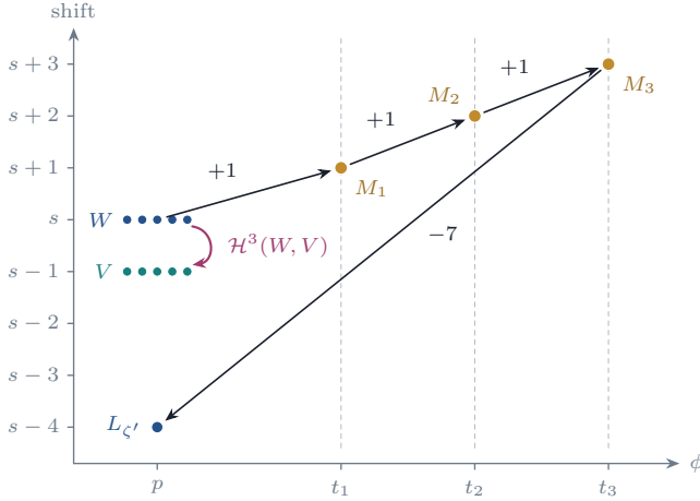
FIGURE 29. Lemma 18.38 and Theorem 18.39 , in the placement p < t_1 < t_2 < t_3 . Horizontal: the value \phi of a piece; vertical: its shift. The pieces L_\zeta with \prod \zeta = \epsilon sit at the shift s and the others at s - 1 . A run through the multiples, up three times with Ext degree 0 and down once with Ext degree 8, ends four shifts lower, the least drop of Lemma 18.38(iii) , so it never joins a top piece W to a partner V one shift lower; the group \mathcal{H}^3(W, V) survives in \text{Ext}^2(E, E) .
