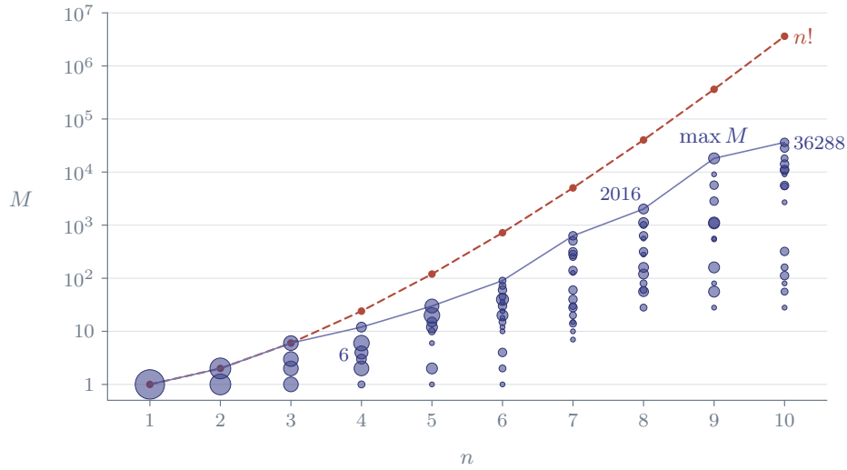
FIGURE 15. Remark 14.14. The least multiple M of Theorem 14.13 for 1 \leq n \leq 10 , over the seventy-two cases d \in \{1, 2, 3, 5, 7, 11\} , a \in \{1, 2, 3\} , b \in \{\pm 1, \pm 2\} for each n , on a logarithmic scale; the area of a disc counts the cases with that value. The solid line joins the largest values and the dashed one is n! , which every M divides: the quotient of \mathbb{Z}^{n+1} by the lattice of the characters (1, j, \dots, j^n) of the powers of a line bundle is dual to the integer-valued polynomials of degree at most n , spanned by the \binom{x}{k} , whose coefficients have denominators dividing n! .
