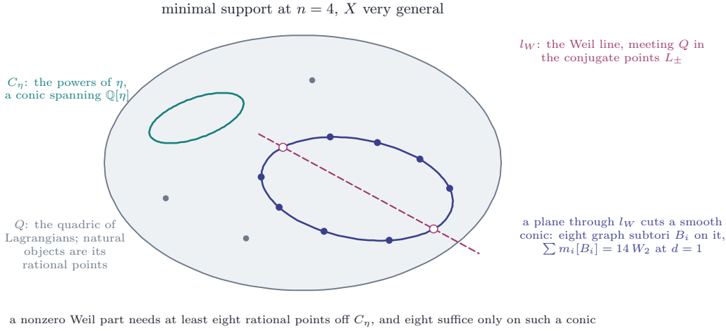
FIGURE 25. Theorem 17.25. The quadric Q of Lagrangians; the rational points are the Chern characters of the natural objects on the split member at n = 4 , up to the Veronese map \nu_4 . The powers of the polarisation fill the conic C_\eta (teal), and the Weil line is spanned by the conjugate points L_\pm (open circles) in which the line l_W (dashed) meets Q . A combination of natural characters with a nonzero Weil part needs at least eight rational points off C_\eta , and with eight they lie on one conic cut out by a plane through l_W (indigo), such as the eight graph subvarieties B_i of Example 17.26 ; the grey points are natural objects off any such conic, which no relation of this size can use.
