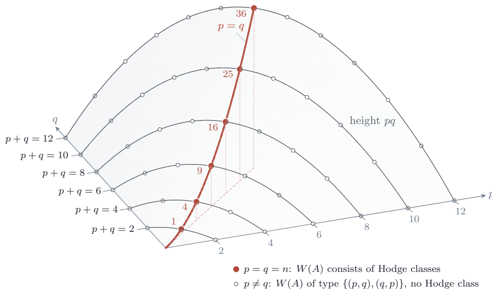
FIGURE 65. The signatures (p, q) of an imaginary quadratic action, with p + q = \dim A , drawn on the surface of height pq , which is the dimension of the family of abelian varieties carrying that action, the unitary Shimura variety of signature (p, q) . Each curve on the surface collects the signatures available in one dimension, and on it the diagonal point is the highest. The divisibility conditions of Theorem C.3 put no constraint on which of them occur when \text{End}^0(A) = K , by Proposition C.9(i) . By Proposition C.7 the Weil line consists of Hodge classes exactly at the filled points on the ridge p = q , and at every open point it is a rational sub-Hodge structure of type \{(p, 2n - p), (2n - p, p)\} carrying no Hodge class at all. The diagonal is the locus that Corollary B.9 shows to be an algebraic subvariety of the moduli.
