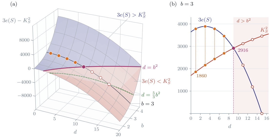
FIGURE 34. Theorem 18.65 over the quarter plane of (b, d) . The height of the surface is the defect 3e(S) - K_S^2 = 24(b^4 - d^2) in the Bogomolov–Miyaoka–Yau inequality for the surface the theorem attaches to the pair, compressed by a signed cube root so that four orders of magnitude fit one frame; the compression is odd and monotone, so the zero locus and the sign are the true ones. The surface is drawn indigo where the defect is positive and clay where it is negative, and it crosses zero along d = b^2 , which is therefore the whole content of the inequality. The weaker wall d = \frac{5}{3}b^2 , where e(S) itself changes sign, is drawn dashed and lies above it. On the line b = 3 , which is the value Proposition 18.50(iii) forces on the fourfold, the four squarefree discriminants d = 1, 3, 5, 7 with N an integer sit above the wall and are marked with their drop lines; d = 9 sits exactly on it, the equality case, and d = 11, 13, 15 sit below and are excluded.
