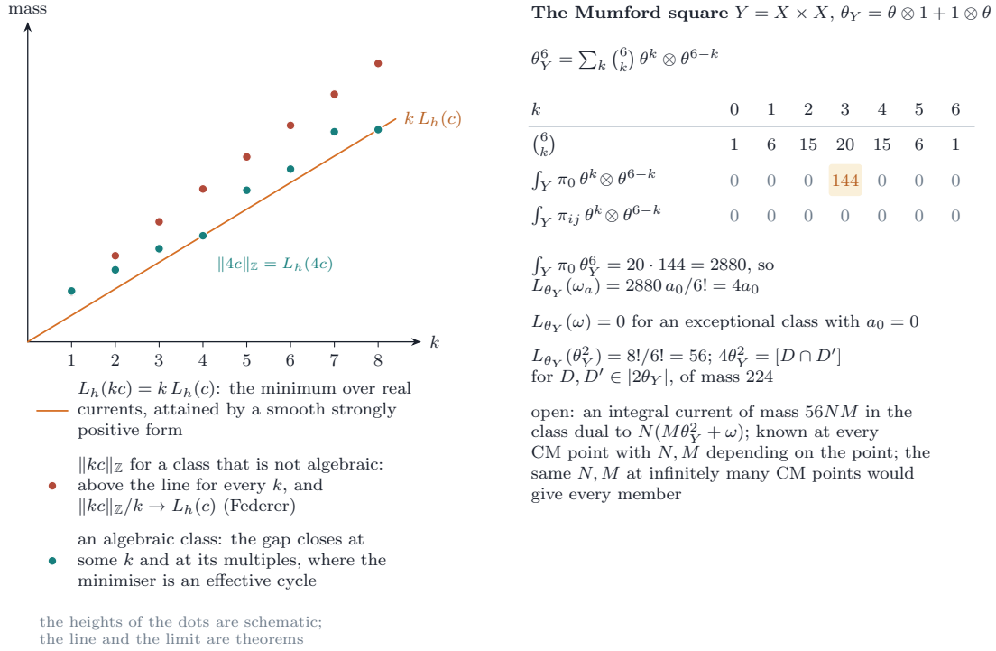
FIGURE 54. Theorem 20.76 and Example 20.77 . Left: the mass of a current in the class dual to kc against k . The line k L_h(c) is the minimum over closed real normal currents, attained by a smooth strongly positive form; the minima over closed integral currents lie on or above it, with \|kc\|_{\mathbb{Z}}/k \rightarrow L_h(c) by Federer's theorem, and for M large the class is algebraic exactly when one of them lies on the line, where the minimiser is an effective algebraic cycle. The heights of the dots are schematic. Right: the numbers of the Mumford square, computed in the split model of [BMB26] . Of the seven terms \binom{6}{k} \theta^k \otimes \theta^{6-k} of \theta_Y^6 only k = 3 pairs with \pi_0 = \frac{1}{4} \theta \otimes \theta , giving 20 \cdot 144 = 2880 , and none pairs with the primitive summands; so L_{\theta_Y}(\omega_a) = 4a_0 , the Wirtinger bound of an exceptional class with a_0 = 0 is zero, and the perturbation of NM\theta_Y^2 by N\omega changes the bound 56NM by nothing.
