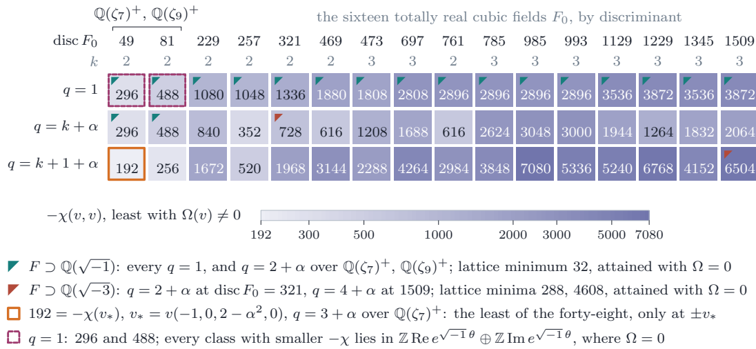
FIGURE 39. Proposition 19.52 case by case. For each of the sixteen totally real cubic fields F_0 of Proposition 19.50(v) , ordered by discriminant, and each of q = 1 , k + \alpha and k + 1 + \alpha , the cell gives the least -\chi(v, v) of an integral point v of S(0, q) whose Orlov square has a nonzero F -Weil part, that is with \Omega(v) \neq 0 ( Lemma 19.51 ), as computed in [ BMB26 ]; the shading is logarithmic in this value, which lies between 192 and 7080, and between 296 and 3872 for q = 1 . A corner mark shows that F = F_0(\sqrt{-q}) contains an imaginary quadratic field, \mathbb{Q}(\sqrt{-1}) in eighteen cases and \mathbb{Q}(\sqrt{-3}) in two ( Proposition 19.52(ii) ); in those cases the lattice has classes of smaller -\chi , namely 32, respectively 288 and 4608, all with \Omega = 0 . The heavy frame marks the least value 192, attained only at \pm v_* over \mathbb{Q}(\zeta_7)^+ with q = 3 + \alpha , the target of Remark 19.53 ; the dashed frames mark the values 296 and 488 for q = 1 over \mathbb{Q}(\zeta_7)^+ and \mathbb{Q}(\zeta_9)^+ , below which every integral class lies in \mathbb{Z} \operatorname{Re} e^{\sqrt{-1}\theta} \oplus \mathbb{Z} \operatorname{Im} e^{\sqrt{-1}\theta} ( Proposition 19.52(iii) ). These are least values over the lattices computed, not bounds, and a character does not give a complex.
