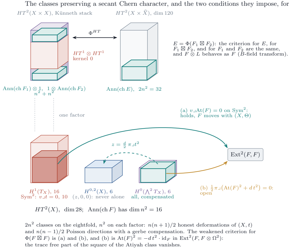
FIGURE 32. Theorem 18.54 for n = 4 . Top: the Künneth stack of HT^2(X \times X) , whose middle summand HT^1 \otimes HT^1 meets the kernel in zero by (i), so that the classes preserving \text{ch}(F_1 \boxtimes F_2) are two copies of the kernel on one factor; across Orlov's isomorphism, HT^2 of the eightfold with the 2n^2 classes preserving \text{ch}(E) . Bottom: HT^2(X) as three slabs with heights proportional to their dimensions, and inside them the n^2 classes of (55): the polarised deformations in front of H^1(T_X) , and the whole of H^0(\wedge^2 T_X) , each bivector tilted into H^{0,2} by its compensation \frac{d}{2} \pi \lrcorner t^2 ; nothing in H^{0,2} alone preserves \text{ch}(F) . On the right, the two conditions that the evaluation map imposes on the two parts, (a) closed by the construction of \mathcal{F} and (b) the identity (57).
