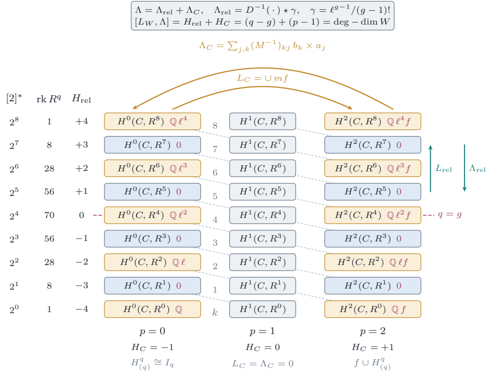
FIGURE 35. The proof of Theorem 20.22 for relative dimension four. The boxes are the summands H^p(C, R^q \pi_* \mathbb{Q}) of H^*(W, \mathbb{Q}) , split off by the eigenvalue 2^q of [2]^* shown on the left; the dotted diagonals join the summands of one H^k(W, \mathbb{Q}) , k = p + q , and the dashed magenta line is the axis q = g of hard Lefschetz on the fibres. The relative operators L_{\text{rel}} and \Lambda_{\text{rel}} , in teal, move within a column; \Lambda_{\text{rel}} is a Pontryagin product with an algebraic class on every abelian scheme ( Proposition 20.21 ). The base operators L_C and \Lambda_C , in ochre, move along a row between the outer columns and kill the middle one; \Lambda_C is the displayed cycle built from bases (a_j) , (b_k) of the invariant summands, and is algebraic exactly when the invariant cycles are. Below each column is the weight of H = [L_W, \Lambda] on it, and the panel at the top is Step 6 of the proof. The ochre boxes carry the invariant cycles and their images under L_C ; for a Mumford family they are the lines listed in magenta on the right, spanned by \ell^i f (and by \ell^i in the left column), and the other boxes of the outer columns are zero ( Corollary 20.23 ).
