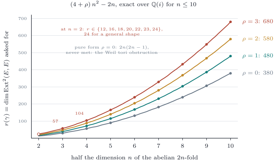
FIGURE 20. The dimension r(\gamma) = (4 + \rho)n^2 - 2n that \text{Ext}^2(E, E) must have for a complex with Chern character \gamma = N\omega_1 + \sum_k c_k \theta^k to meet the polarised criterion, for the four Hankel ranks \rho of Theorem 17.9; the dots are the values computed exactly over \mathbb{Q}(i) by [BMB26], through n = 10 , where HT^2 has dimension 780. The pure form, \rho = 0 , is the bottom curve 2n(2n - 1) , which no complex attains (Theorem 17.5); a general shape lies on the top curve 7n^2 - 2n . At n = 2 the weight argument fails for one pair of weights and seven values occur.
