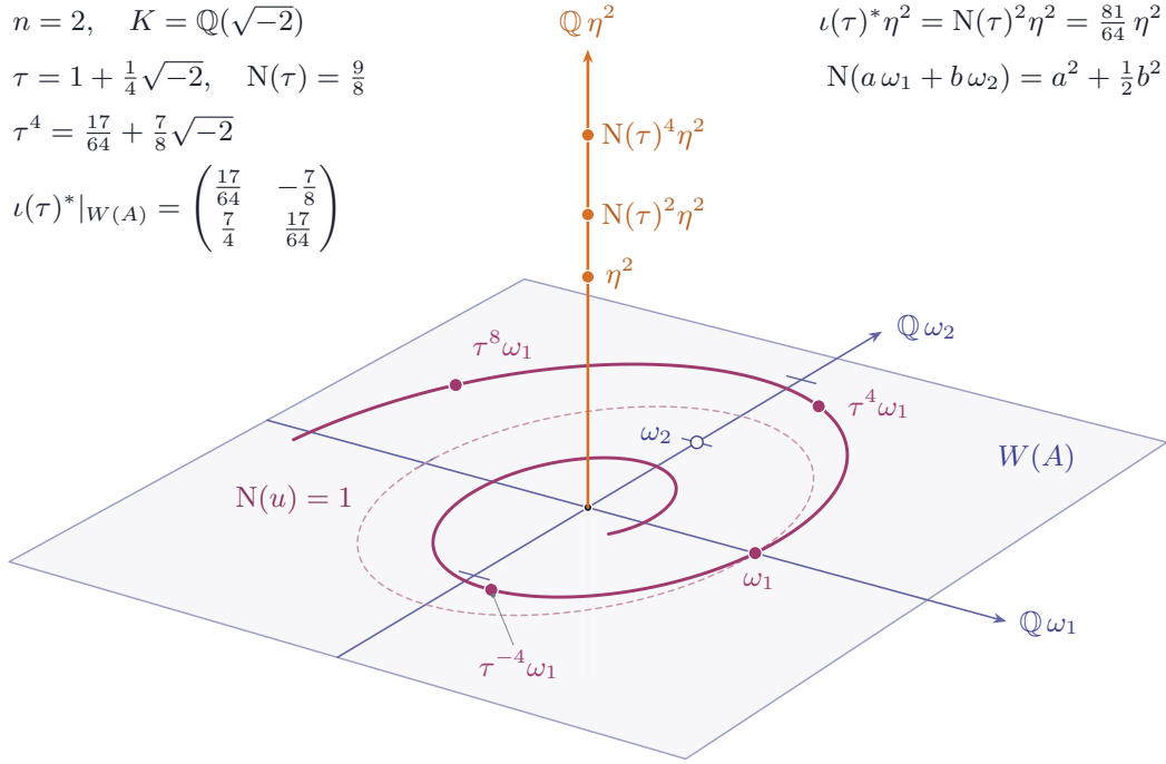
FIGURE 5. The linear algebra behind Theorem 7.3 , drawn inside H^{2n}(A, \mathbb{Q}) . The Weil line W(A) is a plane, free of rank one over K and of rank two over \mathbb{Q} , and K^\times acts on it through \tau^{2n} , so the orbit of any nonzero class is a spiral that spans the plane and lies on no line in it. The transverse axis carries \eta^n , on which K^\times acts through the norm. A construction returning a single eigenclass returns a line, and by Proposition 13.1 no line inside W(A) is stable.
