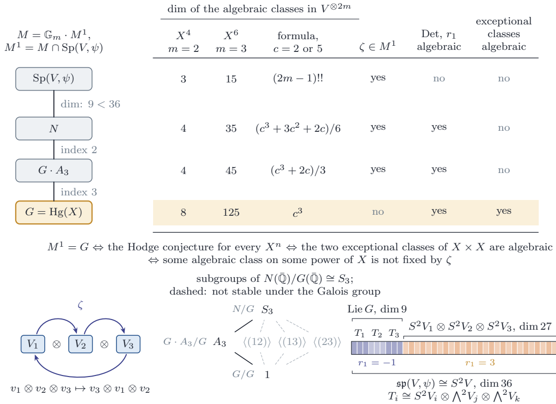
FIGURE 50. The four possible groups M^1 = M \cap \mathrm{Sp}(V, \psi) of Proposition 21.47, where M = \mathbb{G}_m \cdot M^1 , as the chain G \subset G \cdot A_3 \subset N \subset \mathrm{Sp}(V, \psi) : the first two inclusions have index 3 and 2, and N , whose identity component is G , has dimension 9 against 36. For each case the table gives the dimension of the algebraic classes in the multilinear part V^{\otimes 2m} of H^{2m}(X^{2m}, \mathbb{Q}) for m = 2 and m = 3 , from the c = 2 , respectively c = 5 , non-crossing pairings (a computation in [BMB26]); whether M^1 contains the cyclic permutation \zeta of the three tensor factors; whether Det and r_1 are algebraic; and whether the two exceptional classes of X \times X are. Only M^1 = G makes the exceptional classes algebraic, and it is equivalent to the Hodge conjecture for every power of X (Proposition 21.47(ii)); the proposition does not decide which of the four cases occurs. Below, from left to right: \zeta ; the subgroups of N(\bar{\mathbb{Q}})/G(\bar{\mathbb{Q}}) \cong S_3 , of which only 1 , A_3 and S_3 are stable under the Galois group, which acts transitively on the three factors; and \mathfrak{sp}(V, \psi) = \mathrm{Lie} G \oplus S^2 V_1 \otimes S^2 V_2 \otimes S^2 V_3 , 36 = 9 + 27 , the second summand irreducible under G , with the eigenvalues -1 and 3 of r_1 on the two summands.
