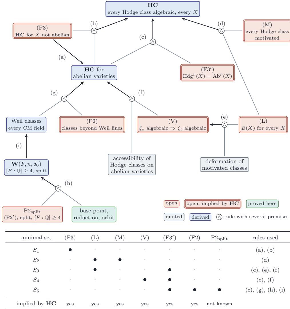
FIGURE 41. The rule set of Setup 20.57 with the rules of Section 20.6 , drawn as a hypergraph. A rule with several premises is a junction marked \wedge , joined to its premises and with one arrow to its conclusion. The letters name the results that prove the rules: (a) is Proposition 20.35 ; (b) and (g) are the closure map of Section 20.5 ; (c) is Proposition 20.37(i) ; (d) is Proposition 20.17 ; (e) is Proposition 20.18 ; (f) is Theorem 20.19 ; (h) is Theorem 19.7 ; and (i) is the chain of Proposition 20.13 , Proposition 20.12 , Proposition 19.3 and Appendix C . Clay marks a hypothesis, a double frame a hypothesis that the conjecture implies, grass what this paper proves, slate what it quotes, and indigo a derived statement. The table lists the five minimal sufficient sets of Theorem 20.58(ii) , the rules each of them uses, and which of the hypotheses the conjecture implies; only P2 split , which asks for a particular complex, is drawn without that frame. The secant route, which reaches the imaginary quadratic families only, is drawn in Figure 42 .
