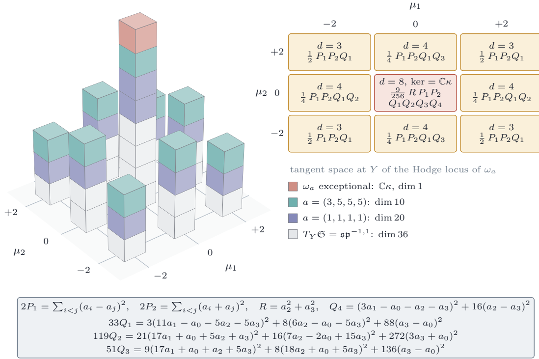
FIGURE 45. Theorem 21.21 . Left: the Siegel space \mathfrak{S} of dimension 36 near Y = X_c \times X_c and three Hodge loci through it, labelled by the tangent dimension T at Y : the class with equal coefficients ( T = 20 ), the products of divisor classes with a_1 = a_2 = a_3 ( T = 10 , the diagonal Siegel space), and a rational exceptional class ( T = 1 ), whose locus is the compact Mumford curve with its CM points (hollow). The dashed rim is the boundary of \mathfrak{S} , which the curve does not reach. Right: the nine weight blocks of \mathfrak{sp}^{-1,1} under the torus of the first two factors, with their dimensions and the forms whose product is the Gram determinant of each; only the block of weight (0, 0) has a kernel, the direction \kappa of the curve. The same holds in the 46 blocks of HT^2(Y) off the hyperplane L_0 = 0 . Below: the sums of squares that make the determinants nonzero at the conjugates of an irrational element of F .
