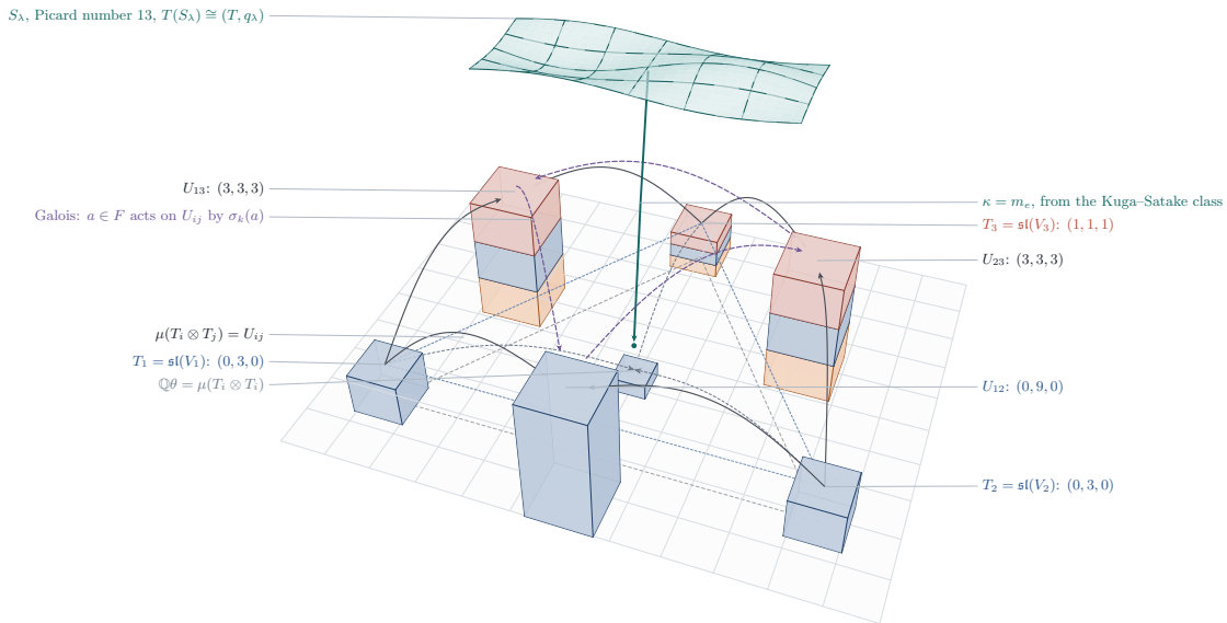
FIGURE 44. Proposition 21.2 and Lemma 21.3 , drawn over the triangle of the three factors of the Hodge group; every height is a dimension. At the corners stand the summands T_i = \mathfrak{sl}(V_i) of T = \text{Lie } G , banded by Hodge type after the Tate twist T(-1) : blue for (1, 1) , clay for (2, 0) and amber for (0, 2) , so that only T_3 carries the K3 type. On the edges stand the three summands U_{ij} of the primitive part of H^2(X) , of dimension nine, U_{12} of pure type (1, 1) and the other two in three bands of three; in the middle is the line of \theta . The solid arcs are the product map \mu , which carries T_i \otimes T_j onto U_{ij} , and the dashed ones carry T_i \otimes T_i to \mathbb{Q}\theta . The violet arcs are the Galois group permuting the U_{ij} as it permutes the embeddings of F , which is why the two exceptional classes may be taken to be the trace-zero part of a cubic field. Above, the K3 surface S_\lambda of Theorem 21.4 , whose Kuga–Satake class, if algebraic, comes down to T as the map \kappa = m_e .
