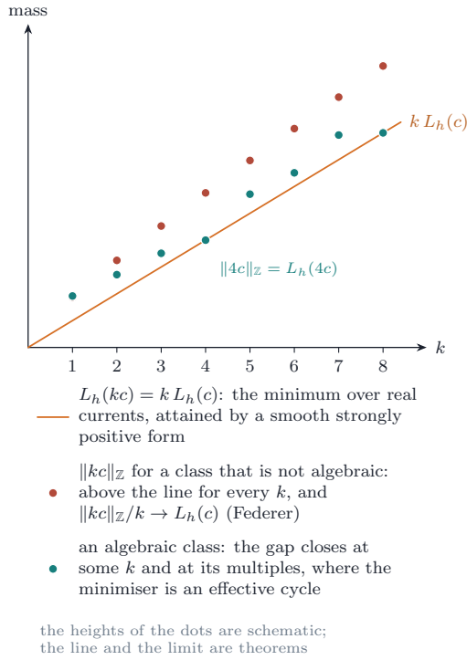
FIGURE 43. Theorem 20.68 and Example 20.69 . Left: the mass of a current in the class dual to kc against k . The line k L_h(c) is the minimum over closed real normal currents, attained by a smooth strongly positive form; the minima over closed integral currents lie on or above it, with \|kc\|_Z/k \rightarrow L_h(c) by Federer's theorem, and for M large the class is algebraic exactly when one of them lies on the line, where the minimiser is an effective algebraic cycle. The heights of the dots are schematic. Right: the numbers of the Mumford square, computed in the split model of [BMB26] . Of the seven terms \binom{6}{k} \theta^k \otimes \theta^{6-k} of \theta_Y^6 only k = 3 pairs with \pi_0 = \frac{1}{4} \theta \otimes \theta , giving 20 \cdot 144 = 2880 , and none pairs with the primitive summands; so L_{\theta_Y}(\omega_a) = 4a_0 , the Wirtinger bound of an exceptional class with a_0 = 0 is zero, and the perturbation of NM\theta_Y^2 by N\omega changes the bound 56NM by nothing.
