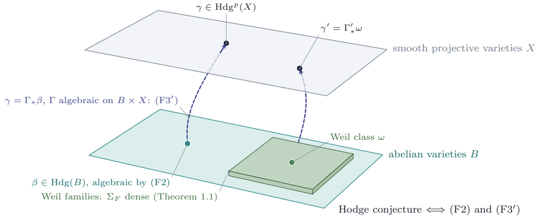
FIGURE 52. The two halves of the conjecture in Theorem 23.1(vi) . A Hodge class \gamma on a smooth projective variety X is the image \Gamma_*\beta of a Hodge class \beta on an abelian variety B under an algebraic correspondence \Gamma on B \times X , which is (F3'); the class \beta is algebraic, which is (F2), equivalently the conjecture for abelian varieties ( Proposition 21.49 ). The raised plate on the lower sheet stands for the families of Weil type, on which Theorem 1.1 makes the algebraic locus of the Weil class \omega dense; the dashed part of each correspondence is the part behind the upper sheet.
