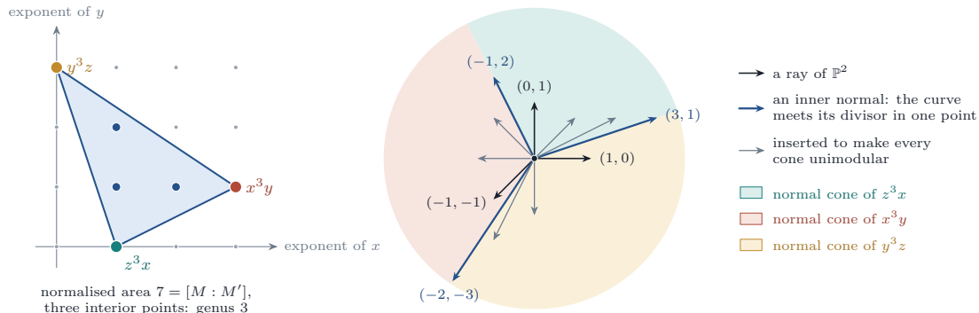
FIGURE 39. The Klein quartic x^3y + y^3z + z^3x in the proof of Theorem 20.53 . Left: its Newton triangle in the lattice M of the torus of \mathbb{P}^2 , in the chart z = 1 , with normalised area 7 = [M : M'] and three interior points, the genus. Right: the rays of a smooth fan adapted to it, the three rays of \mathbb{P}^2 , the three inner normals of the triangle and the six rays inserted to make every cone unimodular. The curve meets only the three divisors of the inner normals, in one point each, the lattice length of the edge, so its Euler number is -7 + 3 = -4 . With e_A = 7 the isogeny of the proof makes it the quotient of the Fermat septic by a group of order seven.
