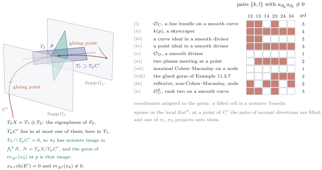
FIGURE 32. Theorem 19.44 and Corollary 19.46. Left: the support of Markman's sheaf E' near a point p of the glued curve C' , between two of the translated supports that the curve crosses at its gluing points. The tangent space at p is the sum of the eigenplanes T_1 and T_2 of the real multiplication; the tangent line of C' lies in at most one of them, here in T_1 , so \pi_2 has nonzero image in \wedge^2 N , N = T_pX/T_pC' , which is the germ of \text{ev}_{E'}(x_2) at p . Right: for ten germs at the origin of \mathbb{C}^4 , the pairs \{k, l\} of coordinate directions whose jet classes have nonzero product in the local \text{Ext}^2 , and the projective dimension; rows (i), (ii) and (x) are Lemma 19.42, row (iii) is Lemma 19.43, row (vi) is Lemma 18.48.
