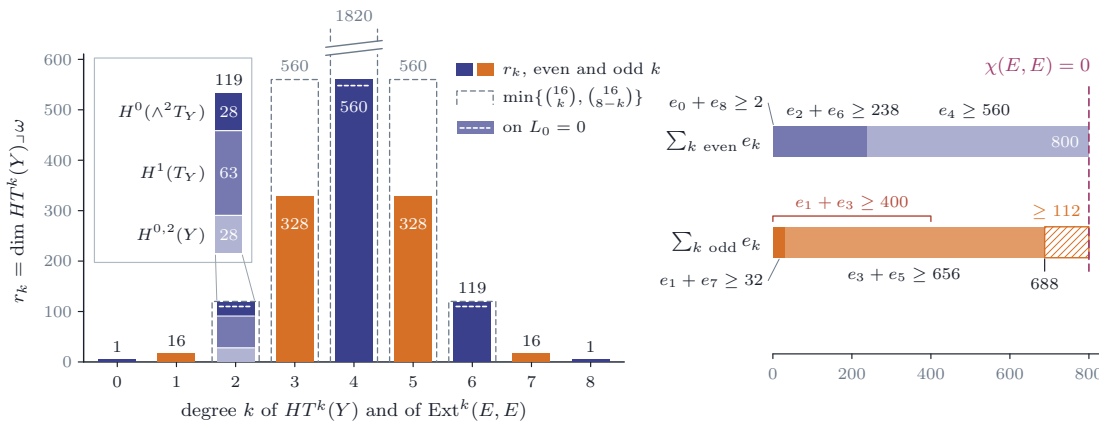
FIGURE 49. Theorem 21.34 . Left: the lower bounds r_k for \dim \text{Ext}^k(E, E) when \text{ch}(E) = N\omega , one bar per degree, symmetric about k = 4 as Lemma 21.33 predicts; the bar at k = 2 is the 119 of Theorem 21.21 , made of 28 classes in H^{0,2} , 63 in H^1(T) and 28 bivectors. On the hyperplane L_0 = 0 the bars at 2, 4 and 6 drop to 110, 548 and 110 at a sample point. Right: \chi(E, E) = 0 balances the even and the odd degrees, so the odd side, which Hochschild cohomology fills only to 688, carries at least 800.
