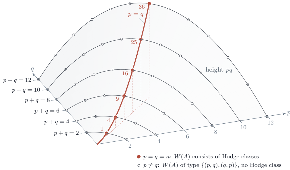
FIGURE 53. The signatures (p, q) of an imaginary quadratic action, with p + q = \dim A , drawn on the surface of height pq , which is the dimension of the family of abelian varieties carrying that action, the unitary Shimura variety of signature (p, q) . Each curve on the surface collects the signatures available in one dimension, and on it the diagonal point is the highest. The divisibility conditions of Theorem C.3 put no constraint on which of them occur when \text{End}^0(A) = K , by Proposition C.9(i) . By Proposition C.7 the Weil line consists of Hodge classes exactly at the filled points on the ridge p = q , and at every open point it is a rational sub-Hodge structure of type \{(p, 2n - p), (2n - p, p)\} carrying no Hodge class at all. The diagonal is the locus that Corollary B.9 shows to be an algebraic subvariety of the moduli.
