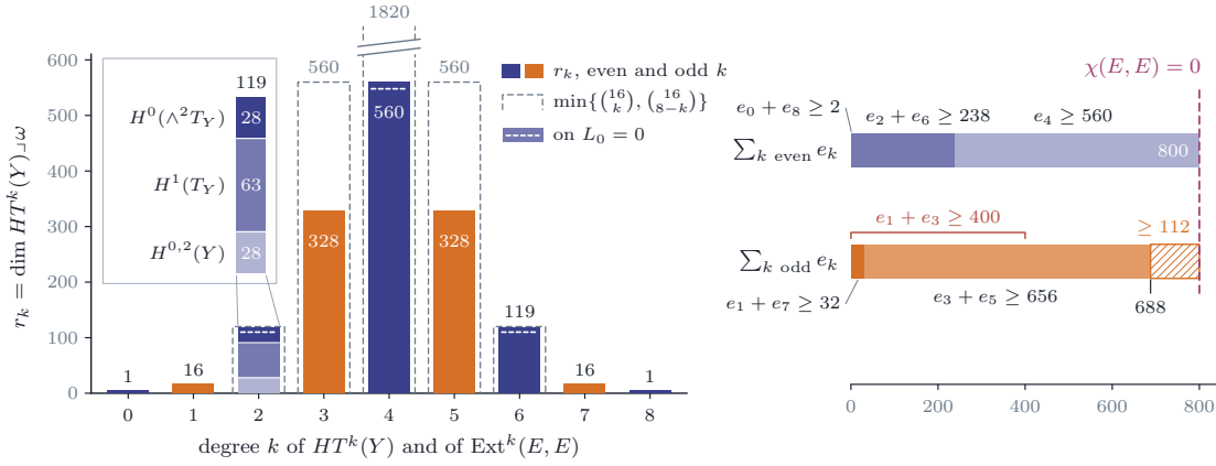
FIGURE 35. Theorem 21.31 . Left: the lower bounds r_k for \dim \text{Ext}^k(E, E) when \text{ch}(E) = N\omega , one bar per degree, symmetric about k = 4 as Lemma 21.30 predicts; the bar at k = 2 is the 119 of Theorem 21.21 , made of 28 classes in H^{0,2} , 63 in H^1(T) and 28 bivectors. On the hyperplane L_0 = 0 the bars at 2, 4 and 6 drop to 110, 548 and 110 at a sample point. Right: \chi(E, E) = 0 balances the even and the odd degrees, so the odd side, which Hochschild cohomology fills only to 688, carries at least 800.
