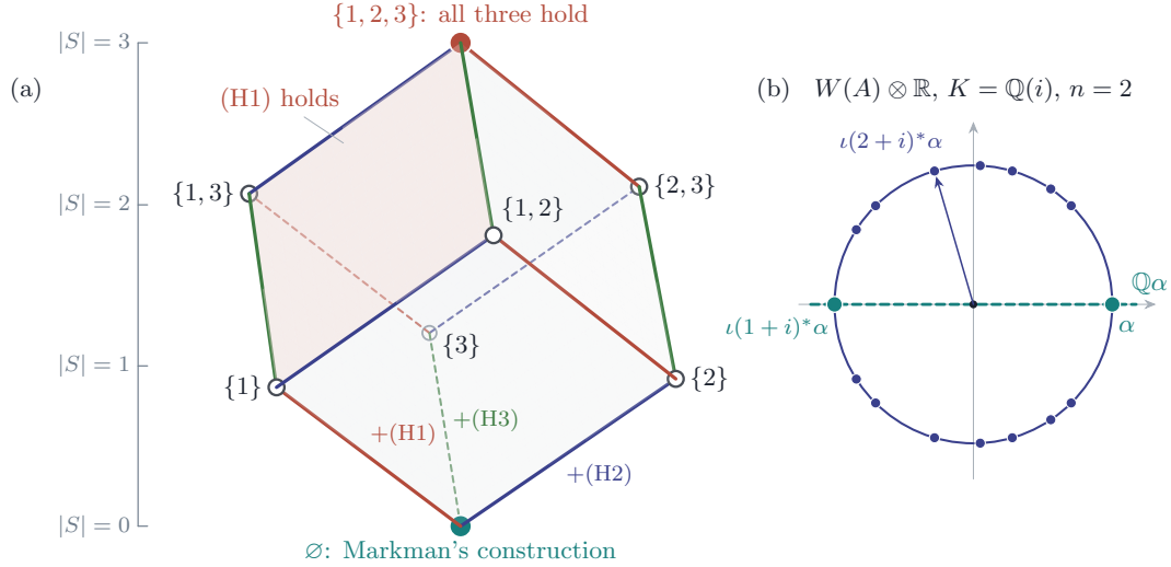
FIGURE 11. (a) The eight positions a construction can occupy, drawn as the Boolean lattice of the subsets S of three hypotheses: (H1) the Chern character of the input lies in the subring generated by divisor classes; (H2) the output is a K^\times -eigenclass; (H3) the output spans a single line rather than a plane. (H1) and (H2) are the hypotheses negated in (i) and (iii) of Proposition 13.5 , and (H3) is what Corollary 13.2 excludes for a nonzero Weil class. At the top vertex all three hold, and both Theorem 1.1 and Theorem 1.3 apply; on the shaded face (H1) holds, and Theorem 1.1 alone already applies. Markman's construction sits at the bottom vertex, where none of the three holds. (b) The orbit of a Weil class \alpha under K^\times for K = \mathbb{Q}(i) and n = 2 , in W(A) \otimes \mathbb{R} \cong \mathbb{C} and normalised to the unit circle. Since \iota(\tau)^* acts through \tau^4 , the class \iota(1+i)^*\alpha = -4\alpha stays on the line \mathbb{Q}\alpha , while \iota(2+i)^*\alpha , with (2+i)^4 = -7 + 24i , does not; the orbit spans the plane, as Proposition 13.1 asserts.
