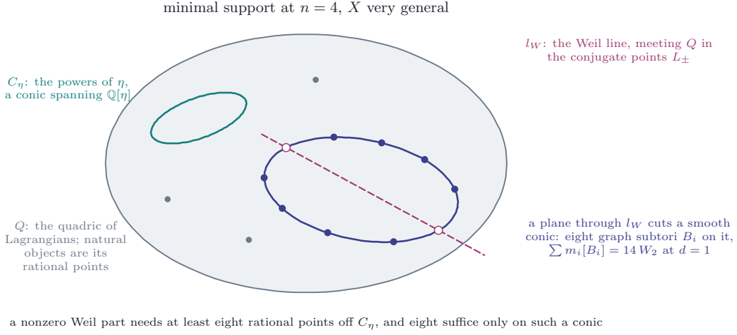
FIGURE 24. Theorem 17.25. The quadric Q of Lagrangians; the rational points are the Chern characters of the natural objects on the split member at n = 4 , up to the Veronese map \nu_4 . The powers of the polarisation fill the conic C_\eta (teal), and the Weil line is spanned by the conjugate points L_\pm (open circles) in which the line l_W (dashed) meets Q . A combination of natural characters with a nonzero Weil part needs at least eight rational points off C_\eta , and with eight they lie on one conic cut out by a plane through l_W (indigo), such as the eight graph subvarieties B_i of Example 17.26 ; the grey points are natural objects off any such conic, which no relation of this size can use.
