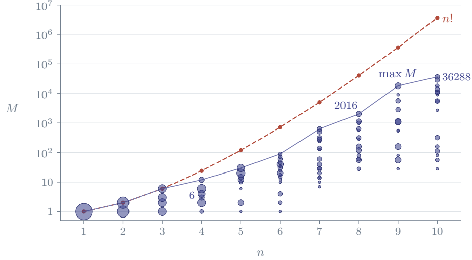
FIGURE 14. Remark 14.14. The least multiple M of Theorem 14.13 for 1 \leq n \leq 10 , over the seventy-two cases d \in \{1, 2, 3, 5, 7, 11\} , a \in \{1, 2, 3\} , b \in \{\pm 1, \pm 2\} for each n , on a logarithmic scale; the area of a disc counts the cases with that value. The solid line joins the largest values and the dashed one is n! , which every M divides: the quotient of \mathbb{Z}^{n+1} by the lattice of the characters (1, j, \dots, j^n) of the powers of a line bundle is dual to the integer-valued polynomials of degree at most n , spanned by the \binom{x}{k} , whose coefficients have denominators dividing n! .
