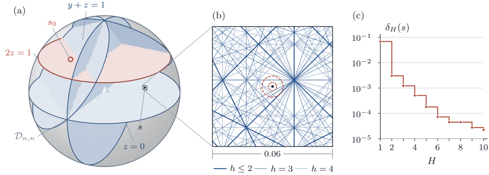
FIGURE 19. The dichotomy of Corollary 16.5. Each stratum \Sigma_{P,q} is Zariski closed by Theorem 16.4, and there are countably many of them; the base point s_0 of Theorem 15.27 lies on one. By Proposition 16.7 the union of the strata is dense, so every neighbourhood of a point s lying off all of them meets infinitely many strata. The conjecture for the family is the assertion that no such s exists, and by Corollary 16.5 it is enough that one stratum has nonempty interior.
