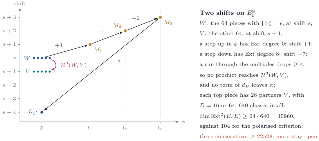
FIGURE 28. Lemma 18.38 and Theorem 18.39, in the placement p < t_1 < t_2 < t_3 . Horizontal: the value \phi of a piece; vertical: its shift. The pieces L_\zeta with \prod \zeta = \epsilon sit at the shift s and the others at s - 1 . A run through the multiples, up three times with Ext degree 0 and down once with Ext degree 8, ends four shifts lower, the least drop of Lemma 18.38(iii), so it never joins a top piece W to a partner V one shift lower; the group \mathcal{H}^3(W, V) survives in \text{Ext}^2(E, E) .
