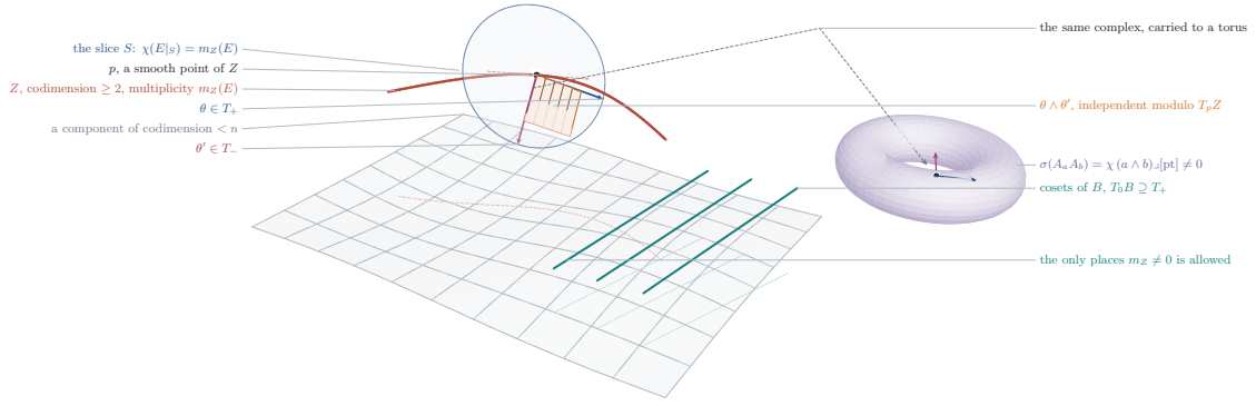
FIGURE 21. The proof of Theorem 16.38 . The grey sheet stands for a component of the support of codimension less than n , which the theorem forces to exist; the clay curve Z for a component of codimension at least two. At a smooth point p of Z the directions \theta \in T_+ and \theta' \in T_- span the slice S , transverse to Z , on which E restricts to a complex of finite length with Euler characteristic m_Z(E) ; the amber parallelogram is the bivector \theta \wedge \theta' , independent modulo T_p Z . Carried to a torus of the same dimension, the product of the two jet classes is seen by the semiregularity map as m_Z(E) times the class of a point contracted with the bivector, which is not zero, so m_Z(E) = 0 or the bivector degenerates. The teal lines are cosets of an abelian subvariety B tangent to T_+ , the only components of codimension at least two on which a nonzero multiplicity survives. The scene is schematic in the dimensions and exact in the incidences.
