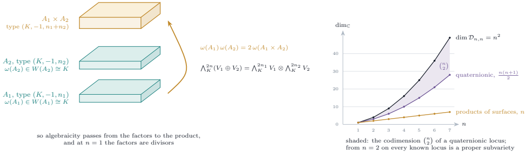
FIGURE 17. Theorem 15.7 and its reach. Left: the Weil line of each factor is a K -line, the Weil line of the product is the tensor product of the two over K , and in the K -valued notation the class is multiplicative up to the factor 2. Algebraicity therefore passes from the factors to the product, and at n = 1 the factors are divisor classes, so a product of n abelian surfaces of Weil type carries an explicit algebraic Weil class in every dimension. Right: the dimensions of the loci on which the class is known to be algebraic, against the dimension n^2 of the family. Both the quaternionic locus and the product locus are proper subvarieties once n \geq 2 , and a general member lies on neither.
