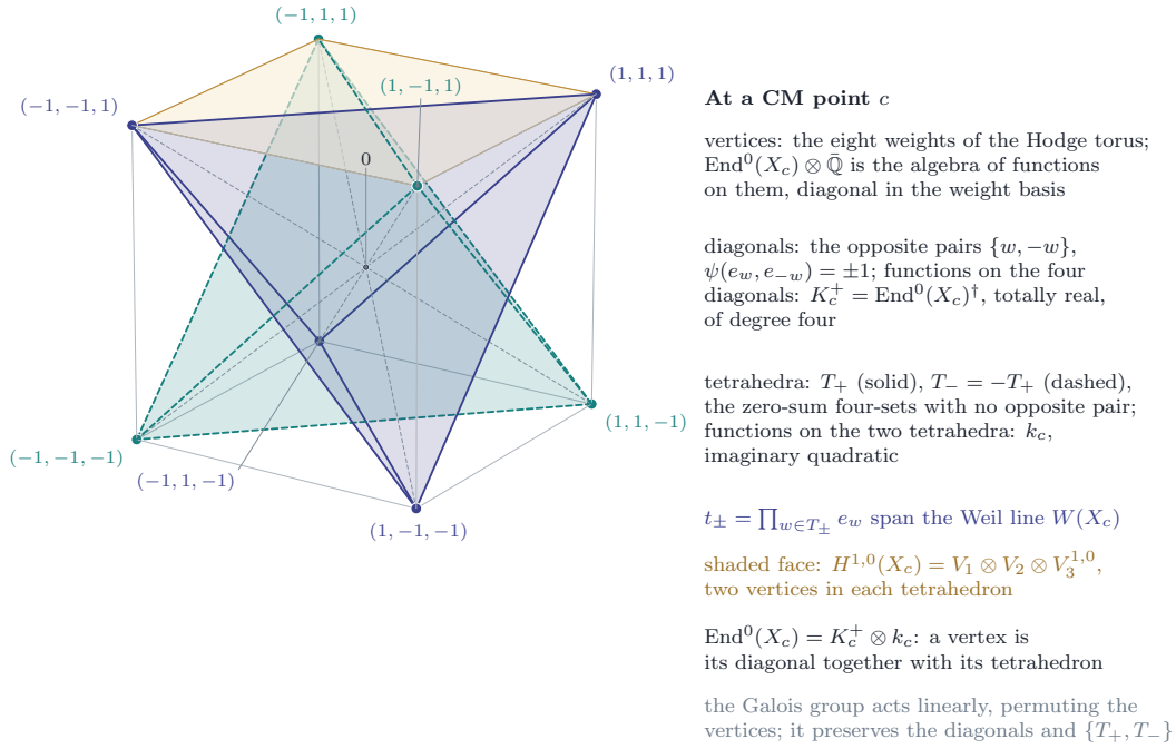
FIGURE 43. Proposition 21.29(i). The eight weights (\pm 1, \pm 1, \pm 1) of the Hodge torus at a CM point are the vertices of a cube. The four diagonals are the pairs of opposite weights, paired by the polarisation; the two inscribed tetrahedra T_+ (an even number of entries -1 ) and T_- = -T_+ are the only zero-sum four-sets without an opposite pair, and t_{\pm} = \prod_{w \in T_{\pm}} e_w span the Weil line. The Galois group acts by linear maps permuting the vertices, so it preserves the diagonals and the pair of tetrahedra: the functions constant on the tetrahedra form the imaginary quadratic Weil field k_c , those constant on the diagonals the totally real quartic algebra K_c^+ of Rosati-fixed endomorphisms, and \text{End}^0(X_c) = K_c^+ \otimes k_c because a vertex is determined by its diagonal and its tetrahedron.
