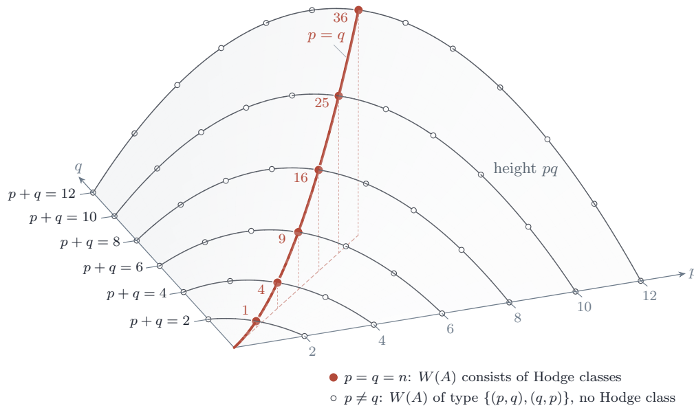
FIGURE 50. The signatures (p, q) of an imaginary quadratic action, with p + q = \dim A , drawn on the surface of height pq , which is the dimension of the family of abelian varieties carrying that action, the unitary Shimura variety of signature (p, q) . Each curve on the surface collects the signatures available in one dimension, and on it the diagonal point is the highest. The divisibility conditions of Theorem C.3 put no constraint on which of them occur when \text{End}^0(A) = K , by Proposition C.9(i) . By Proposition C.7 the Weil line consists of Hodge classes exactly at the filled points on the ridge p = q , and at every open point it is a rational sub-Hodge structure of type \{(p, 2n - p), (2n - p, p)\} carrying no Hodge class at all. The diagonal is the locus that Corollary B.9 shows to be an algebraic subvariety of the moduli.
