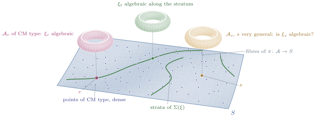
FIGURE 48. Theorem 22.5 in one family. The sheet is the base S of a polarised abelian scheme \pi: \mathcal{A} \rightarrow S through a given Hodge class, as in Proposition 22.4 ; the small dots are its points of CM type, dense by Lemma 22.3 , and the green curves are strata of the algebraic locus \Sigma(\xi) of the flat class \xi ( Lemma 22.2 ). Above three points the fibres are drawn as tori, and the loop on each stands for \xi , carried from fibre to fibre by parallel transport. At the CM member \mathcal{A}_c the class is algebraic, and it stays algebraic along the stratum through c . At a very general member \mathcal{A}_s it is algebraic exactly when \Sigma(\xi) has an interior point, and (F2) is the statement that this happens in every such family.
