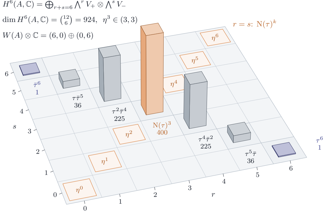
FIGURE 6. The K^\times -grading at n = 3 on the grid of pairs (r, s) , 0 \leq r, s \leq 6 . The summands \bigwedge^r V_+ \otimes \bigwedge^s V_- of H^6(A, \mathbb{C}) lie on the antidiagonal r + s = 6 and are drawn at their dimensions \binom{6}{r}\binom{6}{s} , which sum to \binom{12}{6} = 924 ; on the summand (r, s) the group K^\times acts by \tau^r \bar{\tau}^s . The two end cells (6, 0) and (0, 6) , with characters \tau^6 and \bar{\tau}^6 , span the Weil line; the middle cell (3, 3) , with character N(\tau)^3 , contains \eta^3 . The outlined cells on the diagonal r = s are the summands on which K^\times acts through a power of the norm, and they carry the powers \eta^k . That the end cells and the middle cell differ is the content of Theorem 5.6 .
