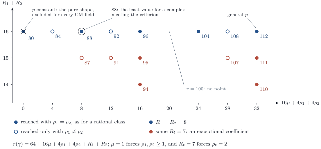
FIGURE 30. The rank r(\gamma) of Theorem 19.24, over the plane of the Hankel part 16\mu + 4\rho_1 + 4\rho_2 and of R_1 + R_2 . The fifteen points are the tuples allowed by the two conditions of the theorem, and each carries its value. Filled points are reached with \rho_1 = \rho_2 , as the character of a complex with rational coefficients is (Corollary 19.25(ii)); red points need an exceptional coefficient at one place at least. The value 80 is the pure shape, excluded for every CM field by Theorem 19.14; so 88 is the least rank a complex meeting the criterion can have. The level r = 100 meets no point.
