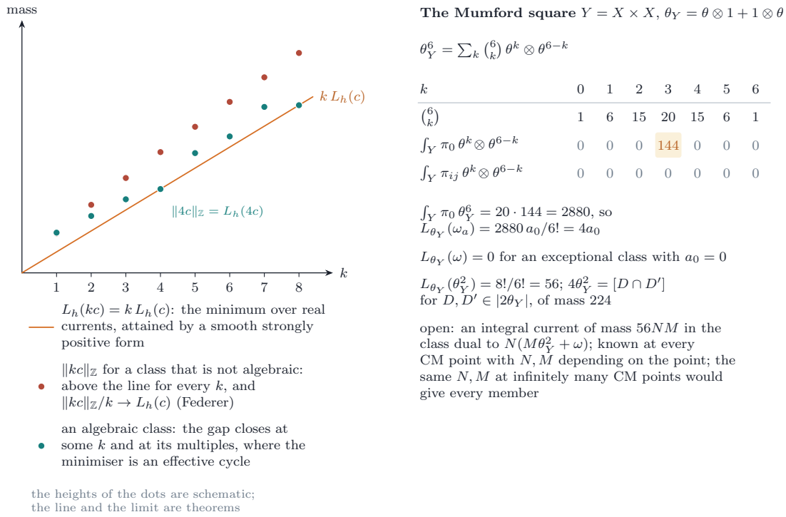
FIGURE 42. Theorem 20.68 and Example 20.69 . Left: the mass of a current in the class dual to kc against k . The line k L_h(c) is the minimum over closed real normal currents, attained by a smooth strongly positive form; the minima over closed integral currents lie on or above it, with \|kc\|_{\mathbb{Z}}/k \rightarrow L_h(c) by Federer's theorem, and for M large the class is algebraic exactly when one of them lies on the line, where the minimiser is an effective algebraic cycle. The heights of the dots are schematic. Right: the numbers of the Mumford square, computed in the split model of [BMB26] . Of the seven terms \binom{6}{k} \theta^k \otimes \theta^{6-k} of \theta_Y^6 only k = 3 pairs with \pi_0 = \frac{1}{4} \theta \otimes \theta , giving 20 \cdot 144 = 2880 , and none pairs with the primitive summands; so L_{\theta_Y}(\omega_a) = 4a_0 , the Wirtinger bound of an exceptional class with a_0 = 0 is zero, and the perturbation of NM\theta_Y^2 by N\omega changes the bound 56NM by nothing.
