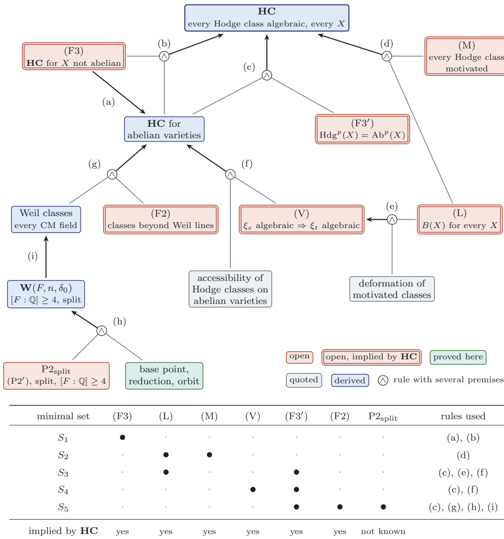
FIGURE 37. The rule set of Setup 20.57 with the rules of Section 20.6 , drawn as a hypergraph. A rule with several premises is a junction marked \wedge , joined to its premises and with one arrow to its conclusion. The letters name the results that prove the rules: (a) is Proposition 20.35 ; (b) and (g) are the closure map of Section 20.5 ; (c) is Proposition 20.37(i) ; (d) is Proposition 20.17 ; (e) is Proposition 20.18 ; (f) is Theorem 20.19 ; (h) is Theorem 19.6 ; and (i) is the chain of Proposition 20.13 , Proposition 20.12 , Proposition 19.3 and Appendix C . Clay marks an open statement, a double frame an open statement that the conjecture implies, grass what this paper proves, slate what it quotes, and indigo a derived statement. The table lists the five minimal sufficient sets of Theorem 20.58(ii) , the rules each of them uses, and which of the open statements the conjecture implies; only P2_{\text{split}} , which asks for a particular complex, is not known to follow from it. The secant route, which reaches the imaginary quadratic families only, is drawn in Figure 38 .
