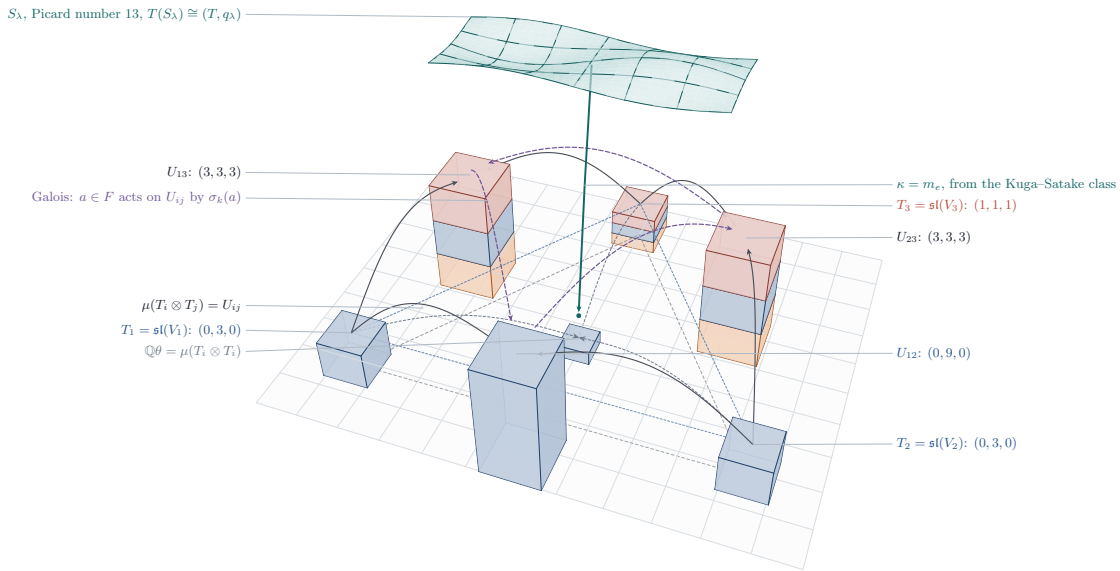
FIGURE 40. Proposition 21.2 and Lemma 21.3 , drawn over the triangle of the three factors of the Hodge group; every height is a dimension. At the corners stand the summands T_i = \mathfrak{sl}(V_i) of T = \text{Lie } G , banded by Hodge type after the Tate twist T(-1) : blue for (1, 1) , clay for (2, 0) and amber for (0, 2) , so that only T_3 carries the K3 type. On the edges stand the three summands U_{ij} of the primitive part of H^2(X) , of dimension nine, U_{12} of pure type (1, 1) and the other two in three bands of three; in the middle is the line of \theta . The solid arcs are the product map \mu , which carries T_i \otimes T_j onto U_{ij} , and the dashed ones carry T_i \otimes T_i to \mathbb{Q}\theta . The violet arcs are the Galois group permuting the U_{ij} as it permutes the embeddings of F , which is why the two exceptional classes may be taken to be the trace-zero part of a cubic field. Above, the K3 surface S_\lambda of Theorem 21.4 , whose Kuga–Satake class, if algebraic, comes down to T as the map \kappa = m_e .
