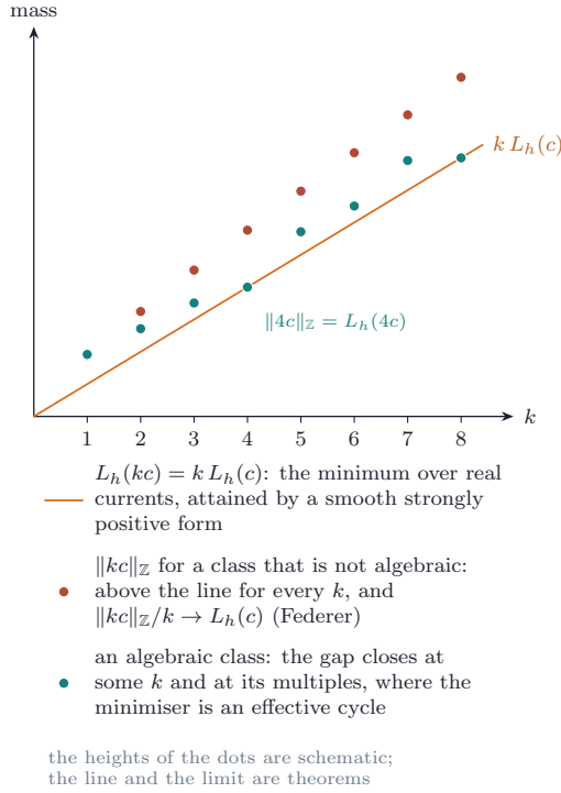
FIGURE 54. Theorem 20.76 and Example 20.77. Left: the mass of a current in the class dual to kc against k . The line k L_h(c) is the minimum over closed real normal currents, attained by a smooth strongly positive form; the minima over closed integral currents lie on or above it, with \|kc\|_{\mathbb{Z}}/k \rightarrow L_h(c) by Federer's theorem, and for M large the class is algebraic exactly when one of them lies on the line, where the minimiser is an effective algebraic cycle. The heights of the dots are schematic. Right: the numbers of the Mumford square, computed in the split model of [BMB26]. Of the seven terms \binom{6}{k} \theta^k \otimes \theta^{6-k} of \theta_Y^6 only k = 3 pairs with \pi_0 = \frac{1}{4} \theta \otimes \theta , giving 20 \cdot 144 = 2880 , and none pairs with the primitive summands; so L_{\theta_Y}(\omega_a) = 4a_0 , the Wirtinger bound of an exceptional class with a_0 = 0 is zero, and the perturbation of NM\theta_Y^2 by N\omega changes the bound 56NM by nothing.
