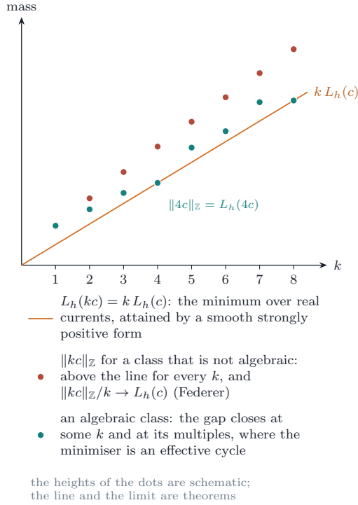
FIGURE 53. Theorem 20.78 and Example 20.79 . Left: the mass of a current in the class dual to kc against k . The line k L_h(c) is the minimum over closed real normal currents, attained by a smooth strongly positive form; the minima over closed integral currents lie on or above it, with \|kc\|_{\mathbb{Z}}/k \rightarrow L_h(c) by Federer's theorem, and for M large the class is algebraic exactly when one of them lies on the line, where the minimiser is an effective algebraic cycle. The heights of the dots are schematic. Right: the numbers of the Mumford square, in the split model. Of the seven terms \binom{6}{k} \theta^k \otimes \theta^{6-k} of \theta_Y^6 only k = 3 pairs with \pi_0 = \frac{1}{4} \theta \otimes \theta , giving 20 \cdot 144 = 2880 , and none pairs with the primitive summands; so L_{\theta_Y}(\omega_a) = 4a_0 , the Wirtinger bound of an exceptional class with a_0 = 0 is zero, and the perturbation of NM\theta_Y^2 by N\omega changes the bound 56NM by nothing.
