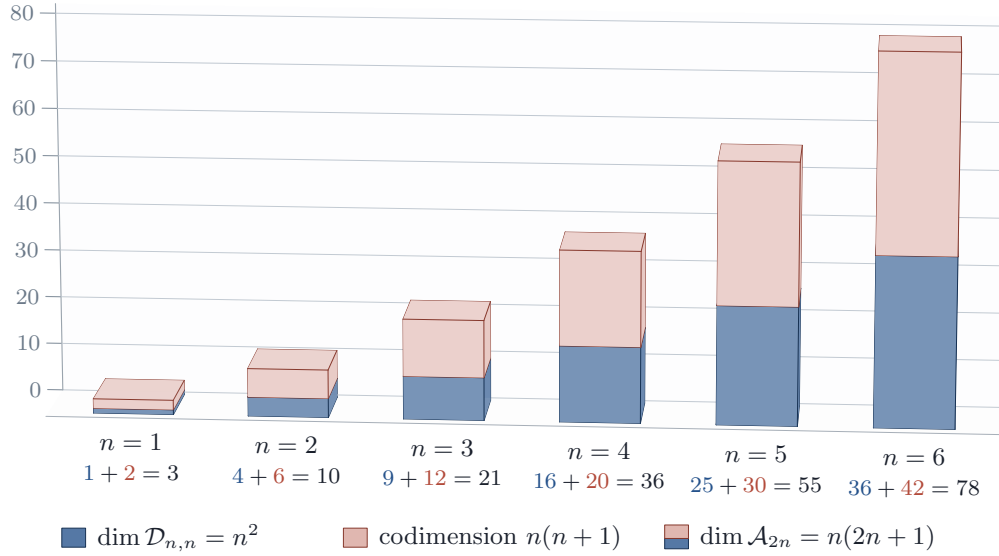
FIGURE 10. The Weil locus inside the moduli of principally polarised abelian 2n -folds, for n = 1, \dots, 6 . Each prism has the height n(2n+1) of the moduli space \mathcal{A}_{2n} ; its lower part, of height n^2 , is the dimension of the period domain \mathcal{D}_{n,n} of Proposition B.8, and its upper part is the codimension n(n+1) . The codimension grows quadratically, so the Weil locus is thin, and by Corollary B.9 it is an algebraic subvariety. Both facts matter for propagation: the locus along which one would have to deform is small and is a variety, but neither fact produces a cycle on it.
