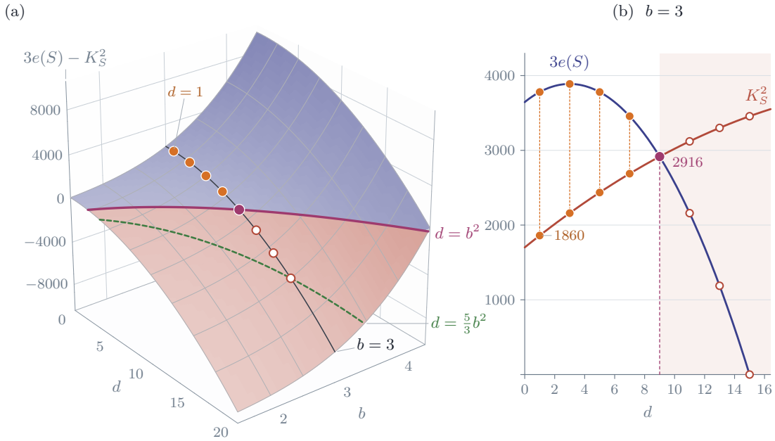
FIGURE 25. Theorem 18.40 over the quarter plane of (b, d) . The height of the surface is the defect 3e(S) - K_S^2 = 24(b^4 - d^2) in the Bogomolov–Miyaoka–Yau inequality for the surface the theorem attaches to the pair, compressed by a signed cube root so that four orders of magnitude fit one frame; the compression is odd and monotone, so the zero locus and the sign are the true ones. The surface is drawn indigo where the defect is positive and clay where it is negative, and it crosses zero along d = b^2 , which is therefore the whole content of the inequality. The weaker wall d = \frac{5}{3}b^2 , where e(S) itself changes sign, is drawn dashed and lies above it. On the line b = 3 , which is the value Proposition 18.25(iii) forces on the fourfold, the four squarefree discriminants d = 1, 3, 5, 7 with N an integer sit above the wall and are marked with their drop lines; d = 9 sits exactly on it, the equality case, and d = 11, 13, 15 sit below and are excluded.
