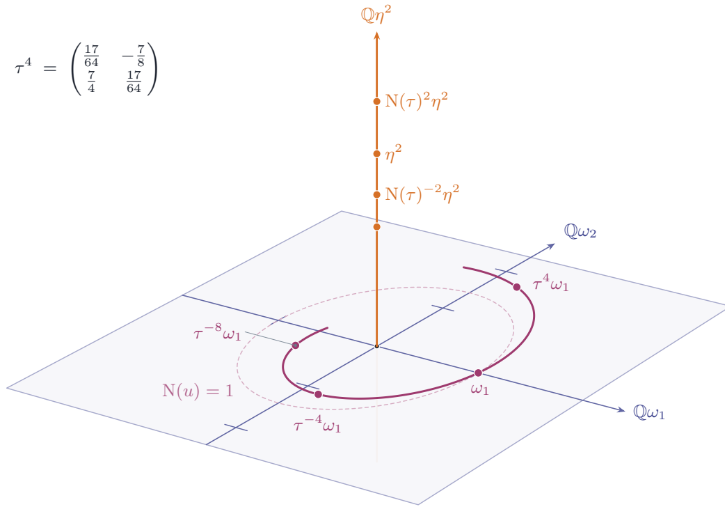
FIGURE 4. The linear algebra behind Theorem 1.1 , drawn inside H^{2n}(A, \mathbb{Q}) . The Weil line W(A) is a plane, free of rank one over K and of rank two over \mathbb{Q} , and K^\times acts on it through \tau^{2n} , so the orbit of any nonzero class is a spiral that spans the plane and lies on no line in it. The transverse axis carries \eta^n , on which K^\times acts through the norm. A construction returning a single eigenclass returns a line, and by Proposition 13.1 no line inside W(A) is stable.
