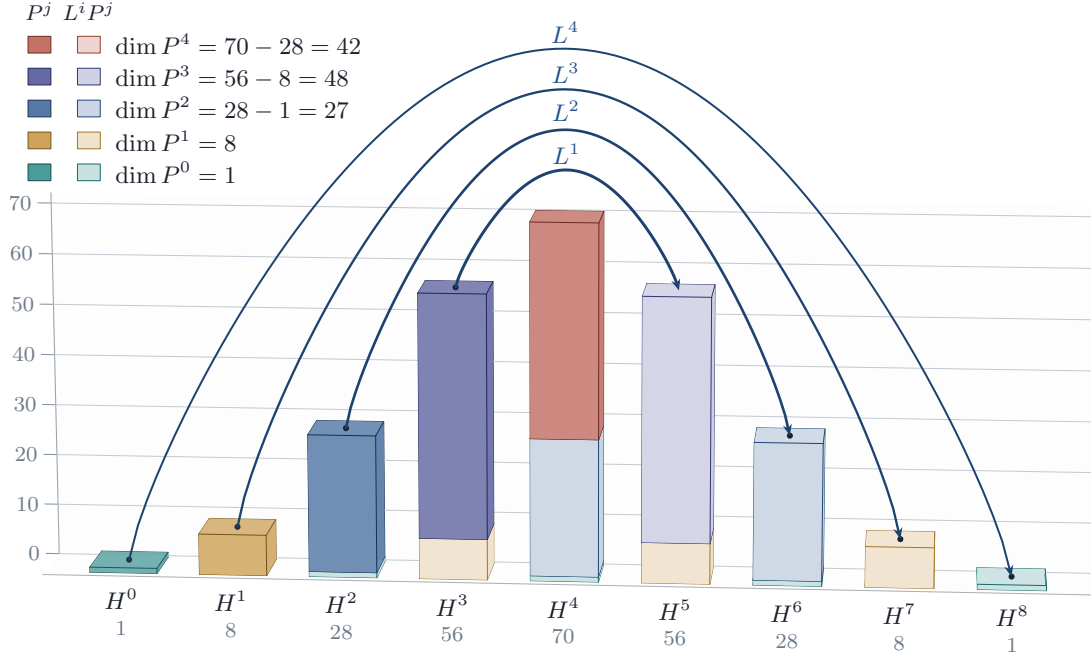
FIGURE 8. The Betti numbers \binom{8}{k} of an abelian fourfold, drawn as prisms and divided according to the Lefschetz decomposition H^k = \bigoplus_i L^i P^{k-2i} ; the primitive part P^k is drawn dark, and each image L^i P^{k-2i} is drawn light in the colour of P^{k-2i} . The arcs are the hard Lefschetz isomorphisms L^{4-k}: H^k \rightarrow H^{8-k} . Below the middle degree the restriction j^* to a smooth ample hypersurface is injective and a class descends, but the return trip j_* j^* multiplies by L , and recovering the class is the Lefschetz standard conjecture; above the middle degree a class is carried to the lower half by an arc. The primitive middle cohomology P^4 , of dimension 70 - 28 = 42 , is annihilated by j^* (Theorem 1.4), and neither an arc nor a restriction reaches it.
