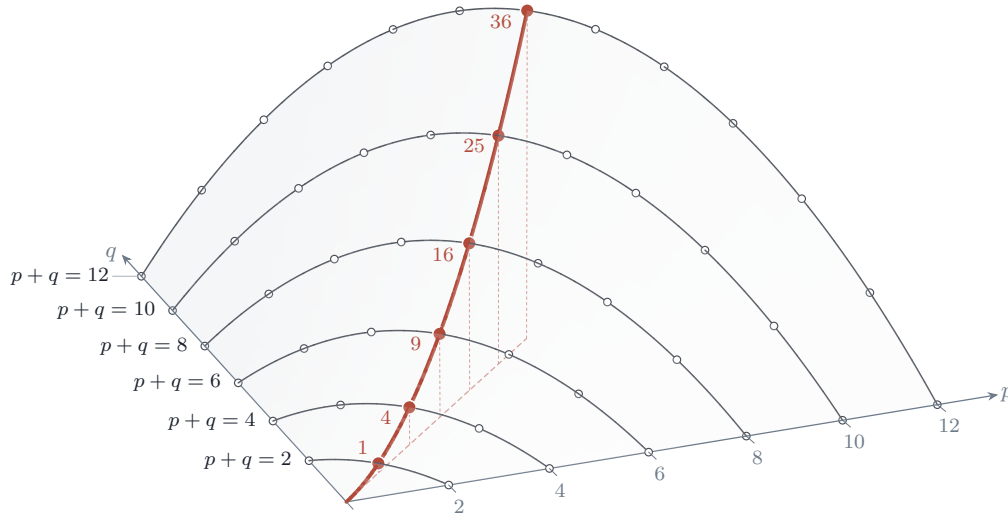
FIGURE 36. The signatures (p, q) of an imaginary quadratic action, with p + q = \dim A , drawn on the surface of height pq , which is the dimension of the family of abelian varieties carrying that action, the unitary Shimura variety of signature (p, q) . Each curve on the surface collects the signatures available in one dimension, and on it the diagonal point is the highest. The divisibility conditions of Theorem C.3 put no constraint on which of them occur when \text{End}^0(A) = K , by Proposition C.9(i) . By Proposition C.7 the Weil line consists of Hodge classes exactly at the filled points on the ridge p = q , and at every open point it is a rational sub-Hodge structure of type \{(p, 2n - p), (2n - p, p)\} carrying no Hodge class at all. The diagonal is the locus that Corollary B.9 shows to be an algebraic subvariety of the moduli.
