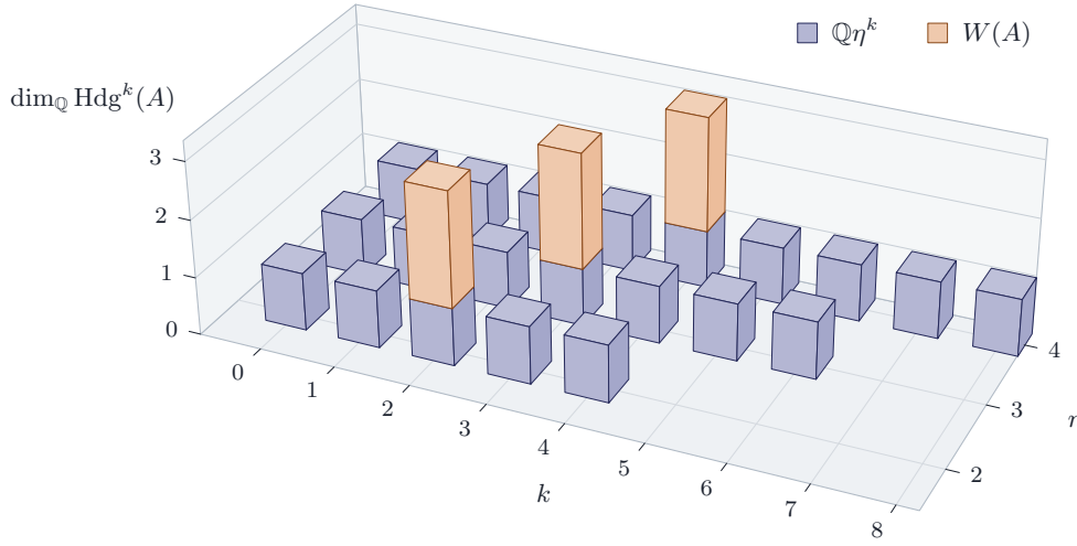
FIGURE 2. The dimensions of \mathrm{Hdg}^k(A) for a general abelian variety of (K, -1, n) -Weil type, 0 \leq k \leq 2n , at n = 2, 3, 4 , as computed in Theorem 4.14 . Every degree carries the line \mathbb{Q}\eta^k ; the middle degree k = n carries in addition the two dimensions of the Weil line W(A) , and nothing else occurs. The profile is the same for every n .
