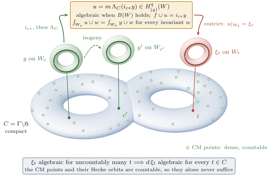
FIGURE 29. Theorem 20.29(ii) along a compact Shimura curve C . An algebraic class y on one fibre, at a base point of a Weil family or at a CM point of a Mumford family (hollow dots: the CM points, countable and dense), is pushed into W by the Gysin map and brought back to the invariant summand by the base operator \Lambda_C . When B(W) holds the result u is an algebraic class on W , pinned down by the displayed pairing against the invariant classes, and its restriction to a very general fibre is the invariant part of y . The dashed arcs are isogenies between CM members along Hecke orbits: they carry algebraic classes to algebraic classes but reach only countably many points, and Lemma 20.28 , in the box, needs uncountably many. This is how Corollary 20.32 and Corollary 20.31 turn each target into one case of (L).
