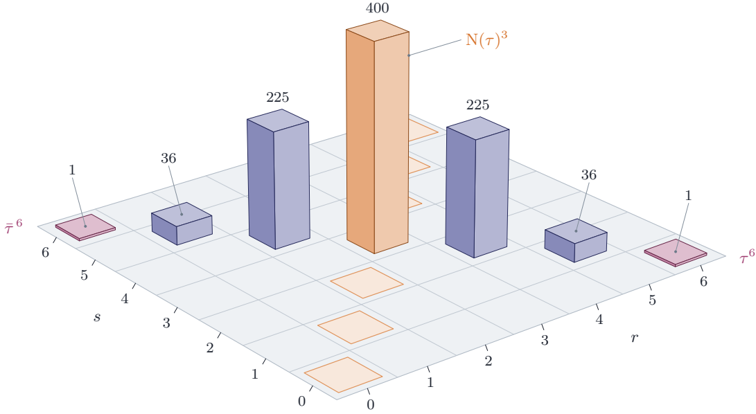
FIGURE 3. The K^\times -grading at n = 3 on the grid of pairs (r, s) , 0 \leq r, s \leq 6 . The summands \bigwedge^r V_+ \otimes \bigwedge^s V_- of H^6(A, \mathbb{C}) lie on the antidiagonal r + s = 6 and are drawn at their dimensions \binom{6}{r} \binom{6}{s} , which sum to \binom{12}{6} = 924 ; on the summand (r, s) the group K^\times acts by \tau^r \bar{\tau}^s . The two end cells (6, 0) and (0, 6) , with characters \tau^6 and \bar{\tau}^6 , span the Weil line; the middle cell (3, 3) , with character N(\tau)^3 , contains \eta^3 . The outlined cells on the diagonal r = s are the summands on which K^\times acts through a power of the norm, and they carry the powers \eta^k . That the end cells and the middle cell differ is the content of Theorem 1.3 .
