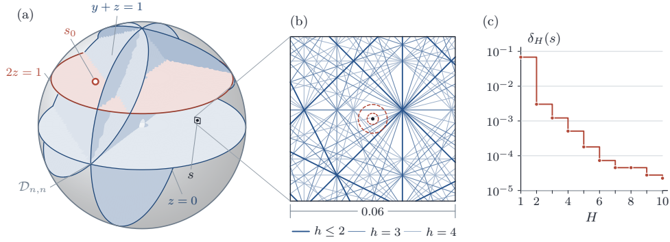
FIGURE 16. The dichotomy of Corollary 16.5 . Each stratum \Sigma_{\underline{p}, \underline{q}} is Zariski closed by Theorem 16.4 , and there are countably many of them; the base point s_0 of Theorem 15.27 lies on one. By Proposition 16.7 the union of the strata is dense, so every neighbourhood of a point s lying off all of them meets infinitely many strata. The conjecture for the family is the assertion that no such s exists, and by Corollary 16.5 it is enough that one stratum has nonempty interior.
