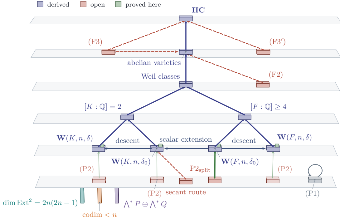
FIGURE 31. The route of this paper in Theorem 20.45 , drawn as a stack of plates, one per level of the derivation; the other routes of the literature are drawn in Figure 30 . The spine in indigo runs from the Weil families at the bottom to the conjecture at the top. The two statements (F2) and (F3) enter in clay from the right, each at the level where it is needed; (F2) is the conjecture for a class of Hodge classes that no Weil line reaches, not a reduction, and (F3) is the whole conjecture ( Proposition 20.35 ), so the route drawn is minimal only with (F3) replaced by (F3') of Definition 20.36 . From below, the propagation statement (P2) in grass reaches the two discriminant cases of the quadratic fields and the fields of higher degree alike, because Theorem 15.27 and Theorem 19.4 put a base point in every family; it is read in the corrected form of Remark 17.6 . The two edges inside the levels are Proposition 20.13 : descent from the trivial discriminant to the others, and scalar extension from the fields of degree at least four to the quadratic fields; with them (P2) is needed only for the split families of the fields of higher degree. The three pillars under the grass node are the results of Theorem 16.36 , Theorem 16.38 and Corollary 16.34 on the first form, in which the Chern character is exactly a Weil class; by Theorem 17.5 that form is never met, so the number on the first pillar is attained by no complex. The secant route in clay reaches the trivial discriminant, since the member it is built on is split, and through descent the rest of the quadratic case; it has no edge to the fields of higher degree. The bounded criterion (P1) is drawn apart, in slate, closed on itself: it is equivalent to its own conclusion.
