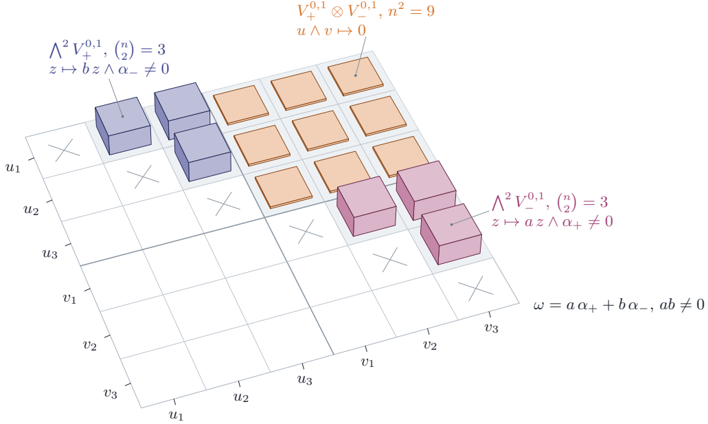
FIGURE 5. The structure behind Lemma 9.6, drawn at n = 3 . H^{0,2}(A) = \bigwedge^2 H^{0,1} splits into three blocks by how many factors come from V_+^{0,1} and how many from V_-^{0,1} . The two outer blocks, of dimension \binom{n}{2} = 3 each, are carried injectively by multiplication with the Weil class. The middle block, of dimension n^2 = 9 and spanned by the mixed products, goes to zero, because each such product repeats a factor of \alpha_+ and a factor of \alpha_- . Its dimension n^2 is the deficit in Proposition 9.10.
