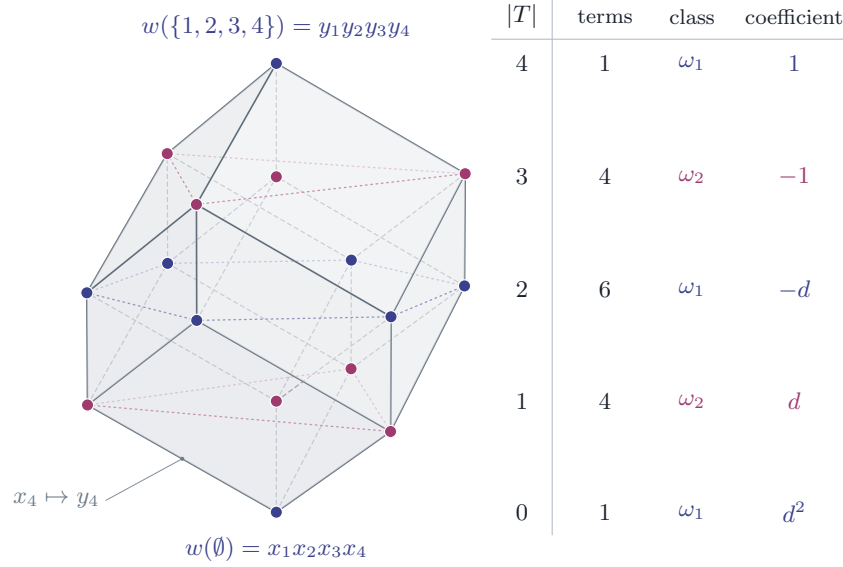
FIGURE 1. The 2^{2n} = 16 monomials w^{(T)} of Notation 4.8 at n = 2 , as the vertices of the 4-cube, projected so that the height of w^{(T)} is |T| . An edge joins two monomials whose index sets differ in one element, that is, two monomials related by a single substitution x_j \mapsto y_j . The two colours are the bipartition by the parity of |T| : the eight even vertices carry \omega_1 and the eight odd ones carry \omega_2 . The coefficient of w^{(T)} depends only on |T| and is given by (13) and (14).
