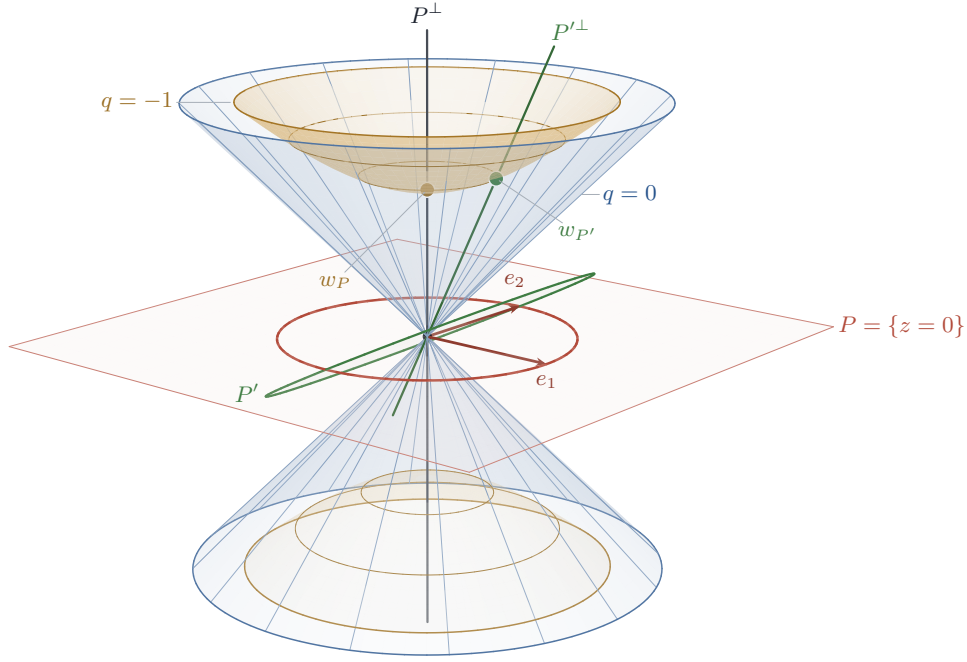
FIGURE 9. The geometry from which the Kuga–Satake construction starts, in the smallest case b = 3 . The quadratic form is q = x^2 + y^2 - z^2 , of signature (2, 1) , with its null cone q = 0 ; the horizontal plane P = \{z = 0\} is positive definite and meets the cone only at the origin. The construction needs such a plane, and Setup 11.1 supplies one: P = \langle \Re\sigma, \Im\sigma \rangle for the period \sigma spanning T^{2,0} . An orthonormal basis e_1, e_2 of P gives J = e_1 e_2 with J^2 = -1 by Lemma 11.4 , and J is the complex structure of \text{KS}(T) . A positive definite plane P is determined by the negative line P^\perp , which meets the upper sheet of the hyperboloid q = -1 in one point w_P ; that sheet is the period domain, and a second plane P' with its point w_{P'} is drawn for comparison. The hypothesis behind all of this is \dim T^{2,0} = 1 , and by Proposition 11.11 an abelian variety of Weil type with Hodge group \text{SU}(V, H) supplies it in H^2 only when n = 1 , or n = 2 at trivial discriminant.
