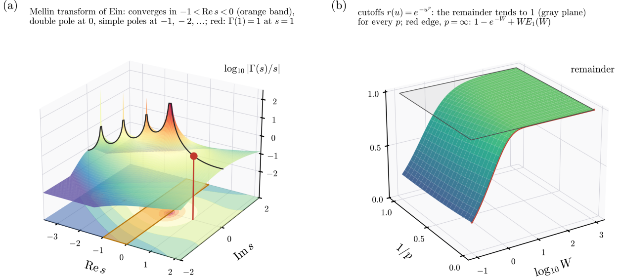
FIG. 12. The finite zero-point energy. (a) \log_{10} |\Gamma(s)/s| over the complex s plane, the Mellin transform (79) of Ein. The integral converges in the strip -1 < \text{Re } s < 0 (orange band on the floor, which also carries the contours of the surface); its continuation has a double pole at s = 0 and simple poles at s = -1, -2, \dots (black curve along the real axis), and is regular at s = 1 , where it equals 1 (red). That value is the whole answer (80). (b) The integral \int_0^\infty \text{Ein}(w) r(w/W) dw with the cutoffs r(u) = e^{-u^p} , after the terms that grow with W are subtracted, \tilde{r}(1) W \log W + [\tilde{r}'(1) + \gamma_E \tilde{r}(1)] W , with \tilde{r} the Mellin transform of r . The surface is drawn over \log_{10} W and 1/p \in [0, 1] . The coefficients of the subtracted terms depend on p , the remainder does not: it tends to 1 (gray plane) for every p , and at W = 10^3 it lies within 10^{-3} of 1 across the whole family. The red edge 1/p = 0 is the sharp cutoff, where the remainder is 1 - e^{-W} + WE_1(W) .
