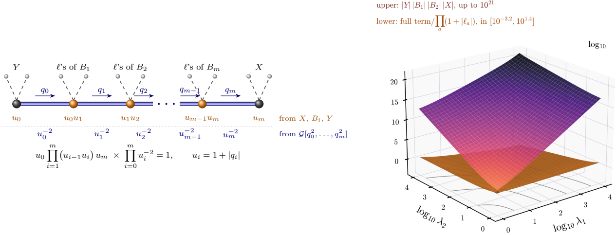
FIG. 9. The chain behind the vertex bound. (a) A function of the covariant d'Alembertian between two field monomials, X\mathcal{G}(-\square)Y , expanded as in Eq. (61). Each insertion B_i of the field-dependent part of \square attaches legs (dashed, gray balls) and changes the running momentum from q_{i-1} to q_i ; the function enters only through the divided difference \mathcal{G}[q_0^2, \dots, q_m^2] . By Eq. (64) each insertion costs one power of the running momentum on each side of it (orange), and Y and X one power each; by Eq. (62) the divided difference returns u_i^{-2} for every segment (blue). The running momenta cancel exactly, and only the legs are left. (b) A numerical check of this bookkeeping for a chain with two insertions and n = 4 , in units M = 1 . The running momenta are q_0 = \ell_Y with |q_0| = 1 , q_1 = q_0 + \ell_1 with |q_1| \simeq \lambda_1 , and q_2 = q_1 + \ell_2 with |q_2| \simeq \lambda_2 ; each insertion is given its largest size (|q_{i-1}| + |\ell_i|)^2 and X, Y the sizes u_2, u_0 . The upper surface is \log_{10} of the product of these sizes, which grows like the fifth power of the momenta, to 10^{21} ; the lower surface is \log_{10} of the full term, with the exact divided difference of the skeleton's \hat{\mathcal{G}} , divided by (1 + |\ell_1|)(1 + |\ell_2|) . It stays between 10^{-3.2} and 10^{1.4} over the four decades in \lambda_1 and \lambda_2 .
