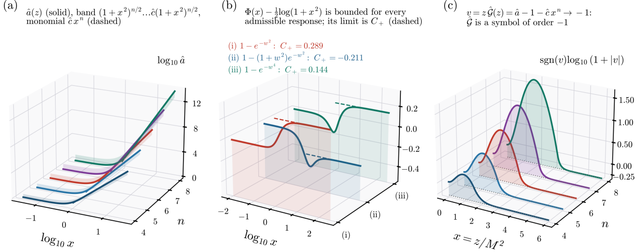
FIG. 5. The skeleton on the real axis. (a) \log_{10} \hat{a}(z) for n = 4, \dots, 8 (solid) inside the band of the two-sided bound (23), (1+x^2)^{n/2} \leq \hat{a} \leq \hat{c}(1+x^2)^{n/2} (shaded), with the monomial \hat{c}x^n that \hat{a} approaches at large x (dashed). (b) \Phi(x) - \frac{1}{2}\log(1+x^2) for the three admissible responses of Table I: it is bounded for each of them, as Eq. (29) states, and tends to the constant C_+ (dashed) of Eq. (30). (c) v = z\hat{\mathcal{G}}(z) = \hat{a} - 1 - \hat{c}x^n for n = 4, \dots, 8 , plotted as \text{sgn}(v)\log_{10}(1+|v|) : it is bounded and tends to -1 (dotted), so the nonlocal remainder (26) is a symbol of order -1 for every n .
