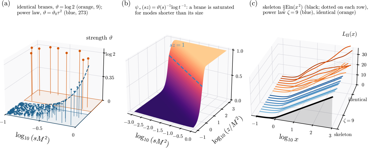
FIG. 4. Two gases with the same strength per e -fold. (a) One realization of each, for n = 4 and sizes between 0.1 M^{-2} and M^{-2} : identical branes with \vartheta_0 = \log 2 (orange) and the fine-grained power law (10) with \zeta = 2 (blue). Each brane is a stem at its size, at a random transverse position, with height equal to its strength. At the smallest sizes the fine-grained gas has 100 times more branes per e -fold, each 100 times weaker. The dashed curve is the strength \vartheta_0 \tau^2 of the power law. The value \zeta = 2 keeps the number of stems small enough to draw; condition (G) needs \zeta > 4 . (b) The exponent of the single-brane factor in units of the strength of the brane, \psi_*(sz) = \vartheta(s)^{-1} \log t^{-1} , over the plane of \log s and \log z . It switches on across the line sz = 1 (dashed), so at fixed z the exponent L_\Pi of Eq. (14) collects the strength of the branes larger than 1/z , which is the origin of the power law (19). (c) The exponent L_\Pi(x) along the Euclidean axis for eight realizations of each gas, identical branes and the power law with \zeta = 9 , drawn as a waterfall against the skeleton n\Phi(x) = \frac{n}{2} \text{Ein}(x^2) (thick, in front, and dotted on each row). The fine-grained realizations run parallel to the skeleton at large x , offset by R_\infty ; the realizations of identical branes drift away from it like random walks in \log x (Sec. II H). For \zeta = 9 the branes smaller than 0.3 M^{-2} are represented by the Gaussian limit of their compensated strength, as in Fig. 8.
