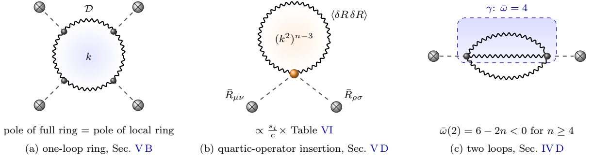
FIG. 11. Graphs behind the argument. Wavy lines are quantum gravitons (or ghosts), dashed lines end on background insertions \otimes . (a) A one-loop ring contributing to \Gamma_1[\bar{g}] . Replacing any vertex or propagator by its nonlocal remainder lowers the degree by at least 2n , so the ultraviolet pole is that of the local theory. (b) The insertion of a quartic operator with two background curvatures: the loop of (-\square)^{n-3} between two linearized curvatures has an integrand \propto k^{-4} and gives the poles of Table VI. (c) A two-loop graph. The graph as a whole is convergent for n \geq 4 ; the shaded one-loop subgraph \gamma has degree 4 and is the only possible source of a subdivergence.
