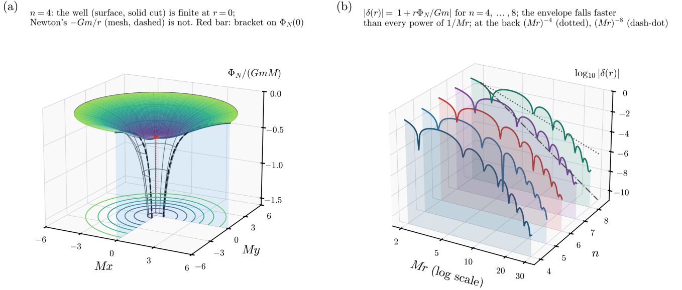
FIG. 16. Newtonian limit. (a) The potential (95) of a point mass for the skeleton with n = 4 , in units of GmM , drawn over a plane through the source with one quarter cut away. The surface and the solid profiles on the cut faces are \Phi_N ; the mesh and the dashed profiles are Newton's -Gm/r . The red bar on the axis is the bracket 0.4852 \leq |\Phi_N(0)|/GmM \leq 0.5303 of Eqs. (97) and (100); the floor carries the contours of \Phi_N . (b) The relative deviation |\delta(r)| of Eq. (103) for n = 4, \dots, 8 , on logarithmic axes. The dips are zeros of \delta , which oscillates because of the Fourier kernel. The envelope falls faster than the reference lines (Mr)^{-4} (dotted) and (Mr)^{-8} (dash-dot) drawn at the back, as Eq. (104) requires. The curves are numerical evaluations of the closed-form integrals and serve as illustration only.
