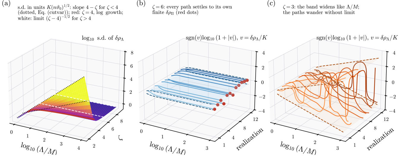
FIG. 13. Why condition (G) needs \zeta > 4 , for n = 4 , \vartheta_0 = \log 2 , \psi_* and a sharp momentum cutoff \Lambda . (a) The standard deviation of the realization's part \delta\rho_\Lambda of the zero-point energy, in units of K(n\vartheta_0)^{1/2} , as a surface over \log_{10}(\Lambda/M) and \zeta , in \log_{10} , computed from the exact integral in the footnote to Eq. (86). For \zeta > 4 it levels off at (\zeta - 4)^{-1/2} , the spread of the finite \delta\rho_\Pi of Eq. (82); for \zeta < 4 it grows with slope 4 - \zeta (dotted lines, Eq. (86)); the red curve is \zeta = 4 , where the growth is logarithmic. (b) Twelve realizations of v = \delta\rho_\Lambda/K as functions of the cutoff for \zeta = 6 , on the compressed scale \text{sgn}(v)\log_{10}(1 + |v|) , with the band \pm(\mathbb{E}\delta\rho_\Lambda^2)^{1/2}/K (translucent sheet with dashed edges). Every path settles to its own finite value, marked by a dot. (c) The same for \zeta = 3 . The band widens like \Lambda/M and the paths wander without limit, so the zero-point energy of a realization depends on where the regulator is put. In (b) and (c) the branes smaller than 0.3M^{-2} are represented, shell by shell in \log\tau , by their Gaussian limit; the larger ones are drawn individually.
