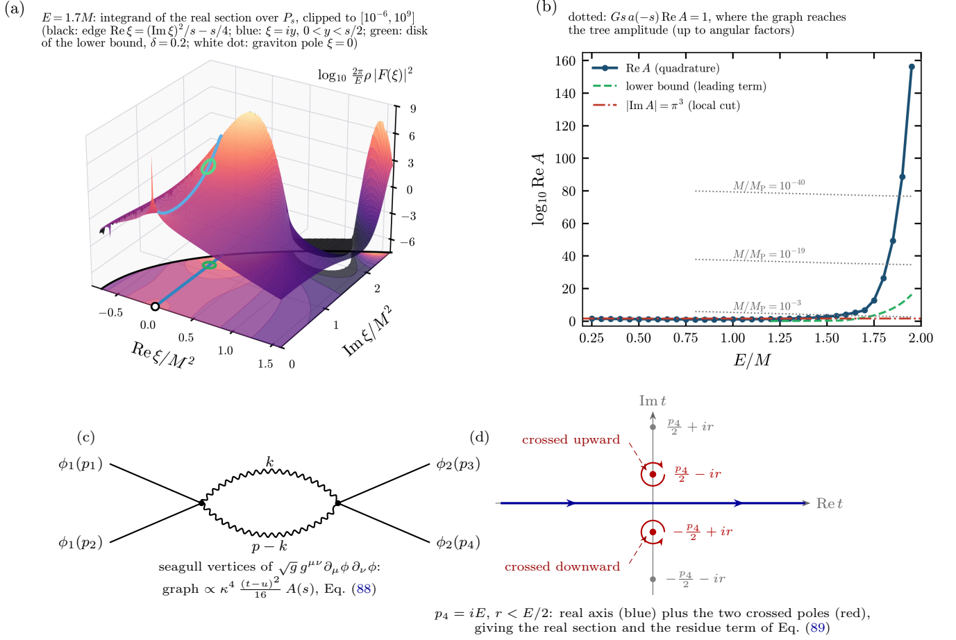
FIG. 15. The one-loop bubble in the Efimov–Pius–Sen prescription, for the skeleton with n = 4 . (a) The integrand of the real section of Eq. (89) at E = 1.7M , \log_{10}[(2\pi/E)\rho|F(\xi)|^2] , over the region P_s of the \xi plane that the loop momentum covers, upper half (the lower half is its mirror image); the surface is clipped to [10^{-6}, 10^9] , and the flat dark patch is a trough where |a| is large. Its edge, \text{Re } \xi = (\text{Im } \xi)^2/s - s/4 , is the black curve on the floor, where \rho = r = 0 . The blue segment is \xi = iy , 0 < y < s/2 , where |F|^2 = y^{-2} \exp[n \text{Ein}^-(y^2/M^4)] , and the green circle is the disk used in the bound (91) with \delta = 0.2 , both drawn on the floor and lifted onto the surface; the white dot is the graviton pole \xi = 0 , whose logarithmic singularity is removed by the subtraction. The ridges near the edge lie where \text{Re } \xi^2 is most negative and the oscillating part of \log a , of size \frac{n}{2}|E_1(\xi^2/M^4)| , has the sign that makes |a| small. (b) \log_{10} \text{Re } A against E/M from Eq. (89) (dots), the leading term of the lower bound (91) maximized over \delta (green, dashed), and \log_{10} |\text{Im } A| = \log_{10} \pi^3 (red, dash-dotted). The dotted curves are \log_{10}[(M_P/M)^2/(sa(-s))] for M/M_P = 10^{-3}, 10^{-19}, 10^{-40} , where \text{Re } A crosses one of them, the graph reaches the tree amplitude, up to angular factors. (c) The graph: each pair of scalars annihilates into two gravitons through the seagull vertex, and the loop integral is A . (d) The contour in the plane of the loop energy t at the physical point: of the four poles of the two propagators, two have crossed the real axis during the continuation, and the contour that keeps its ends fixed is the real axis plus circles around them.
