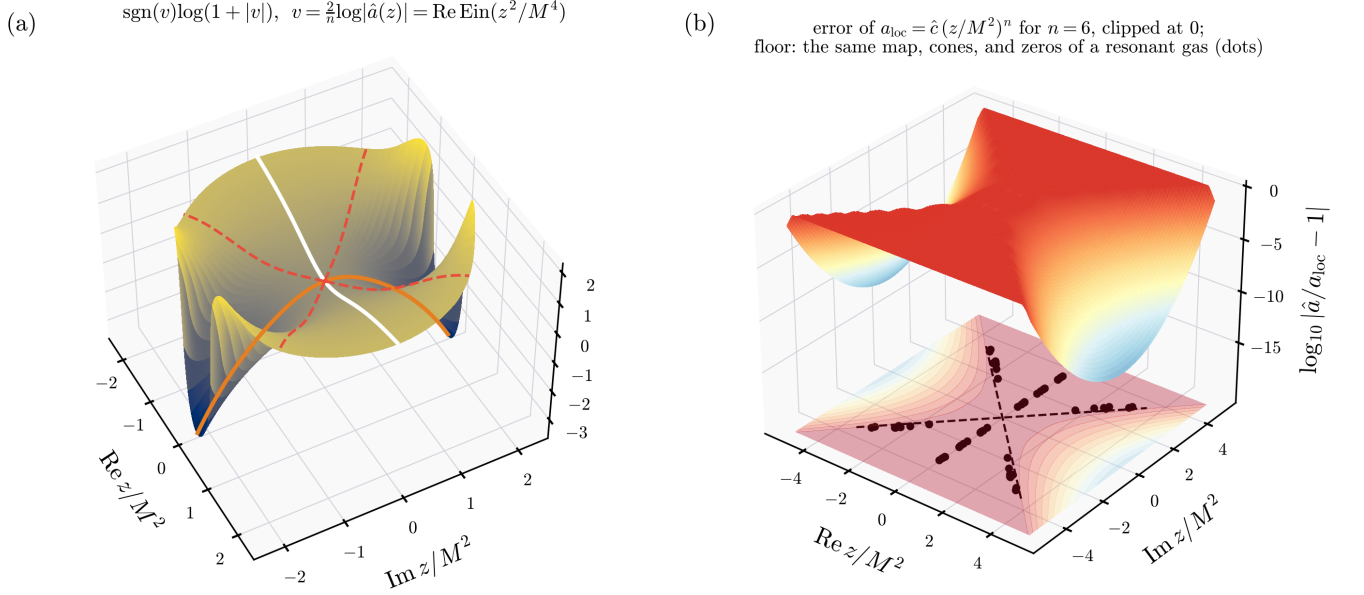
FIG. 6. The skeleton in the complex z plane. (a) v = \frac{2}{n}\log|\hat{a}| = \text{Re Ein}(z^2/M^4) over the disk |z| \leq 2.2M^2 , plotted as \text{sgn}(v)\log(1+|v|) to compress its range. Along the real axis (white) it rises like 2\log|z| ; along the imaginary axis (orange) it falls without bound; the dashed red lines are the cone boundaries \arg z = \pm\pi/4, \pm3\pi/4 , between which |\hat{a}| oscillates. (b) Accuracy of the local approximation \hat{c}(z/M^2)^n for n=6 , \log_{10}|\hat{a}/(\hat{c}z^n/M^{2n}) - 1| clipped at 0: the error is exponentially small inside the cones |\arg(\pm z)| < \pi/4 (blue), Eq. (28), and of order one outside. The floor repeats the map as a contour plot, with the cone boundaries (dashed) and, as black dots, the zeros that a frozen gas of the resonant factors 2 - e^{-s^2 z^2} of Eq. (4) would have for sizes in [0.15, 1]M^{-2} . They all lie outside the cones. A gas of branes obeying (S5) has none.
