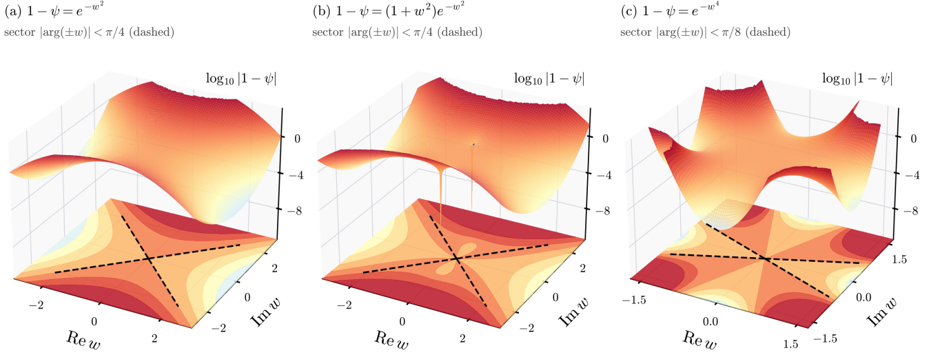
FIG. 7. The saturation sectors of condition (S4) for the three admissible exponents of Table I. Each surface is \log_{10} |1 - \psi(w)| over the complex w plane, clipped at -8 below and +3 above, with the floor showing the same quantity as a contour map. Where the surface is low the brane is saturated, \psi \simeq 1 ; the dashed lines are the sector boundaries, \arg w = \pm\pi/4 in (a) and (b) and \arg w = \pm\pi/8 in (c). The exponent 1 - e^{-w^4} of panel (c) is also saturated around the imaginary axis, which (S4) does not require.
