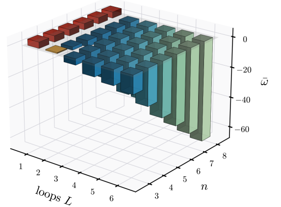
FIG. 10. Upper bound \bar{\omega}(L) on the superficial degree of an L -loop graph, Eq. (65), for n = 3, \dots, 8 and L \leq 6 , drawn as bars hanging from the plane \bar{\omega} = 0 . One-loop graphs have degree 4 for every n (red). For n=3 the two-loop bound is 0 (amber), so power counting alone leaves a possible logarithm; for n \geq 4 every graph with L \geq 2 has negative degree (blue to green), and the degree falls without bound as L grows. The bars are drawn for m_\sigma = 0 , which holds for the skeleton and whenever \sigma > 2n ; the lower block of Table V gives the bound for the weakest fine graining, m_\sigma \rightarrow n-2 , which is negative for L \geq 2 as well.
