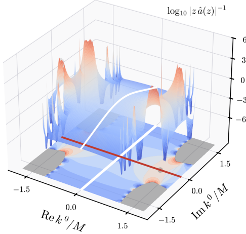
FIG. 14. Unitarity in the Efimov–Pius–Sen prescription. (a) The size of a propagator, \log_{10} |z \hat{a}(z)|^{-1} for the skeleton, over the complex plane of the loop energy k^0 at fixed spatial momentum |\mathbf{k}| = 1.2M , for n = 4 , with z = \mathbf{k}^2 - (k^0)^2 . Along the Euclidean contour (white, \text{Re } k^0 = 0 , drawn on the floor and on the surface) and along the real axis away from the poles at k^0 = \pm|\mathbf{k}| (red, black dots) the propagator is small. In the wedges around \arg k^0 = \pm\pi/4, \pm 3\pi/4 , where z is close to the imaginary axis, \log |\hat{a}| has an oscillating part of size \frac{n}{2}|E_1(z^2/M^4)| , which grows like e^{|\text{Re } z^2|/M^4} , so the propagator swings between extremely large and extremely small values; this is why the loop energies cannot be rotated to the real axis. The surface is clipped at \pm 6 and left out where that oscillating part exceeds 6 decades (gray on the floor). (b) The cutting rule of Sec. VII A: the anti-Hermitian part of an amplitude is the sum over cuts with all eighteen on-shell modes of the redefined fields. Between physical states, those in \ker Q_B , the contributions of the four BRST quartets cancel (Sec. VII B), and only the two helicities of the graviton remain.
