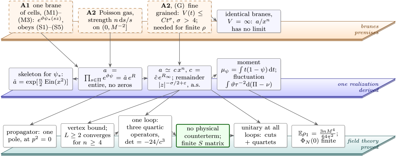
FIG. 1. Logical structure of the paper, in three layers. The top layer holds the premises about branes (dashed boxes): the response of one brane, A1, derived from a model of cells, and the gas, A2, whose fine-graining condition (G) is what lets a single realization carry the theory and is needed, up to factors slower than any power, for a finite zero-point energy; without it, for identical branes, the form factor has no power-law asymptotics (box on the right). The middle layer holds the properties of the form factor of one realization, derived for every admissible response and almost every realization (Secs. II E–II H), with the closed-form skeleton for \psi_* as one instance. The bottom layer holds the field theory, which uses the form factor only through the middle layer and is proved for n \geq 4 ; the box with the heavy frame is the main result. Arrows point from what is used to what is derived.
