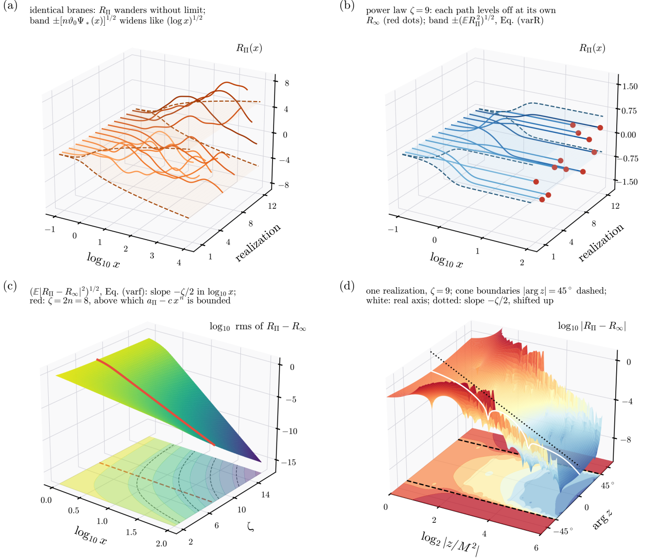
FIG. 8. Fluctuations of a realization, for n=4 , \vartheta_0 = \log 2 and \psi_* . (a) Sample paths of R_{\Pi}(x) for twelve realizations of a gas of identical branes, drawn as ribbons over \log_{10} x and the index of the realization, with the band \pm(\mathbb{E}R_{\Pi}^2)^{1/2} of Eq. (44) (translucent sheets with dashed edges). The band widens like (\log x)^{1/2} and the paths wander without limit. (b) The same for the fine-grained gas with \zeta=9 , with the band of Eq. (45). Each path levels off at its own value of R_{\infty} , marked by a dot at the right end. (c) The root-mean-square remainder (\mathbb{E}|R_{\Pi} - R_{\infty}|^2)^{1/2} , Eq. (46), as a surface over \log_{10} x and \zeta , in \log_{10} . Its slope in \log_{10} x is -\zeta/2 ; the red line marks \zeta=2n=8 , above which the remainder of a_{\Pi} after the monomial is subtracted is bounded; condition (G) asks only for \zeta > 4 . (d) \log_{10} |R_{\Pi}(z) - R_{\infty}| for one realization with \zeta=9 over the plane of \log_2 |z/M^2| and \arg z , for |\arg z| \leq 72^\circ , with the cone boundaries |\arg z| = 45^\circ (dashed) and the real axis (white). Inside the cone the surface falls along every ray with slope close to -\zeta/2 (dotted reference line, shifted up), as Eq. (38) states; the dips on the real axis are sign changes of R_{\Pi} - R_{\infty} . Outside the cone, where (S4) gives no control, the surface rises and is cut off at 10. In (b) and (d) the branes smaller than 0.3 M^{-2} in the fine-grained gas, about 3 \times 10^5 per e -fold and more, are represented by their Gaussian limit; all other branes are drawn individually.
