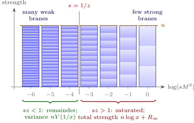
FIG. 3. How a fine-grained gas shares its strength. Each column is one e -fold of size and carries expected strength n (dashed line), Eq. (8). The number of branes in a column, drawn as slabs, grows toward small sizes while each slab gets thinner, as for the power law (10). A mode with z = p^2 saturates the branes larger than 1/z , whose total strength is n \log x plus a fluctuation that converges to R_\infty ; the branes smaller than 1/z act only through a remainder whose variance is nV(1/x) (Sec. II H).
