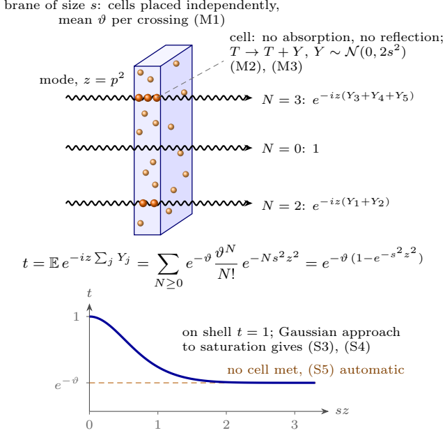
FIG. 2. A brane made of cells, Sec. II B. A mode of squared momentum z crosses a brane of size s at every point of its worldvolume. At each point it meets a Poisson number N of cells with mean \vartheta , (M1), each of which shifts its proper time by an independent Gaussian amount Y_j of variance 2s^2 , (M2) and (M3), and so multiplies it by the phase e^{-iY_j z} . Three crossing points are drawn, which meet, from bottom to top, two, zero and three cells. The coherent transmitted wave is the average of the phase, Eq. (6), which is the single-brane factor (3) with \psi = \psi_* , Eq. (7). Lower panel: t as a function of sz for \vartheta = 1.2 . It equals 1 on shell and falls to the saturation value e^{-\vartheta} , the probability that a crossing meets no cell, as the mode becomes shorter than the brane.
