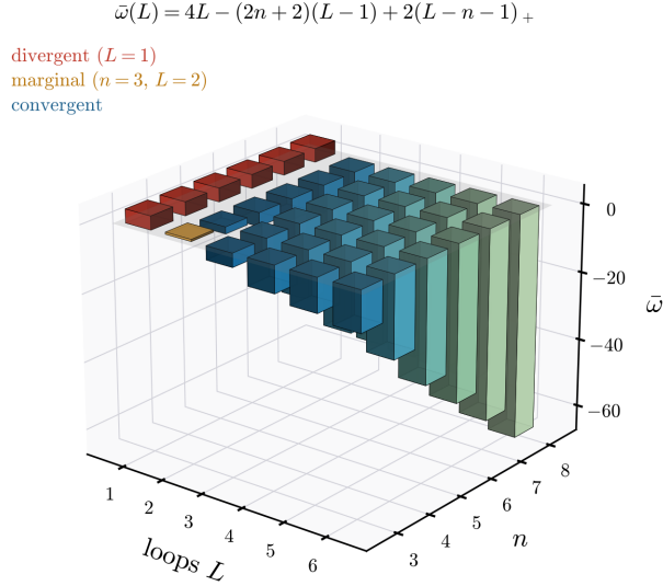
FIG. 9. Upper bound \bar{\omega}(L) on the superficial degree of an L -loop graph, Eq. (62), for n = 3, \dots, 8 and L \leq 6 , drawn as bars hanging from the plane \bar{\omega} = 0 . One-loop graphs have degree 4 for every n (red). For n=3 the two-loop bound is 0 (amber), so power counting alone leaves a possible logarithm; for n \geq 4 every graph with L \geq 2 has negative degree (blue to green), and the degree falls without bound as L grows.
