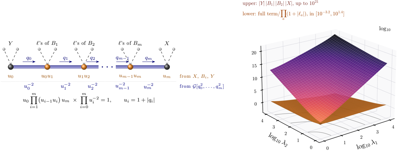
FIG. 8. The chain behind the vertex bound. (a) A function of the covariant d'Alembertian between two field monomials, X \mathcal{G}(-\square) Y , expanded as in Eq. (58). Each insertion B_i of the field-dependent part of \square attaches legs (dashed, gray balls) and changes the running momentum from q_{i-1} to q_i ; the function enters only through the divided difference \mathcal{G}[q_0^2, \dots, q_m^2] . By Eq. (61) each insertion costs one power of the running momentum on each side of it (orange), and Y and X one power each; by Eq. (59) the divided difference returns u_i^{-2} for every segment (blue). The running momenta cancel exactly, and only the legs are left. (b) A numerical check of this bookkeeping for a chain with two insertions and n = 4 , in units M = 1 . The running momenta are q_0 = \ell_Y with |q_0| = 1 , q_1 = q_0 + \ell_1 with |q_1| \simeq \lambda_1 , and q_2 = q_1 + \ell_2 with |q_2| \simeq \lambda_2 ; each insertion is given its largest size (|q_{i-1}| + |\ell_i|)^2 and X, Y the sizes u_2, u_0 . The upper surface is \log_{10} of the product of these sizes, which grows like the fifth power of the momenta, to 10^{21} ; the lower surface is \log_{10} of the full term, with the exact divided difference of the skeleton's \hat{\mathcal{G}} , divided by (1 + |\ell_1|)(1 + |\ell_2|) . It stays between 10^{-3.2} and 10^{1.4} over the four decades in \lambda_1 and \lambda_2 .
