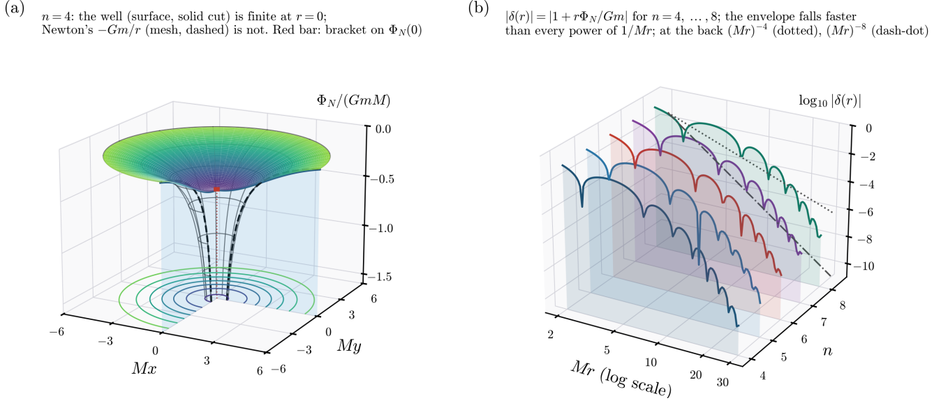
FIG. 13. Newtonian limit. (a) The potential (84) of a point mass for the skeleton with n = 4 , in units of GmM , drawn over a plane through the source with one quarter cut away. The surface and the solid profiles on the cut faces are \Phi_N ; the mesh and the dashed profiles are Newton's -Gm/r . The red bar on the axis is the bracket 0.4852 \leq |\Phi_N(0)|/GmM \leq 0.5303 of Eqs. (86) and (89); the floor carries the contours of \Phi_N . (b) The relative deviation |\delta(r)| of Eq. (92) for n = 4, \dots, 8 , on logarithmic axes. The dips are zeros of \delta , which oscillates because of the Fourier kernel. The envelope falls faster than the reference lines (Mr)^{-4} (dotted) and (Mr)^{-8} (dash-dot) drawn at the back, as Eq. (93) requires. The curves are numerical evaluations of the closed-form integrals and serve as illustration only.
