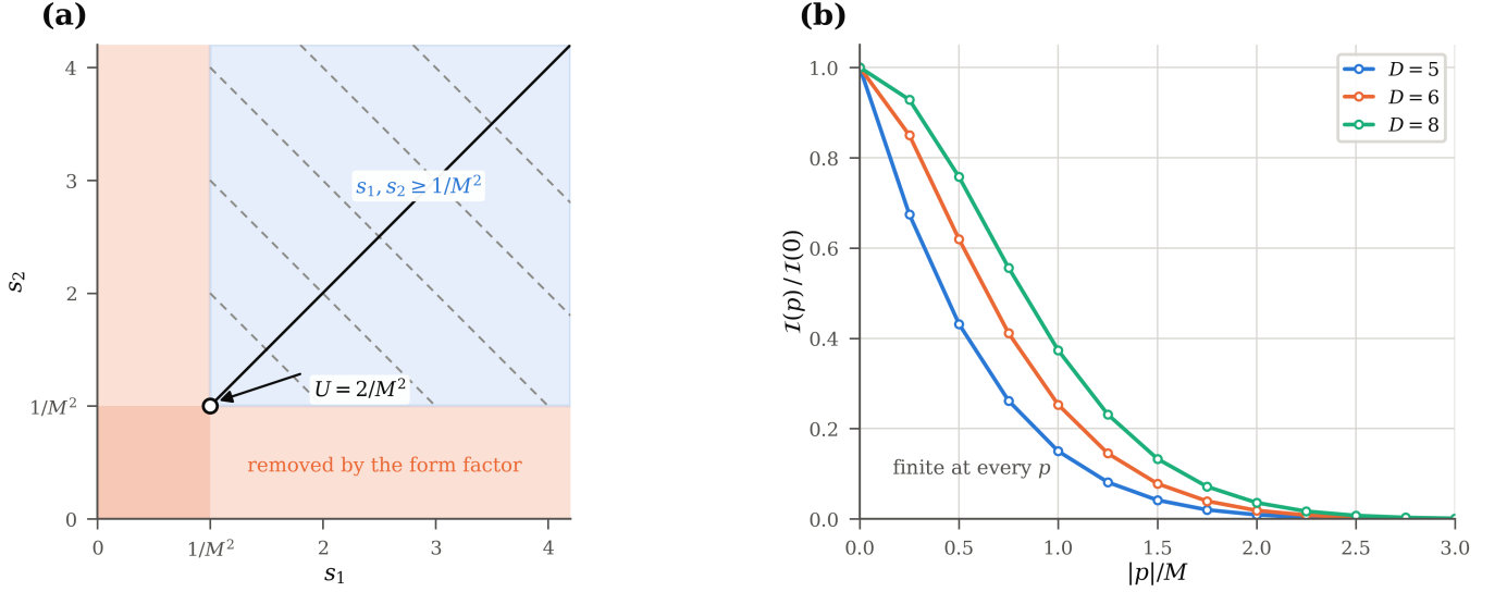
FIG. 7. The parametric domain of the one-loop bubble, (24). Dressing the propagators with e^{-k^2/M^2} removes the shaded corner near the origin, where the ultraviolet divergence of the undressed graph comes from, and leaves the quadrant s_1, s_2 \geq 1/M^2 . Along the diagonal U = s_1 + s_2 attains its minimum 2/M^2 on the domain, which is (23) for this graph. (b) The integral (24), normalized to its value at p = 0 , against the external momentum in D = 5, 6, 8 ; it is finite at every p .
