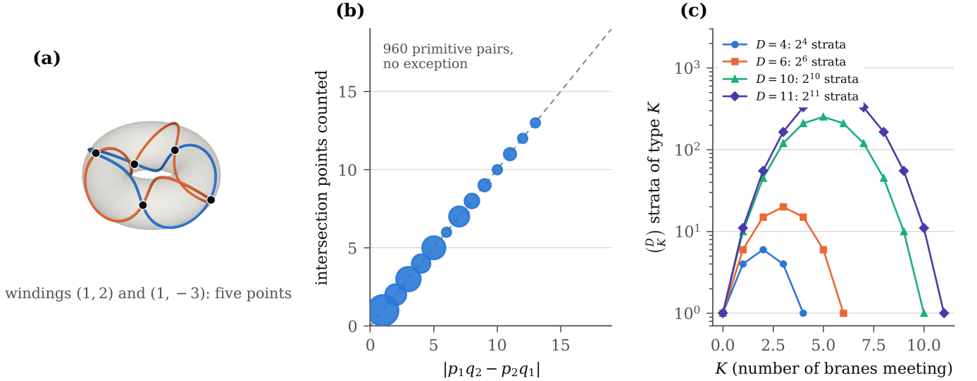
FIG. 2. (a) Two closed curves of winding numbers (1, 2) and (1, -3) on a torus meet in exactly |1 \cdot (-3) - 1 \cdot 2| = 5 points. (b) The determinant law of Proposition 2 on all 960 pairs of primitive winding vectors with entries in [-3, 3] ; marker area grows with the number of pairs at each point. (c) The census of Proposition 3 in several dimensions.
