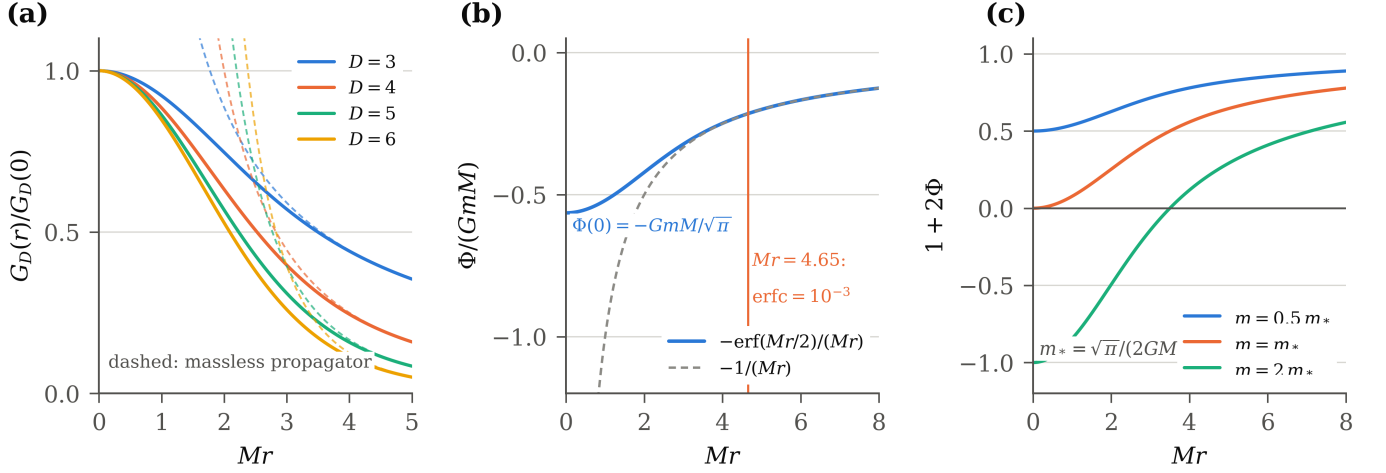
FIG. 8. The Gaussian form factor in position space. (a) The Euclidean propagator G_D of Theorem 6 in D = 3, 4, 5, 6 , normalized by its value at the origin, against the massless propagator it approaches. (b) The Newtonian potential (28) against -Gm/r ; the relative deviation \text{erfc}(Mr/2) drops below 10^{-3} at Mr = 4.65 . (c) The weak-field metric function 1 + 2\Phi for masses below, at and above the threshold m_* = \sqrt{\pi}/(2GM) of Theorem 7(d).
