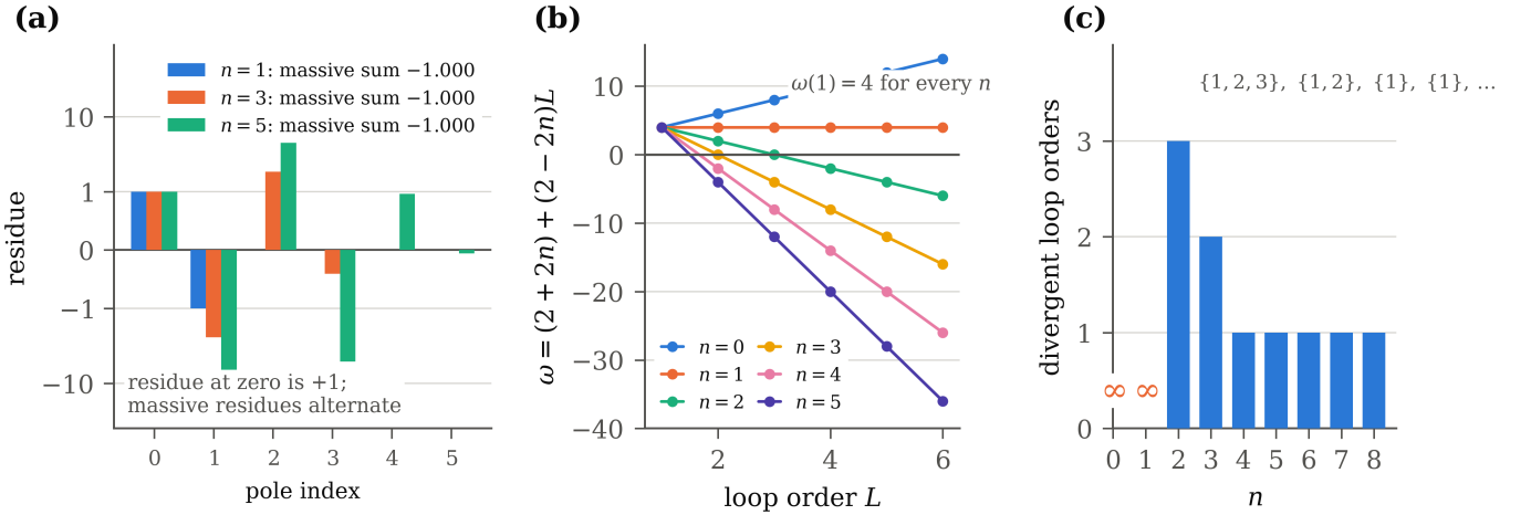
FIG. 6. (a) Residues of 1/(za(z)) at the poles of the propagator for three deterministic arrangements with real masses, ordered by mass: the residue at zero is +1, the massive residues alternate starting negative, and in every case they sum to -1 (Theorem 3). The vertical scale is linear within one unit of zero and logarithmic outside it, so that the five-mass case, whose residues run from -7.0 to +10.2, fits beside the others. (b) The superficial degree of divergence \omega(L) in four dimensions for n = 0, \dots, 5 (Theorem 4); \omega(1) = 4 for every n . (c) The number of divergent loop orders: infinite for n \leq 1 , then 3, 2, and 1 for every n \geq 4 .
