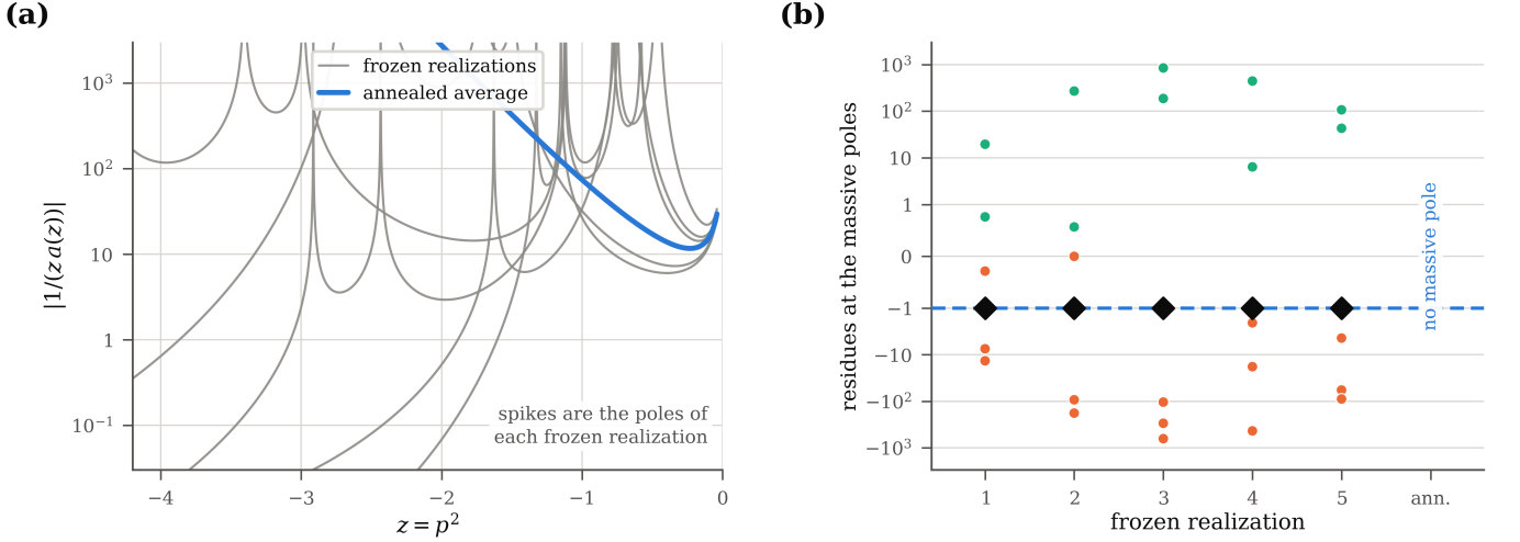
FIG. 4. Annealed against quenched, for a five-brane gas. (a) The modulus of the spin-two propagator along the negative real axis for five frozen realizations, each spiking at its own poles, against the annealed propagator built from the averaged kinetic operator. The annealed curve is finite at every z \neq 0 and simply leaves the plotted range; it has no pole. (b) The residues at the massive poles of each realization, which scatter over four decades, and their total, which is -1 in every case by Theorem 3. The annealed form factor has no massive pole and so no budget to balance.
