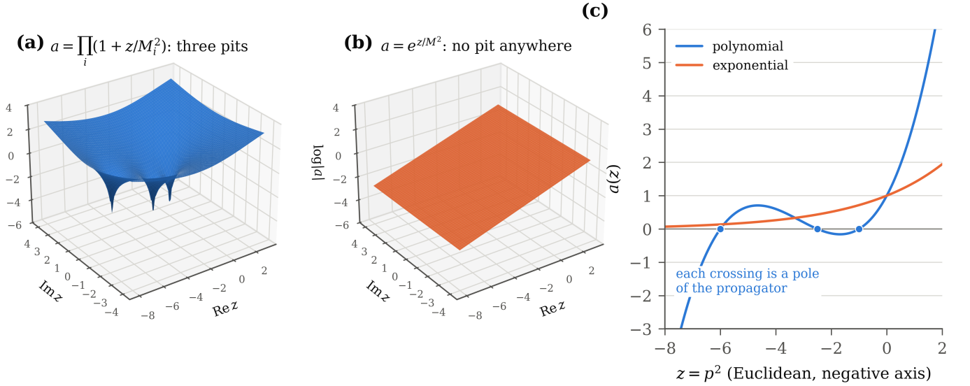
FIG. 5. (a) \log |a(z)| over the complex z = p^2 plane for the arrangement of three branes with a(z) = (1+z)(1+z/2.5)(1+z/6) : three logarithmic pits at the zeros, each a pole of the propagator. (b) The same for the Poisson average a(z) = e^{z/3} : a plane, no pit anywhere. (c) Along the negative real axis the polynomial crosses zero three times and the exponential never does; the crossings are the masses of the extra poles.
