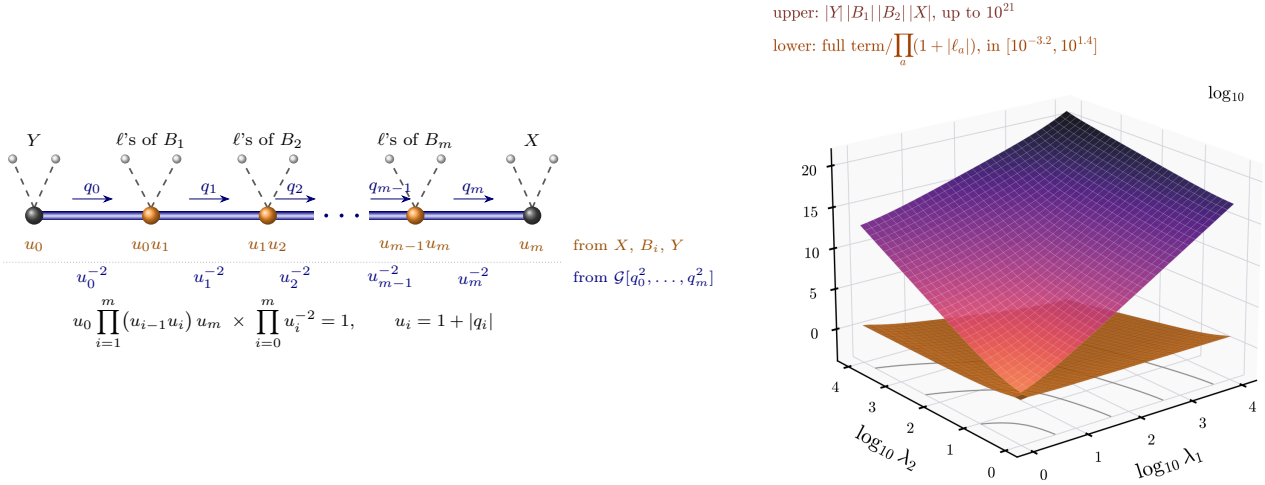
FIG. 9. The chain behind the vertex bound. (a) A function of the covariant d'Alembertian between two field monomials, X \mathcal{G}(-\square) Y , expanded as in Eq. (61). Each insertion B_i of the field-dependent part of \square attaches legs (dashed, gray balls) and changes the running momentum from q_{i-1} to q_i ; the function enters only through the divided difference \mathcal{G}[q_0^2, \dots, q_m^2] . By Eq. (64) each insertion costs one power of the running momentum on each side of it (orange), and Y and X one power each; by Eq. (62) the divided difference returns u_i^{-2} for every segment (blue). The running momenta cancel exactly, and only the legs are left. (b) A numerical check of this bookkeeping for a chain with two insertions and n = 4 , in units M = 1 . The running momenta are q_0 = \ell_Y with |q_0| = 1 , q_1 = q_0 + \ell_1 with |q_1| \simeq \lambda_1 , and q_2 = q_1 + \ell_2 with |q_2| \simeq \lambda_2 ; each insertion is given its largest size (|q_{i-1}| + |\ell_i|)^2 and X, Y the sizes u_2, u_0 . The upper surface is \log_{10} of the product of these sizes, which grows like the fifth power of the momenta, to 10^{21} ; the lower surface is \log_{10} of the full term, with the exact divided difference of the skeleton's \hat{\mathcal{G}} , divided by (1 + |\ell_1|)(1 + |\ell_2|) . It stays between 10^{-3.2} and 10^{1.4} over the four decades in \lambda_1 and \lambda_2 .
