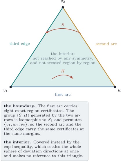
FIGURE 26. The fundamental domain of Lemma 8.1: one triangle with vertices v_1, w_1, v_2 , obtained from the full sphere of deviation directions by the two order-2 symmetries S and H . The three edges carry the certificates of Sections 10 and 12, through the identifications of Propositions 8.3 and 8.5; the interior is settled separately, in Section 13, by an argument that does not use the triangle at all.
