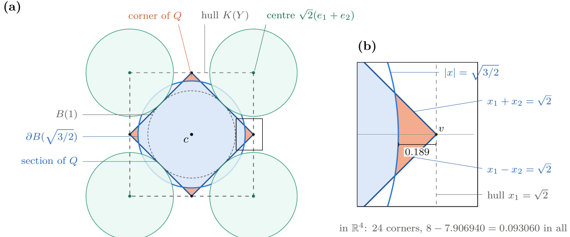
FIGURE 8. Why the pair terms stop at twenty-three centres, to scale. (a) The section of the 24-cell Q by the plane x_3 = x_4 = 0 : the square |x_1| + |x_2| \leq \sqrt{2} , whose sides touch the unit ball and whose corners are vertices of Q at radius \sqrt{2} . The ball B(\sqrt{3/2}) , inside which Lemma 2.15 makes the cell an exact function of the pairs, cuts the corners off (orange). The four centres of the plane, \sqrt{2}(\pm e_1 \pm e_2) at distance 2, with their unit balls, and their inversion hull (dashed), which meets Q only at its vertices. (b) One corner, magnified: the vertex v = \sqrt{2}e_1 , the two sides through it and the side x_1 = \sqrt{2} of the hull; the corner is \sqrt{2} - \sqrt{3/2} = 0.189 deep. In \mathbb{R}^4 the 24 corners hold 8 - 7.906940 = 0.093060 of the volume of Q .
