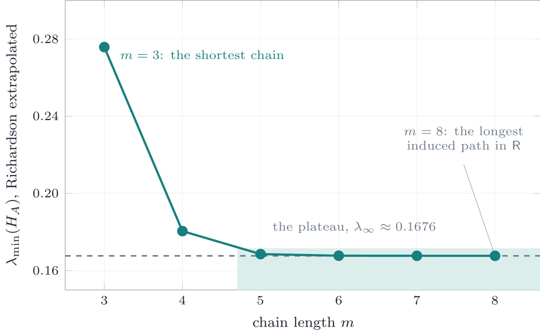
FIGURE 31. Richardson-extrapolated minimum eigenvalue of the joint Hessian H_A for chain configurations of length m = 3, \dots, 8 (Lemma 15.3; full values in Appendix G). The eigenvalue falls sharply from m = 3 to m = 5 and then plateaus near 0.1676 instead of continuing to collapse, which is the antipodal-axis mechanism described below. It stays well clear of zero for every chain length up to m = 8 , the longest induced path in the contact graph of R , so the second-order method certifies positivity on the whole chain family.
