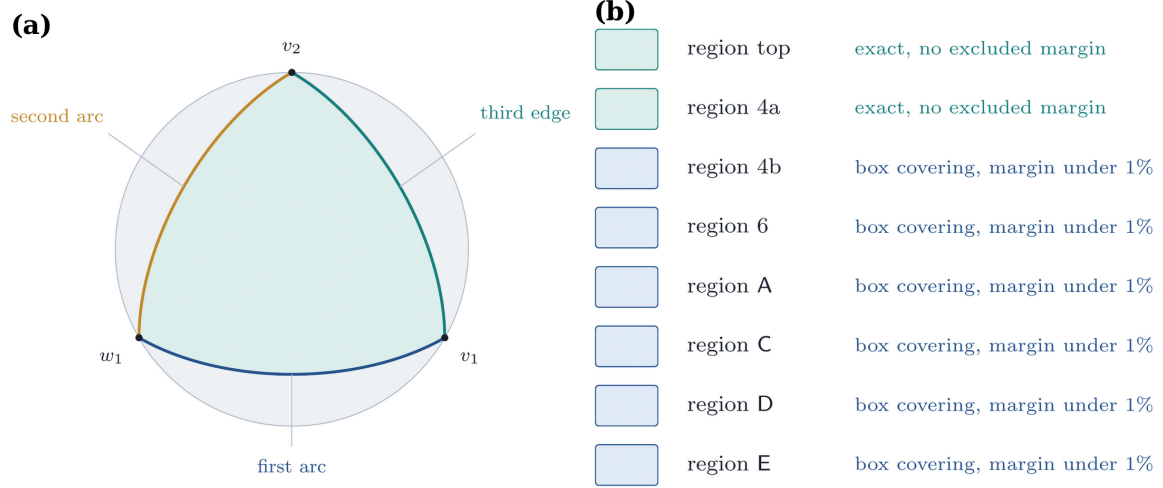
FIGURE 28. (a) The transverse sphere of deviation directions and the spherical octant left by the two symmetries of Lemma 8.1. The vertices v_1, w_1, v_2 are pairwise orthogonal, so the octant's three edges are quarter great circles, and \langle S, H \rangle \cong S_3 fixes u_0 and permutes them; a certificate on the first arc is therefore a certificate on the whole boundary of the octant. (b) The eight combinatorial regions of the first arc and the kind of certificate each carries. Two are exact with no excluded margin; the other six are certified by box covering, with the excluded margin in each case a few tenths of one percent of the region's own area. Through the identifications of Propositions 8.3 and 8.5, these eight certificates cover the whole boundary of the octant.
