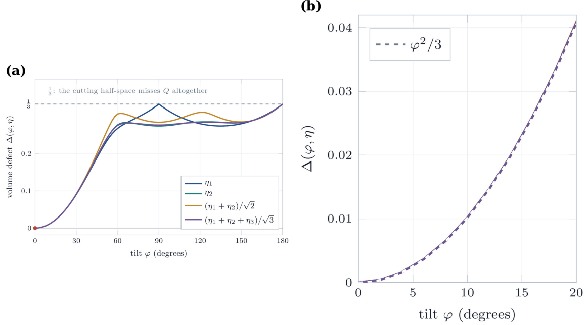
FIGURE 30. (a) The volume defect \Delta(\varphi, \eta) over the whole range of tilts, for four deviation directions spanning the transverse sphere: two of the orthonormal frame directions and two diagonal combinations of them. The defect is nonnegative throughout and vanishes only at \varphi = 0 , as Theorem 13.7 asserts, and it returns to the value \frac{1}{3} at \varphi = \pi , where the cutting half-space misses Q entirely and the cell is exactly Q itself. The intermediate maxima and minima are where the breakpoint structure of Section 9 shows itself. The curves are computed from directly enumerated cell volumes, by a route independent of the proof. (b) The same four curves at small tilt, against the second-order rate \varphi^2/3 of Proposition 13.9. The four are indistinguishable there, and from each other, at plotting accuracy.
