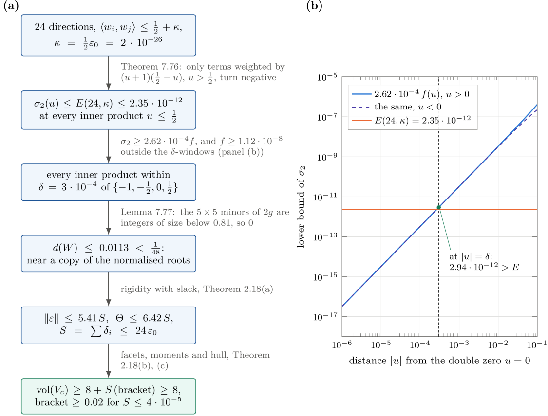
FIGURE 25. Where \varepsilon_0 = 4 \cdot 10^{-26} comes from. (a) The chain of explicit bounds that replaces the compactness argument of Theorem 2.18, with the number each step produces ( explicit_eps0.py ). Twenty-four directions with inner products at most \frac{1}{2} + \kappa make every sign-changing sum-of-squares term of the certificate at least -E in total (Theorem 7.76); so \sigma_2 \leq E at each inner product up to \frac{1}{2} , which pins it near a zero of \sigma_2 ; Lemma 7.77 turns that into a distance from the root system; the rigidity of Theorem 7.51, with slack, bounds the displacement by the sum S of the distances beyond contact; and the facet, moment and hull estimates close the argument. (b) To scale: the lower bound 2.62 \cdot 10^{-4} f(u) of \sigma_2 near its double zero u = 0 , for u > 0 and u < 0 , against the level E(24, \kappa) = 2.35 \cdot 10^{-12} . The two cross at |u| \approx 2.7 \cdot 10^{-4} , inside the window |u| \leq \delta = 3 \cdot 10^{-4} , where the bound is already 2.94 \cdot 10^{-12} . The other double zero, -\frac{1}{2} , gives the same picture; at the simple zeros -1 and \frac{1}{2} the bound is linear and the window is far wider than needed.
