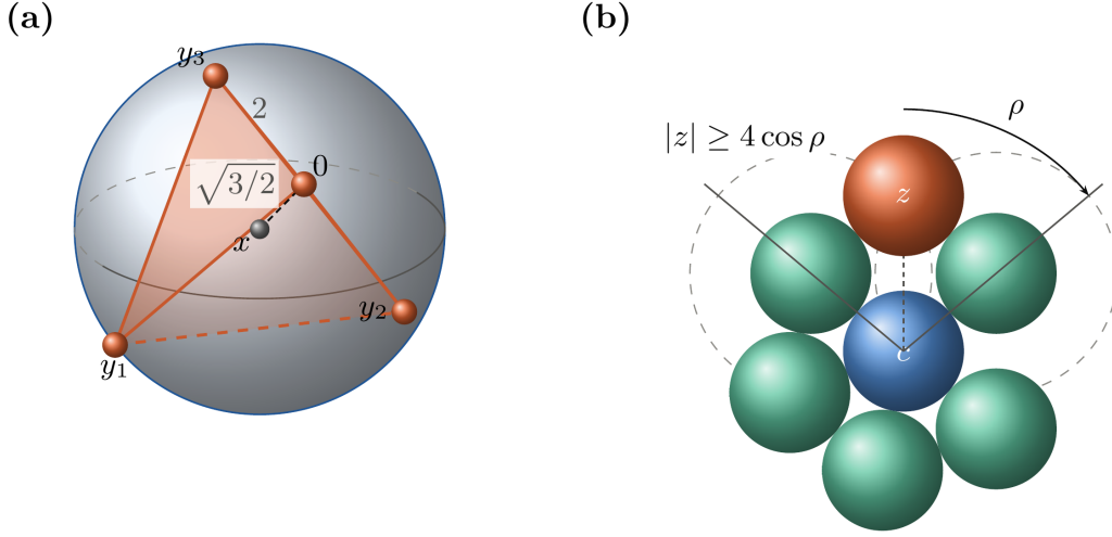
FIGURE 4. Two elementary facts behind Section 2.8, to scale. (a) Lemma 2.15: four points pairwise at least 2 apart do not fit in a ball of radius less than \sqrt{3/2} , and the regular tetrahedron of edge 2 in the ball of radius \sqrt{3/2} is the extreme case; so no point x of the open ball B(\sqrt{3/2}) about the centre 0 is closer to three other centres than to 0. (b) Lemma 2.12 in a plane section: the balls of the contacts (green) leave a hole of angular radius \rho , here 50^\circ , and a further centre z can enter it only at a distance |z| \geq 4 \cos \rho from c , where it meets the circles of radius 2 (dashed) about the two contacts at the rim.
