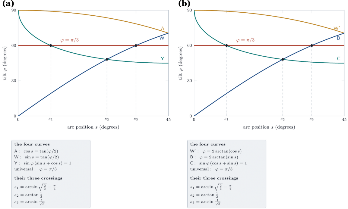
FIGURE 23. (a) The four breakpoint curves of the first arc, drawn to scale from the closed forms of Theorem 9.1: the universal curve \varphi = \pi/3 and the curves A, W, Y. They meet in exactly three points, at the abscissae s_1 , s_2 , s_3 listed at the right, and the eight combinatorial regions of Section 10.2 are the cells of the resulting arrangement. The curves A and W meet only at s = \pi/4 , where the reflection symmetry of the arc identifies them. (b) The four breakpoint curves of the second arc, drawn to scale from the closed forms of Theorem 11.1. Comparing with Figure 23(a) shows what Proposition 8.5 later proves: the three equations here are exactly those of A, W and Y on the first arc, and the arrangement, crossings included, is the same one, even though the curves come from different vertices of \mathcal{V} . The band immediately below region top splits into three sub-parts at the crossings s_1 , s_2 , s_3 .
