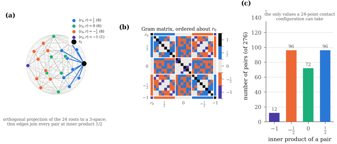
FIGURE 10. What Theorem 7.30 forces. (a) The twenty-four normalised roots of D_4 , projected orthogonally to a generic 3-space so that no two coincide, with every pair at inner product \frac{1}{2} joined; one root r_0 is singled out and the others are coloured by their inner product with it, eight at \frac{1}{2} , six at 0, eight at -\frac{1}{2} and the antipode at -1 . (b) The Gram matrix of the twenty-four directions, rows and columns ordered by these classes; it takes no value outside \{1, \frac{1}{2}, 0, -\frac{1}{2}, -1\} . (c) The 276 pairs by inner product: 96, 72, 96 and 12. The theorem says that every contact configuration of size 24 has a Gram matrix with the values of (b), and Lemma 7.26 that it then is (a) up to an orthogonal map.
