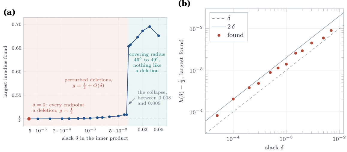
FIGURE 16. (a) The continuation of Table 3: the largest inradius found, against \delta on a logarithmic axis. The plateau near \frac{2}{3} runs down to \delta = 0.009 and is carried by configurations far from any deletion; from \delta = 0.008 down it collapses to \frac{1}{2} + O(\delta) . (b) The same table below the collapse: h(\delta) - \frac{1}{2} against \delta on logarithmic axes, with the lines \delta and 2\delta for comparison. The approach to \frac{1}{2} is linear in \delta , which is what a perturbed deletion gives.
