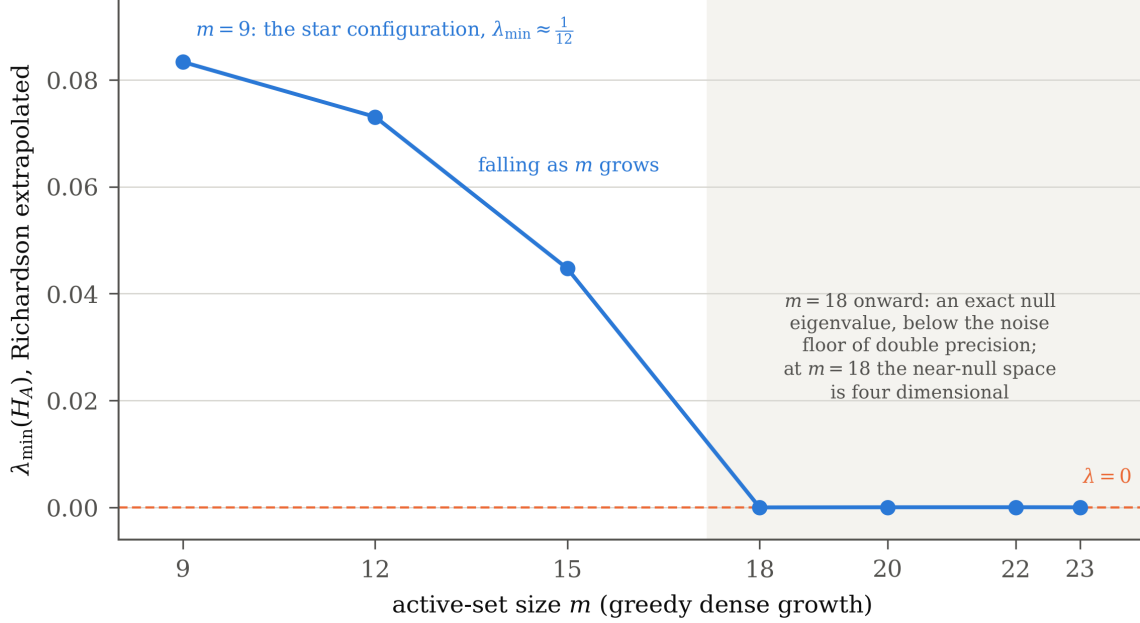
FIGURE 28. Richardson-extrapolated minimum eigenvalue of H_A under greedy dense growth, m = 9 through m = 23 (full values in Appendix G). The contrast with Figure 27 is the point: here there is no plateau above zero. From m = 18 onward, shaded, the extrapolated value is smaller than double-precision finite differences can resolve, which is the regime Section 17 takes up with arbitrary-precision arithmetic instead, and where the vanishing turns out to be exact.
