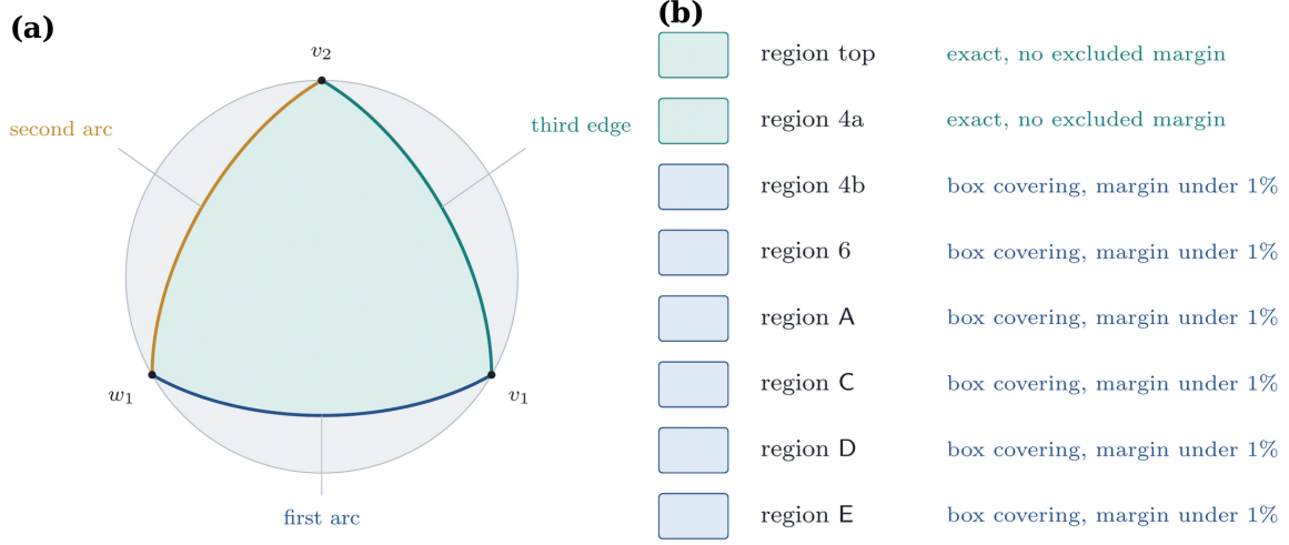
FIGURE 24. (a) The transverse sphere of deviation directions and the spherical octant left by the two symmetries of Lemma 8.1. The vertices v_1, w_1, v_2 are pairwise orthogonal, so the octant's three edges are quarter great circles, and \langle S, H \rangle \cong S_3 fixes u_0 and permutes them; a certificate on the first arc is therefore a certificate on the whole boundary of the octant. (b) The eight combinatorial regions of the first arc and the kind of certificate each carries. Two are exact with no excluded margin; the other six are certified by box covering, with the excluded margin in each case a few tenths of one percent of the region's own area. Through the identifications of Propositions 8.3 and 8.5, these eight certificates cover the whole boundary of the octant.
