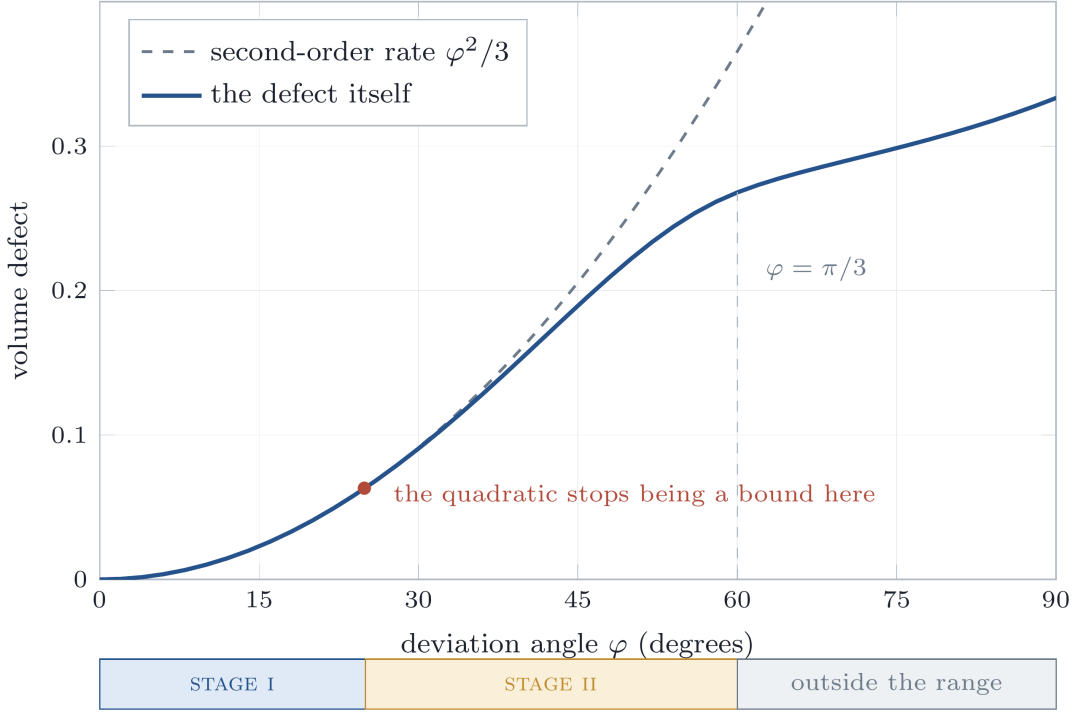
FIGURE 6. The computed volume defect for a root-aligned deviation, against the second-order rate \varphi^2/3 that STAGE I supplies. The two agree to plotting accuracy up to about 25^\circ and part company after it, the quadratic overtaking the defect and ceasing to be a lower bound; this is why the second-order argument alone does not reach the end of the range and STAGE II is needed. The strip beneath marks which argument covers which part of the range. The packing-valid range for a single deviation ends at \varphi = \pi/3 , where a second root becomes the nearest one.
