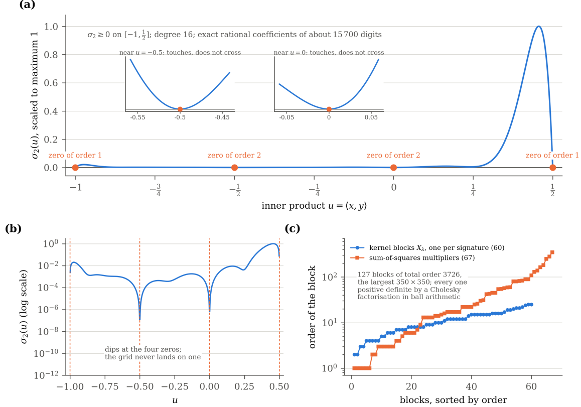
FIGURE 9. The certificate, as Proposition 7.29 reads it. (a) The two-point polynomial \sigma_2 on [-1, \frac{1}{2}] , evaluated exactly from the deposited rational coefficients and scaled by its maximum: it is nonnegative, it vanishes to first order at -1 and \frac{1}{2} and to second order at -\frac{1}{2} and 0 , and nowhere else; the insets show the two double zeros, where the curve touches the axis without crossing it. (b) The same on a logarithmic scale. (c) The orders of the 127 positive definite blocks, the sixty kernel blocks X_\lambda and the sixty-seven sum-of-squares multipliers; the largest is 350 \times 350 .
