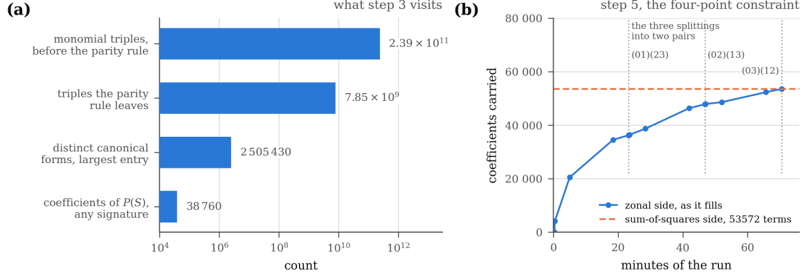
FIGURE 11. The two steps of the verification of the certificate that its authors' own code [LLM24d] leaves out, as they were carried out here. (a) Why step 3 fits in a few hundred megabytes. The integral over O(4) is taken one monomial triple at a time; the parity rule on the exponent matrix discards all but about a thirtieth of the triples, the invariance under permuting rows and columns collapses those onto at most 2 505 430 canonical forms in the largest of the 490 entries, and the answer never has more than \binom{20}{6} = 38\,760 coefficients whatever the signature. The first two counts are the counters in the kernel; the third is the size of its memo table. (b) Step 5 for the four-point constraint, the only one large enough to be difficult. The curve is the zonal side of the constraint filling up, one signature at a time, through the three ways of splitting four points into two pairs; it stops at 53 572 coefficients, which is where the sum-of-squares side stops as well. The two sides sit on the same monomials and each coefficient of one is the exact negative of the other, so the difference is zero at every one of the 53 572 places.
