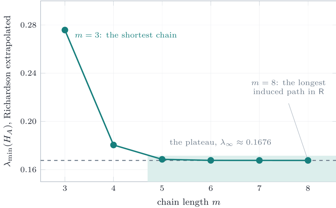
FIGURE 27. Richardson-extrapolated minimum eigenvalue of the joint Hessian H_A for chain configurations of length m = 3, \dots, 8 (Lemma 15.3; full values in Appendix G). The eigenvalue falls sharply from m = 3 to m = 5 and then plateaus near 0.1676 instead of continuing to collapse, which is the antipodal-axis mechanism described below. It stays well clear of zero for every chain length up to m = 8 , the longest induced path in the contact graph of R , so the second-order method certifies positivity on the whole chain family.
