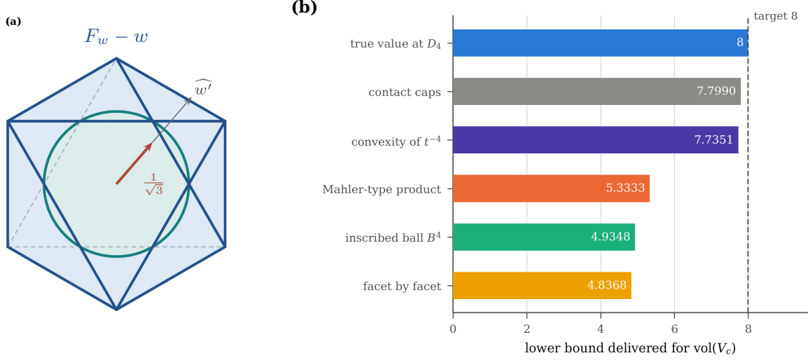
FIGURE 8. (a) A single facet of the reference cell, drawn inside the 3-space orthogonal to its own contact direction. At the root configuration the eight tight neighbours cut out the regular octahedron (Lemma 7.11); the pairwise contact condition on its own guarantees no more than the inscribed ball, and the gap between the two is what the boundary form (7.6) has to absorb. (b) The bounds the boundary form and the other global routes actually deliver, all of them evaluated at the D_4 configuration where the conjecture is tight (Remarks 7.12 and 7.13).
