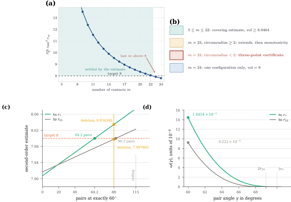
FIGURE 12. (a) The covering bound (7.12) at every admissible contact count m , against the target 8. It clears the target for all m \leq 22 and falls below at m = 23 . (b) How each part of the range of contact counts is settled: the estimate below 22 (Corollary 7.17), extension followed by monotonicity at 23 when the circumradius reaches 2 (Proposition 7.38), and the classification at 24 (Theorem 7.25). The third row is settled by the pair inequality of Theorem 7.69 and its certificate, Theorem 7.73. (c) The pairwise estimate at m = 23 , for the two integration limits r_{23} and r_* : the right-hand side of (7.17) as a function of the number of pairs at exactly 60^\circ , with the bracket alone at 0 pairs, the deletion configuration at 88 on both lines, the crossings of the target at 90.3 and at 64.2 pairs, and the elementary ceiling of Proposition 7.41 at 115. (d) The per-pair weight \omega(\gamma) for each integration limit: 0.000922\dots and 0.001445\dots at 60^\circ , vanishing at 2r_{23} = 69.2213\dots^\circ and at 2r_* = 70.5288\dots^\circ .
