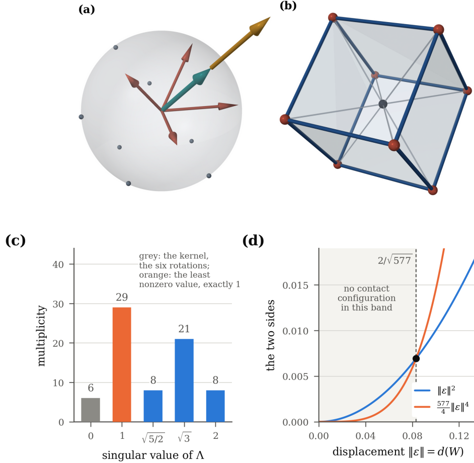
FIGURE 13. (a) The neighbour sum in dimension three, where it fits in one picture: a contact direction of the face-centred cubic lattice (teal), the four contact directions at 60^\circ from it (clay), and their sum (ochre), which is twice the direction itself. (b) The same identity in dimension four, drawn where it lives. The eight roots at inner product 1 from a root \alpha fill the hyperplane \langle \alpha, x \rangle = 1 , a copy of \mathbb{R}^3 , as the vertices of a cube centred at \alpha/2 (dark); eight times that centre is 4\alpha . (c) The singular values of the rigidity operator \Lambda on the 72-dimensional tangent space, with multiplicities (Lemma 7.50). The kernel is the six infinitesimal rotations, and the smallest nonzero value is the constant that turns the first-order argument into a radius. (d) The two sides of the inequality that closes Theorem 7.51. Feasibility forces \|\varepsilon\|^2 \leq \frac{577}{4} \|\varepsilon\|^4 , so the displacement is either zero or at least 2/\sqrt{577} : the shaded band holds no contact configuration of 24 directions.
