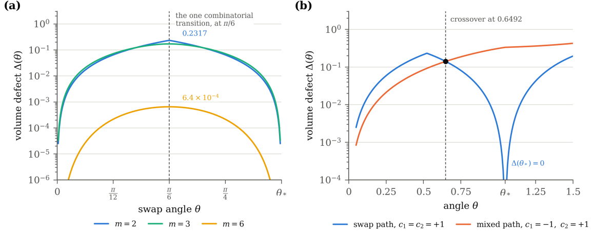
FIGURE 29. (a) The volume defect along the three swap paths of this section, over the whole packing-valid range (0, \theta_*) , \theta_* = \pi/3 . The vertical scale is logarithmic because the three sit nearly three orders of magnitude apart: the two-direction and three-direction paths peak at 0.2317 and 0.1692 at the midpoint, the six-direction path at 6.4 \times 10^{-4} . All three are positive throughout and vanish at both ends, which is what Theorems 20.2 to 20.4 assert exactly. The dashed line is the single combinatorial transition, at \theta = \pi/6 , visible as the corner in the m = 2 curve; the m = 6 path has none, and its curve is smooth there. The values plotted are enumerated cell volumes, computed by swap_defect_curves.py through a route independent of the closed forms, and for m = 6 they agree with the closed form of Section 20.6 to 9 \times 10^{-9} . (b) The swap path against the mixed path, the two differing only in the sign c_1 . The more adversarial of the two is the lower one, and which that is changes at \theta = 0.6492 : below the crossover the mixed path is lower, at \theta = 0.05 by 0.000834 against 0.002474, and above it the swap path is, through \theta_* and beyond. Second-order theory cannot tell the two apart, since the Hessian entry that distinguishes them enters only through its magnitude. The zero of the swap curve at \theta_* is the swap point itself, where the configuration is again a root system.
