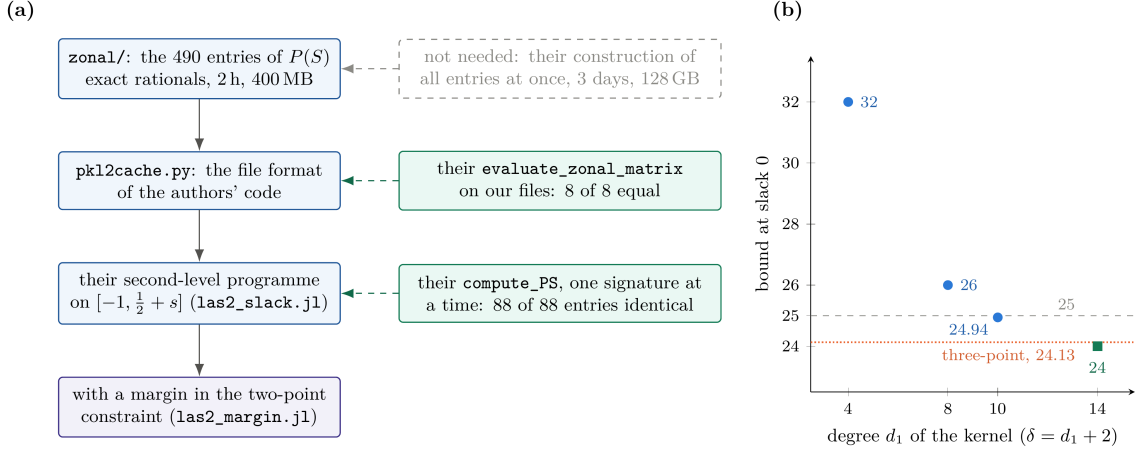
FIGURE 34. The second level of the hierarchy at slack 0. (a) The zonal matrices of Section 4.5.3 replace the construction of [LLM24] in their second-level programme, and the two checks against their entries. (b) The bound of the programme at slack 0 against the degree d_1 of the kernel, with \delta = d_1 + 2 : 32 at (4, 6), 26 at (8, 10), 24.942 at (10, 12), and the certificate's 24 at (14, 16); beside the three-point bound at degree 10, 24.13, and the level 25 that a bound on the number of points has to beat.
