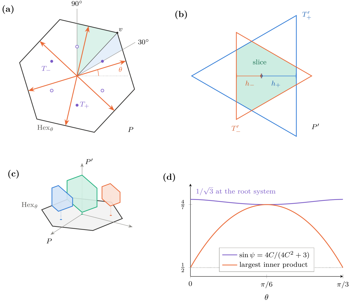
FIGURE 36. The curve of Proposition 6.19, drawn at \theta = 17^\circ . (a) The plane P : the six roots of the hexagon turned by \theta from the reference direction (dotted), the hexagon \text{Hex}_\theta of inradius 1 that they cut out, the directions in P of the other eighteen roots, at radius \sigma (filled: the triangle T_+ at 30^\circ, 150^\circ, 270^\circ ; open: T_- ), and the sector between the rays at 30^\circ and 90^\circ , split at the vertex v into the two triangles (blue and green) over which J_1 and J_2 are computed. (b) The slice over a point of \text{Hex}_\theta : the intersection of two opposite triangles of inradii h_+ and h_- in P' , a hexagon while h_+ \leq 2h_- and h_- \leq 2h_+ . (c) The cell as the union of its slices over \text{Hex}_\theta , with the exact slices over three points; the two-dimensional slices are drawn in one plane transverse to P . (d) Along the curve: the tilt \sin \psi of the eighteen roots and the largest inner product, which exceeds \frac{1}{2} for 0 < \theta < \pi/3 and reaches \frac{4}{7} at \theta = \pi/6 .
