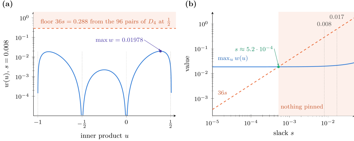
FIGURE 32. The margin of the second level against the root system (Proposition 6.10). (a) The weight w at s = 0.008 on a logarithmic scale, with its zeros at -1 , -\frac{1}{2} and 0 and at \frac{1}{2} + s ; the largest value is 0.01978 , near u = 0.3855 , and the 96 pairs of the root system at \frac{1}{2} force (N - 24)/\mu \geq 36s = 0.288 (shaded). No inner product is excluded. (b) The largest value of w and the floor 36s as functions of the slack. They cross near s = 5.2 \cdot 10^{-4} ; to the right of the crossing, which contains the slacks 0.008 of Theorem 4.73 and 0.017 of Proposition 6.21, the margin excludes nothing.
