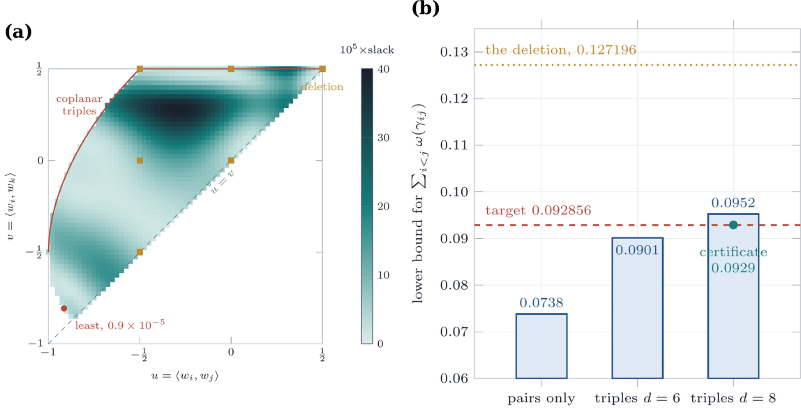
FIGURE 19. (a) The certificate of Theorem 4.67: the slack of the condition (4.49), the amount by which its left-hand side exceeds 0, on the slice of the admissible domain in which one pair of the triple is at 60^\circ . It is positive throughout, least near a coplanar triple with one nearly antipodal pair, and largest, about 4 \times 10^{-4} , in the interior. The six squares are the triples that occur in a deletion of a root. (b) The values of the relaxations against the target 8 - A_* : the pair angles alone (Remark 4.45), the three-point relaxation at degrees 6 and 8, and the certificate, at which the bound is fixed at 0.0929 and the least slack is maximised.
