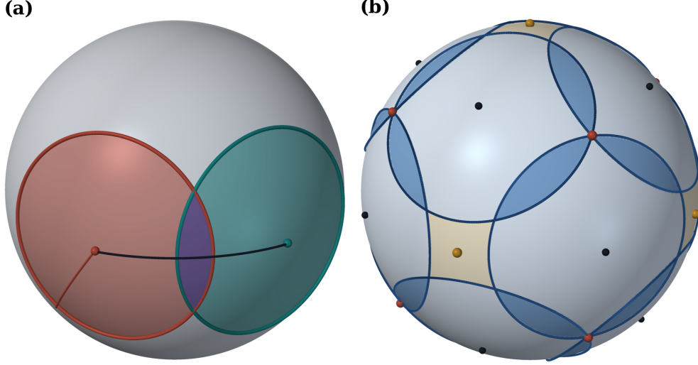
FIGURE 17. (a) Two contact directions at angle \gamma = 60^\circ and their caps of radius r = r_* . The lens in which the caps overlap (violet) has measure \Lambda(r, \gamma) , and \omega(\gamma) integrates it against d(\sec^4 r) ; the dark arc is \gamma and the clay arc is r . (b) The caps of radius r_* about the twelve contact directions of the same lattice, the sphere shaded by how many caps cover it: one (pale blue), two in the lenses, three at the eight triangle circumcentres (clay), and none in the six square holes (ochre).
