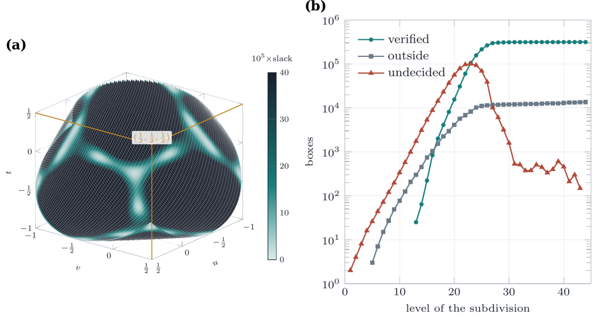
FIGURE 20. (a) The domain of the certificate condition: the admissible region of Lemma 4.66 in three dimensions, where the triples (u, v, t) of pairwise inner products of three contact directions fill the part of the cube [-1, \frac{1}{2}]^3 enclosed by the surface of coplanar triples. The surface is coloured by the slack of (4.49), which is least along the curves where two of the three directions are nearly antipodal. (b) The branch and bound of the proof of Theorem 4.67, level by level: the boxes live, the boxes discarded on the enclosure, and the width reached.
