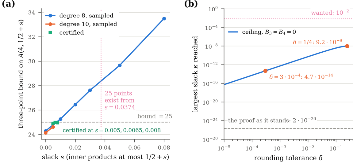
FIGURE 22. The two halves of Theorem 4.25 at positive slack. (a) The three-point bound on the number of points of S^3 with inner products at most \frac{1}{2} + s , from sampled programmes of degree 8 and 10 (each sampled value is slightly optimistic), with the three certified values: degree 8 at s = 0.005 and 0.0065 , degree 10 at s = 0.008 , the one Theorem 4.73 uses. It crosses 25 near s = 0.009 ; a 25-point code exists from s = 0.0374 on. (b) How far the proof of Theorem 4.70 could be pushed if the triple and quadruple terms cost nothing ( B_3 = B_4 = 0 ): the largest slack \kappa it reaches, against the tolerance \delta that a rounding lemma would allow (Remark 4.72). The curve grows like \delta^2 and stops below 10^{-8} ; the proof as it stands gives 2 \cdot 10^{-26} .
