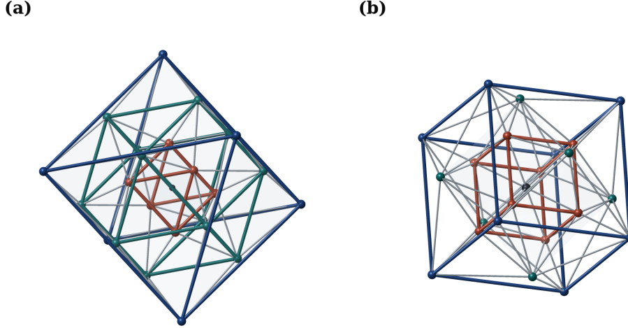
FIGURE 15. (a) The 24 contact directions of D_4 seen from a deep hole (dark), radius proportional to angle: an octahedron at 45^\circ (clay), a cuboctahedron at 90^\circ (teal), an octahedron at 135^\circ (blue), and the 96 pairs at 60^\circ as edges, grey between shells. (b) The dual 24-cell seen from the same hole and on the same scale. The hole is now itself a direction (dark), and the others form a cube at 60^\circ (clay), an octahedron at 90^\circ (teal) and a cube at 120^\circ (blue); the edges are the 88 pairs at 60^\circ that avoid the antipode of the hole, which lies at 180^\circ and is not drawn. The two panels together carry the 48 directions of the binary octahedral group.
