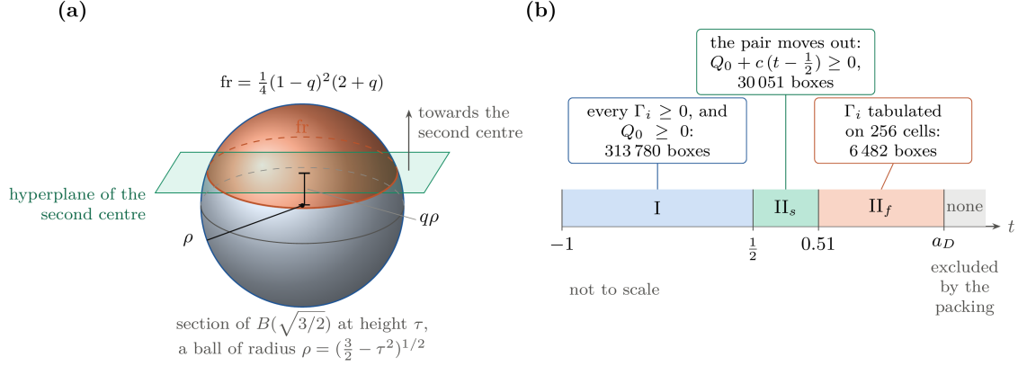
FIGURE 29. The proof of Theorem 6.8. (a) The share \text{fr} : the section of B(\sqrt{3/2}) by the hyperplane of one centre is a ball of dimension three, and the hyperplane of a second centre cuts from it a cap; moving the first hyperplane out removes from the pair term exactly this cap, and from the cap term of the centre the whole section. (b) The three ranges of the largest inner product t of three directions, with what settles each; beyond a_D the packing leaves no room.
