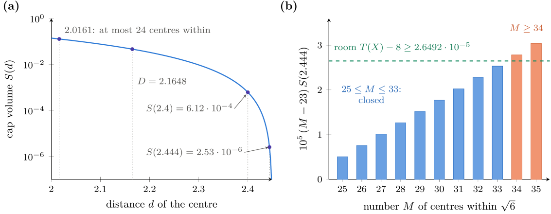
FIGURE 39. The constants of Lemma 6.30. (a) The volume S(d) of the cap of a centre at distance d , which vanishes at \sqrt{6} , with the radii of the argument: 2.0161 of Theorem 4.73, D of Step 1 of Theorem 6.8, 2.4 of Theorem 6.31 and 2.444. (b) The caps of the M - 23 centres beyond 2.444 against the room that Theorem 6.8 leaves above 8 for the twenty-three closest: they fit under it for 25 \leq M \leq 33 and not from M = 34 .
