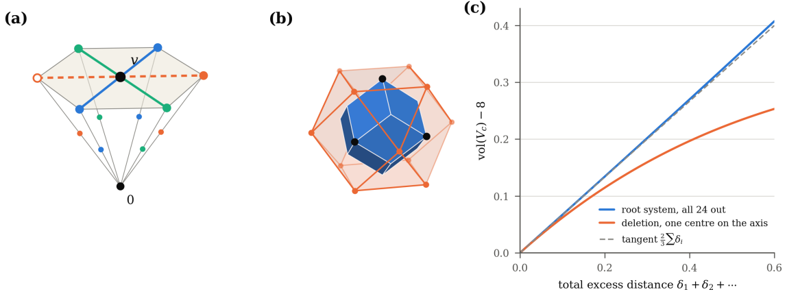
FIGURE 28. (a) Corollary 6.5: a vertex v of the 24-cell and its three orthogonal pairs of normalised roots, in the linear projection of \mathbb{R}^4 that keeps the vertex direction vertical and sends the other three coordinate directions to horizontal unit vectors at 120^\circ . The six roots at v lie on a hexagon, the points 2u on a larger one, and v is the midpoint of the chord from 2u to 2u' of each pair, so it lies in the inversion hull of any contact set that keeps one pair. One root is missing (hollow), its chord is lost (dashed), and v keeps the other two. (b) Proposition 6.4 in three dimensions: the Voronoi cell of the twelve contacts of the face-centred cubic packing, a rhombic dodecahedron (blue), lies in the convex hull of the points 2u (orange) and touches its boundary only at its six four-valent vertices (black), as the 24-cell touches the hull of the points 2u at its 24 vertices; every other centre leaves that hull whole. (c) Theorem 6.9 to first order: the exact volume excess of the root system pushed out uniformly, 8(1 + \delta/2)^4 - 8 with \sum \delta_i = 24\delta , and of the deletion with one centre at 2 + \delta on the deleted axis, \frac{1}{3} - \frac{1}{3}(1 - \frac{\delta}{2})^4 , against the total excess distance; both are tangent at the root system to \frac{2}{3} \sum \delta_i .
