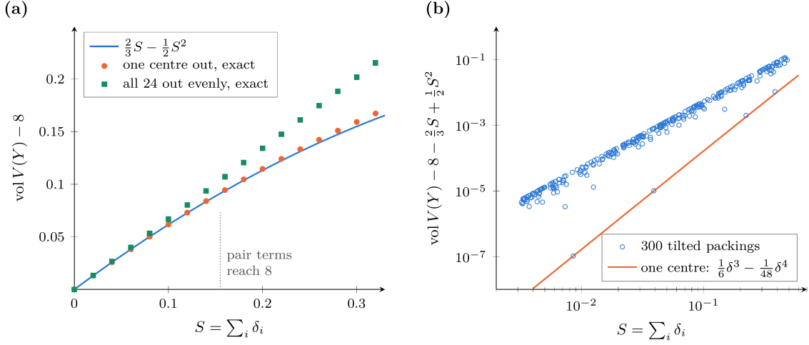
FIGURE 35. The second order at the root system. (a) \text{vol } V(Y) - 8 against S = \sum_i \delta_i : the second-order model \frac{2}{3}S - \frac{1}{2}S^2 , which is the worst case on the packing cone (Proposition 6.14), the exact value with one centre pushed out, on which it is sharp to second order, and the exact value with all twenty-four pushed out evenly; the dotted line is where the pair terms of Lemma 6.6 reach 8 along the even push. Step (b) of the proof of Theorem 6.9 ends at S = 4.5 \cdot 10^{-3} . (b) What is left over, \text{vol } V(Y) - 8 - \frac{2}{3}S + \frac{1}{2}S^2 , on 300 packings near the root system with tilts along the edges of the cone of up to 5.8S (computed in floating point), and exactly on the one-centre ray, \frac{1}{6}\delta^3 - \frac{1}{48}\delta^4 : it is positive on every one, and least on that ray.
