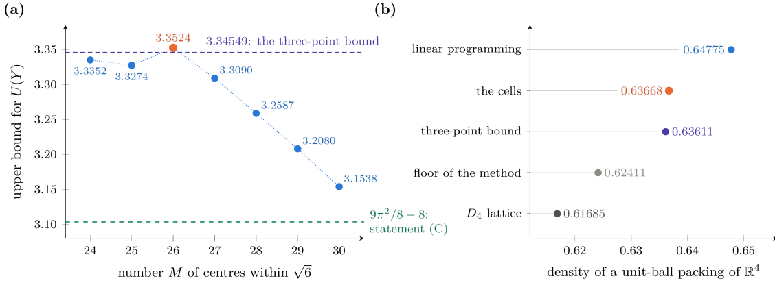
FIGURE 42. The density bound of Theorem 7.2. (a) The levels L_M of Proposition 7.1 against the level \frac{9}{8}\pi^2 - 8 that statement (C) asks for (green) and the level 3.34549 below which every count would have to fall for the bound to pass the three-point bound (violet). Only M = 26 lies above the second. (b) The resulting bound with the others for \mathbb{R}^4 : the density \pi^2/16 of D_4 , the floor of Remark 7.3, the three-point bound [CdLS22], and the linear programming bound [CE03].
