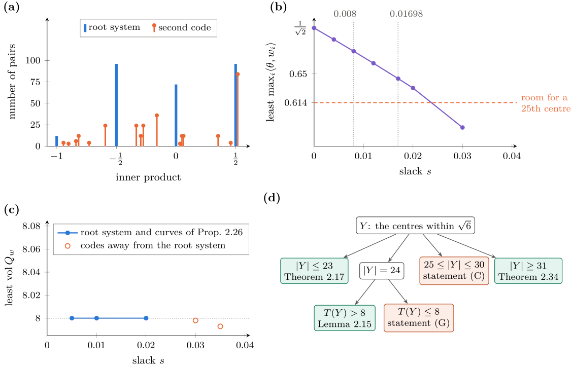
FIGURE 37. Twenty-four-point codes at positive slack, and the two statements that remain. (a) The inner products of the 276 pairs of the root system and of the second code of Proposition 6.21. (b) The deepest hole of a 24-point code of slack s , the least value of \max_i \langle \theta, w_i \rangle found; a further centre within \sqrt{6} beside twenty-four within 2.0161 needs 0.6141 or less, which the codes found reach only near s = 0.025 , beyond the slack 0.008 of Theorem 4.73 and the slack 0.01698 of the second code. (c) The least contact-cell volume found over codes of slack s . (d) The cases of Proposition 6.23; the green boxes are proved, the orange ones are statement (G) and statement (C) for twenty-five to thirty centres, (C) being proved from thirty-one on by Theorem 6.25. Panels (b) and (c) are floating-point minimisations, evidence and not bounds.
