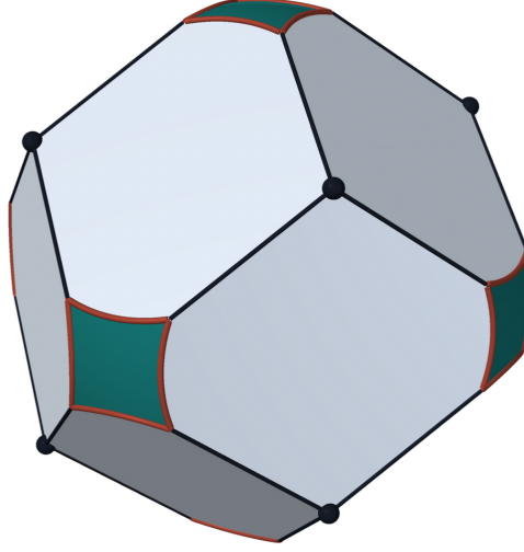
FIGURE 18. The truncated cell in dimension three: the Voronoi cell of the face-centred cubic lattice at inradius 1, a rhombic dodecahedron, cut by the ball of radius (3/2)^{1/2} . The ball passes through the eight three-valent vertices (dark) and replaces the six four-valent corners by spherical squares (teal). Inside the ball the cell is an exact function of the pair angles of its twelve contact directions.
