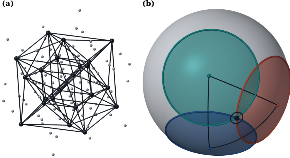
FIGURE 16. (a) The 600-cell seen from one vertex, radius proportional to angle: its vertices in shells at 36^\circ to 144^\circ (grey) and, darker and joined by their 88 edges, the 23 vertices of an inscribed 24-cell, the centre among them, whose twenty-fourth vertex is the antipode at 180^\circ and is not drawn; they form a deletion. (b) The cap lemma on a great 2-sphere: three contact directions 60^\circ apart carry caps of radius r_* = 35.26^\circ that meet in exactly one point, the circumcentre of their triangle (ringed); any smaller radius separates them.
