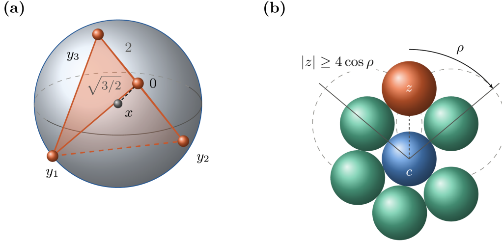
FIGURE 27. Two elementary facts behind Section 6.1, to scale. (a) Lemma 6.6: four points pairwise at least 2 apart do not fit in a ball of radius less than \sqrt{3/2} , and the regular tetrahedron of edge 2 in the ball of radius \sqrt{3/2} is the extreme case; so no point x of the open ball B(\sqrt{3/2}) about the centre 0 is closer to three other centres than to 0. (b) Lemma 6.3 in a plane section: the balls of the contacts (green) leave a hole of angular radius \rho , here 50^\circ , and a further centre z can enter it only at a distance |z| \geq 4 \cos \rho from c , where it meets the circles of radius 2 (dashed) about the two contacts at the rim.
