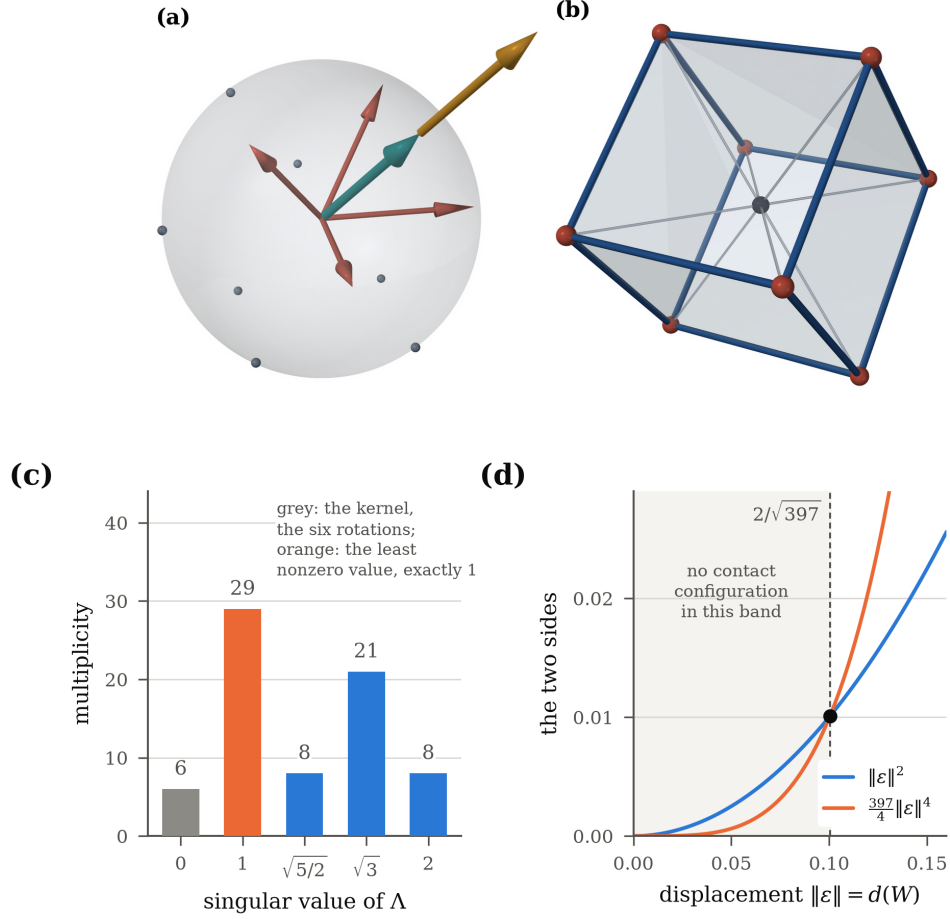
FIGURE 13. (a) The neighbour sum in dimension three, where it fits in one picture: a contact direction of the face-centred cubic lattice (teal), the four contact directions at 60^\circ from it (clay), and their sum (ochre), which is twice the direction itself. (b) The same identity in dimension four, drawn where it lives. The eight roots at inner product 1 from a root \alpha fill the hyperplane \langle \alpha, x \rangle = 1 , a copy of \mathbb{R}^3 , as the vertices of a cube centred at \alpha/2 (dark); eight times that centre is 4\alpha . (c) The singular values of the rigidity operator \Lambda on the 72-dimensional tangent space, with multiplicities (Lemma 4.50). The kernel is the six infinitesimal rotations, and the smallest nonzero value is one of the two constants that turn the first-order argument into a radius; the other is the weight \frac{11}{16} that every pair carries in the image of \Lambda . (d) The two sides of the inequality that closes Theorem 4.51. Feasibility forces \|\epsilon\|^2 \leq \frac{397}{4}\|\epsilon\|^4 , so the displacement is either zero or at least 2/\sqrt{397} : the shaded band holds no contact configuration of 24 directions.
