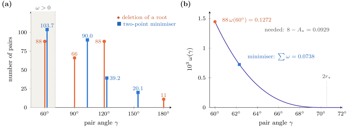
FIGURE 12. Pair angles at twenty-three contacts. (a) The 253 pair angles of the deletion of a root (clay) and the measure that minimises \sum_{i < j} \omega(\gamma_{ij}) over all pair distributions satisfying the Bonferroni inequality and positive definiteness (blue, Remark 4.45). Only pairs closer than 2r_* = 70.53^\circ (shaded) carry weight. (b) The weight \omega of Proposition 4.41. The deletion collects 88\omega(60^\circ) = 0.1272 from its 88 pairs at 60^\circ ; the minimiser moves its 103.7 close pairs out to 62.3^\circ , where \omega has halved, and collects 0.0738, short of the 0.0929 that (4.30) requires.
