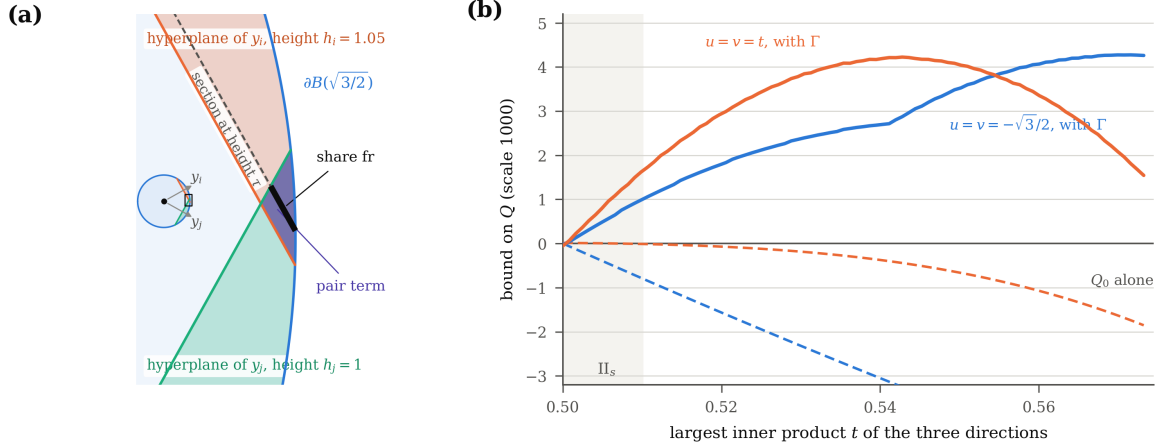
FIGURE 30. (a) A plane section through c and two centres at the packing boundary |y_i - y_j| = 2 , with d_i = 2.10 and d_j = 2 , so that the cosine a(d_i, d_j) = 0.525 of their angle exceeds \frac{1}{2} , which two contacts cannot do; the inset shows the whole section and the window. Beyond the two hyperplanes lie the caps (orange, green) and their overlap, the pair term (violet). The section of B(\sqrt{3}/2) at height \tau (dashed) meets the second cap in the share fr (thick). To scale. (b) The bound along two lines past the face t = \frac{1}{2} where contacts end: Q_0 alone (dashed) turns negative, while Q_0 plus the lower bound for \Gamma_1 + \Gamma_2 + \Gamma_3 that the proof uses (solid) stays positive. Blue: u = v = -\frac{\sqrt{3}}{2} , where (4.49) comes nearest to equality on the face; orange: u = v = t . The shaded strip is the range \Pi_s . The scale is that of the computation, 1000 times the volume.
