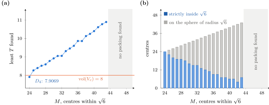
FIGURE 33. The right side of Lemma 6.6 for every count of centres within \sqrt{6} , computed by local minimisation in floating point. (a) The least value found for M centres, M = 24, \dots, 43 , against the level 8; at M = 24 it is the root system, 7.906940\dots . For M \geq 44 no packing was found, in 300 random starts for each count. (b) How the configurations of (a) meet the count: the centres strictly inside the sphere of radius \sqrt{6} , and those on it, whose caps are empty.
