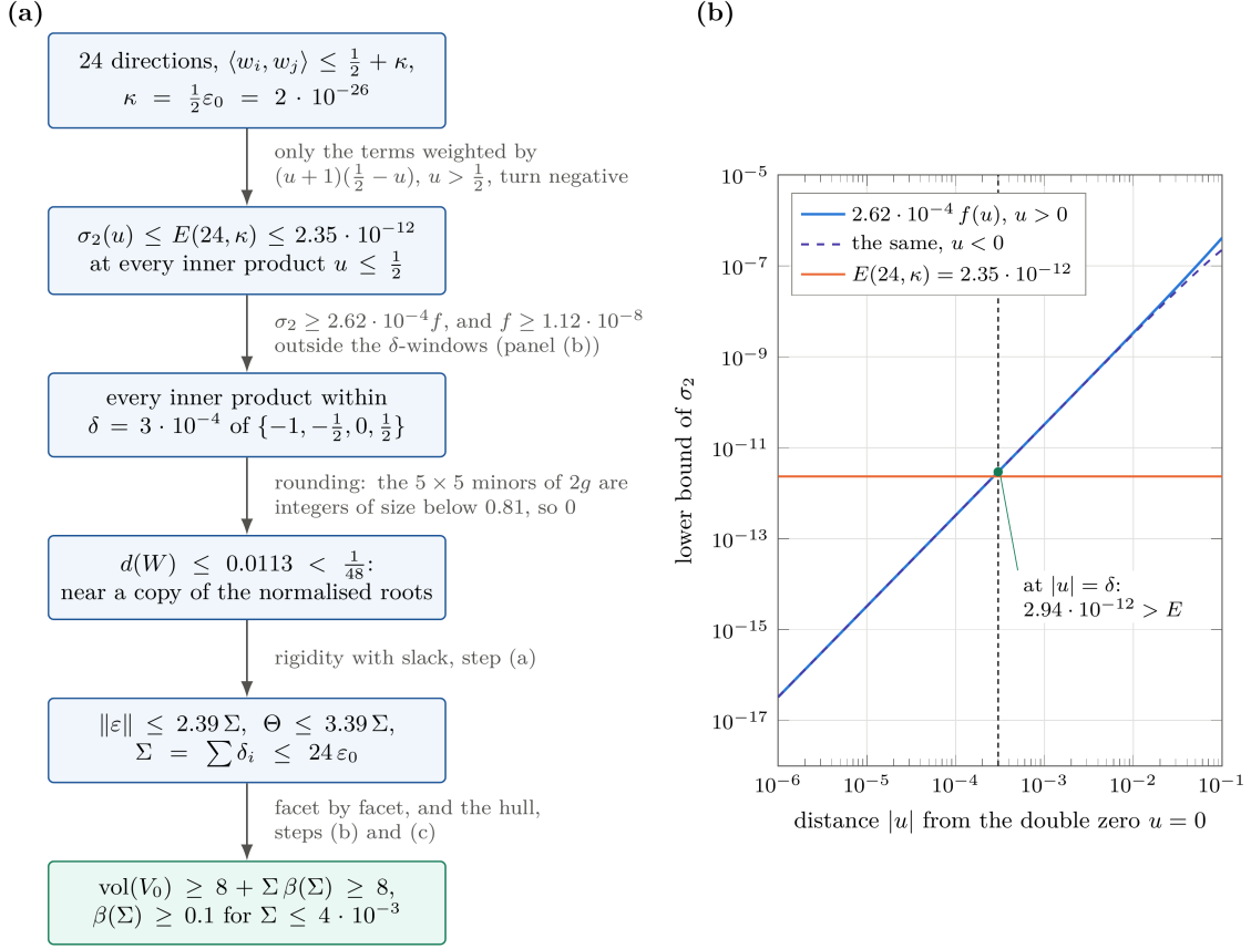
FIGURE 21. Where \varepsilon_0 = 4 \cdot 10^{-26} comes from. (a) The chain of explicit bounds that replaces the compactness argument of Theorem 6.9, with the number each step produces. Twenty-four directions with inner products at most \frac{1}{2} + \kappa make every sign-changing sum-of-squares term of the certificate at least -E in total (Theorem 4.70); so \sigma_2 \leq E at each inner product up to \frac{1}{2} , which pins it near a zero of \sigma_2 ; Lemma 4.71 turns that into a distance from the root system; the rigidity of Theorem 4.51, with slack, bounds the displacement by the sum S of the distances beyond contact; and the facet, moment and hull estimates close the argument. (b) To scale: the lower bound 2.62 \cdot 10^{-4}f(u) of \sigma_2 near its double zero u = 0 , for u > 0 and u < 0 , against the level E(24, \kappa) = 2.35 \cdot 10^{-12} . The two cross at |u| \approx 2.7 \cdot 10^{-4} , inside the window |u| \leq \delta = 3 \cdot 10^{-4} , where the bound is already 2.94 \cdot 10^{-12} . The other double zero, -\frac{1}{2} , gives the same picture; at the simple zeros -1 and \frac{1}{2} the bound is linear and the window is far wider than needed.
