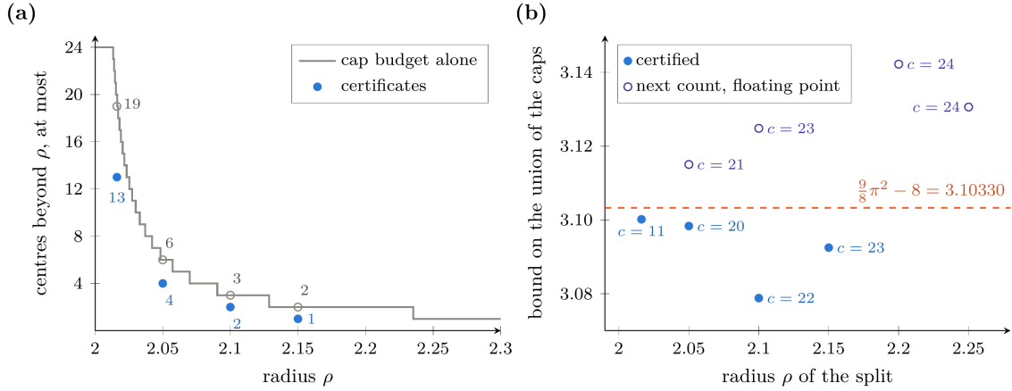
FIGURE 41. Proposition 6.36. (a) For twenty-four centres with T(Y) \leq 8 , the number that can lie beyond a radius \rho : the cap budget alone (step curve, open marks) against the counts that the case certificates prove (filled marks), 13 beyond 2.0161, 4 beyond 2.05, 2 beyond 2.1 and 1 beyond 2.15. (b) For the split N(\rho) \leq c - 1 against N(\rho) \geq c , the bound on the union of the caps in the first case: proved by a certificate (filled marks) and, for the next count, the optimum of the programme of the same degree (open marks), which is not a bound, against the level \frac{9}{8}\pi^2 - 8 that T(Y) > 8 needs.
