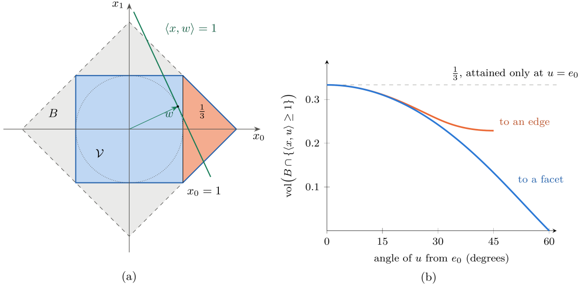
FIGURE 24. The cap argument of Section 5. (a) The plane x_2 = x_3 = 0 in the frame of four orthogonal roots, the deviating root being e_0 , to scale. The cross-polytope B (dashed) meets it in a square, the polytope Q of the twenty-three undeviated roots in the pentagon outlined in blue, and the 24-cell \mathcal{V} in the inner square; the dotted circle is the unit sphere. The half-space x_0 \geq 1 cuts the same piece off Q and off B (orange), of volume \frac{1}{3} in \mathbb{R}^4 , so that \text{vol } Q = 8 + \frac{1}{3} . A deviated contact replaces it by a half-space \langle x, w \rangle \geq 1 tangent to the unit sphere (green). (b) The volume that \langle x, u \rangle \geq 1 cuts off B , from Lemma 5.4, along two arcs of unit normals u leaving the vertex direction e_0 : towards the midpoint of an edge, u = (\cos t, \sin t, 0, 0) , and towards the centre of a facet, u = (\cos t, s, s, s) with s = \sin t/\sqrt{3} . Both stay below \frac{1}{3} for t > 0 , as Theorem 5.6 asserts for every u . In the plane of panel (a) alone the comparison would go the other way, which is why the theorem needs the four-dimensional cap formula.
