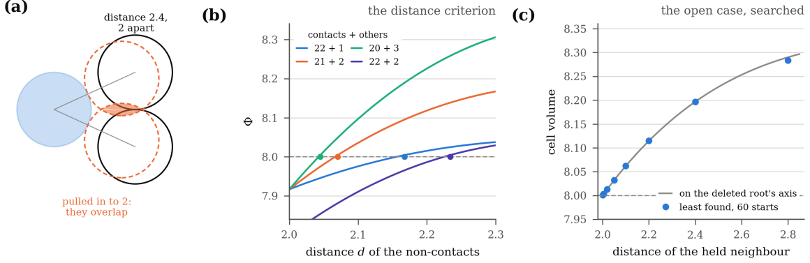
FIGURE 26. Neighbours that do not touch. (a) A two-dimensional section, to scale: two centres at distance 2.4 from the central one and 2 from each other, a packing; pulled in to distance 2 they overlap (shaded), so the configuration at the all-contact corner is not a packing, and Lemma 2.9 gives a lower bound and not a contact configuration. (b) The distance criterion of Proposition 6.1 for m contacts and k further centres at a common distance d ; it passes 8 at the thresholds of Table 2 (dots). (c) The remaining case is tight: the volume \frac{25}{3} - \frac{1}{3}(1 - \frac{\delta}{2})^4 of the cell of the deletion of a root with one further centre at distance 2 + \delta on the deleted root's axis, which tends to 8 as \delta \rightarrow 0 , and the least volume found by local minimisation from 60 starts with one neighbour held at distance 2 + \delta . None is below 8.
