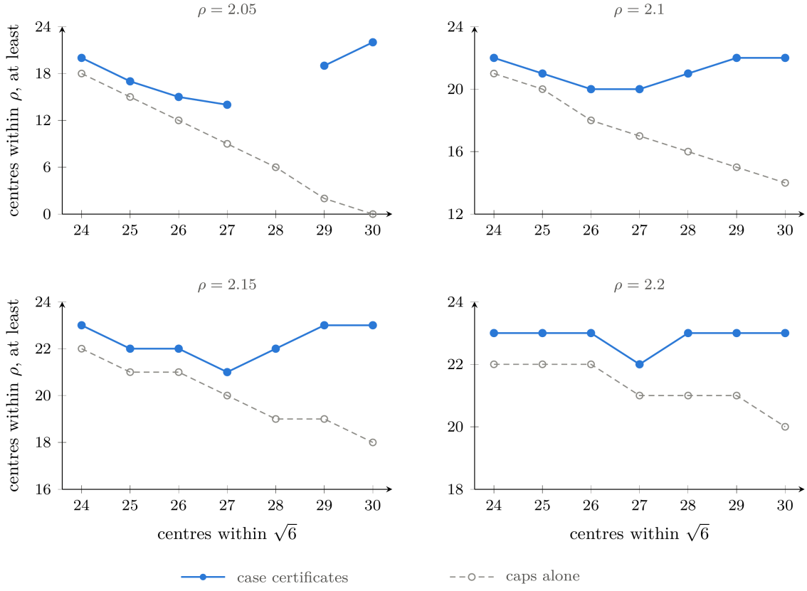
FIGURE 40. Proposition 6.33: for M centres within \sqrt{6} of c with T(Y) \leq 8 , the least number within 2.05, 2.1, 2.15 and 2.2 of c , as the case certificates prove it (filled marks) and as the caps alone force it (open marks). At M = 24 the counts are those of Proposition 6.36, and at M = 30 and \rho = 2.1 that of Theorem 6.31.
