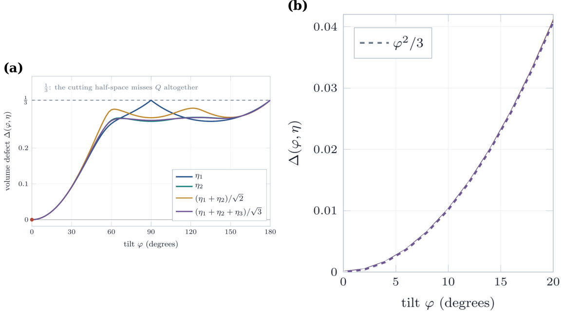
FIGURE 23. (a) The volume defect \Delta(\varphi, \eta) over the whole range of tilts, for four deviation directions spanning the transverse sphere: two of the orthonormal frame directions and two diagonal combinations of them. The defect is nonnegative throughout and vanishes only at \varphi = 0 , as Theorem 13.7 asserts, and it returns to the value \frac{1}{3} at \varphi = \pi , where the cutting half-space misses Q entirely and the cell is exactly Q itself. The intermediate maxima and minima are where the breakpoint structure of Section 9 shows itself. The curves are computed from directly enumerated cell volumes, by a route independent of the proof. (b) The same four curves at small tilt, against the second-order rate \varphi^2/3 of Proposition 13.9. The four are indistinguishable there, and from each other, at plotting accuracy.
