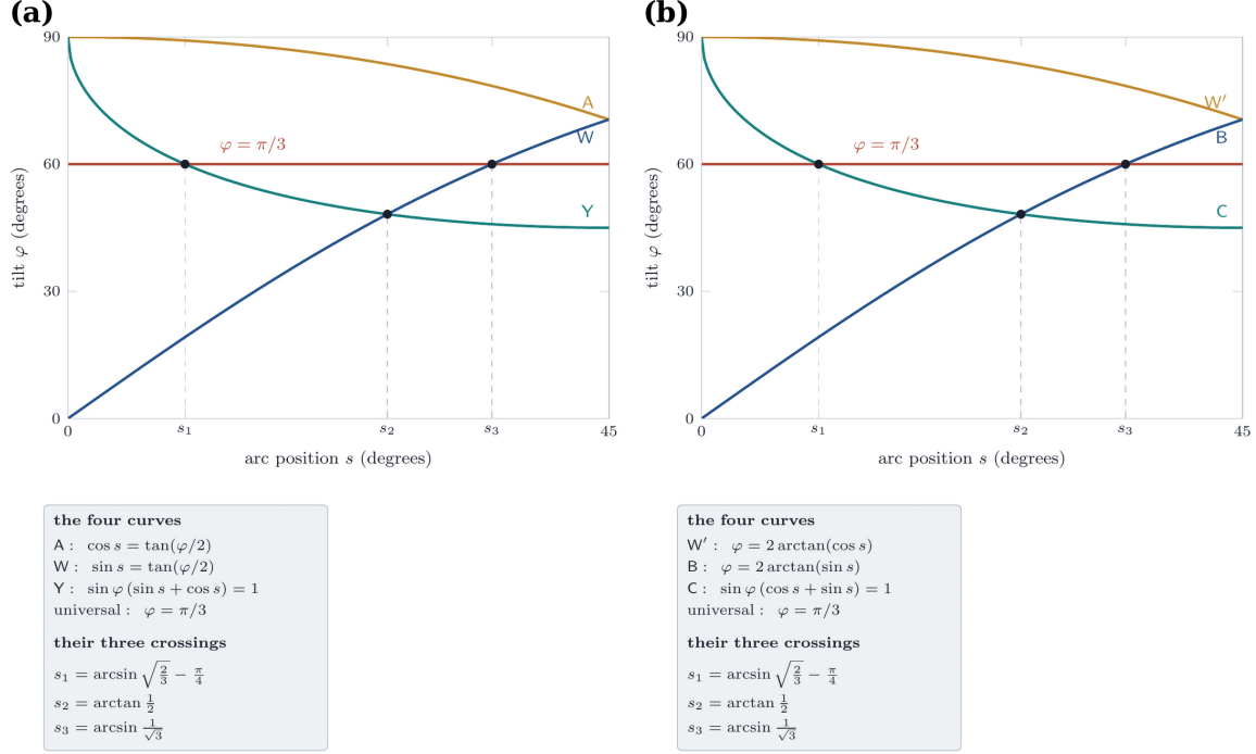
FIGURE 20. (a) The four breakpoint curves of the first arc, drawn to scale from the closed forms of Theorem 9.1: the universal curve \varphi = \pi/3 and the curves A, W, Y. They meet in exactly three points, at the abscissae s_1 , s_2 , s_3 listed at the right, and the eight combinatorial regions of Section 10.2 are the cells of the resulting arrangement. The curves A and W meet only at s = \pi/4 , where the reflection symmetry of the arc identifies them. (b) The four breakpoint curves of the second arc, drawn to scale from the closed forms of Theorem 11.1. Comparing with Figure 20(a) shows what Proposition 8.5 later proves: the three equations here are exactly those of A, W and Y on the first arc, and the arrangement, crossings included, is the same one, even though the curves come from different vertices of \mathcal{V} . The band immediately below region top splits into three sub-parts at the crossings s_1 , s_2 , s_3 .
