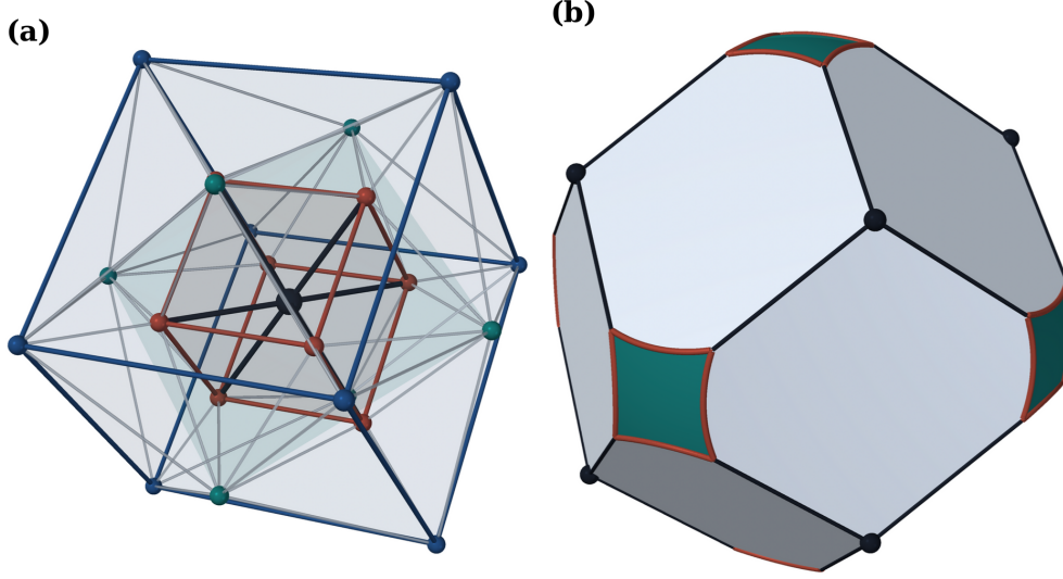
FIGURE 16. (a) The contact graph of the root system from one root (dark, at the centre), the other twenty-three at radius proportional to angle: a cube at 60^\circ (clay), an octahedron at 90^\circ (teal), a cube at 120^\circ (blue), and the 88 tight pairs among them; the eight at the centre are drawn dark, and they sum to four times it. (b) The truncated cell in dimension three: the Voronoi cell of the face-centred cubic lattice at inradius 1, a rhombic dodecahedron, cut by the ball of radius (3/2)^{1/2} . The ball passes through the eight three-valent vertices and replaces the six four-valent corners by spherical squares (teal).
