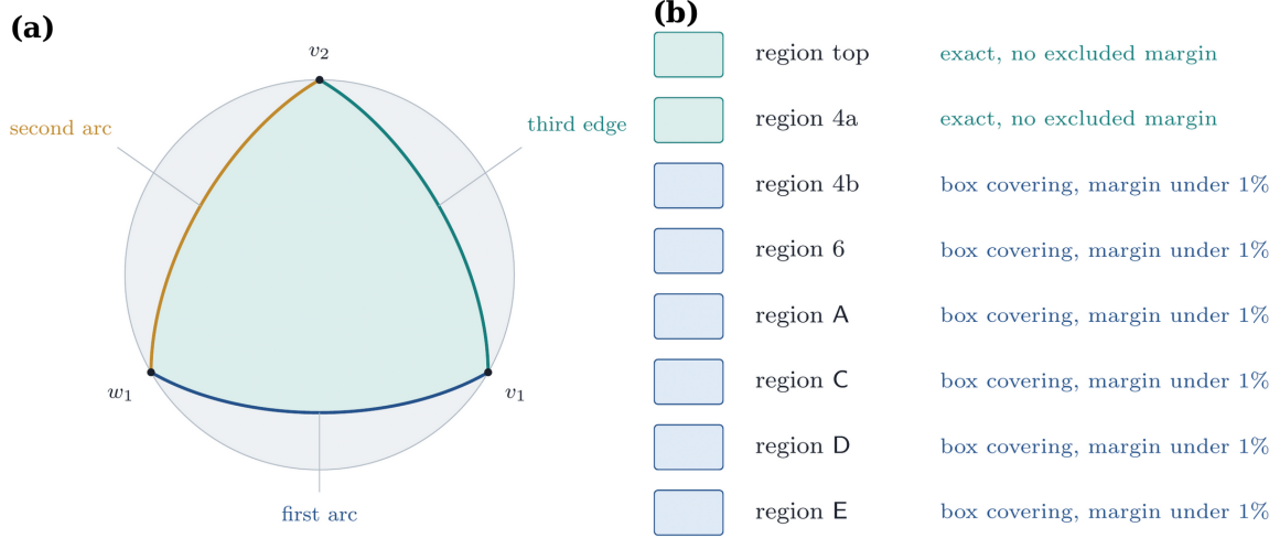
FIGURE 21. (a) The transverse sphere of deviation directions and the spherical octant left by the two symmetries of Lemma 8.1. The vertices v_1, w_1, v_2 are pairwise orthogonal, so the octant's three edges are quarter great circles, and \langle S, H \rangle \cong S_3 fixes u_0 and permutes them; a certificate on the first arc is therefore a certificate on the whole boundary of the octant. (b) The eight combinatorial regions of the first arc and the kind of certificate each carries. Two are exact with no excluded margin; the other six are certified by box covering, with the excluded margin in each case a few tenths of one percent of the region's own area. Through the identifications of Propositions 8.3 and 8.5, these eight certificates cover the whole boundary of the octant.
