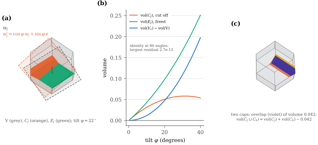
FIGURE 4. The free-volume identity of Theorem 7.1, drawn on real geometry. Because the identity holds in every dimension, it is drawn in three, where its pieces can be seen: the reference cell is the Voronoi cell of the face-centred cubic contacts, the rhombic dodecahedron \{x : \langle x, w_i \rangle \leq 1\} over the twelve directions (\pm 1, \pm 1, 0)/\sqrt{2} and permutations. (a) One direction w_j tilted by 22^\circ to w_j ; the cap C_j is what the tilted half-space cuts off the cell and E_j is what the motion frees beyond the old facet, both computed as half-space intersections and drawn to scale. (b) The two volumes and their difference against the tilt, each piece computed as a polytope of its own; the identity holds at every angle to the precision of the arithmetic. (c) Two directions tilted towards each other: the caps overlap, so for m \geq 2 the corrections are volumes of unions and not sums of volumes (Remark 7.2).
