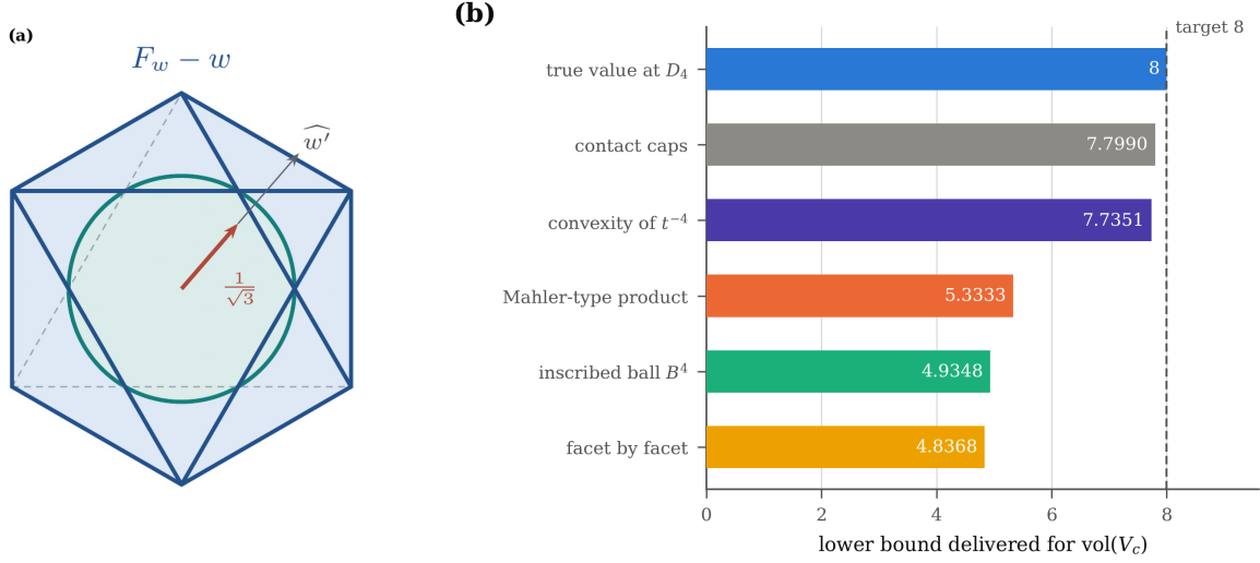
FIGURE 5. (a) A single facet of the reference cell, drawn inside the 3-space orthogonal to its own contact direction. At the root configuration the eight tight neighbours cut out the regular octahedron (Lemma 7.11); the pairwise contact condition on its own guarantees no more than the inscribed ball, and the gap between the two is what the boundary form (7.6) has to absorb. (b) The bounds the boundary form and the other global routes actually deliver, all of them evaluated at the D_4 configuration where the conjecture is tight (Remarks 7.12 and 7.13).
