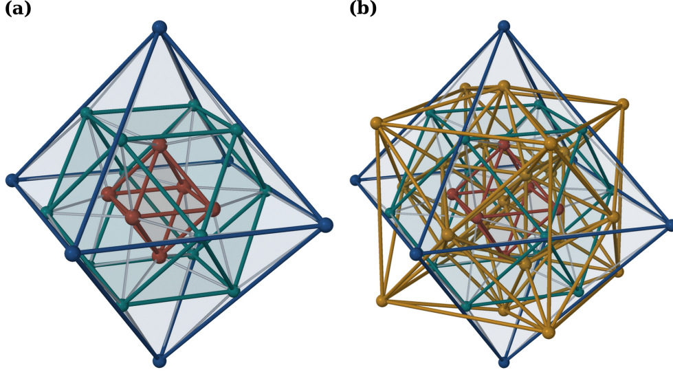
FIGURE 12. (a) The 24 contact directions of D_4 seen from a deep hole, radius proportional to angle: an octahedron at 45^\circ (clay), a cuboctahedron at 90^\circ (teal), an octahedron at 135^\circ (blue), and the 96 pairs at 60^\circ as edges. (b) The same, with the dual 24-cell added (ochre): the 48 directions of the binary octahedral group, a cube, an octahedron and a cube about the hole, which is now itself a direction.
