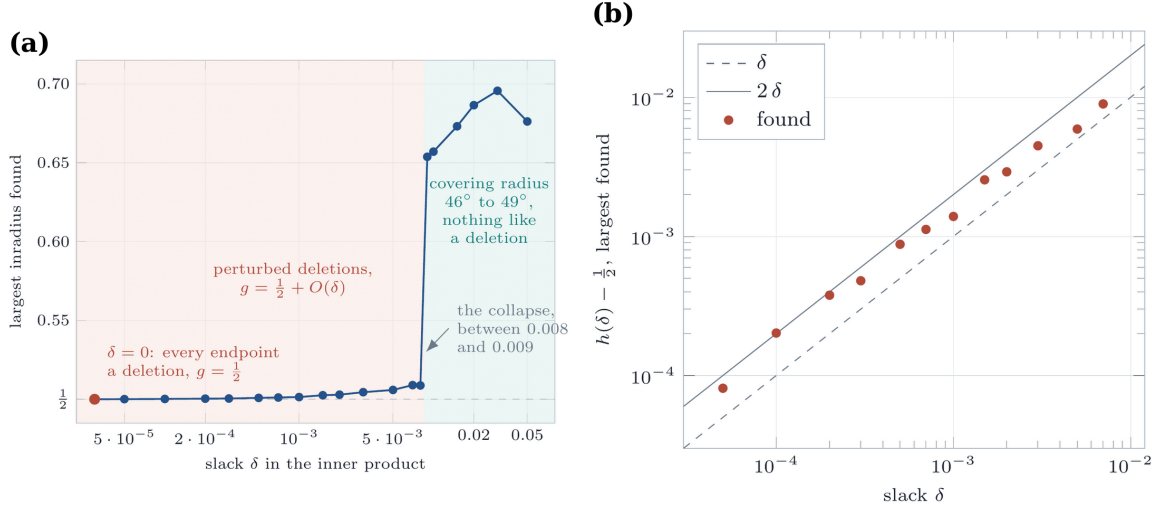
FIGURE 13. (a) The continuation of Table 2: the largest inradius found, against \delta on a logarithmic axis. The plateau near \frac{2}{3} runs down to \delta = 0.009 and is carried by configurations far from any deletion; from \delta = 0.008 down it collapses to \frac{1}{2} + O(\delta) . (b) The same table below the collapse: h(\delta) - \frac{1}{2} against \delta on logarithmic axes, with the lines \delta and 2\delta for comparison. The approach to \frac{1}{2} is linear in \delta , which is what a perturbed deletion gives.
