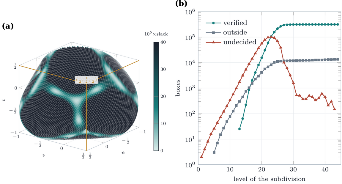
FIGURE 18. (a) The domain of the certificate condition: the admissible region of Lemma 7.72 in three dimensions, where the triples (u, v, t) of pairwise inner products of three contact directions fill the part of the cube [-1, \frac{1}{2}]^3 enclosed by the surface of coplanar triples. The surface is coloured by the slack of (7.47), which is least along the curves where two of the three directions are nearly antipodal. (b) The branch and bound of the proof of Theorem 7.73, level by level: the boxes live, the boxes discarded on the enclosure, and the width reached.
