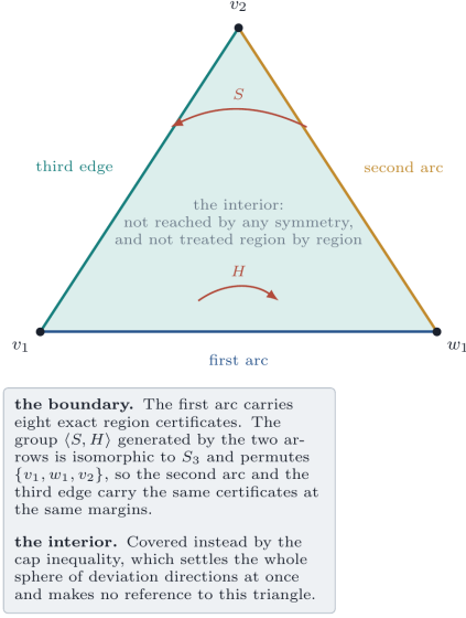
FIGURE 19. The fundamental domain of Lemma 8.1: one triangle with vertices v_1, w_1, v_2 , obtained from the full sphere of deviation directions by the two order-2 symmetries S and H . The three edges carry the certificates of Sections 10 and 12, through the identifications of Propositions 8.3 and 8.5; the interior is settled separately, in Section 13, by an argument that does not use the triangle at all.
