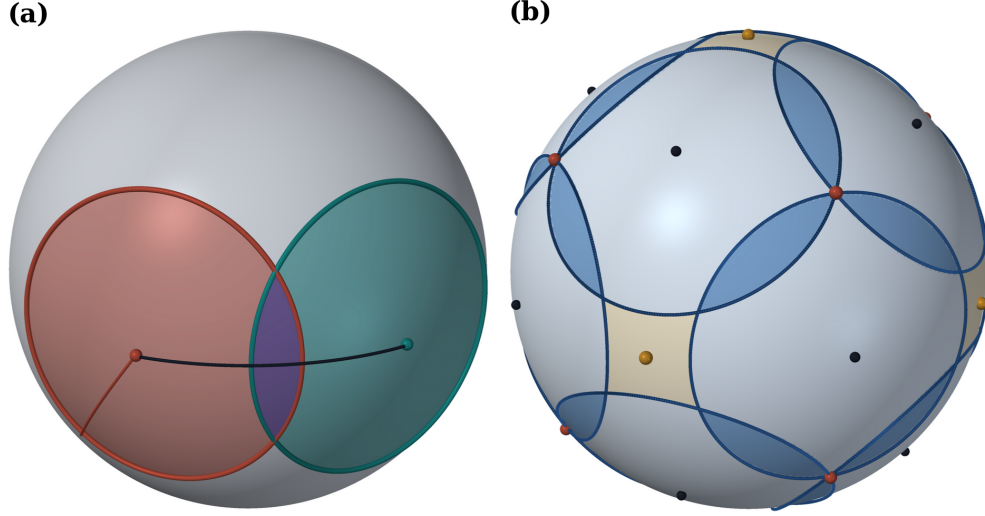
FIGURE 15. (a) Two contact directions at angle \gamma = 60^\circ and their caps of radius r = r_* . The lens in which the caps overlap (violet) has measure \Lambda(r, \gamma) , and \omega(\gamma) integrates it against d(\sec^4 r) ; the dark arc is \gamma and the clay arc is r . (b) The caps of radius r_* about the twelve contact directions of the same lattice, the sphere shaded by how many caps cover it: one (pale blue), two in the lenses, three at the eight triangle circumcentres (clay), and none in the six square holes (ochre).
