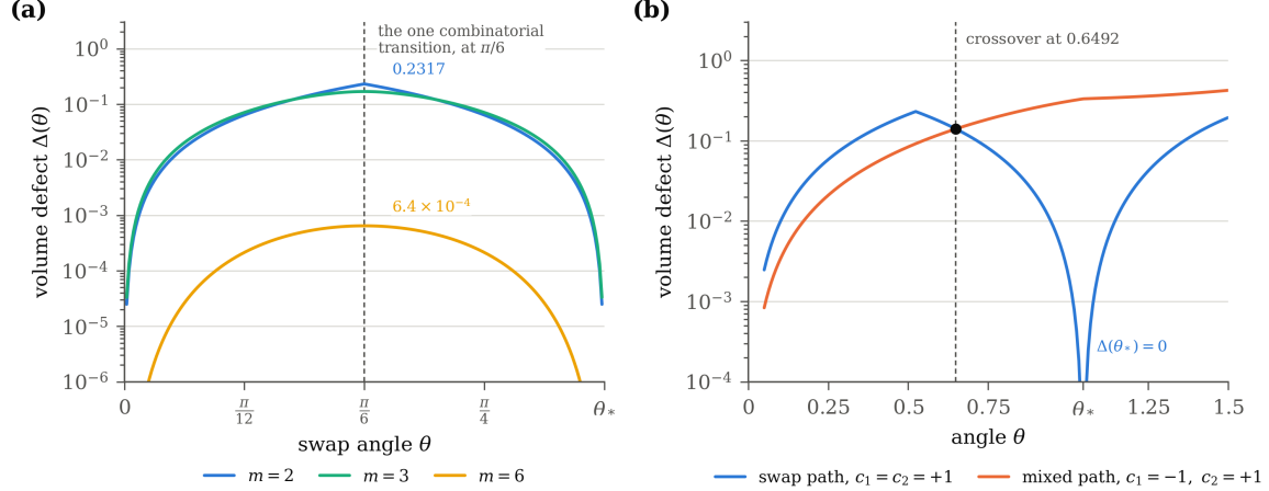
FIGURE 26. (a) The volume defect along the three swap paths of this section, over the whole packing-valid range (0, \theta_*) , \theta_* = \pi/3 . The vertical scale is logarithmic because the three sit nearly three orders of magnitude apart: the two-direction and three-direction paths peak at 0.2317 and 0.1692 at the midpoint, the six-direction path at 6.4 \times 10^{-4} . All three are positive throughout and vanish at both ends, which is what Theorems 20.2 to 20.4 assert exactly. The dashed line is the single combinatorial transition, at \theta = \pi/6 , visible as the corner in the m = 2 curve; the m = 6 path has none, and its curve is smooth there. The values plotted are enumerated cell volumes, computed by swap_defect_curves.py through a route independent of the closed forms, and for m = 6 they agree with the closed form of Section 20.6 to 9 \times 10^{-9} . (b) The swap path against the mixed path, the two differing only in the sign c_1 . The more adversarial of the two is the lower one, and which that is changes at \theta = 0.6492 : below the crossover the mixed path is lower, at \theta = 0.05 by 0.000834 against 0.002474, and above it the swap path is, through \theta_* and beyond. Second-order theory cannot tell the two apart, since the Hessian entry that distinguishes them enters only through its magnitude. The zero of the swap curve at \theta_* is the swap point itself, where the configuration is again a root system.
