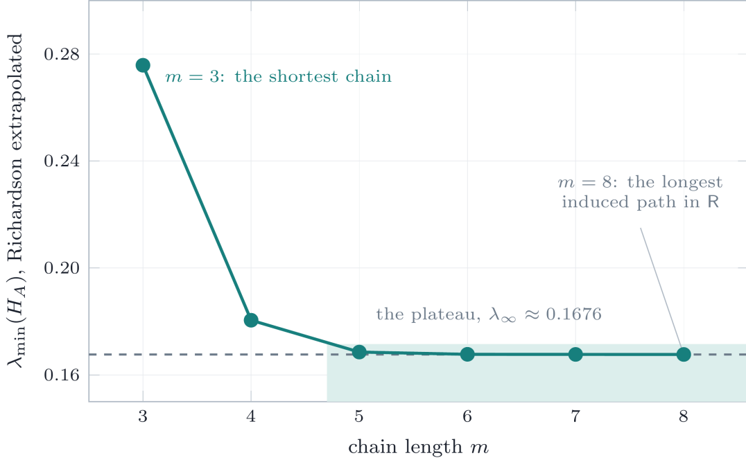
FIGURE 24. Richardson-extrapolated minimum eigenvalue of the joint Hessian H_A for chain configurations of length m = 3, \dots, 8 (Lemma 15.3; full values in Appendix G). The eigenvalue falls sharply from m = 3 to m = 5 and then plateaus near 0.1676 instead of continuing to collapse, which is the antipodal-axis mechanism described below. It stays well clear of zero for every chain length up to m = 8 , the longest induced path in the contact graph of R , so the second-order method certifies positivity on the whole chain family.
