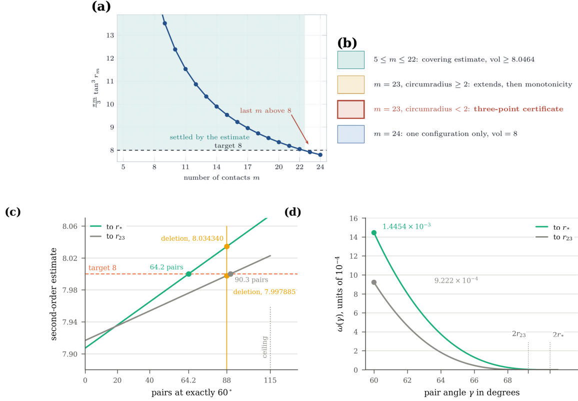
FIGURE 9. (a) The covering bound (7.12) at every admissible contact count m , against the target 8. It clears the target for all m \leq 22 and falls below at m = 23 . (b) How each part of the range of contact counts is settled: the estimate below 22 (Corollary 7.17), extension followed by monotonicity at 23 when the circumradius reaches 2 (Proposition 7.38), and the classification at 24 (Theorem 7.25). The third row is settled by the pair inequality of Theorem 7.69 and its certificate, Theorem 7.73. (c) The pairwise estimate at m = 23 , for the two integration limits r_{23} and r_* : the right-hand side of (7.17) as a function of the number of pairs at exactly 60^\circ , with the bracket alone at 0 pairs, the deletion configuration at 88 on both lines, the crossings of the target at 90.3 and at 64.2 pairs, and the elementary ceiling of Proposition 7.41 at 115. (d) The per-pair weight \omega(\gamma) for each integration limit: 0.000922\dots and 0.001445\dots at 60^\circ , vanishing at 2r_{23} = 69.2213\dots^\circ and at 2r_* = 70.5288\dots^\circ .
