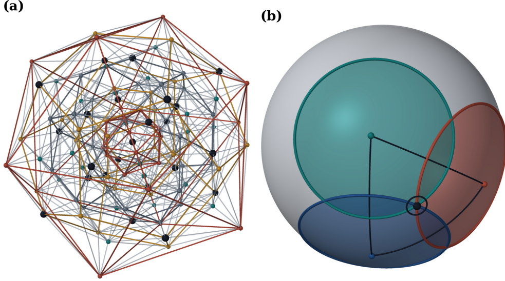
FIGURE 14. (a) The 600-cell seen from one vertex, its 119 other vertices in shells at 36^\circ to 144^\circ with 708 of the 720 edges at 36^\circ ; the dark points are an inscribed 24-cell whose far vertex is the one at infinity, that is, a deletion. (b) The cap lemma on a great 2-sphere: three contact directions 60^\circ apart carry caps of radius r_* = 35.26^\circ that meet in exactly one point, the circumcentre of their triangle (ringed); any smaller radius separates them.
