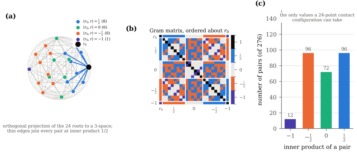
FIGURE 7. What Theorem 7.30 forces. (a) The twenty-four normalised roots of D_4 , projected orthogonally to a generic 3-space so that no two coincide, with every pair at inner product \frac{1}{2} joined; one root r_0 is singled out and the others are coloured by their inner product with it, eight at \frac{1}{2} , six at 0, eight at -\frac{1}{2} and the antipode at -1 . (b) The Gram matrix of the twenty-four directions, rows and columns ordered by these classes; it takes no value outside \{1, \frac{1}{2}, 0, -\frac{1}{2}, -1\} . (c) The 276 pairs by inner product: 96, 72, 96 and 12. The theorem says that every contact configuration of size 24 has a Gram matrix with the values of (b), and Lemma 7.26 that it then is (a) up to an orthogonal map.
