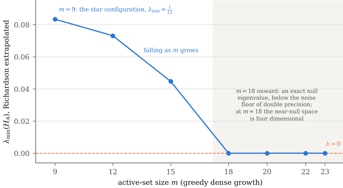
FIGURE 25. Richardson-extrapolated minimum eigenvalue of H_A under greedy dense growth, m = 9 through m = 23 (full values in Appendix G). The contrast with Figure 24 is the point: here there is no plateau above zero. From m = 18 onward, shaded, the extrapolated value is smaller than double-precision finite differences can resolve, which is the regime Section 17 takes up with arbitrary-precision arithmetic instead, and where the vanishing turns out to be exact.
