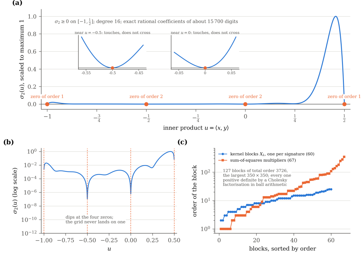
FIGURE 6. The certificate, as Proposition 7.29 reads it. (a) The two-point polynomial \sigma_2 on [-1, \frac{1}{2}] , evaluated exactly from the deposited rational coefficients and scaled by its maximum: it is nonnegative, it vanishes to first order at -1 and \frac{1}{2} and to second order at -\frac{1}{2} and 0 , and nowhere else; the insets show the two double zeros, where the curve touches the axis without crossing it. (b) The same on a logarithmic scale. (c) The orders of the 127 positive definite blocks, the sixty kernel blocks X_\lambda and the sixty-seven sum-of-squares multipliers; the largest is 350 \times 350 .
