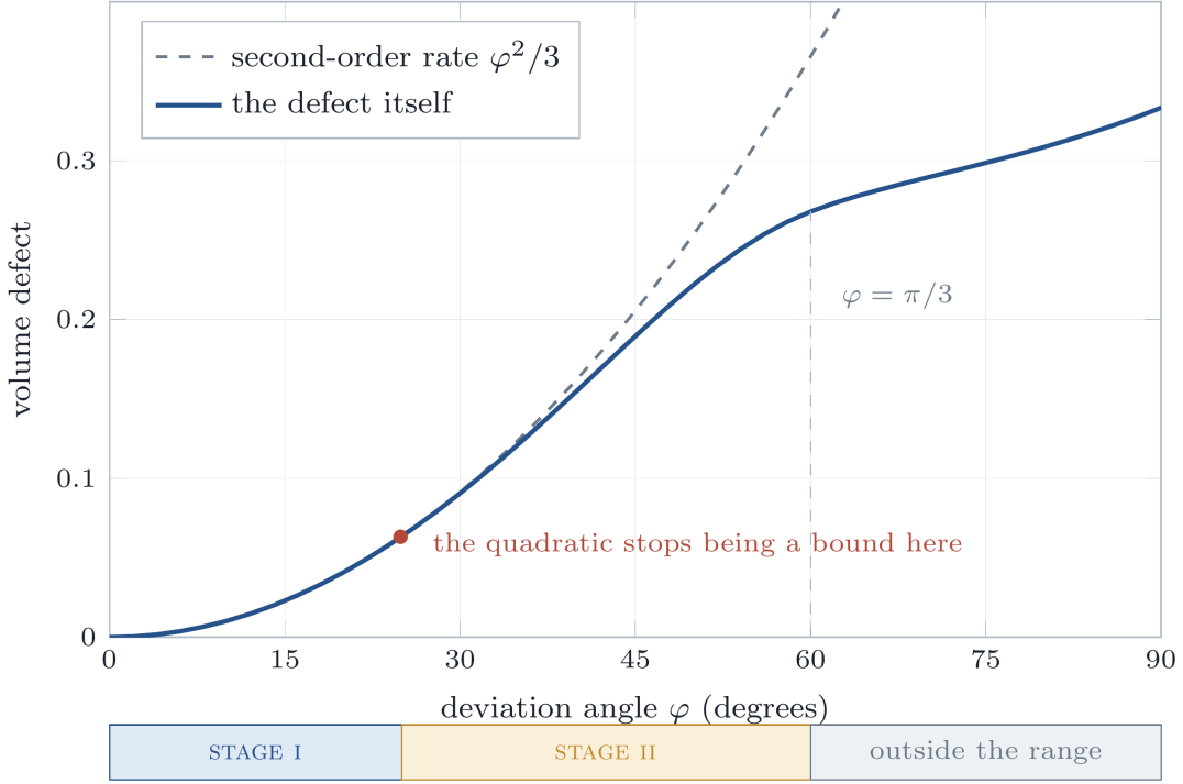
FIGURE 3. The computed volume defect for a root-aligned deviation, against the second-order rate \varphi^2/3 that STAGE I supplies. The two agree to plotting accuracy up to about 25^\circ and part company after it, the quadratic overtaking the defect and ceasing to be a lower bound; this is why the second-order argument alone does not reach the end of the range and STAGE II is needed. The strip beneath marks which argument covers which part of the range. The packing-valid range for a single deviation ends at \varphi = \pi/3 , where a second root becomes the nearest one.
