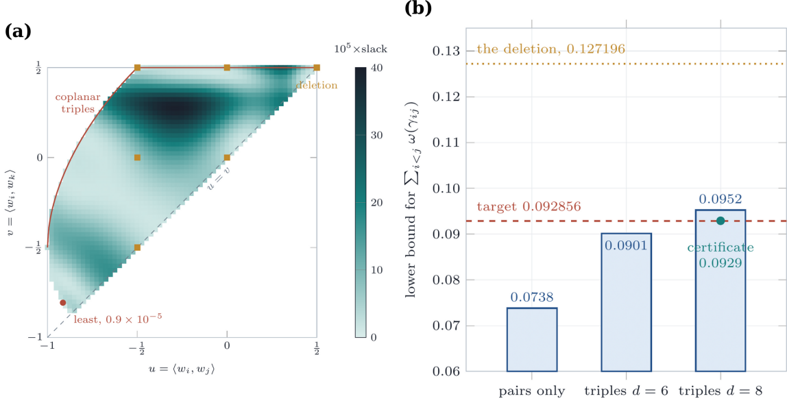
FIGURE 17. (a) The certificate of Theorem 7.73: the slack of the condition (7.47), the amount by which its left-hand side exceeds 0, on the slice of the admissible domain in which one pair of the triple is at 60^\circ . It is positive throughout, least near a coplanar triple with one nearly antipodal pair, and largest, about 4 \times 10^{-4} , in the interior. The six squares are the triples that occur in a deletion of a root. (b) The values of the relaxations against the target 8 - A_* : the pair angles alone (Proposition 7.44), the three-point relaxation at degrees 6 and 8, and the certificate, at which the bound is fixed at 0.0929 and the least slack is maximised.
