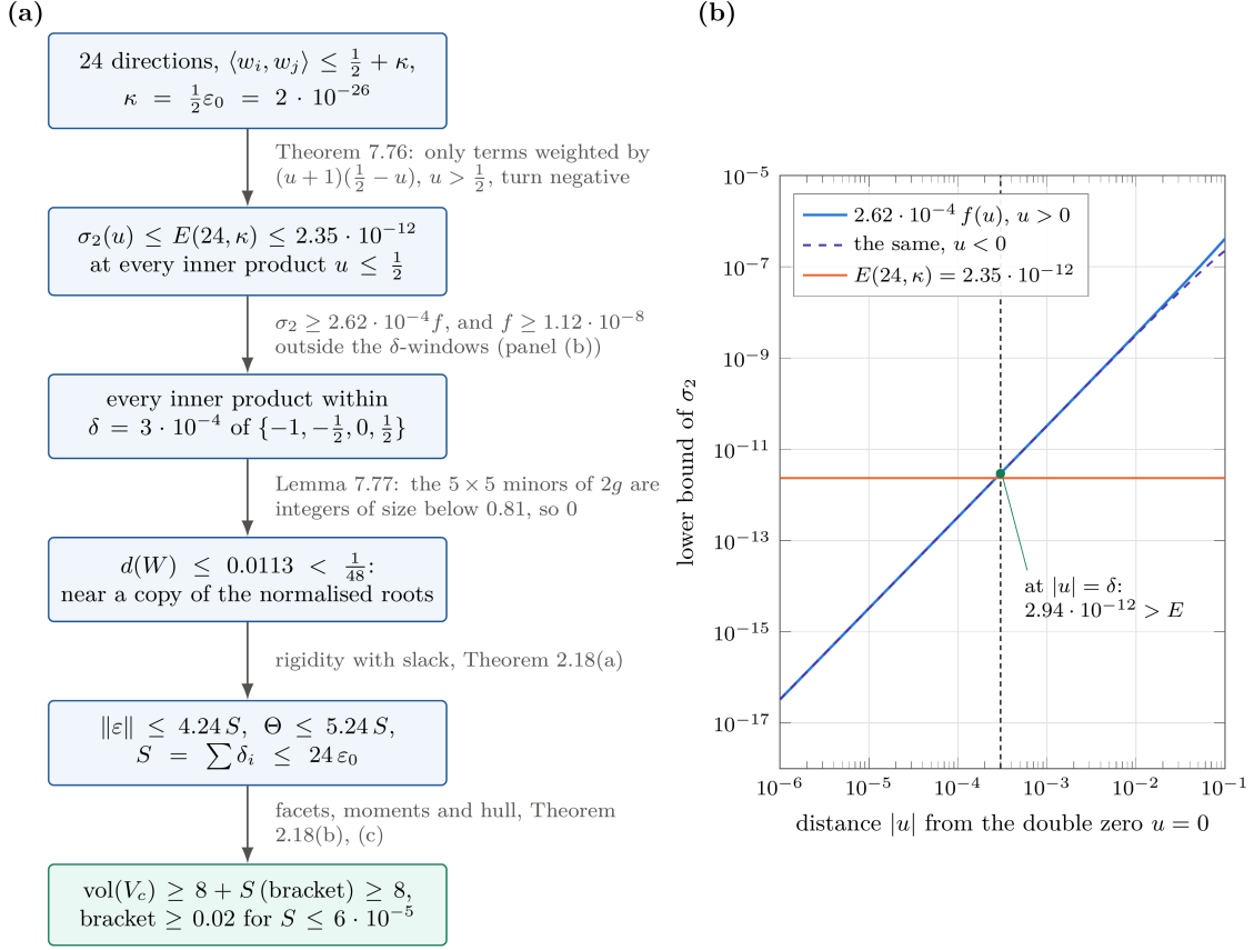
FIGURE 25. Where \varepsilon_0 = 4 \cdot 10^{-26} comes from. (a) The chain of explicit bounds that replaces the compactness argument of Theorem 2.18, with the number each step produces ( explicit_eps0.py ). Twenty-four directions with inner products at most \frac{1}{2} + \kappa make every sign-changing sum-of-squares term of the certificate at least -E in total (Theorem 7.76); so \sigma_2 \leq E at each inner product up to \frac{1}{2} , which pins it near a zero of \sigma_2 ; Lemma 7.77 turns that into a distance from the root system; the rigidity of Theorem 7.51, with slack, bounds the displacement by the sum S of the distances beyond contact; and the facet, moment and hull estimates close the argument. (b) To scale: the lower bound 2.62 \cdot 10^{-4} f(u) of \sigma_2 near its double zero u = 0 , for u > 0 and u < 0 , against the level E(24, \kappa) = 2.35 \cdot 10^{-12} . The two cross at |u| \approx 2.7 \cdot 10^{-4} , inside the window |u| \leq \delta = 3 \cdot 10^{-4} , where the bound is already 2.94 \cdot 10^{-12} . The other double zero, -\frac{1}{2} , gives the same picture; at the simple zeros -1 and \frac{1}{2} the bound is linear and the window is far wider than needed.
