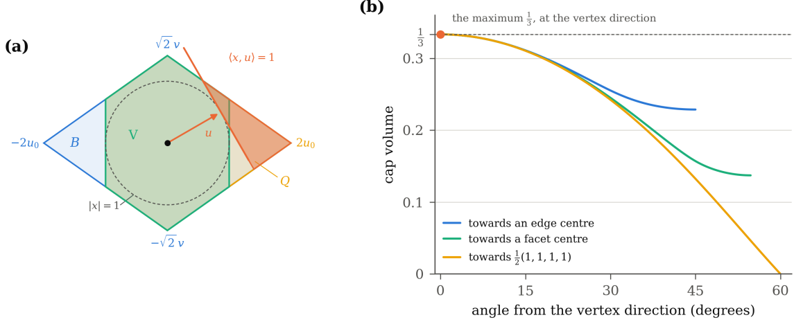
FIGURE 30. (a) The section of the reference cell \mathcal{V} , of Q , and of the cross-polytope B by the plane spanned by the base direction u_0 and one transverse direction. Coordinates are exact: the section of \mathcal{V} is a hexagon, that of Q the same hexagon with its right edge replaced by the two edges meeting at the apex 2u_0 , and that of B a rhombus through the same apex and the same two vertices \pm\sqrt{2}v . The dashed circle is the unit sphere, on which every contact hyperplane is tangent, and the shaded triangle is the section of the cap cut by a half-space at unit distance whose normal is tilted 30^\circ from u_0 . (b) The volume of the cap cut from the cross-polytope by a half-space at unit distance, along three great circles leaving a vertex direction: towards an edge centre, towards a facet centre, and towards \frac{1}{2}(1, 1, 1, 1) , where the half-space meets B only in its four positive vertices and the cap volume falls to zero. The maximum \frac{1}{3} of Theorem 13.6 is attained at the vertex direction, marked.
