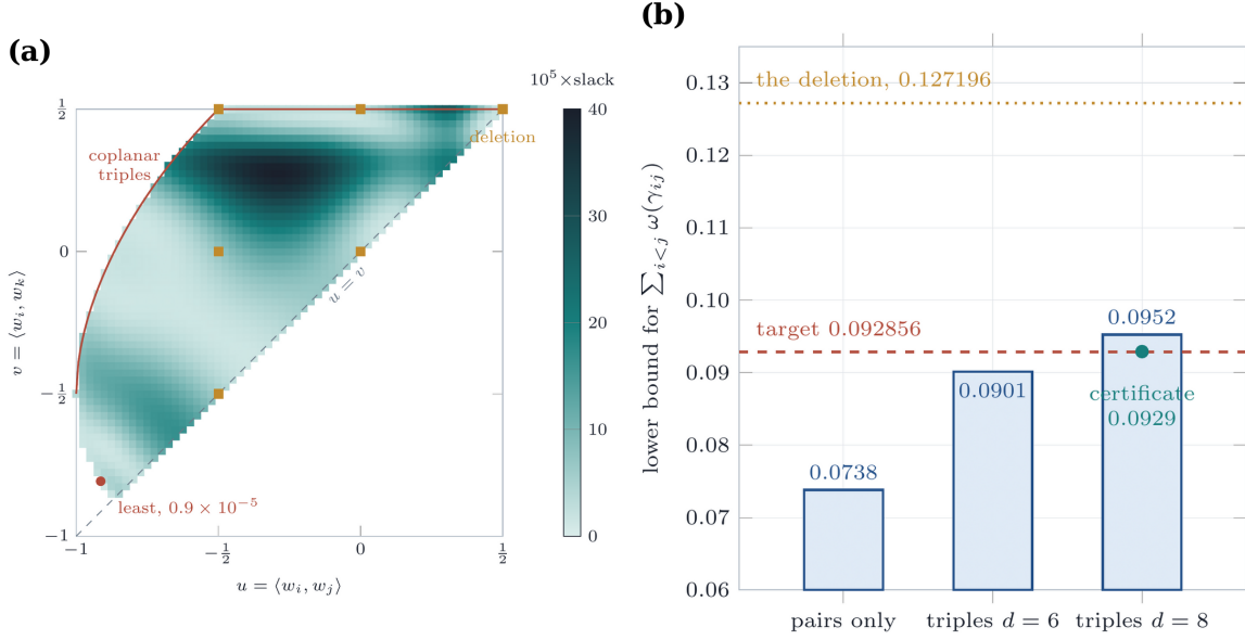
FIGURE 23. (a) The certificate of Theorem 7.73: the slack of the condition (7.48), the amount by which its left-hand side exceeds 0, on the slice of the admissible domain in which one pair of the triple is at 60^\circ . It is positive throughout, least near a coplanar triple with one nearly antipodal pair, and largest, about 4 \times 10^{-4} , in the interior. The six squares are the triples that occur in a deletion of a root. (b) The values of the relaxations against the target 8 - A_* : the pair angles alone (Proposition 7.44), the three-point relaxation at degrees 6 and 8, and the certificate, at which the bound is fixed at 0.0929 and the least slack is maximised.
