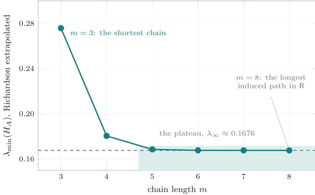
FIGURE 32. Richardson-extrapolated minimum eigenvalue of the joint Hessian H_A for chain configurations of length m = 3, \dots, 8 (Lemma 15.3; full values in Appendix G). The eigenvalue falls sharply from m = 3 to m = 5 and then plateaus near 0.1676 instead of continuing to collapse, which is the antipodal-axis mechanism described below. It stays well clear of zero for every chain length up to m = 8 , the longest induced path in the contact graph of R , so the second-order method certifies positivity on the whole chain family.
