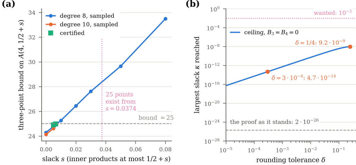
FIGURE 26. The two halves of Theorem 7.25 at positive slack. (a) The three-point bound on the number of points of S^3 with inner products at most \frac{1}{2} + s , from sampled programmes of degree 8 and 10 ( cardinality_sdp.py sweep ; each sampled value is slightly optimistic), with the two certified values of Theorem 7.79 and its companion at s = 0.005 . It crosses 25 near s = 0.009 ; a 25-point code exists from s = 0.0374 on. (b) How far the proof of Theorem 7.76 could be pushed if the triple and quadruple terms cost nothing ( B_3 = B_4 = 0 ): the largest slack \kappa it reaches, against the tolerance \delta that a rounding lemma would allow (Remark 7.78). The curve grows like \delta^2 and stops below 10^{-8} ; the proof as it stands gives 2 \cdot 10^{-26} .
