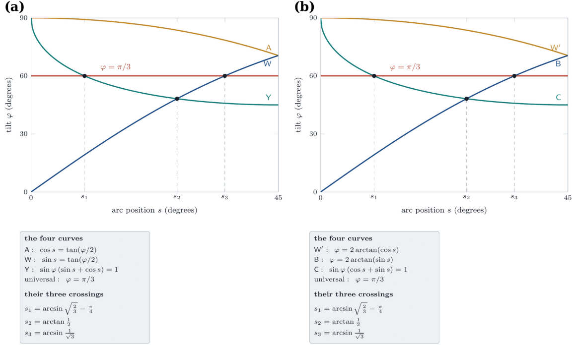
FIGURE 28. (a) The four breakpoint curves of the first arc, drawn to scale from the closed forms of Theorem 9.1: the universal curve \varphi = \pi/3 and the curves A, W, Y. They meet in exactly three points, at the abscissae s_1 , s_2 , s_3 listed at the right, and the eight combinatorial regions of Section 10.2 are the cells of the resulting arrangement. The curves A and W meet only at s = \pi/4 , where the reflection symmetry of the arc identifies them. (b) The four breakpoint curves of the second arc, drawn to scale from the closed forms of Theorem 11.1. Comparing with Figure 28(a) shows what Proposition 8.5 later proves: the three equations here are exactly those of A, W and Y on the first arc, and the arrangement, crossings included, is the same one, even though the curves come from different vertices of \mathcal{V} . The band immediately below region top splits into three sub-parts at the crossings s_1 , s_2 , s_3 .
