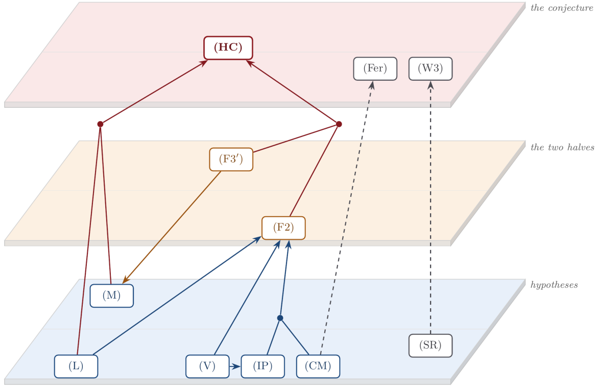
FIGURE 1. The routes of Theorem D. Hypotheses lie on the bottom layer, the two halves (F2) and (F3') in the middle, and (HC) on top. Arrows are implications of Table 1. At each dot two lines combine into a conjunction: (CM) \wedge (IP) \Rightarrow (F2) , (L) \wedge (M) \Rightarrow (HC) and (F2) \wedge (F3') \Rightarrow (HC) . The arrows from (HC) and (F2) to the statements they contain are not drawn. The dashed arrows on the right lead to the special cases (Fer) and (W3) of Section 7, and not to (HC).
