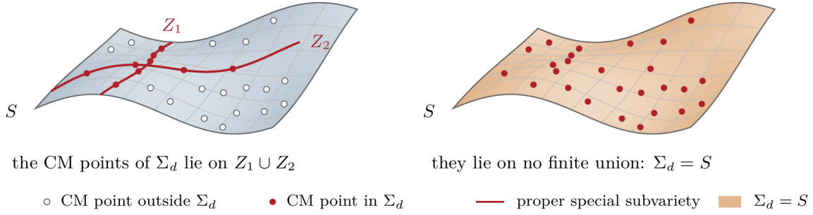
FIGURE 3. The criterion of Theorem F, drawn schematically ( S has dimension n^2 ). CM points are dense in S . On the left the CM points of \Sigma_d lie on two proper special subvarieties Z_1 and Z_2 , and condition (iii) fails for this d . On the right they lie on no finite union of proper special subvarieties; by the André–Oort theorem their Zariski closure is then S , and \Sigma_d = S .
