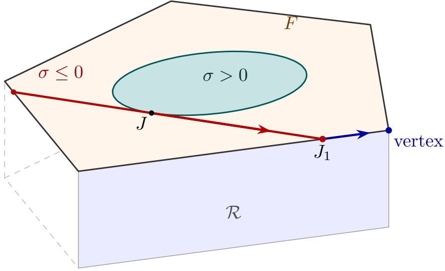
FIGURE 3.1. One step of the proof of Proposition 3.2 in a two-dimensional face F of \mathcal{R} , the case \sigma(J) = 0 . The set F \cap \{\sigma > 0\} (shaded) is convex because \sigma is concave. On the line through J in the direction X , chosen with X[u] = 0 , we have \sigma \leq 0 , and \log \det Q is concave on it, so one of the two ends of the chord, here J_1 , has \det Q(J_1) \leq \det Q(J) . The point J_1 lies on an edge of F . From there the same step moves along the edge to a vertex or to a point with \sigma = 0 .
