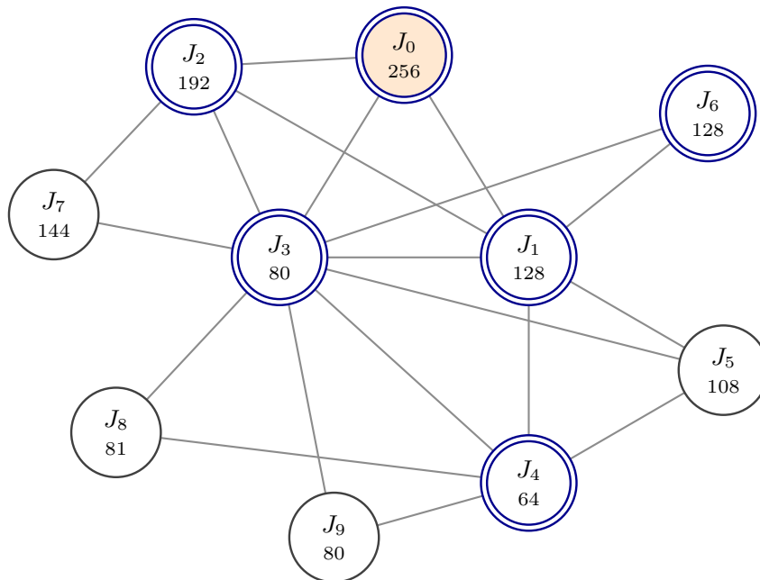
FIGURE 6.1. The ten classes of vertices of \mathcal{R} , labelled with \det Q , and the edges between different classes (Table 5.2). The classes of J_1 , J_3 and J_4 also have edges joining two vertices of the same class. Double circles mark the classes with unbounded edges. The packings of maximal density are the vertex J_0 and a point on an unbounded edge at J_1 .
