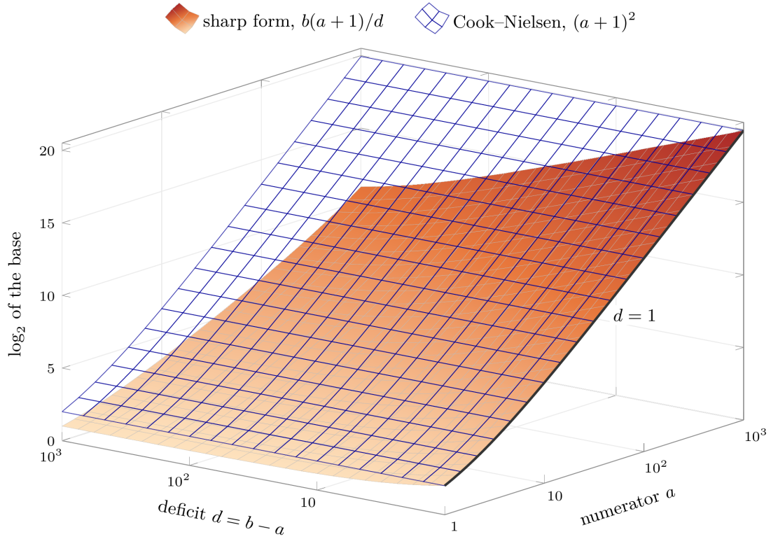
FIGURE 11. The base of the bound for aX_m written as E_{m-1}(\cdot) , on a \log_2 scale, over the numerator a and the deficit d = b - a . The wire mesh is the base (a + 1)^2 of the lemma of Cook and Nielsen, the shaded sheet below it the base b(a + 1)/d of Theorem 6.2. They meet along d = 1 , where the two bounds coincide, and separate as d grows.
