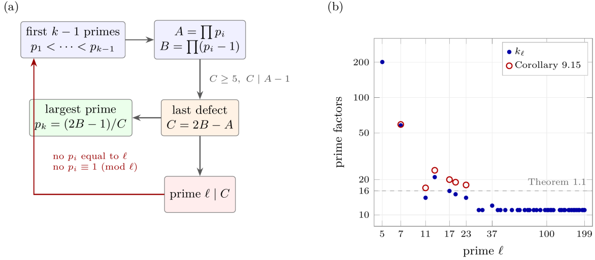
FIGURE 21. (a) The first k-1 prime factors of a solution of n-1 = 2\varphi(n) determine A , B and the last defect C , and C determines the largest prime factor. A prime \ell dividing C excludes \ell and the class 1 modulo \ell from the first k-1 prime factors (Lemma 9.12). (b) The least number k_\ell of prime factors that this exclusion allows, for the primes \ell \leq 199 (Proposition 9.13), and the larger lower bounds of Corollary 9.15 (open circles). The dashed line is the bound \omega(n) \geq 16 of Theorem 1.1.
