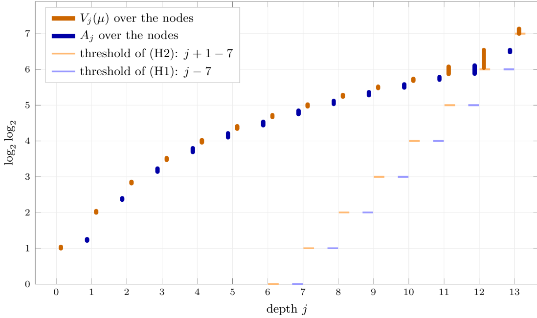
FIGURE 13. The nodes of \mathcal{T}_7 by depth j . The bars span the range of \log_2 \log_2 V_j(\mu) (right of each depth) and of \log_2 \log_2 A_j (left of each depth) over the nodes of depth j , and the short marks below them are the thresholds j + 1 - 7 of (H2) and j - 7 of (H1). The deficit condition (H2) is the one that binds: at depth 13 the smallest value of \log_2 \log_2 V_{13} is 7.0000075\dots
