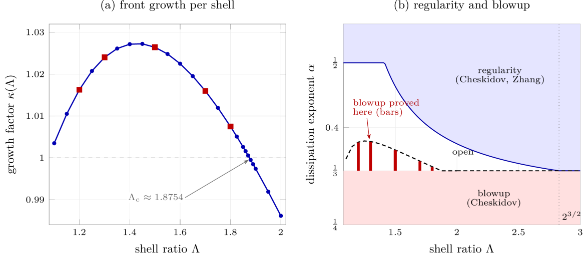
Figure 2: (a) The growth factor \kappa(\Lambda) of the self-similar front (Table 4); squares mark the five verified ratios. (b) Known results in the (\Lambda, \alpha) plane: blowup for \alpha < 1/3 [10]; regularity above \min\{1/2, \max\{1/3, 1/4 + \log 2/(8 \log \Lambda)\}\} [10, 9]; the bars are the ranges [1/3, \alpha_\Lambda] proved here, and the dashed curve is \max\{1/3, \alpha^*(\Lambda)\} .
