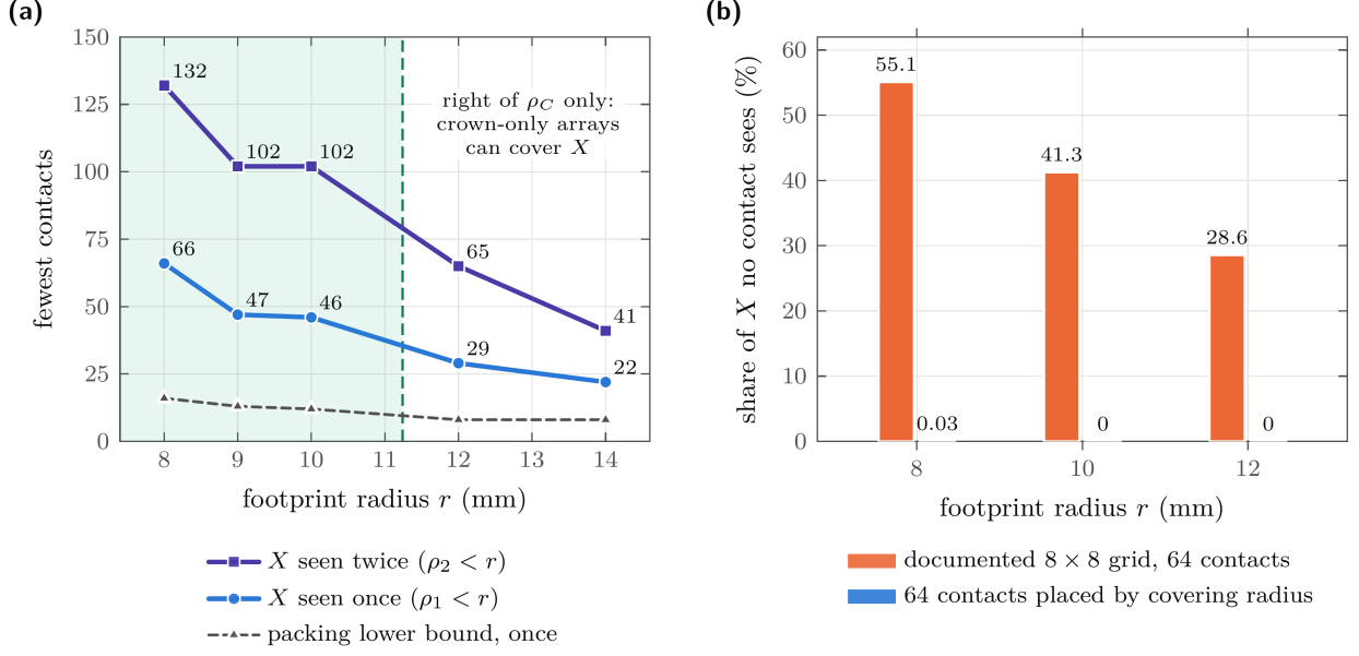
FIGURE 7. (a) Fewest contacts of the farthest-point sequence that see all of X once (blue) and twice (violet), against the packing lower bound for single coverage (grey). Left of the crown floor (shaded) no array with contacts on the crowns sees all of X at any count. (b) The share of X that no contact sees, for the documented 8 \times 8 grid and for the same 64 contacts placed by covering radius.
