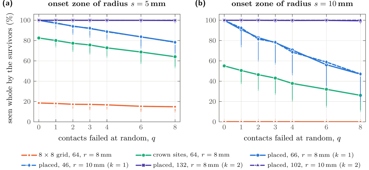
FIGURE 9. Onset zones still seen whole when q contacts fail at random, for onset zones of radius (a) 5 mm and (b) 10 mm. Lines are means over 100 random failure sets for each q ; whiskers reach down to the 5th percentile. Single-coverage designs ( k = 1 , blue) degrade with every failure; double-coverage designs ( k = 2 , violet) stay near 100% through eight failures. The uniform failure model is an assumption; failures clustered in space would be harder on every design.
