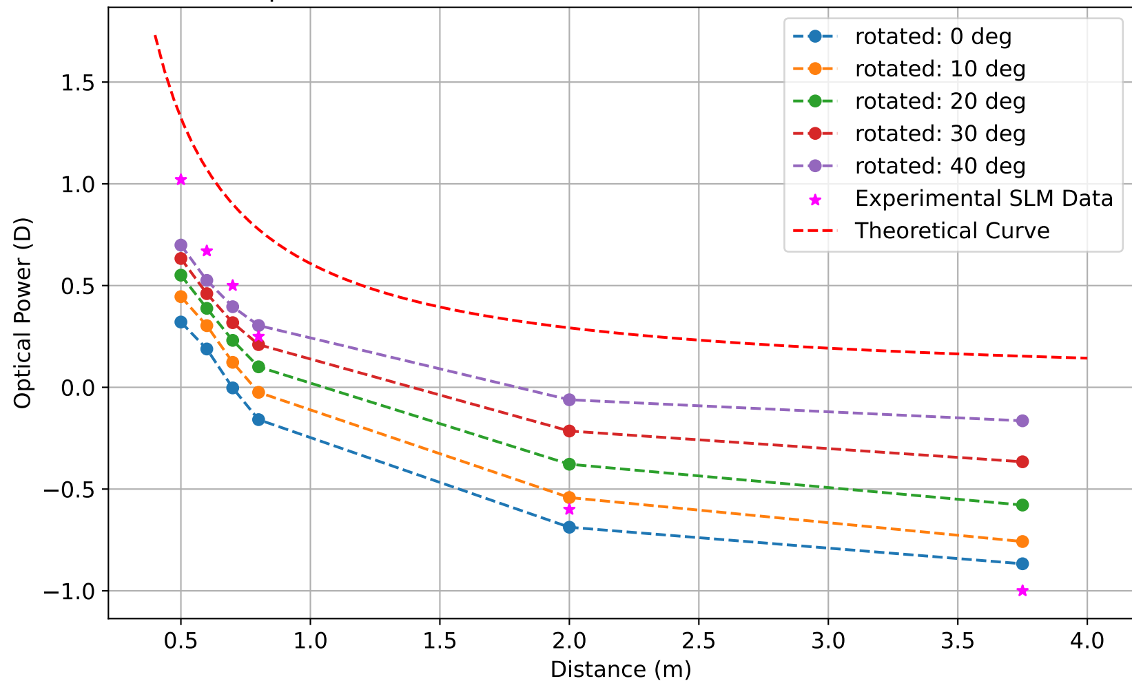
Optical Power vs Distance for Rotated SLM around axis z
