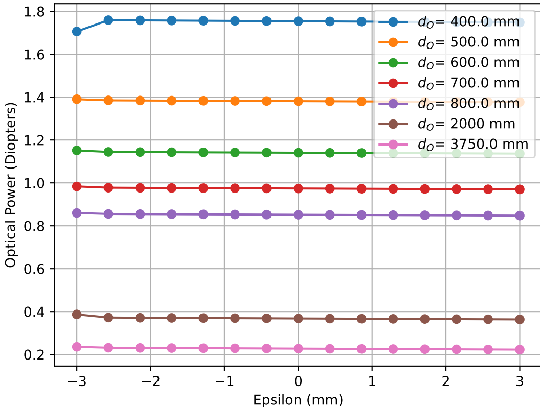
Lens L_2 to L_3
