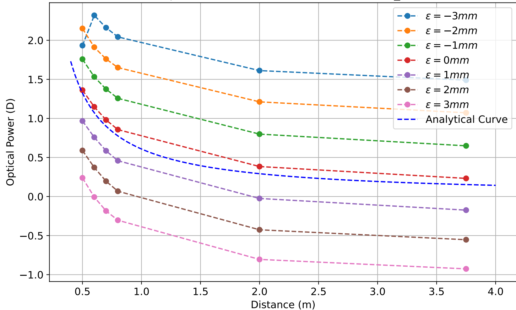
Optical Power vs Distance for Shifted L c
