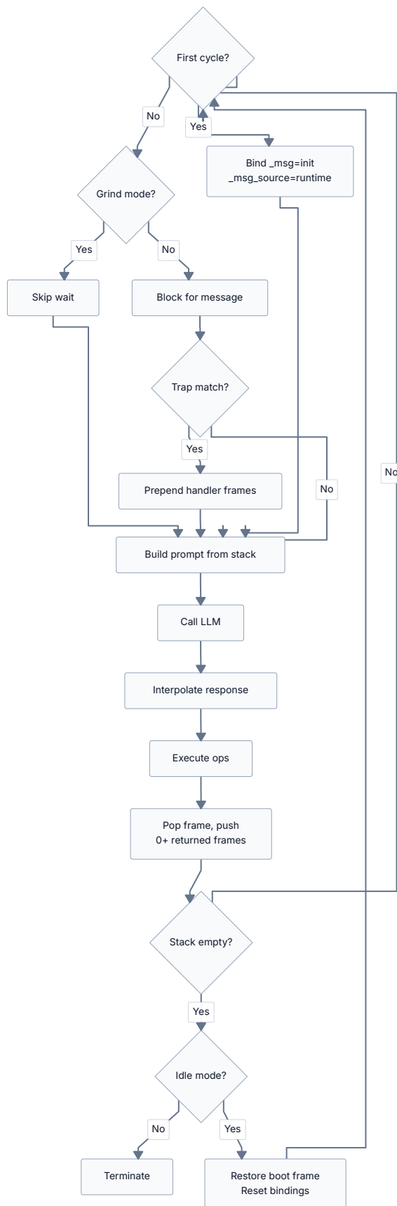
Figure 1: The eval cycle
