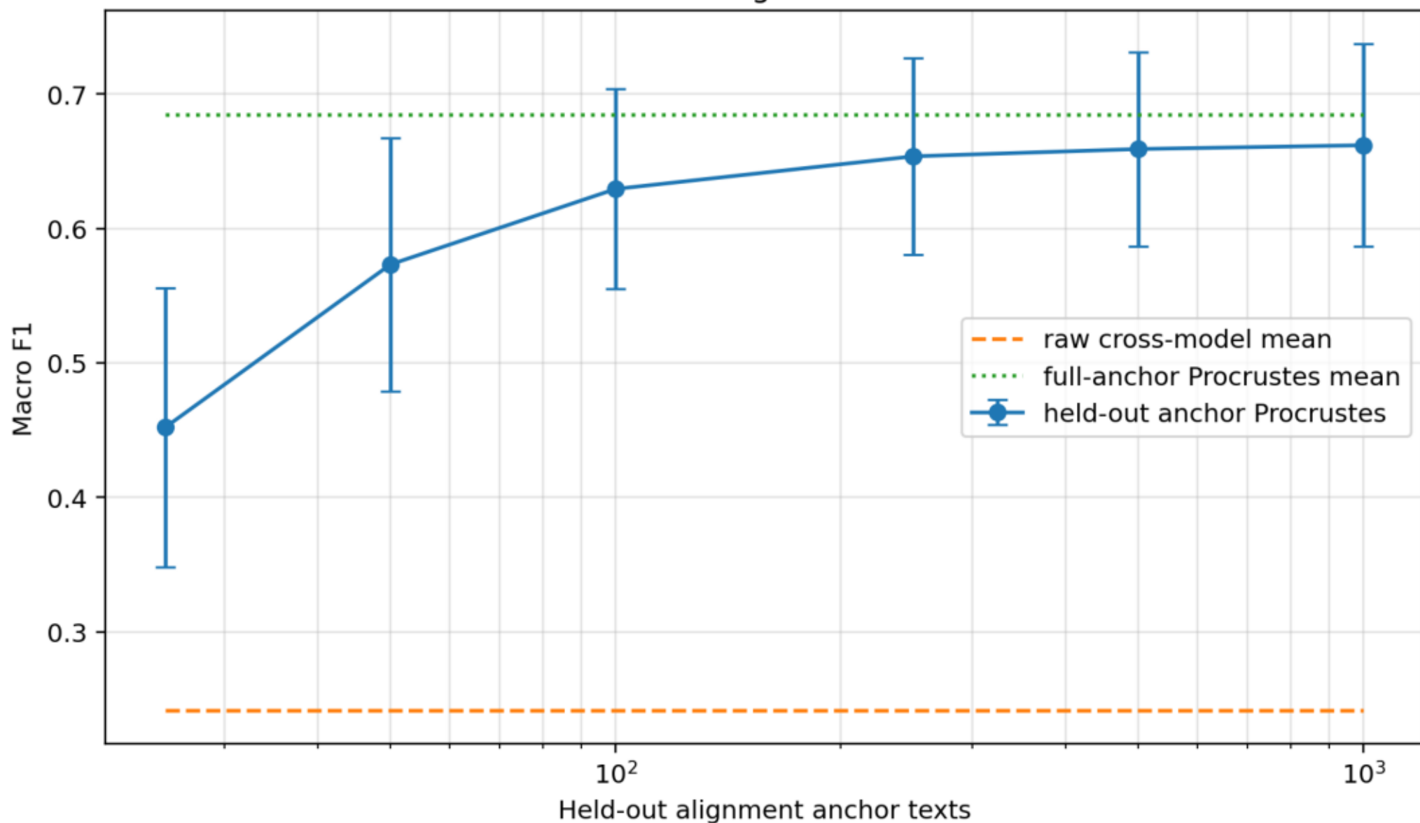
UPAT held-out alignment-size curve
