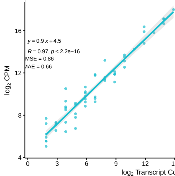
PCR-cDNA
