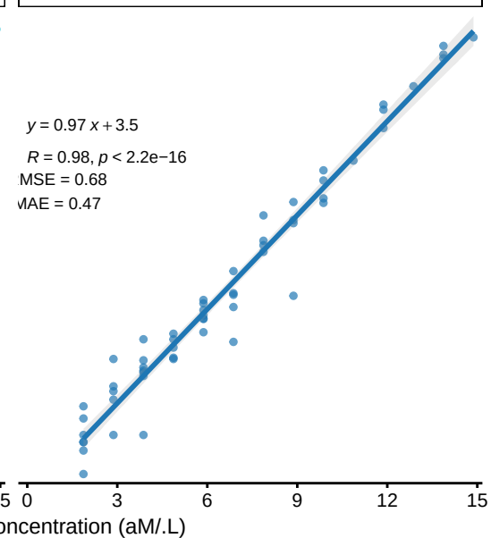
Direct RNA
