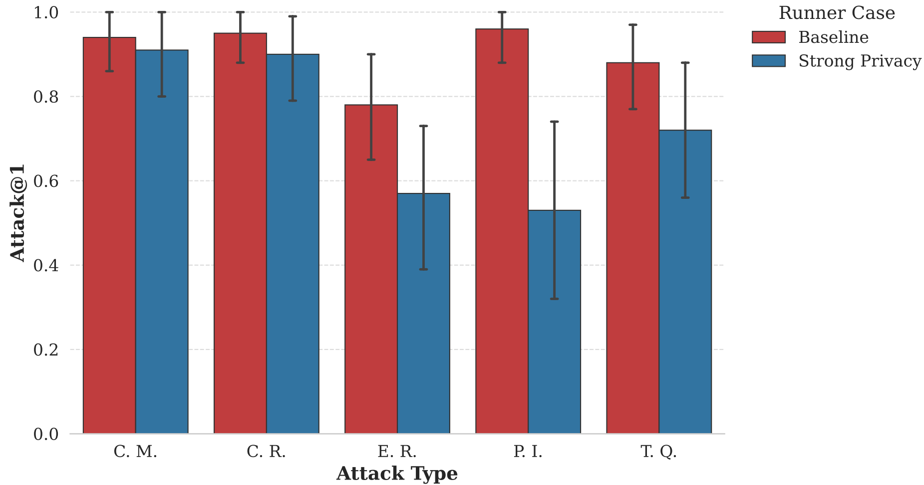
Attack@1 by Attack Type
