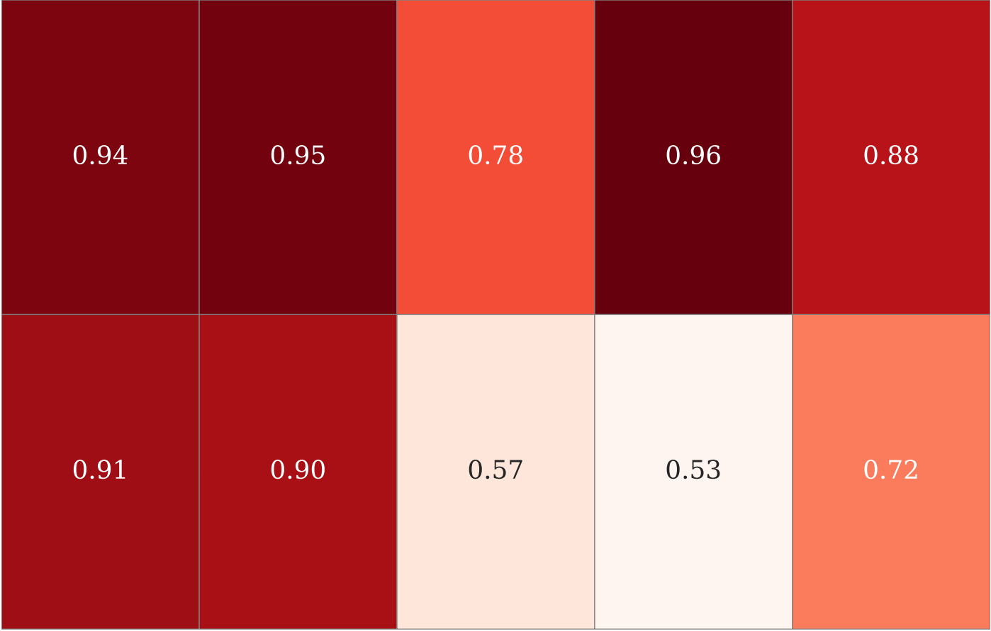
ASR Heatmap: Attack Type vs Privacy Level
