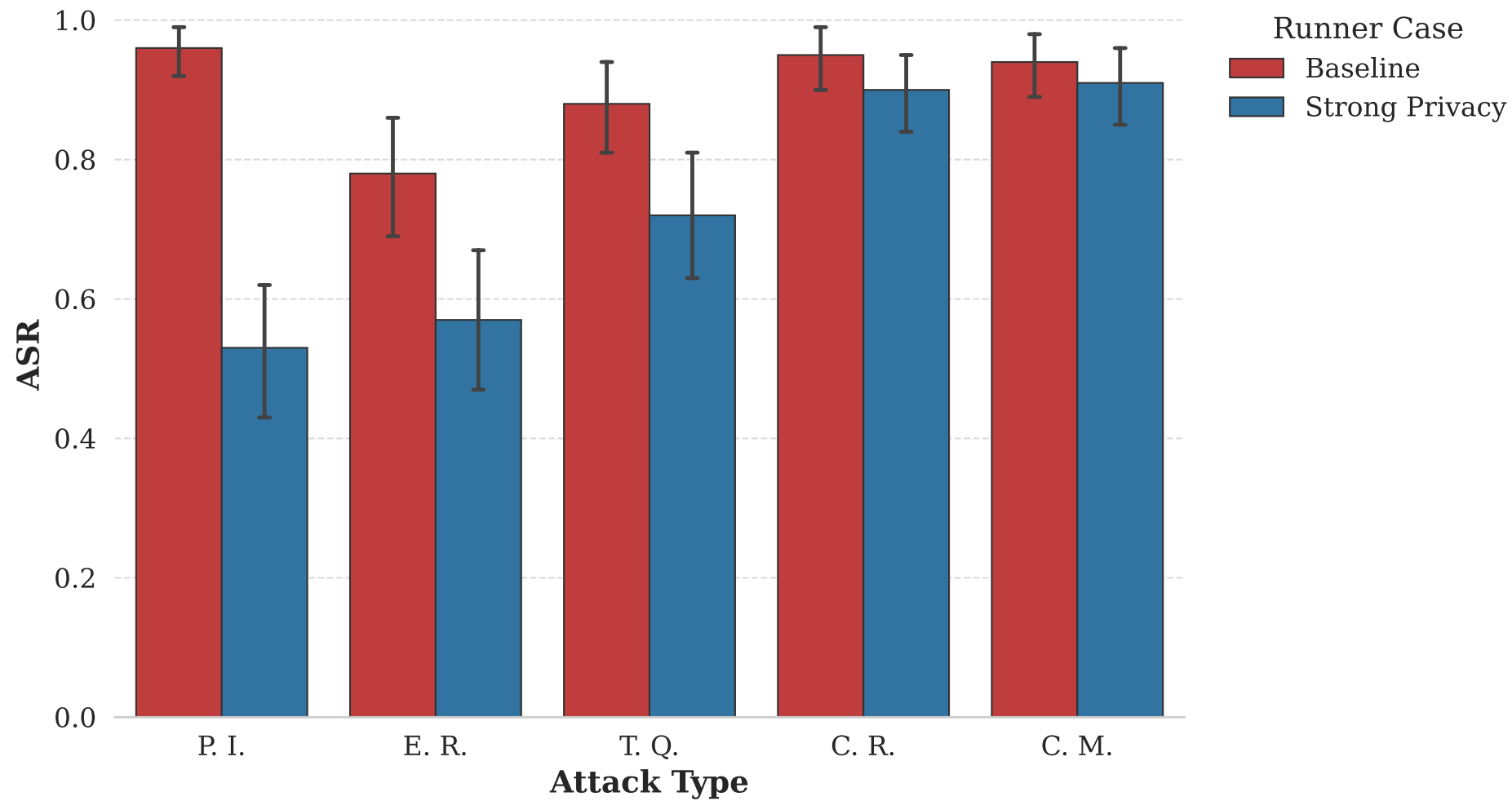
ASR by Attack Type
