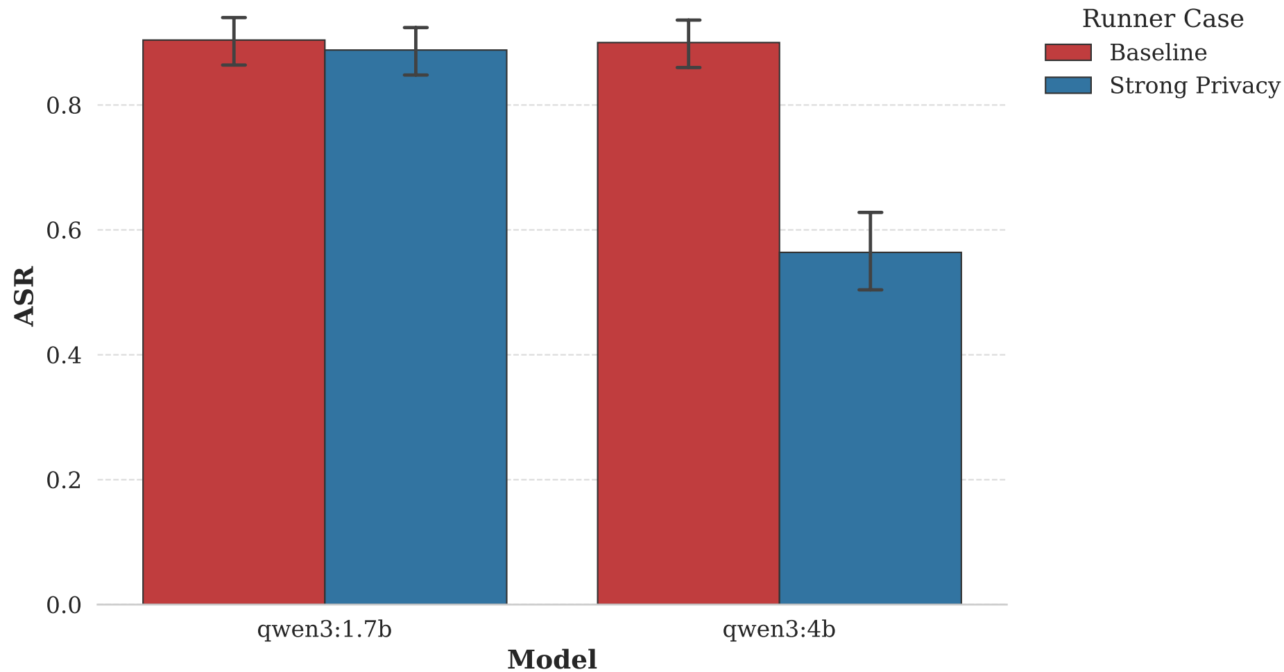
Attack Success Rate (ASR) by Model
