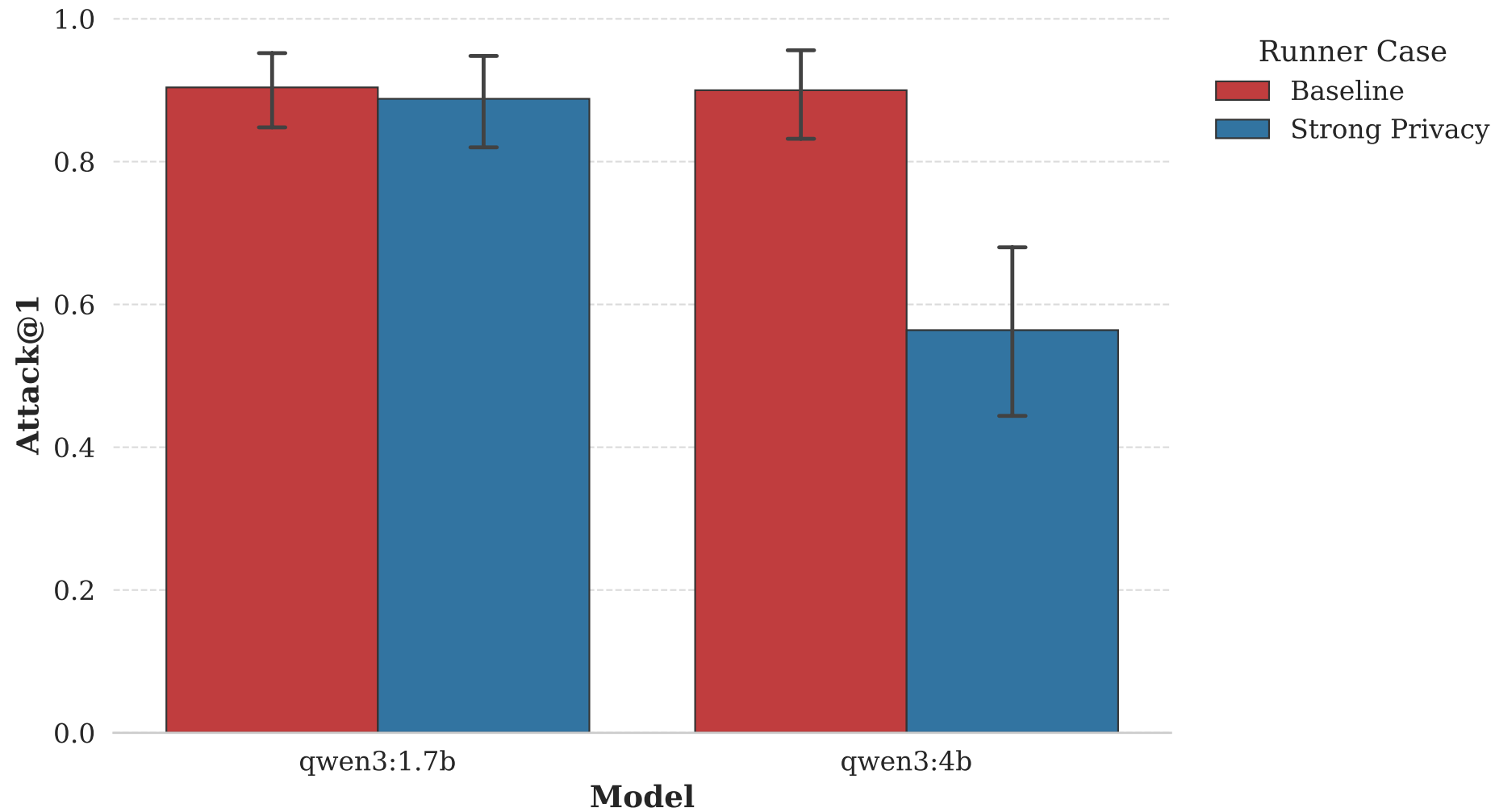
Attack@1 Probability by Model
