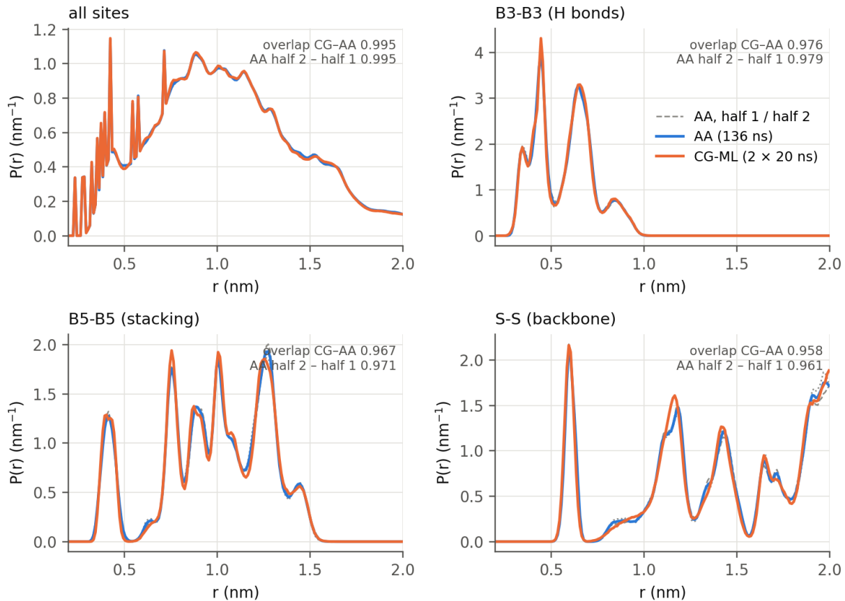
Figure 2. Intramolecular P(r) per channel. Blue: AA over 136 ns; orange: CG-ML over 2 \times 20 ns; grey dashed and dotted: first and second half of the AA. Top right: the CG-AA overlap and the ceiling (half 2 vs half 1).
