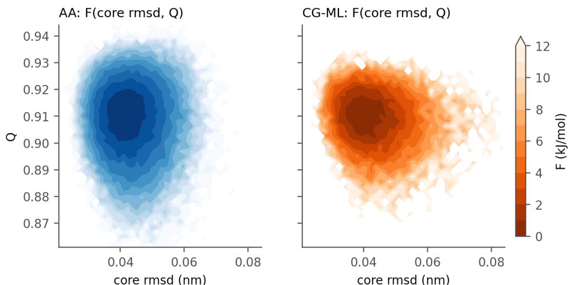
Figure 6. Free energy F = -kT \ln p(\text{core rmsd}, Q) , AA and CG-ML. The JSD between the FES (script 46) is 0.0787, equal to the AA vs AA ceiling (0.0786); the CG is noisier because of the smaller number of frames (20 080 vs 67 880 copy-frames).
