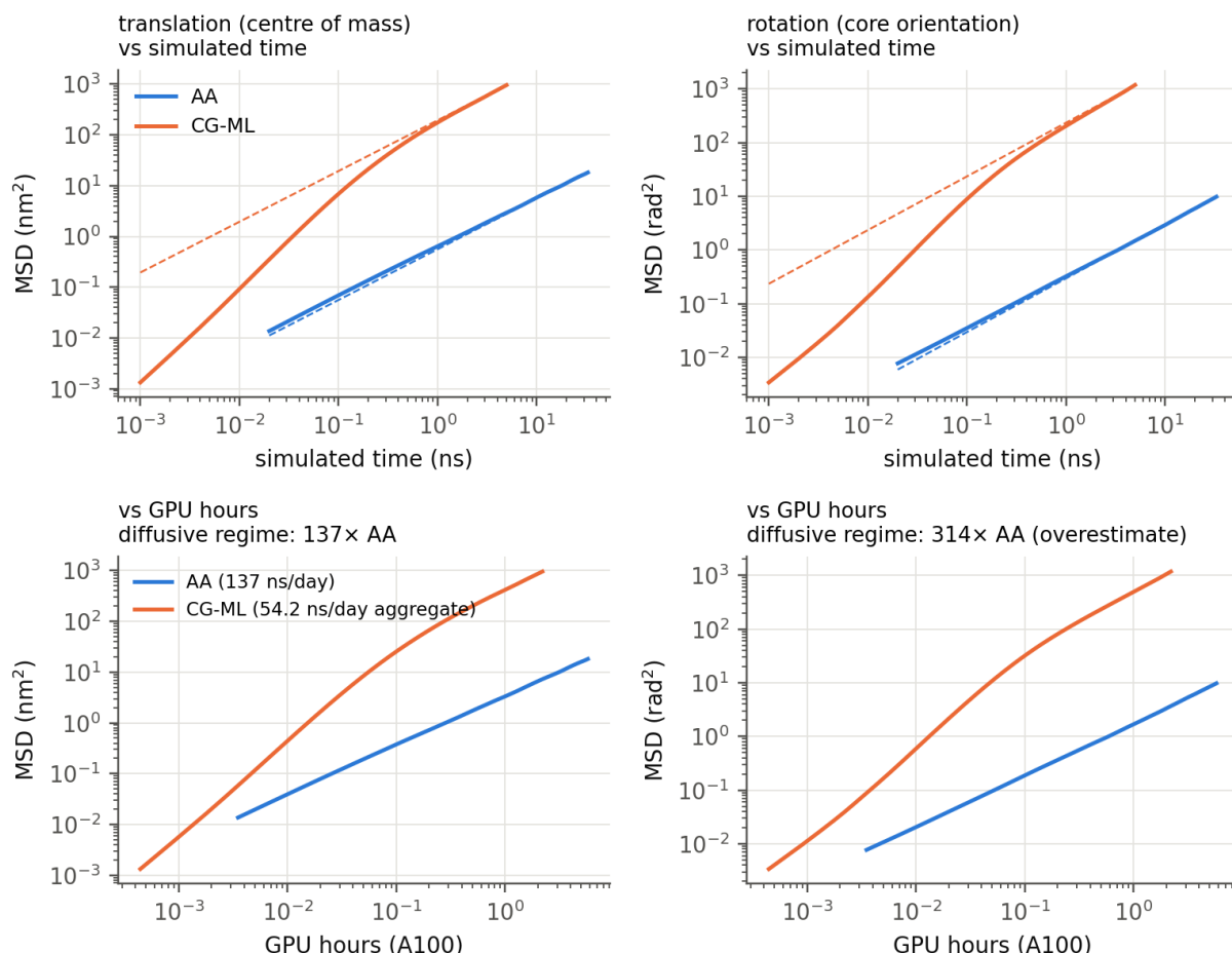
Figure 7. Top: MSD vs simulated time; dashed 6Dt with D from the linear regime. Bottom: the same curves vs A100 GPU hours (AA 137 ns/day; CG-ML 54.2 ns/day aggregate over 2 replicas).
