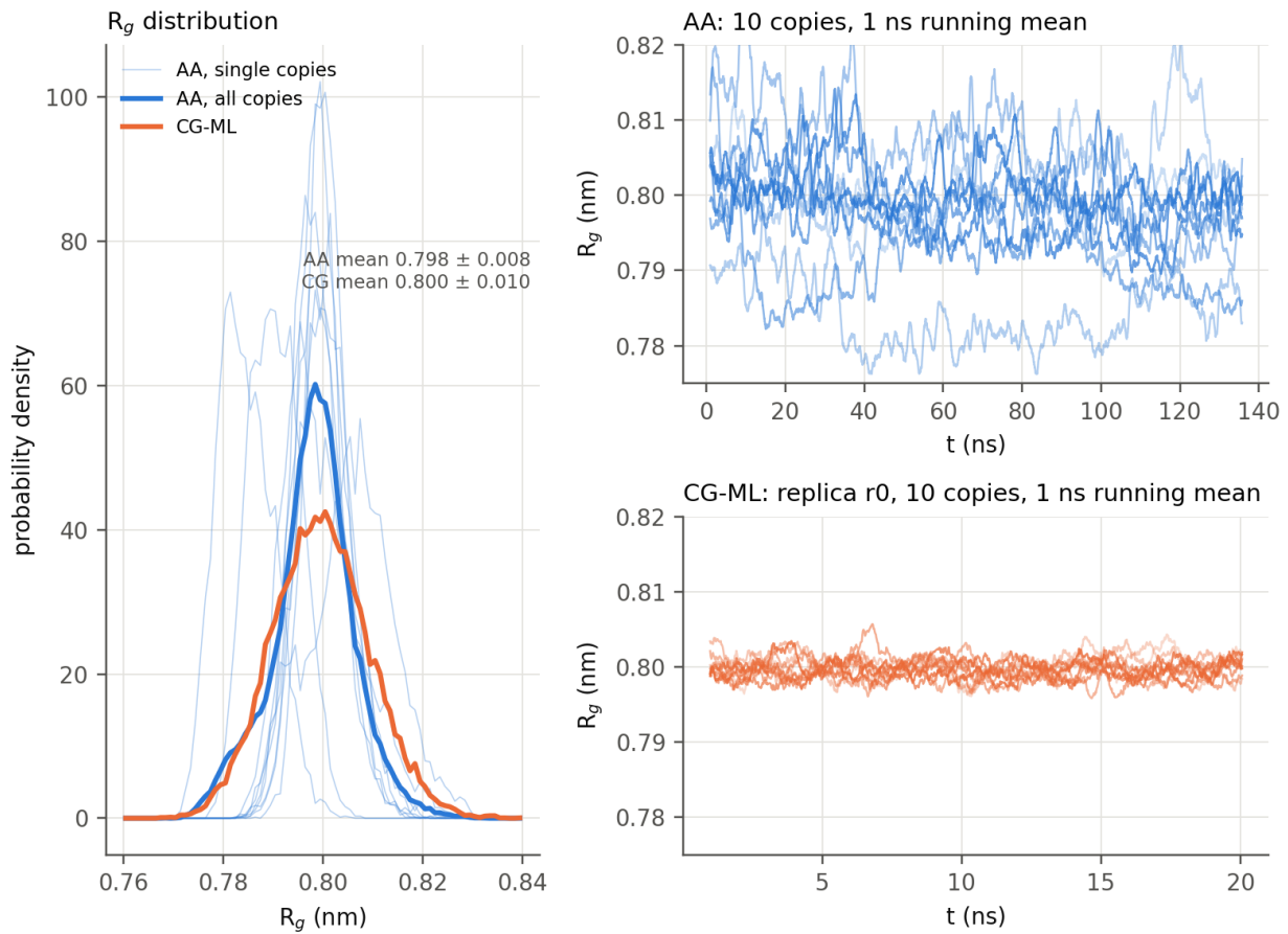
Figure 4. Left: R_g distribution (AA: single copies as thin lines, all copies as a thick line; CG-ML: all copies and replicas). Right: time series with a 1 ns running mean, AA over 136 ns and CG-ML (replica r0) over 20 ns, same vertical scale.
