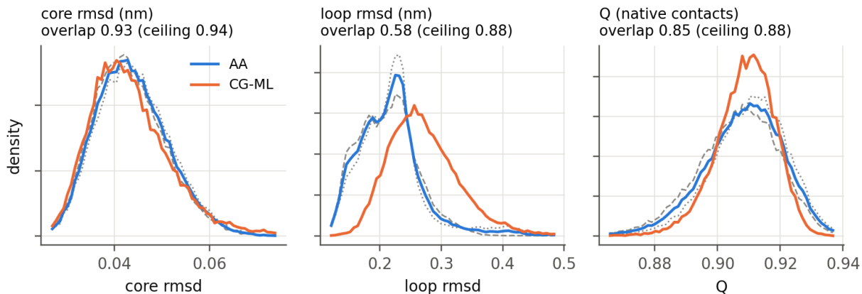
Figure 5. Distributions of core rmsd, loop rmsd and fraction of native contacts Q (grey: AA halves). The titles report the CG-AA overlap and the ceiling.
