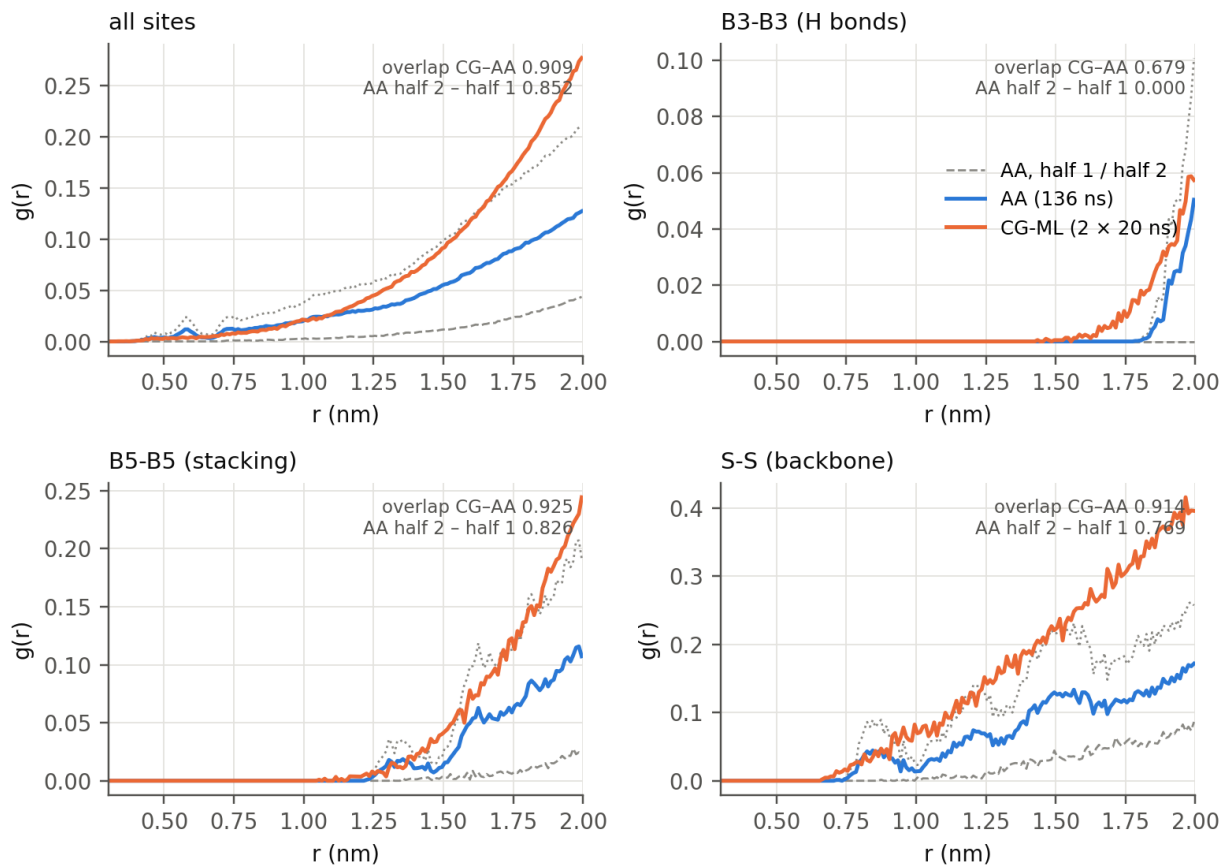
Figure 3. g(r) between sites of different copies, same colours as figure 2. The two AA halves differ by a factor of \sim 5 : the encounters between copies in the AA are few long events.
