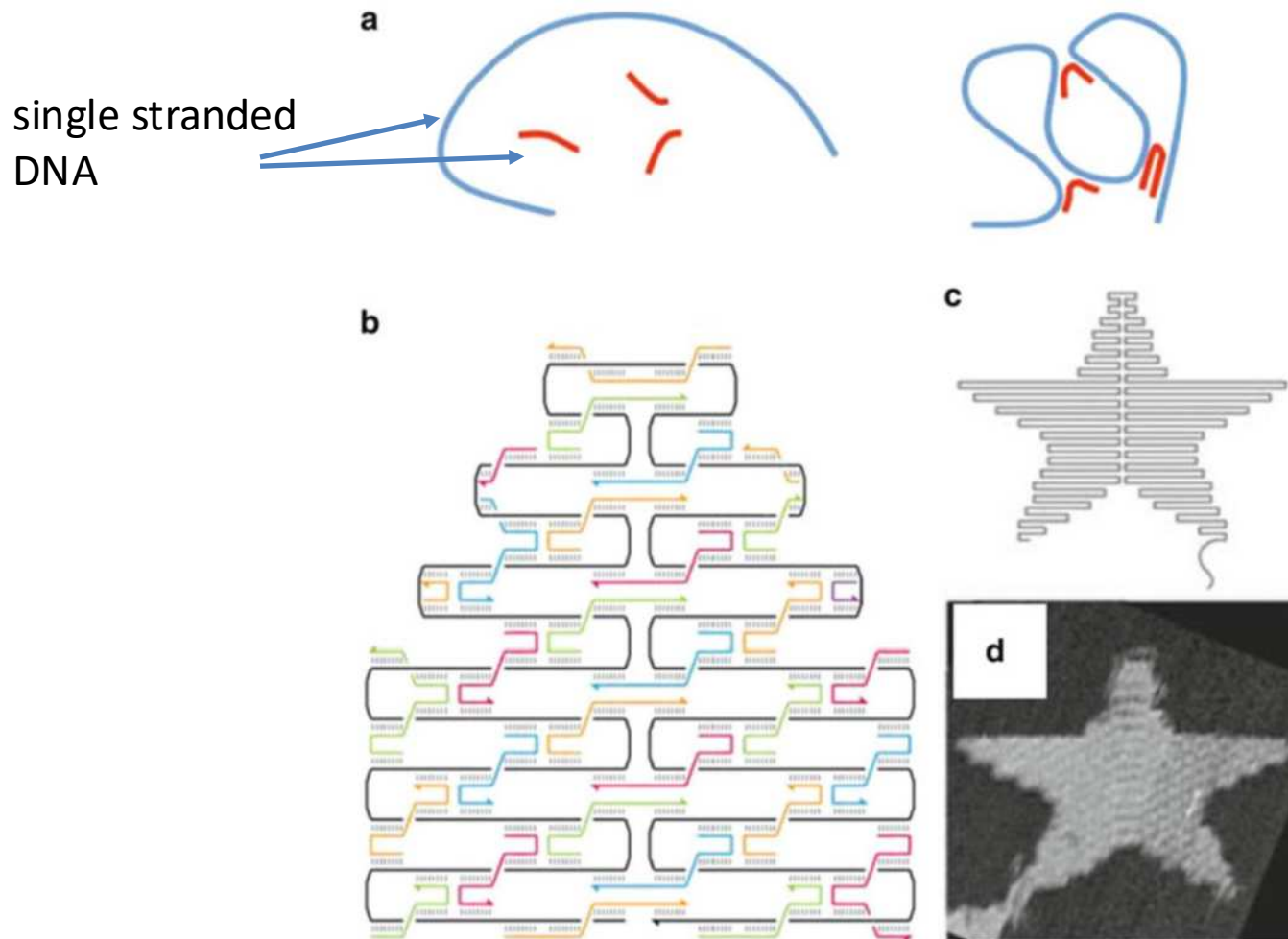
a) Sketch of the basic idea of DNA origami: a long strand is “stapled” by oligonucleotides complementary to specific tracts along its sequence and is folded into designed shapes (b) , as complex as a star (c) . (d) AFM image of the experimental realization of (c) (edge size is 165 \mu\text{m} ).
