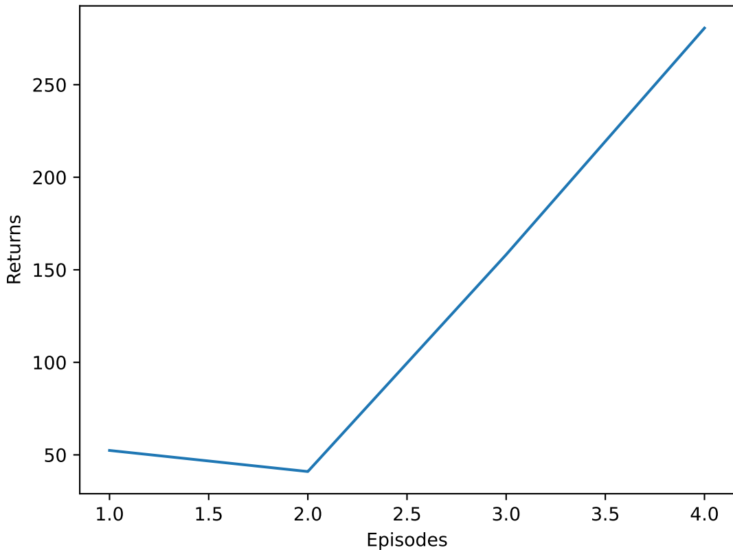
CartPole-v0 (GRPO)
