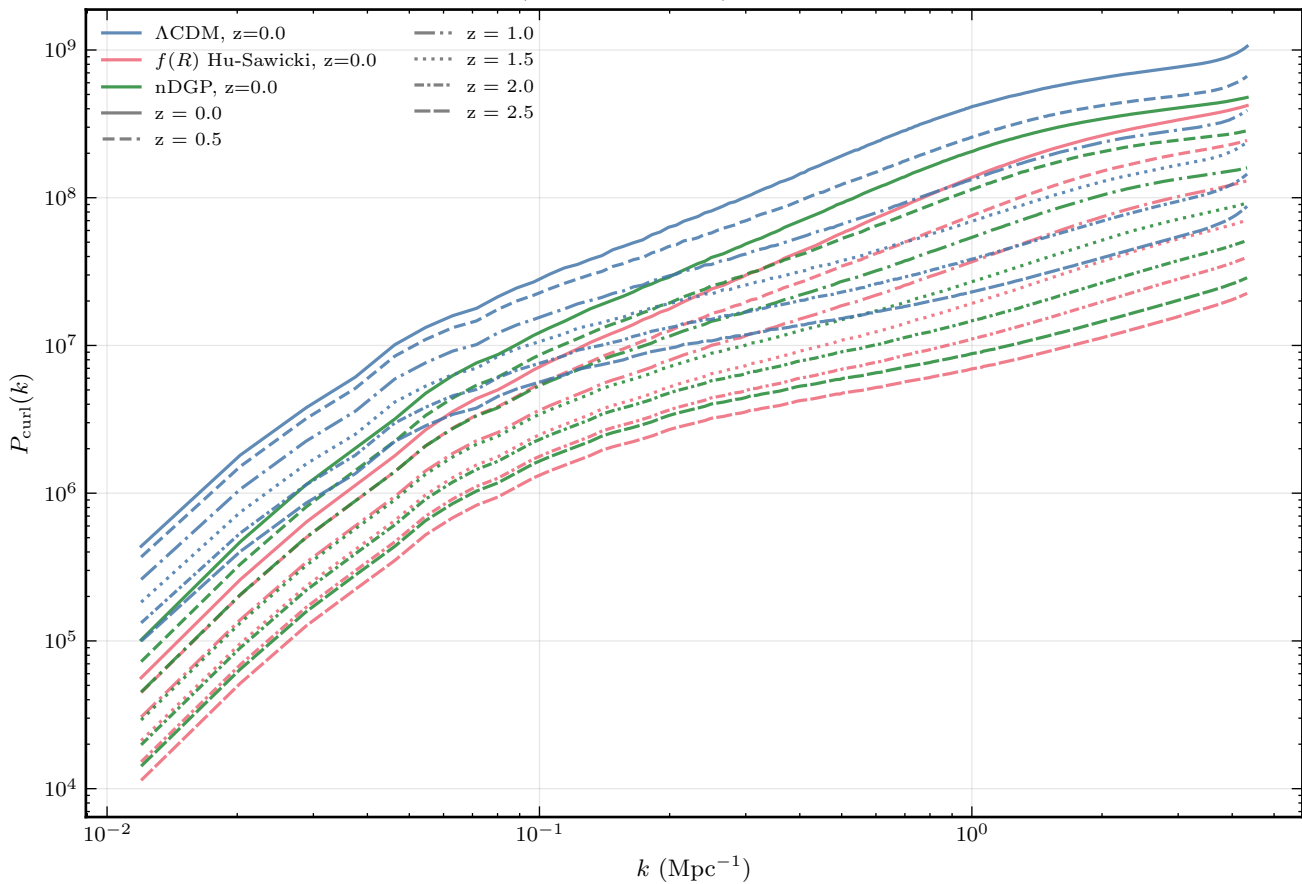
Curl (Gravitomagnetic) Power Spectrum
