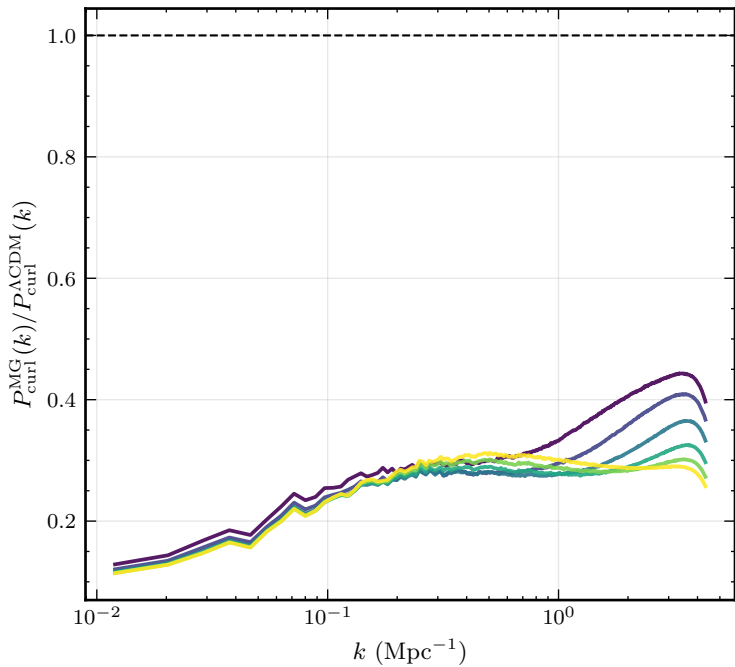
f(R) Hu-Sawicki / \Lambda CDM
