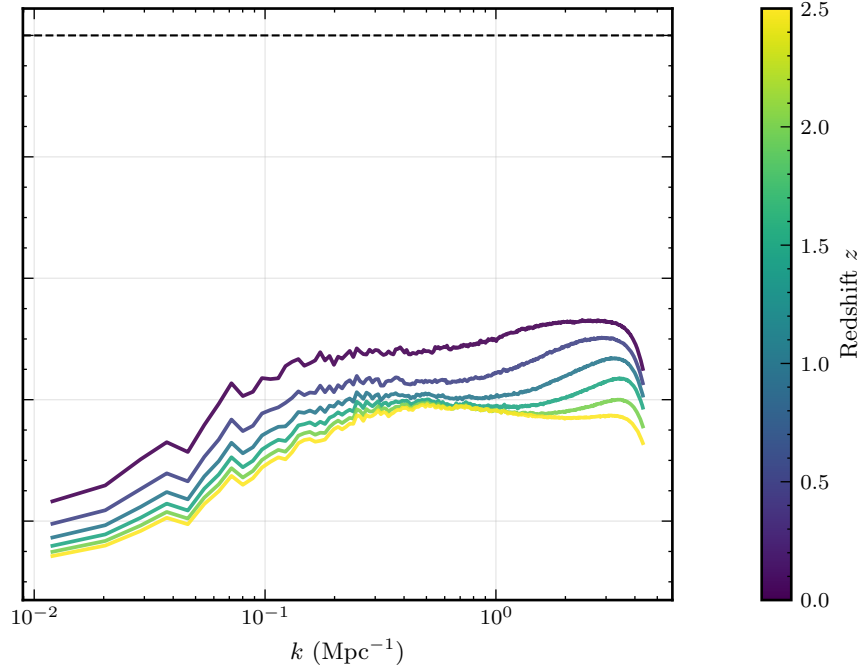
nDGP / \Lambda CDM
