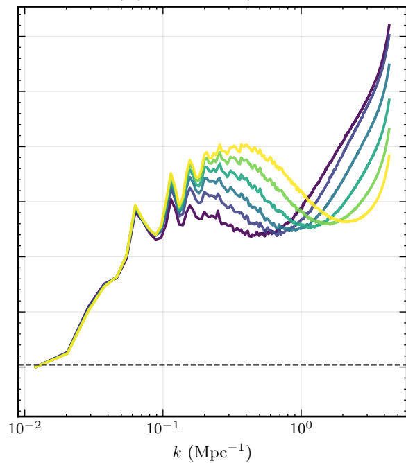
f(R) Hu-Sawicki / \Lambda CDM
