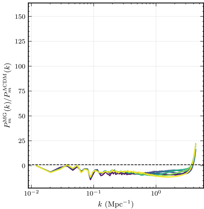
\Lambda CDM / \Lambda CDM
