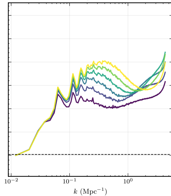
nDGP / \Lambda CDM
