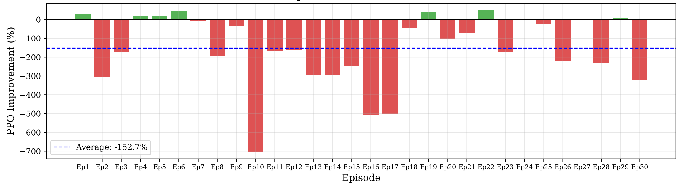
Percentage Error Reduction with PPO (v1)
