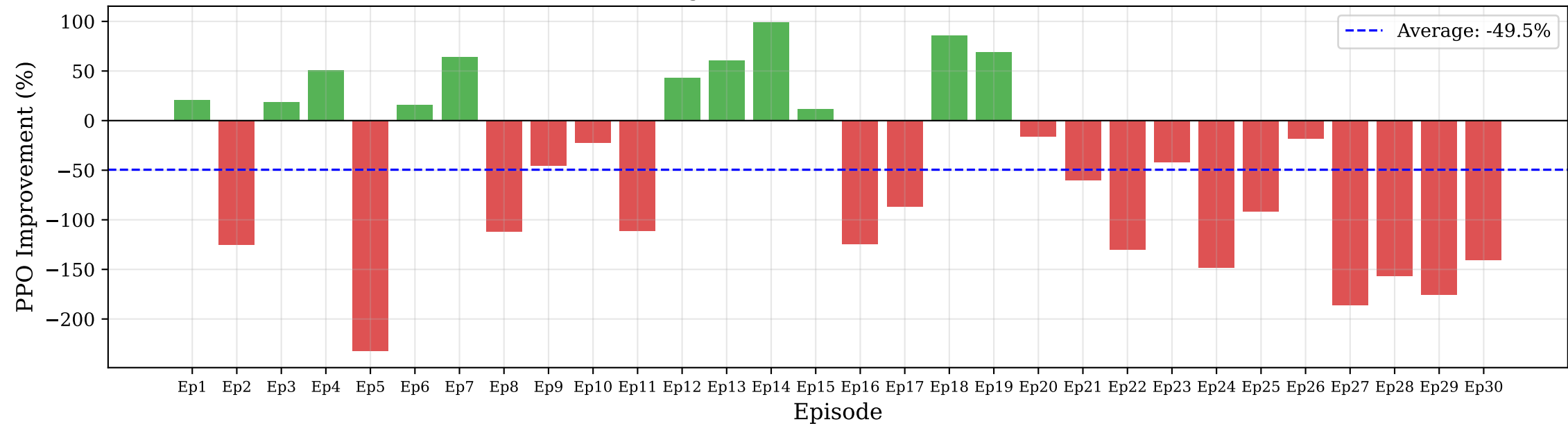
Percentage Error Reduction with PPO (v2)
