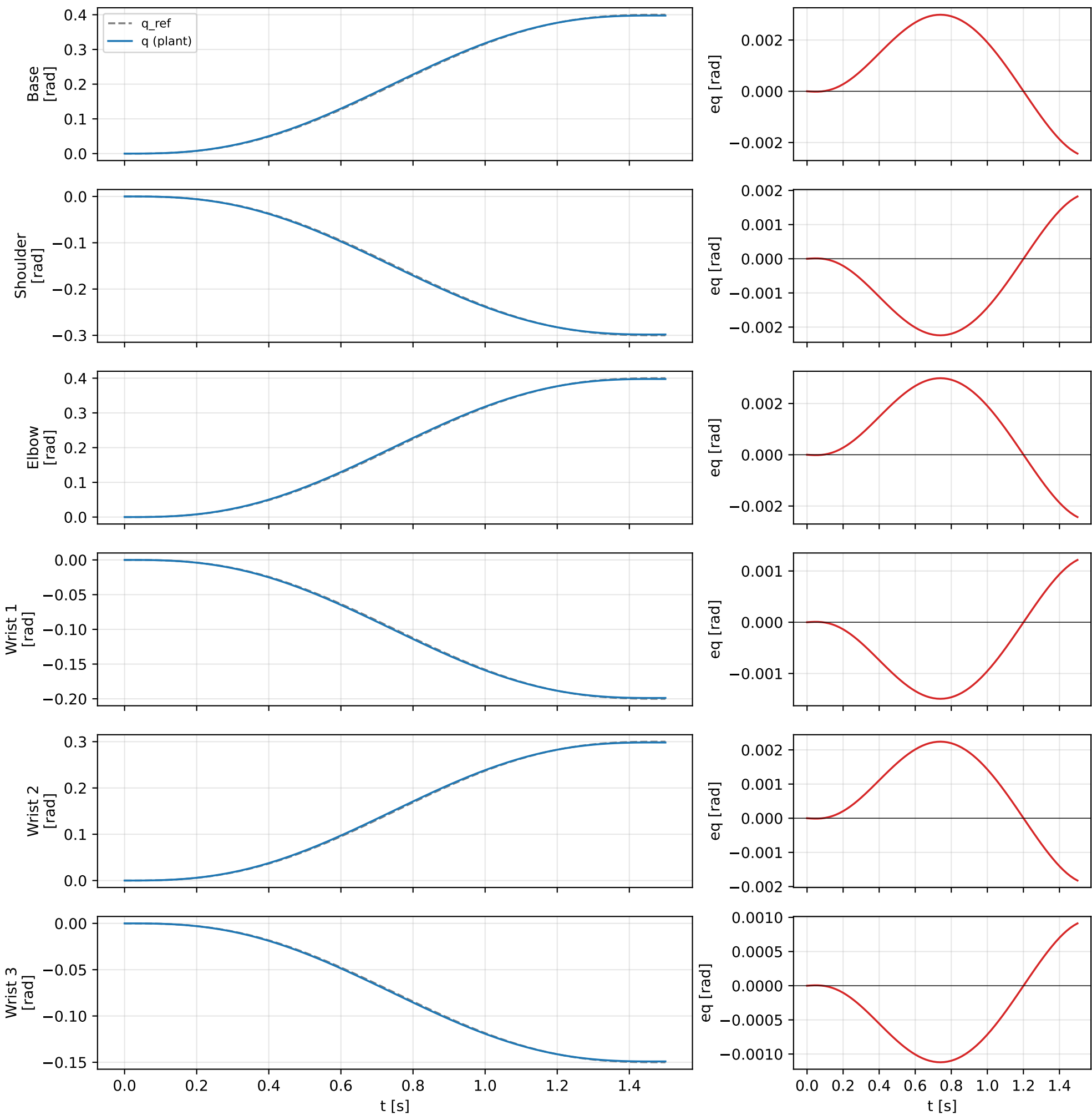
Exp 4 — Target A (moderate) (LQR baseline)
