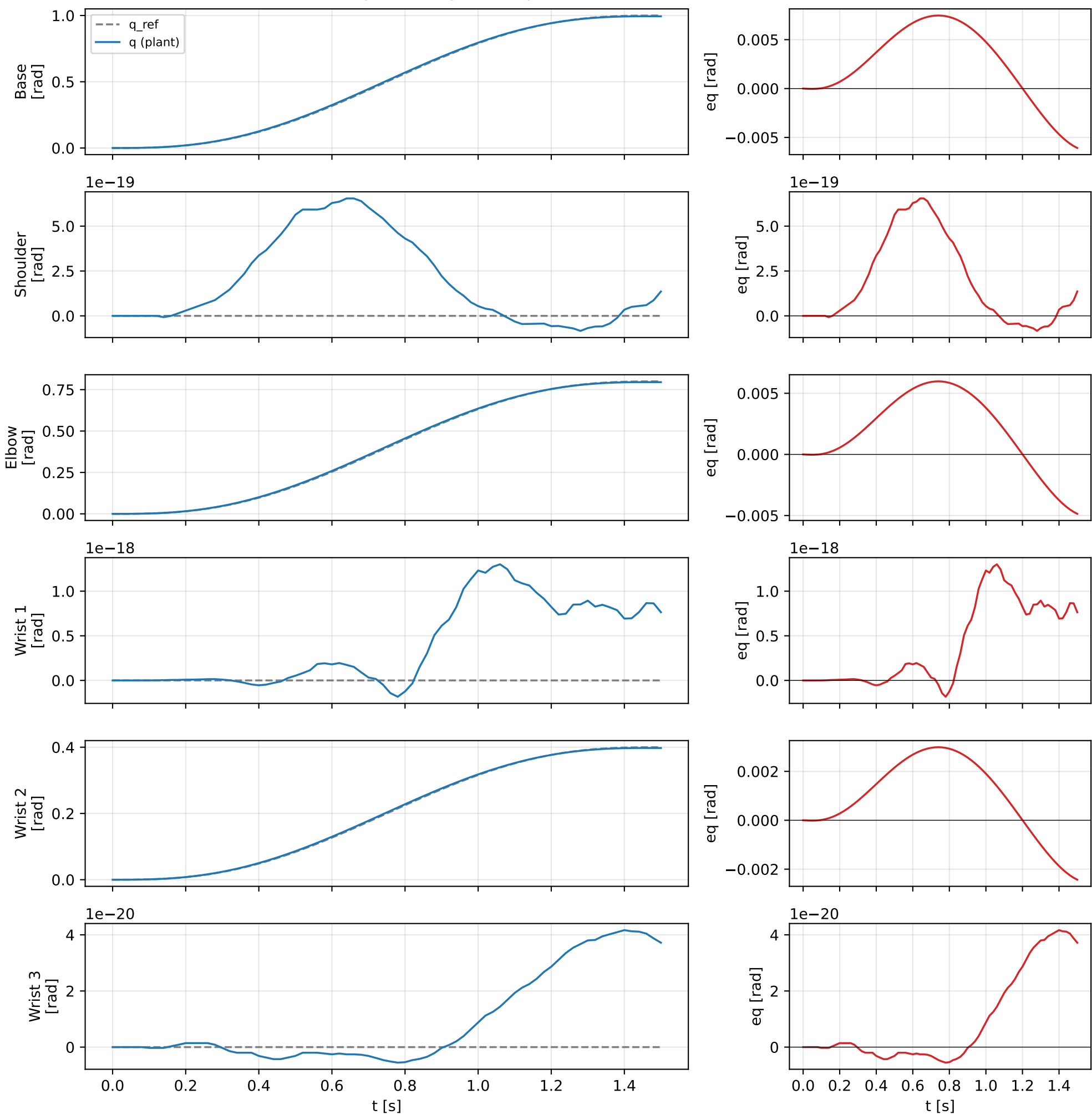
Exp 4 — Target B (asymmetric) (LQR baseline)
